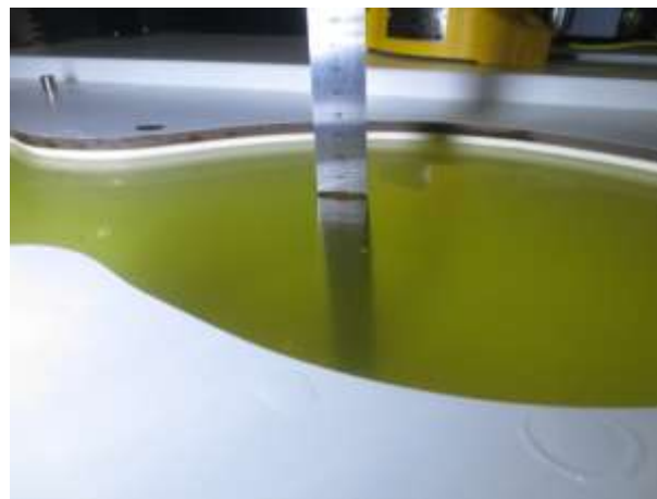
Fig. 9.2 Photo of Liquid Height for Body SAR (700MHz~1000MHz)(depth>15cm)
