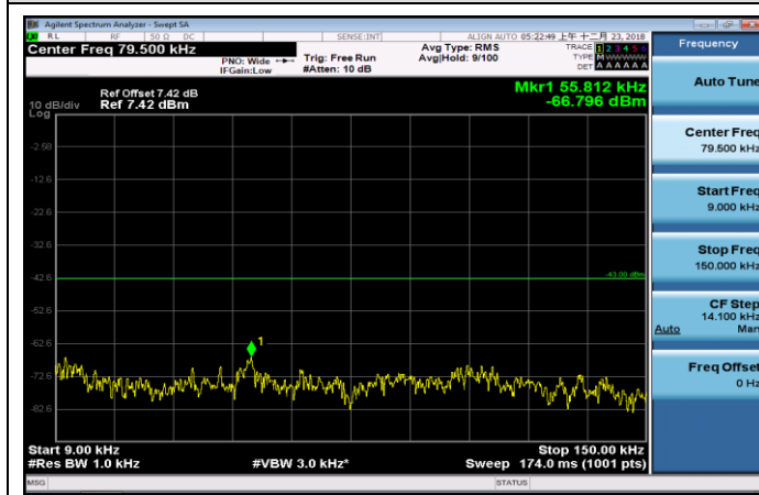
1.4MHz_LCH_QPSK_1RB#0
