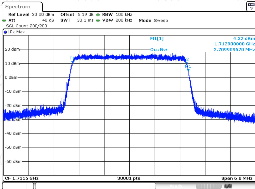
Band4 QPSK BW=3MHz Channel=19965 RB Size=15 Position=#0
