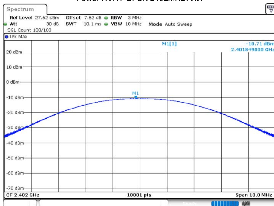
Power NVNT GFSK 2402MHz Ant1
