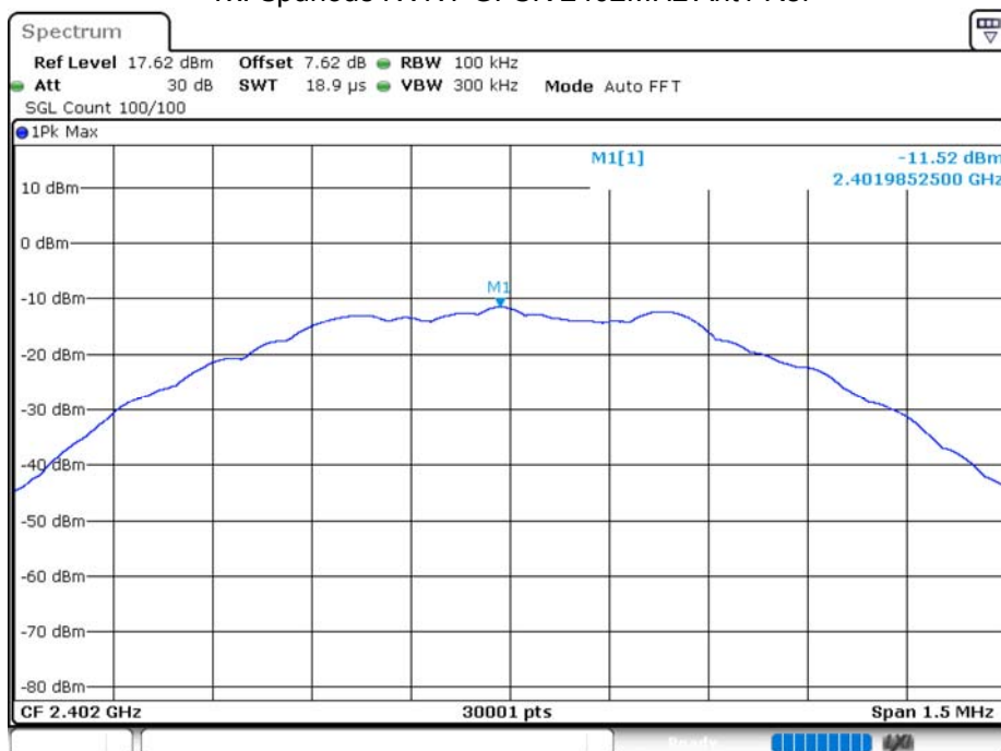
Tx. Spurious NVNT GFSK 2402MHz Ant1 Ref
