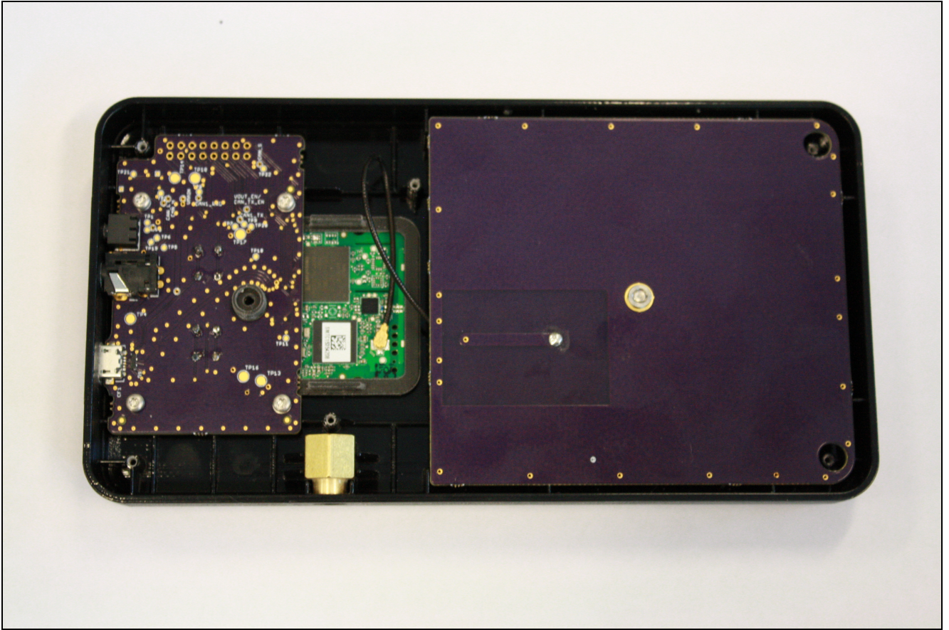
Figure 1: Internal assembly showing external connector interface card and antenna
