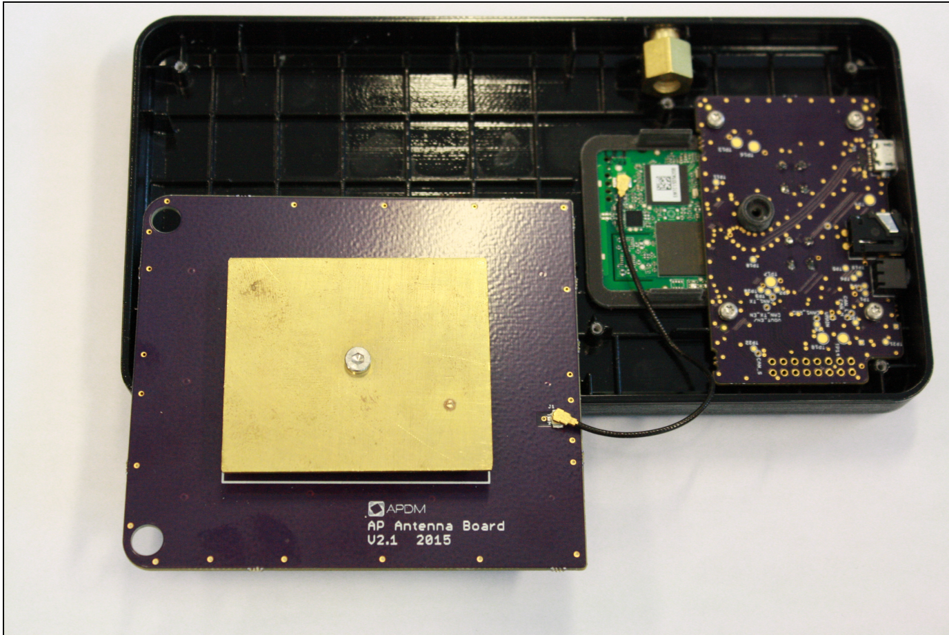
Figure 2: Internal assembly showing top of antenna board
