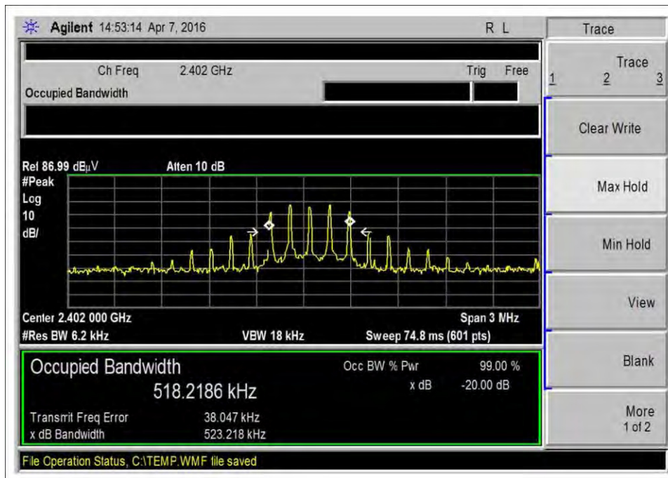
Bluetooth V4, GFSK, 2402MHz
