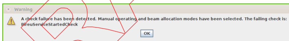
Figure 4-2. 'BireuServiceStartedCheck' Message
