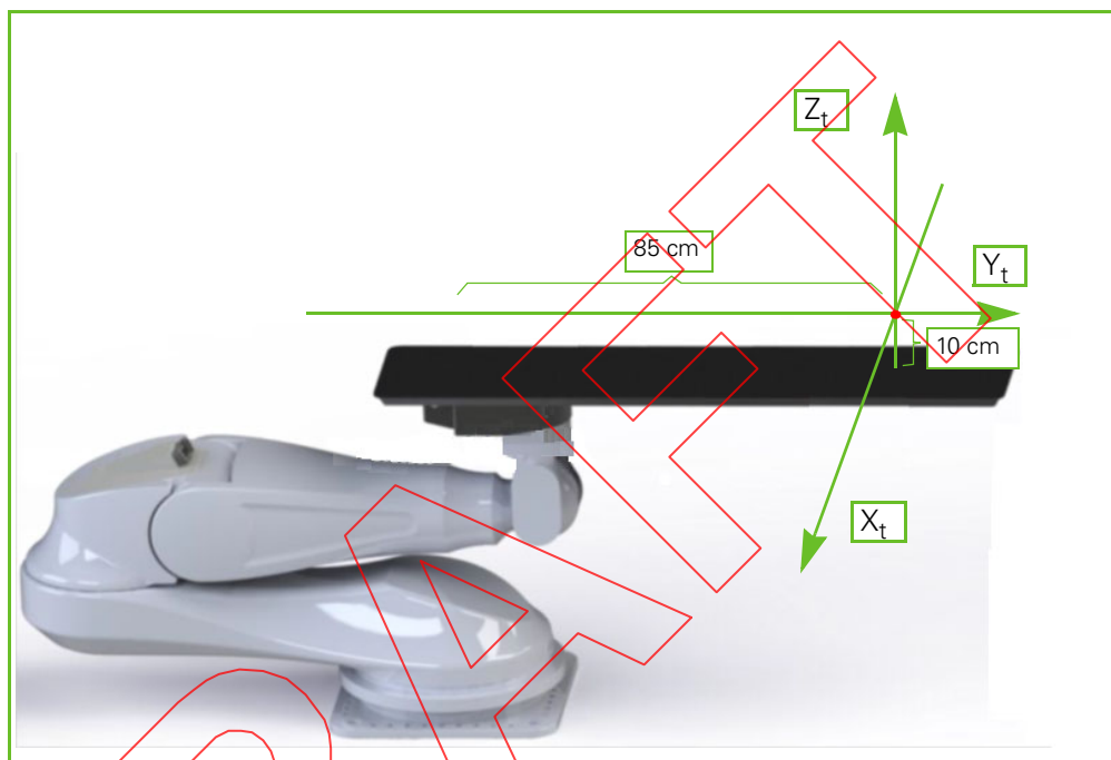
Figure 6-3. Table Top Coordinate System (TTCS)
