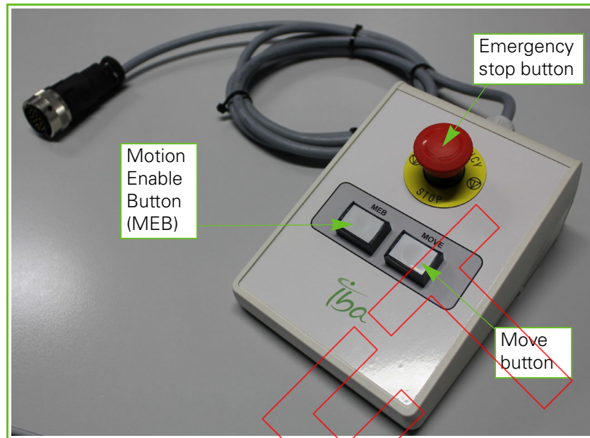
Figure 11-1. Remote Positioning Hardware Console
