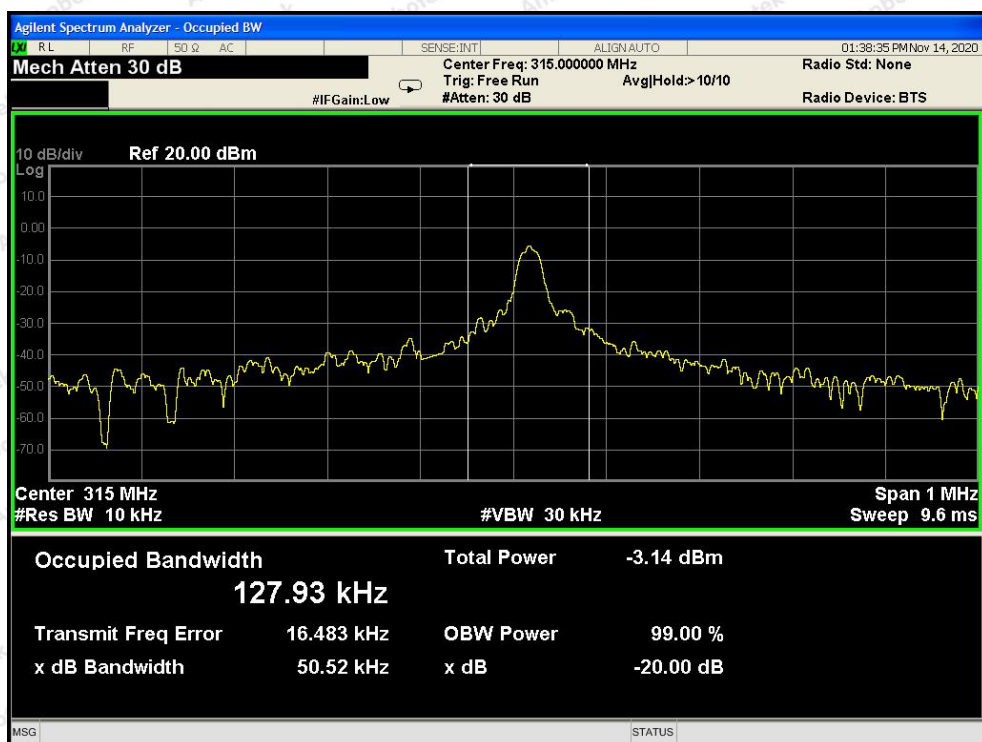
Plot of 20DB&99% Bandwidth
