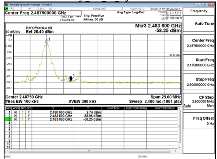
Band Edge_BLE_1M_HighCH39-2480
