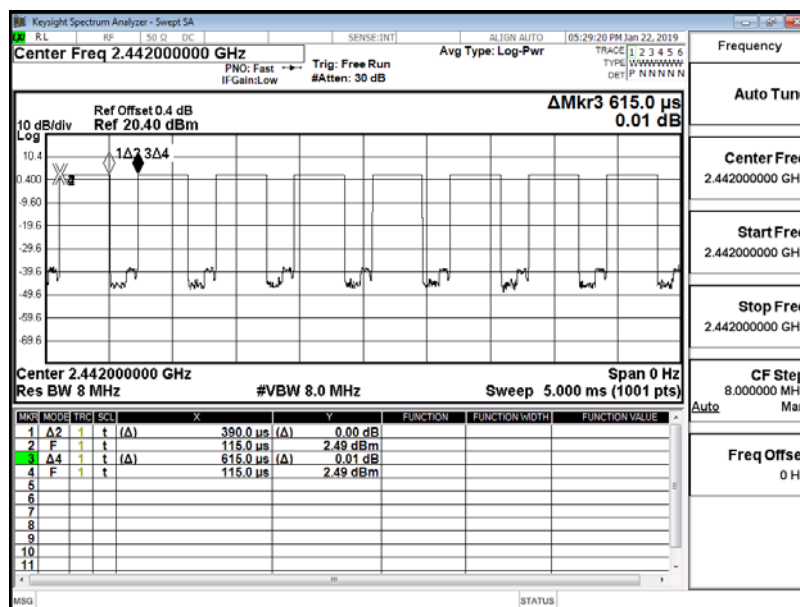
BLE_1M_MidCH20-2442
