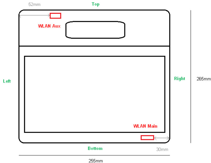
Fig.10 Antenna position of EUT (Front view)
