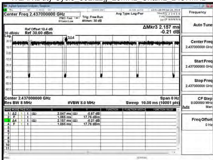
WLAN\Duty Cycle 802.11g 20MHz Chain1 2437MHz
