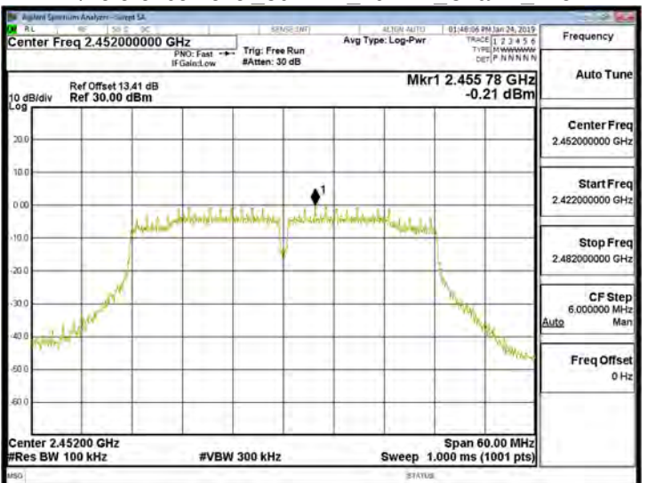
WLAN\Reference Level_802.11n_40MHz_Chain1_2452MHz
