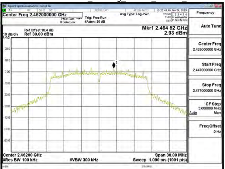
WLAN\Reference Level_802.11g_20MHz_Chain1_2462MHz
