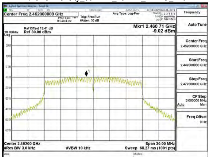
WLAN\Power Density 802.11n 20MHz MIMO 2462MHz
