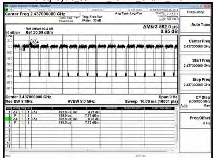
WLAN\Duty Cycle 802.11n 40MHz Chain1 2437MHz
