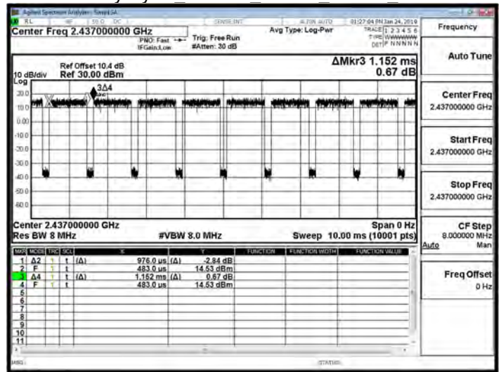
WLAN\Duty Cycle 802.11n 40MHz Chain1 2437MHz
