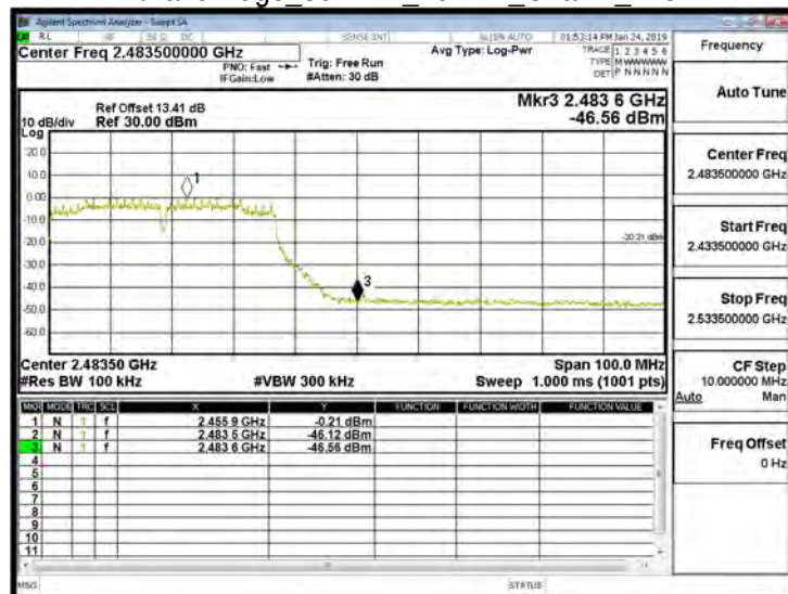
WLAN\Band Edge_802.11n_40MHz_Chain1_2452MHz
