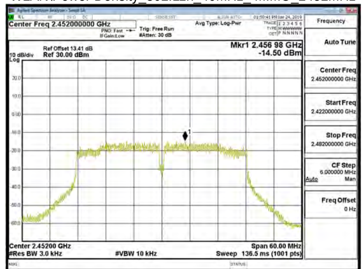
WLAN\Power Density 802.11n 40MHz MIMO 2452MHz
