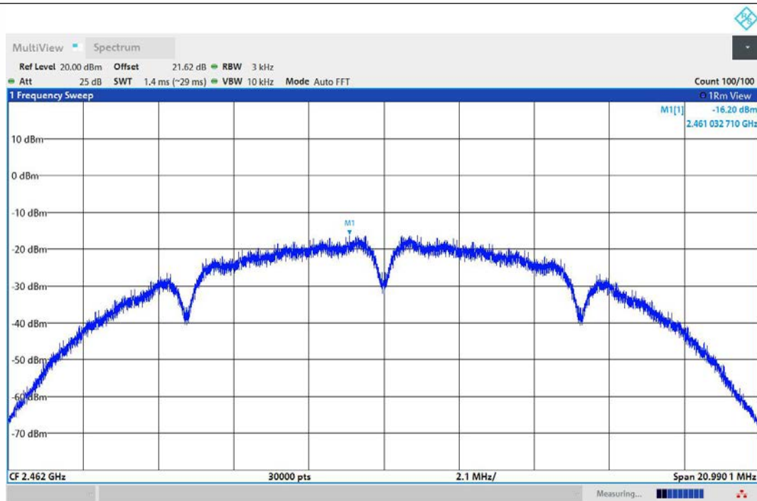
11B-Ant1-2462-PASS
