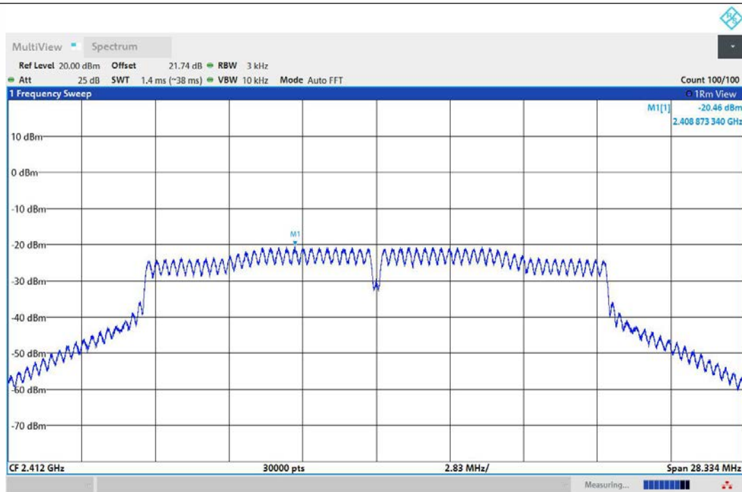
11N20MIMO-Ant1-2412-PASS
