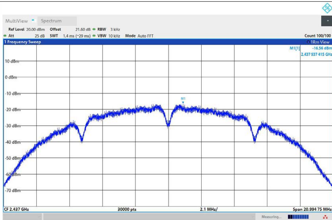
11B-Ant1-2437-PASS
