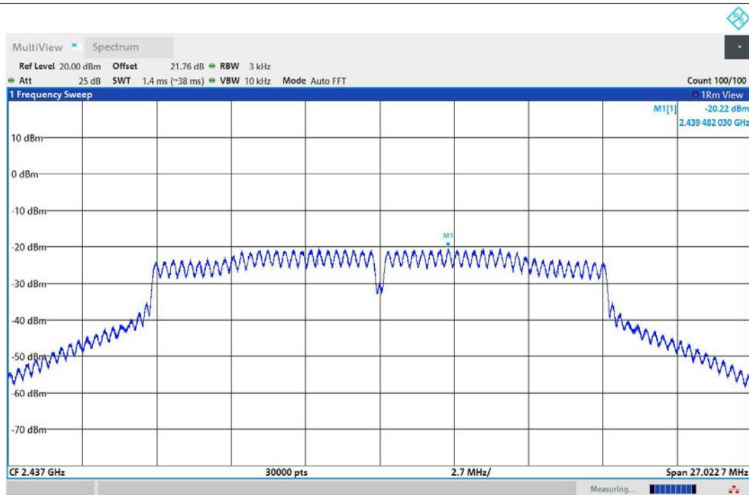
11G-Ant1-2437-PASS
