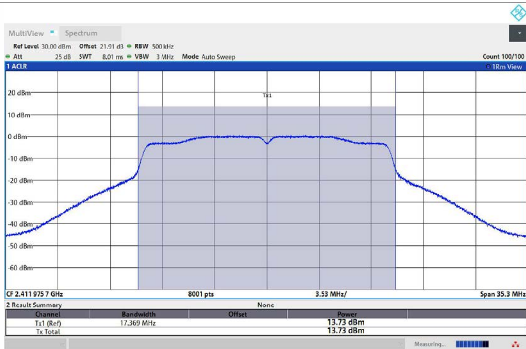
11G-Ant1-2412-PASS
