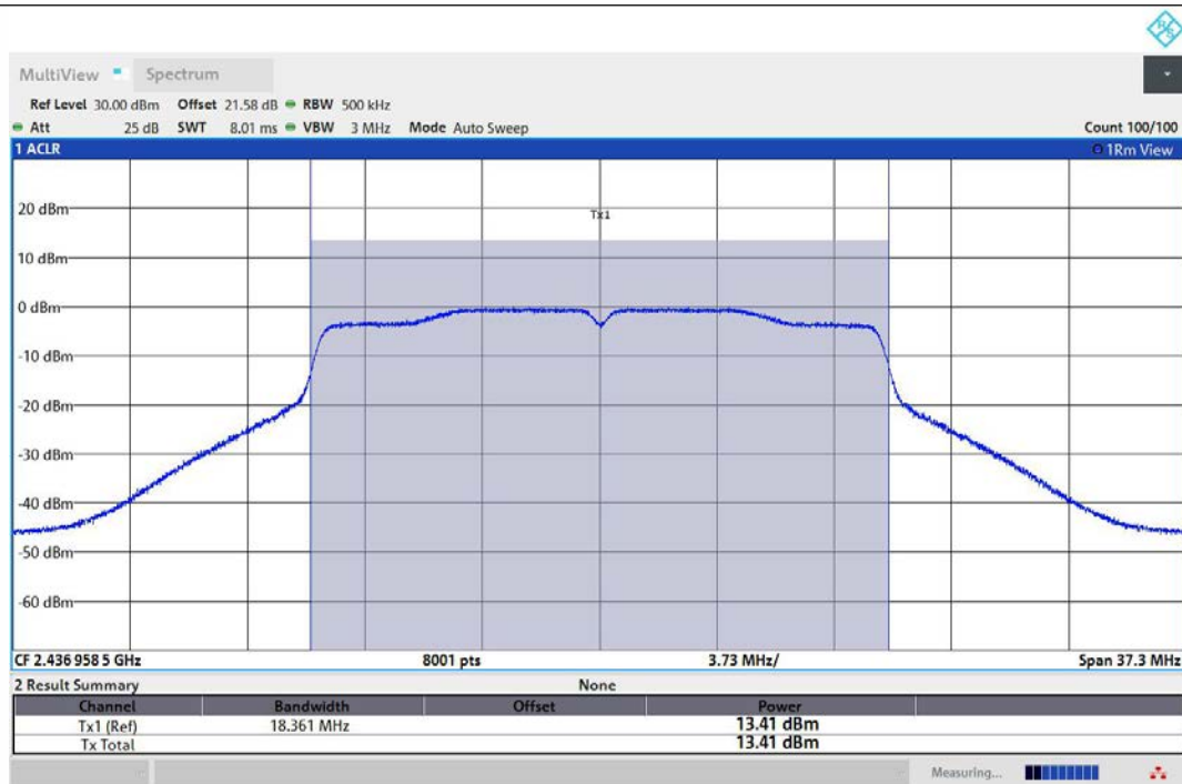
11N20MIMO-Ant1-2437-PASS
