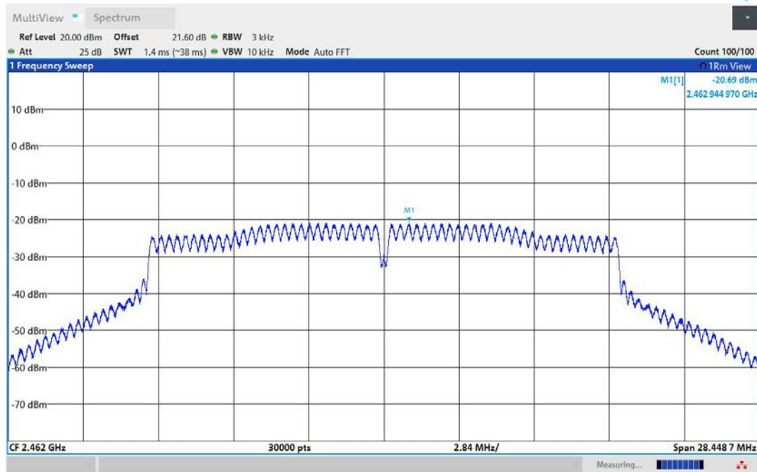
11N20MIMO-Ant1-2462-PASS
