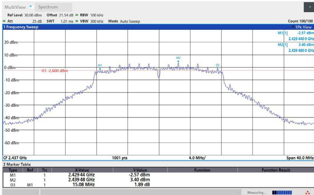
11G-Ant2-2437-PASS
