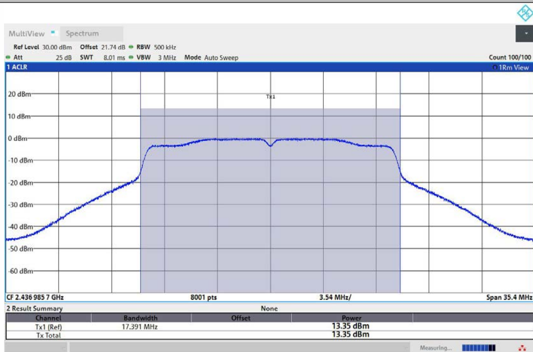
11G-Ant2-2437-PASS
