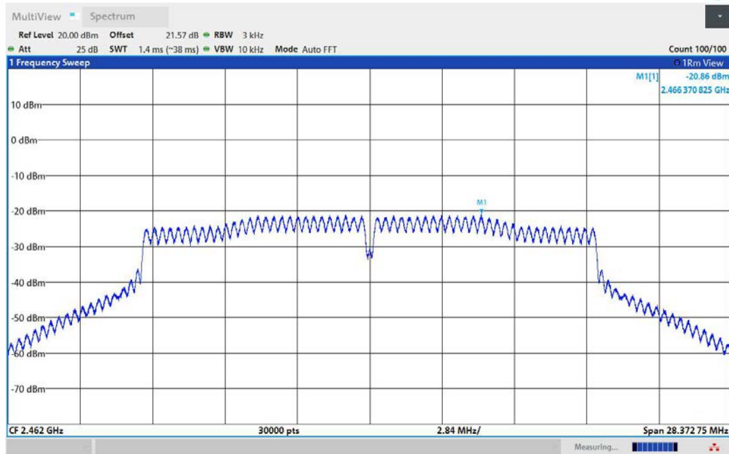
11N20MIMO-Ant2-2462-PASS
