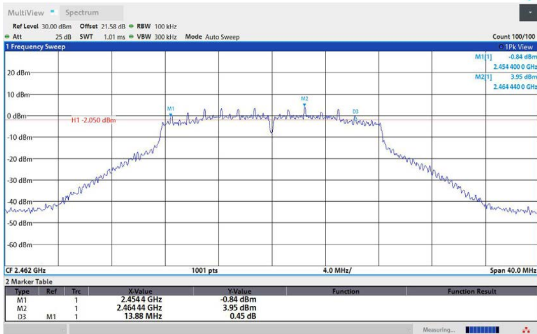
11G-Ant1-2462-PASS
