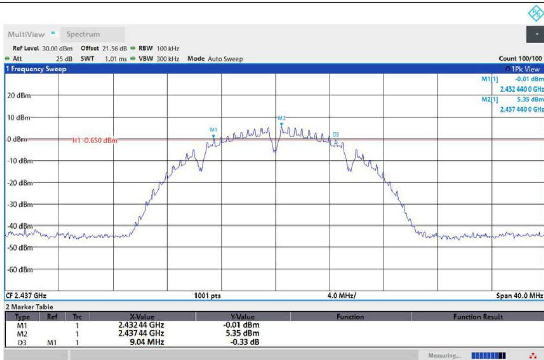
11B-Ant1-2437-PASS
