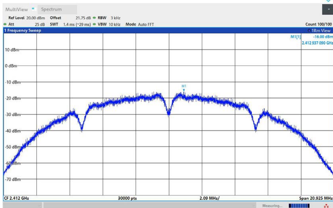
11B-Ant1-2412-PASS
