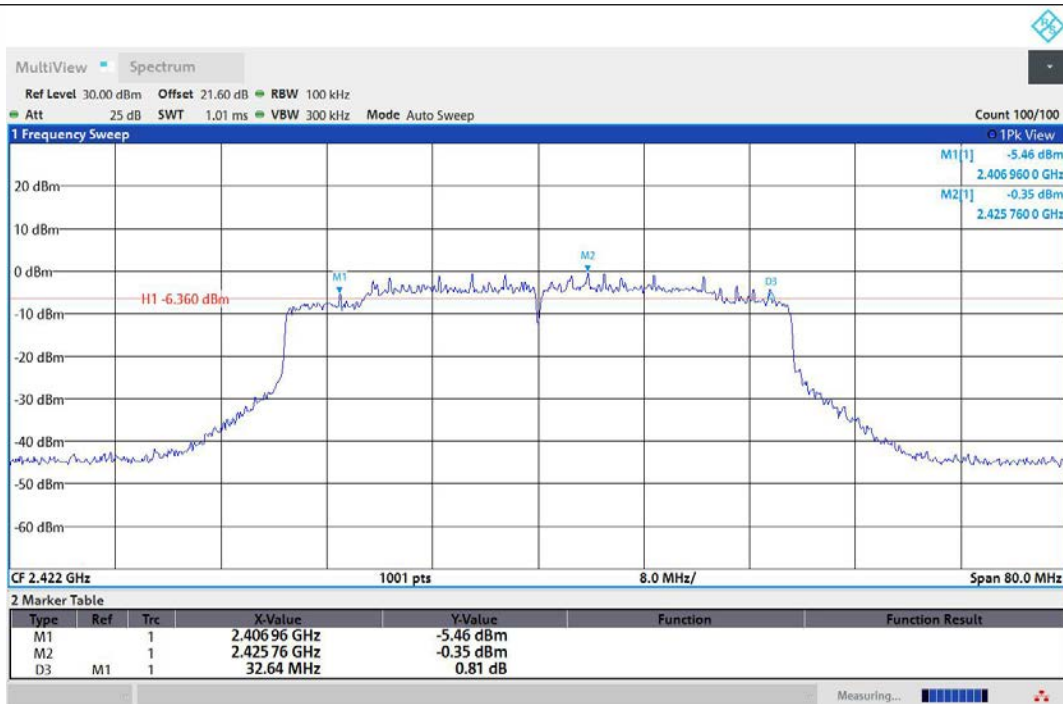
11AX40MIMO-Ant1-2422-PASS
