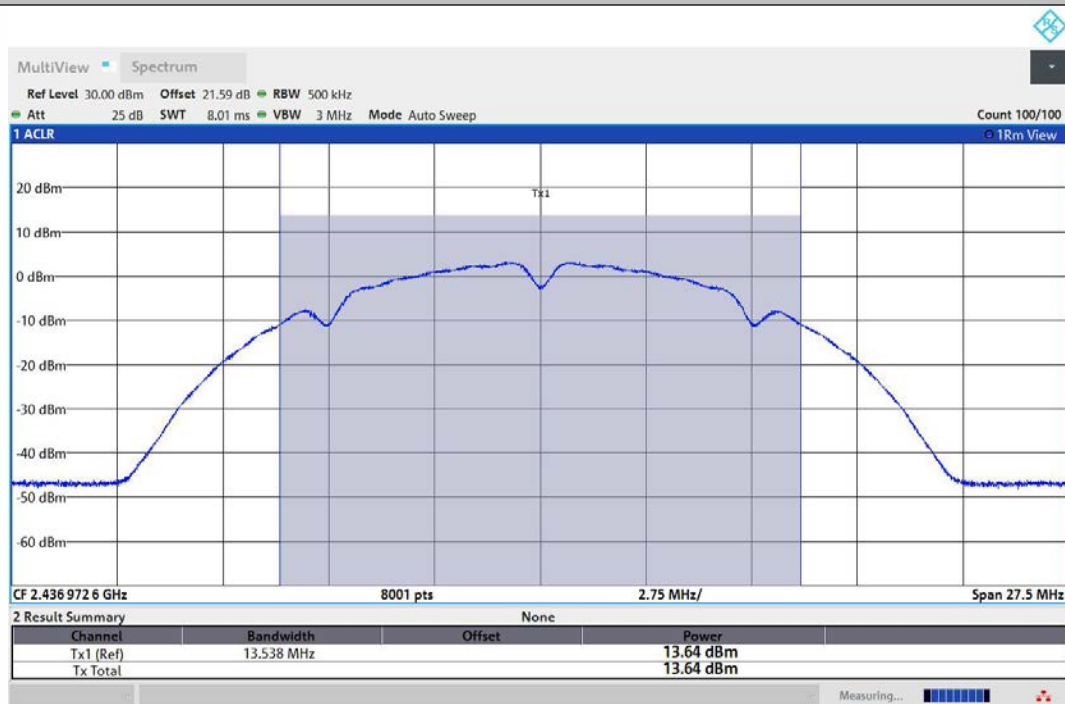
11B-Ant2-2437-PASS
