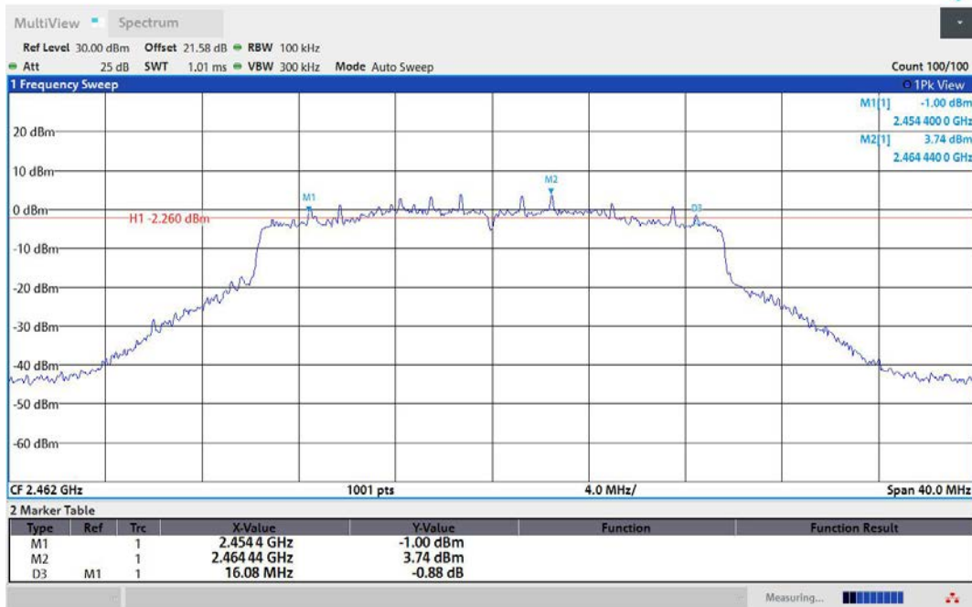
11AX20MIMO-Ant1-2462-PASS
