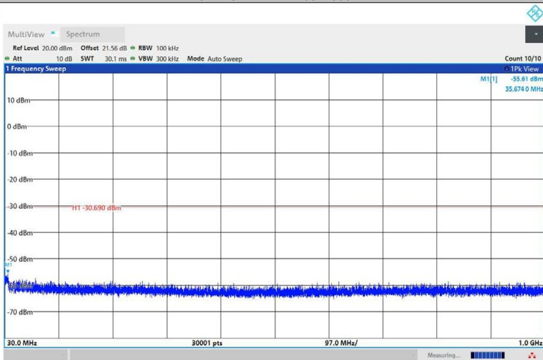
11AX40MIMO-Ant2-2422-30~1000-PASS
