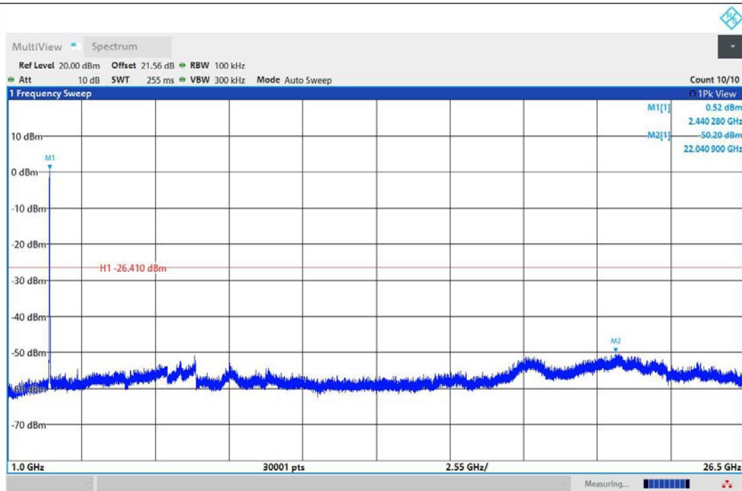
11AX20MIMO-Ant1-2437-1000~26500-PASS
