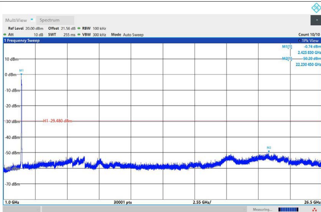
11N40MIMO-Ant1-2437-1000~26500-PASS
