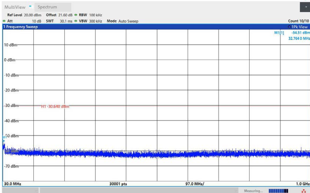
11AX40MIMO-Ant2-2452-30~1000-PASS
