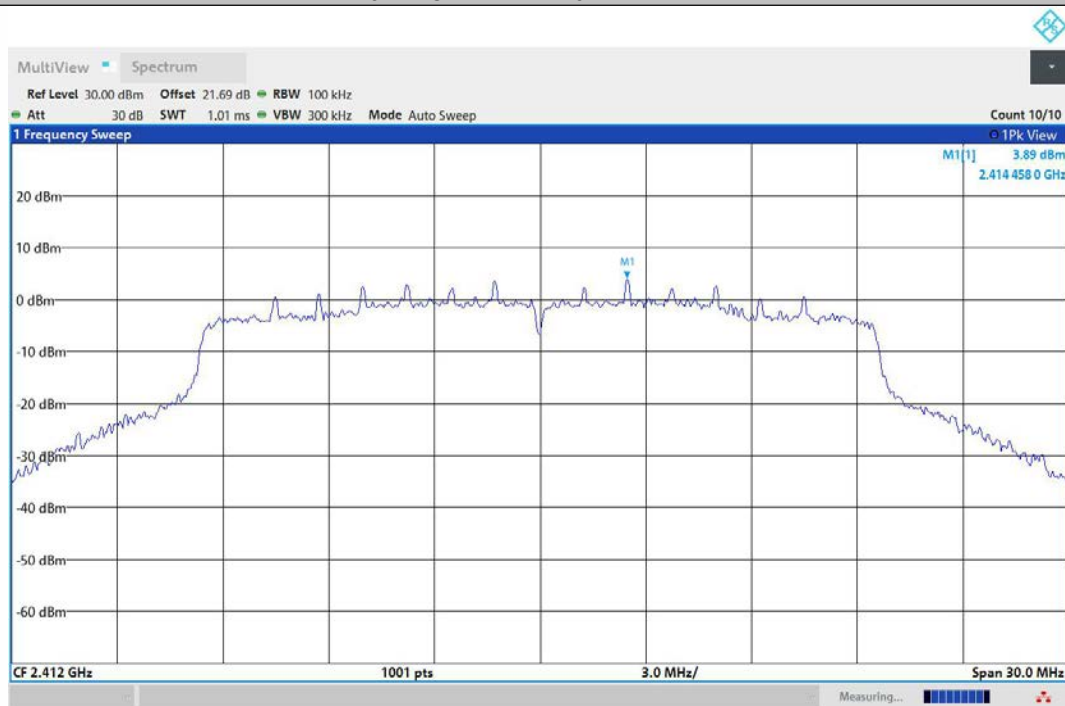
11AX20MIMO-Ant2-2412-0~Reference-PASS
