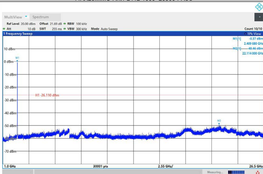
11AX20MIMO-Ant2-2412-1000~26500-PASS
