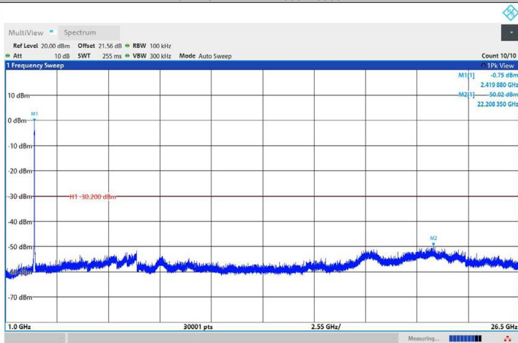
11N40MIMO-Ant2-2422-1000~26500-PASS
