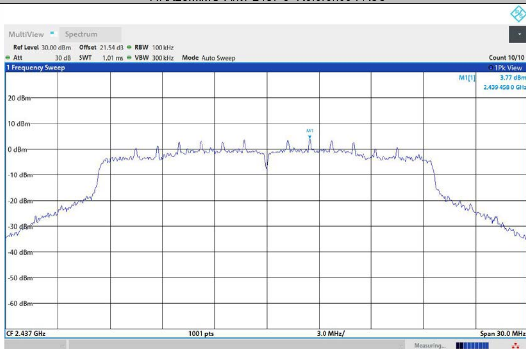
11AX20MIMO-Ant2-2437-0~Reference-PASS
