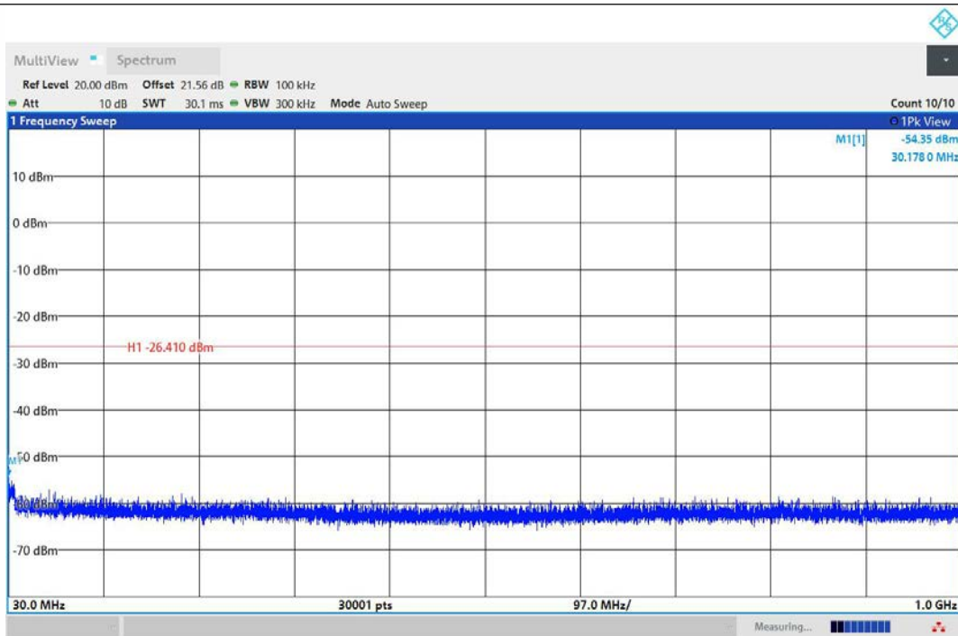
11AX20MIMO-Ant1-2437-30~1000-PASS
