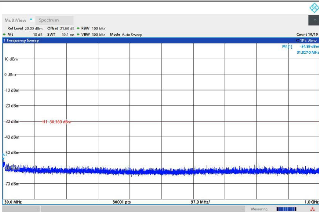
11N40MIMO-Ant2-2452-30~1000-PASS
