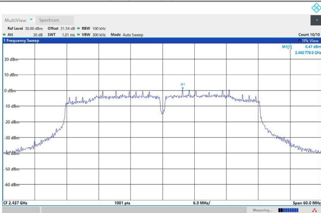
11N40MIMO-Ant2-2437-0~Reference-PASS
