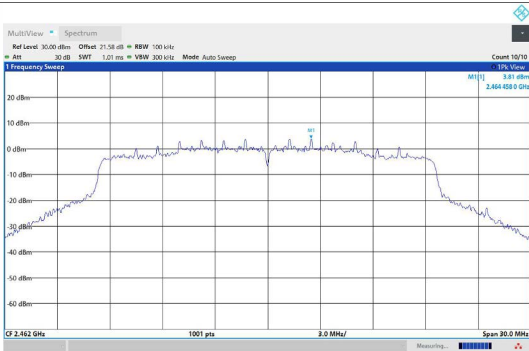
11AX20MIMO-Ant1-2462-0~Reference-PASS
