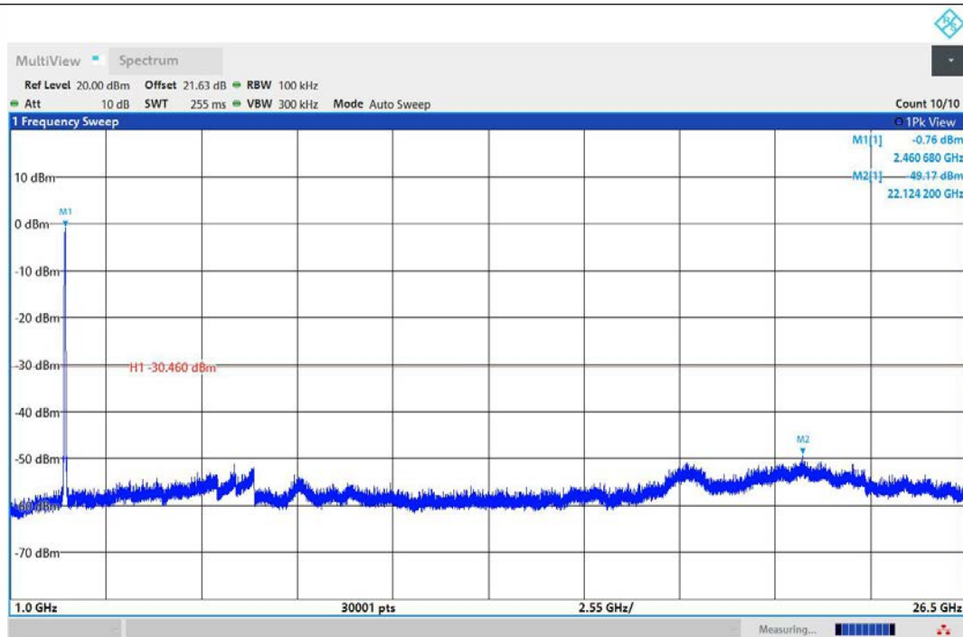
11AX40MIMO-Ant1-2452-1000~26500-PASS
