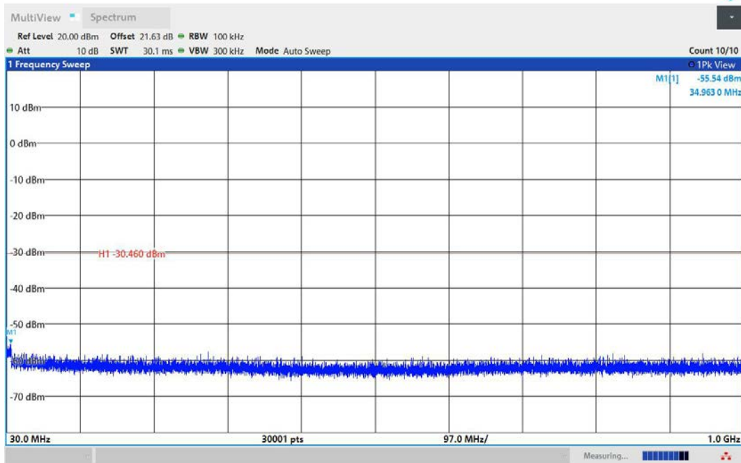
11AX40MIMO-Ant1-2452-30~1000-PASS
