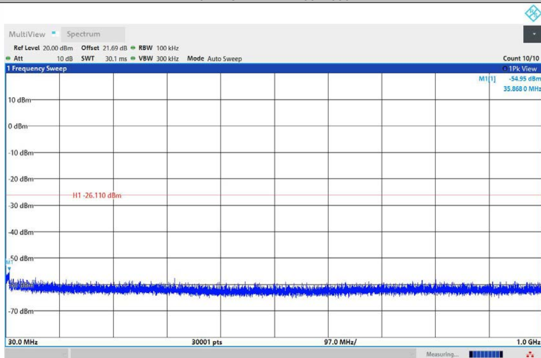
11AX20MIMO-Ant2-2412-30~1000-PASS
