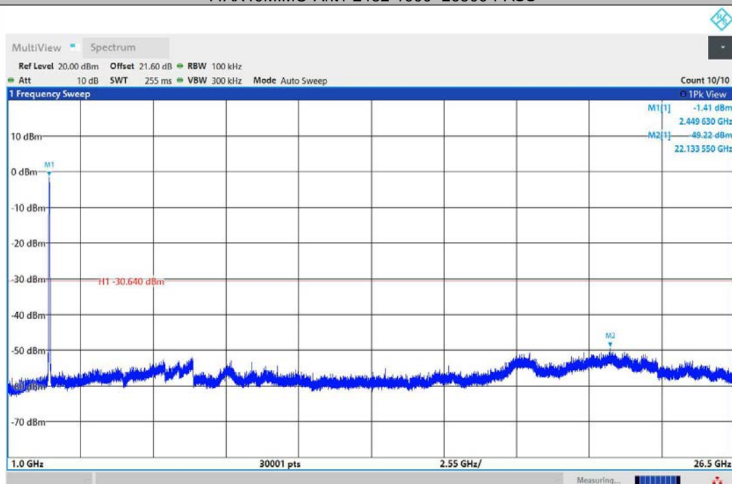
11AX40MIMO-Ant2-2452-1000~26500-PASS
