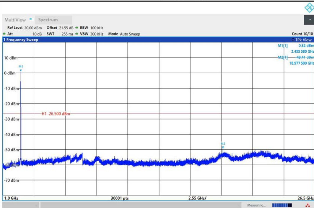
11AX20MIMO-Ant2-2462-1000~26500-PASS
