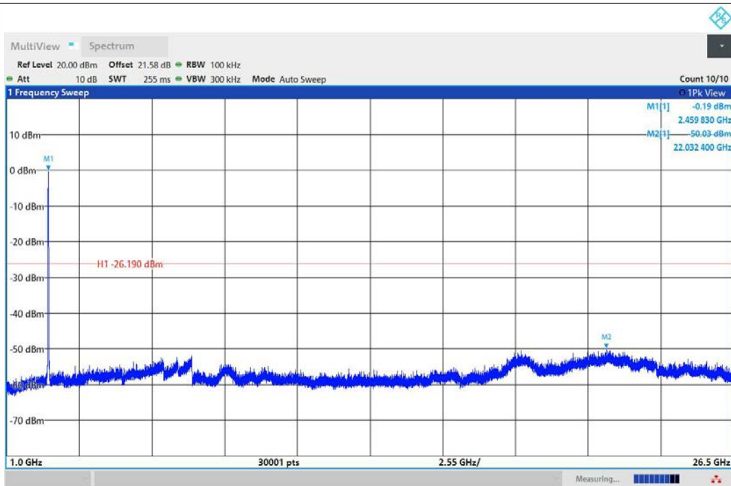
11AX20MIMO-Ant1-2462-1000~26500-PASS
