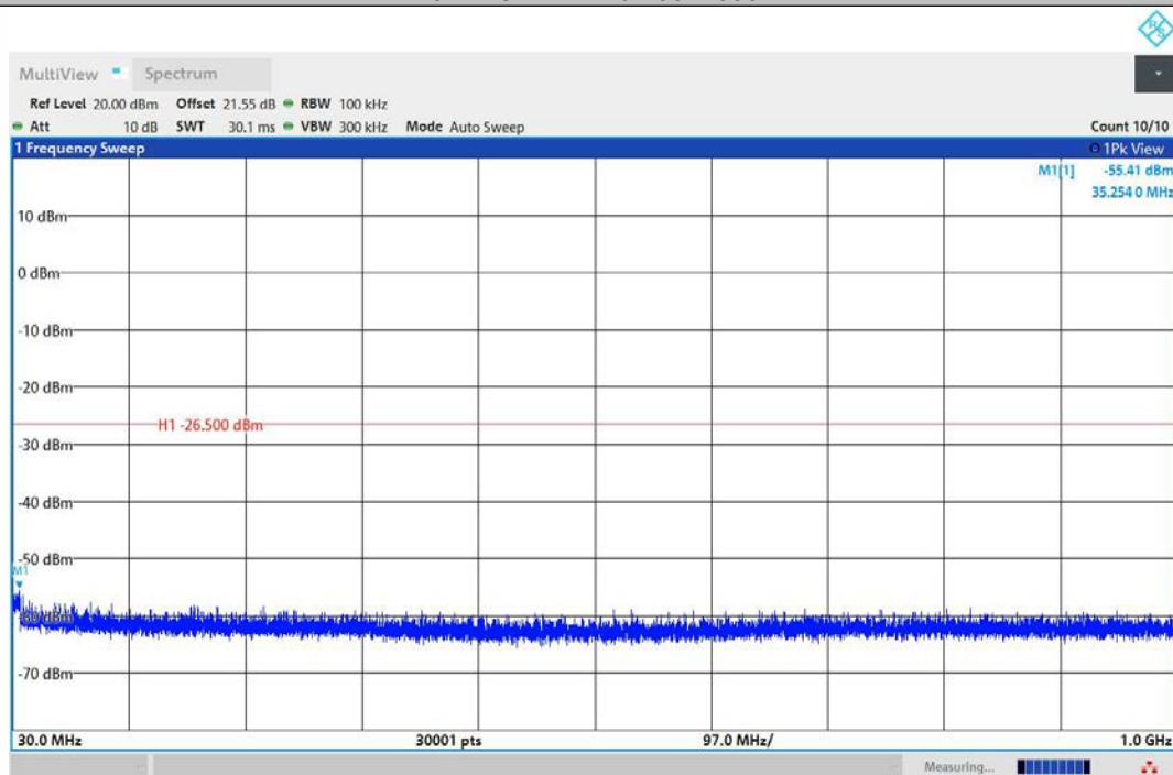
11AX20MIMO-Ant2-2462-30~1000-PASS
