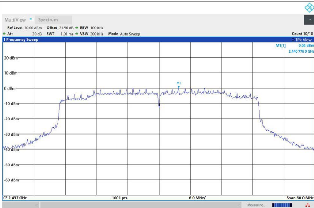
11AX40MIMO-Ant1-2437-0~Reference-PASS
