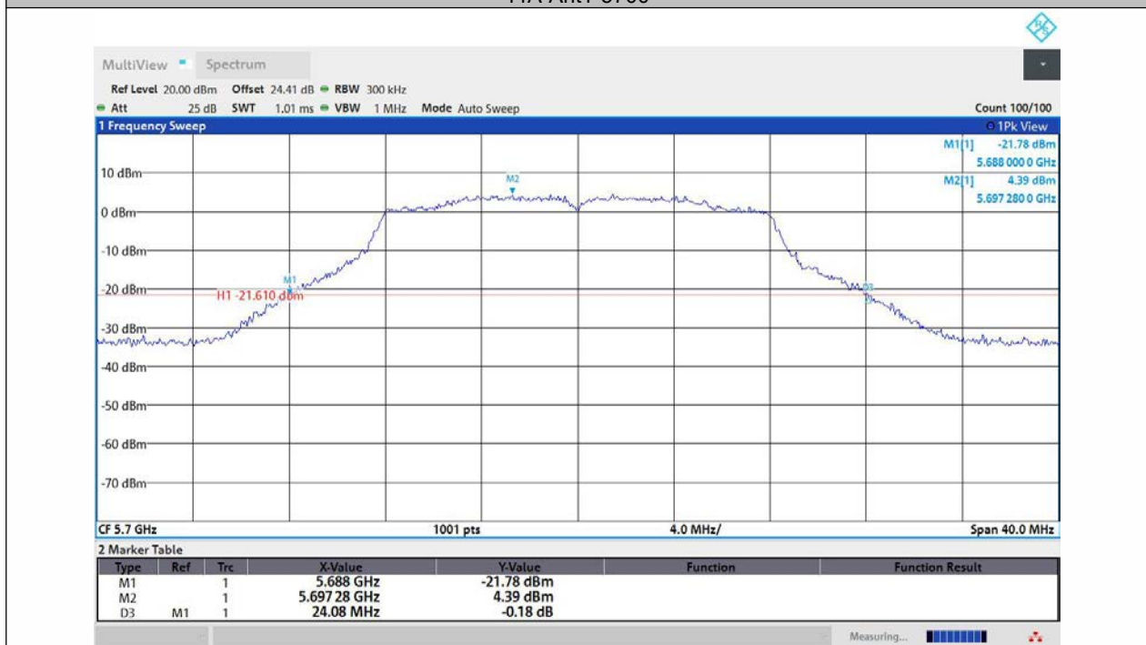
11A-Ant2-5700
