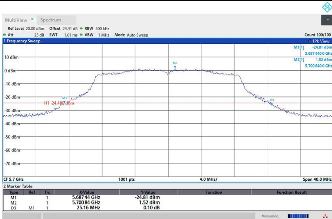
11AC20MIMO-Ant2-5700
