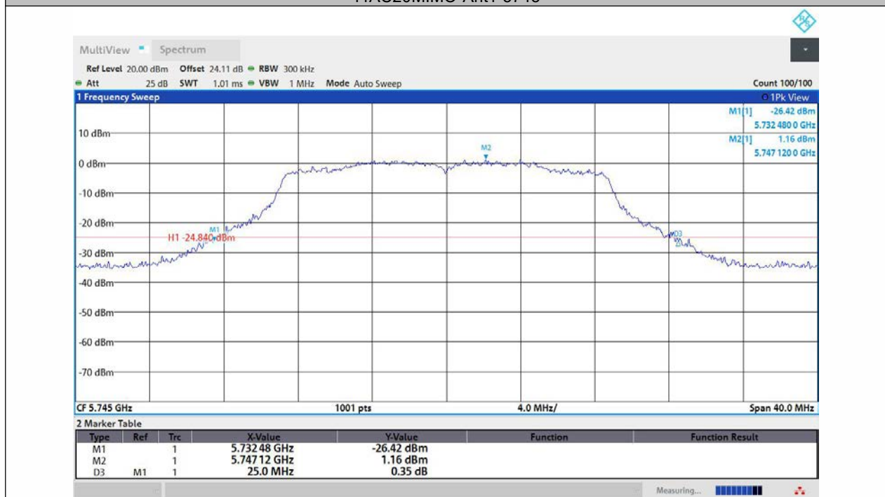
11AC20MIMO-Ant2-5745
