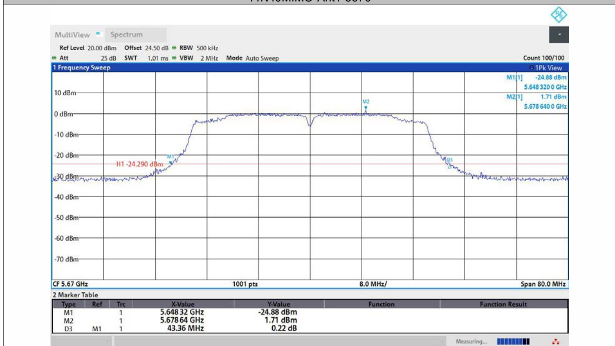
11N40MIMO-Ant2-5670
