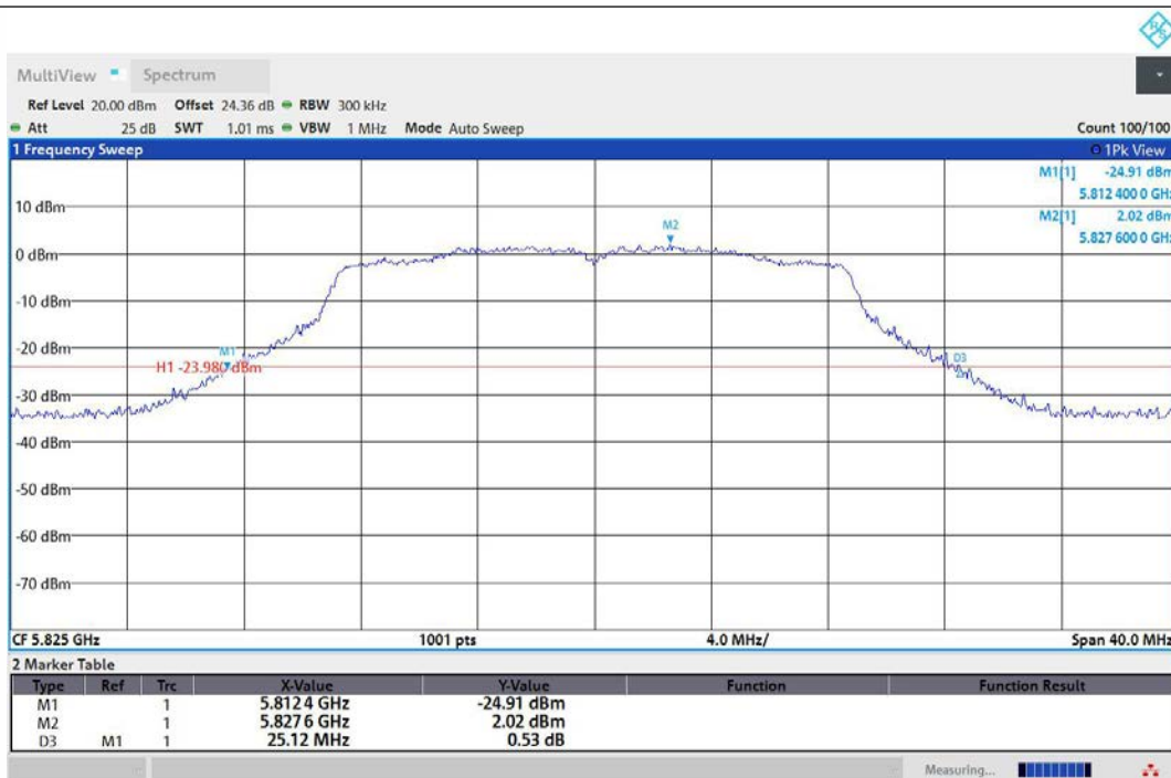
11AC20MIMO-Ant1-5825
