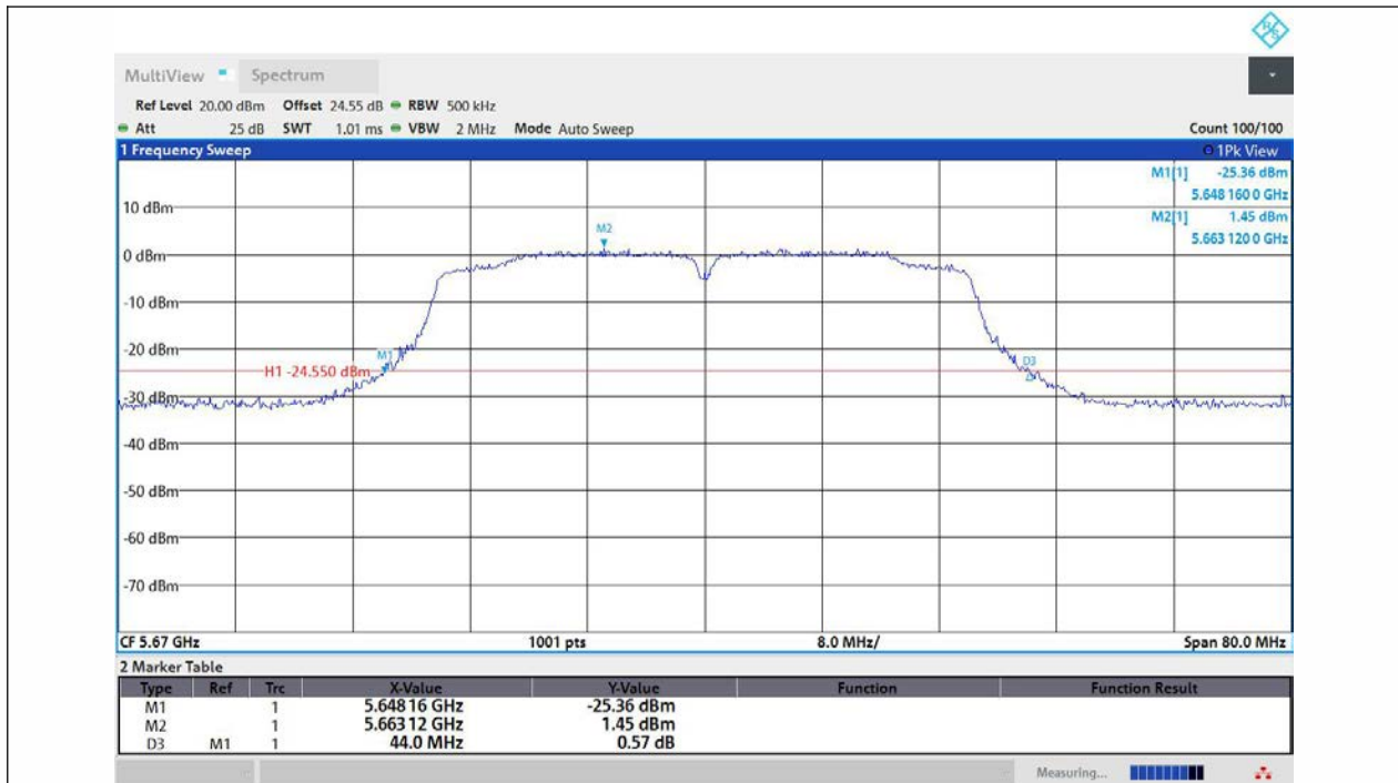
11N40MIMO-Ant1-5670
