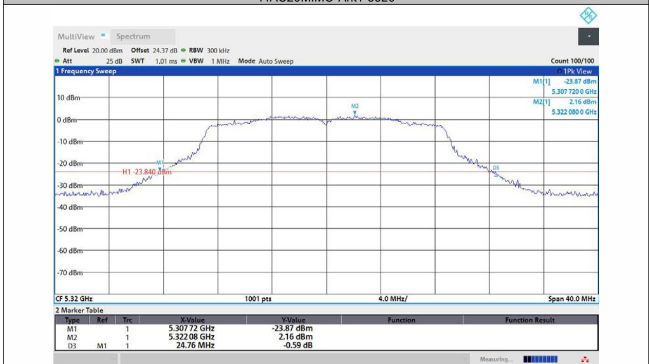
11AC20MIMO-Ant2-5320
