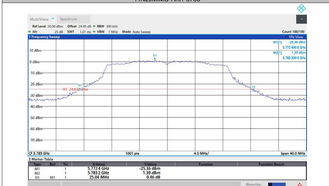
11N20MIMO-Ant2-5785
