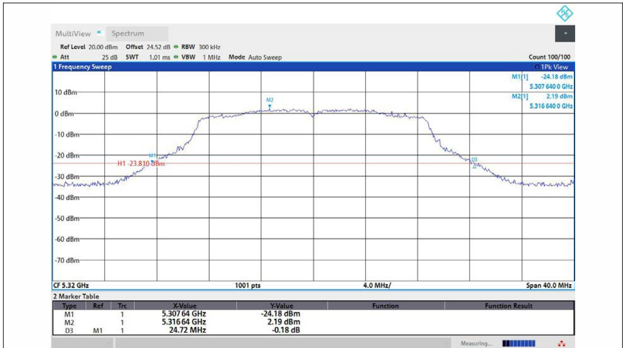
11AC20MIMO-Ant1-5320
