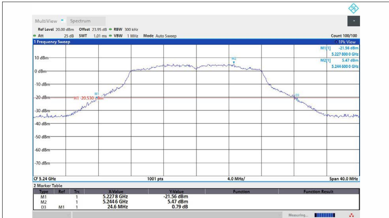
11A-Ant1-5240
