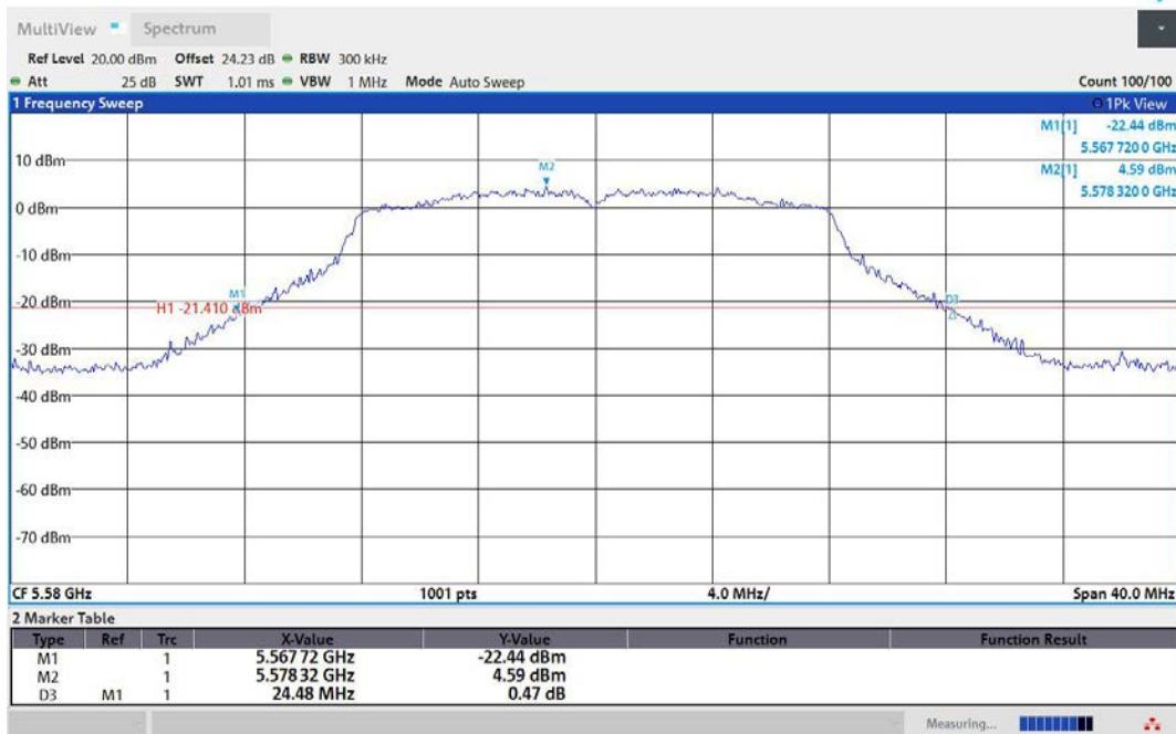
11A-Ant2-5580
