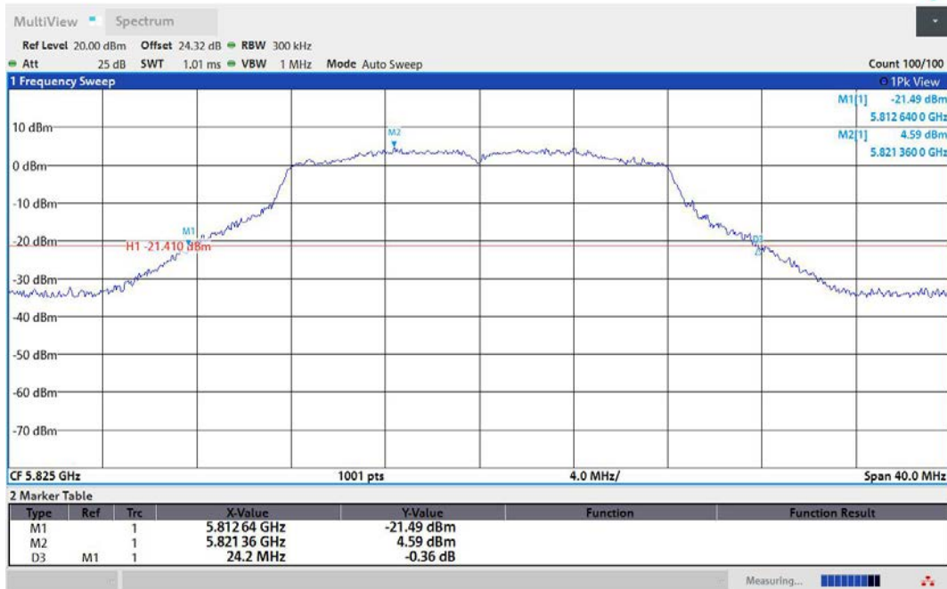
11A-Ant2-5825
