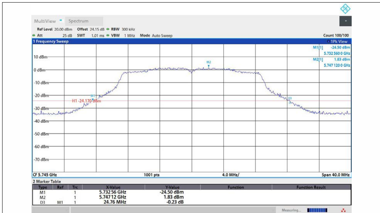
11AC20MIMO-Ant1-5745
