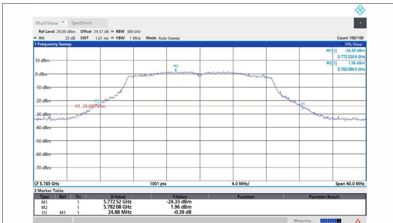
11N20MIMO-Ant1-5785
