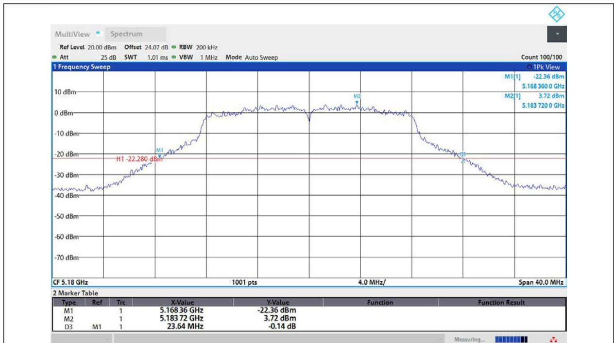
11A-Ant1-5180
