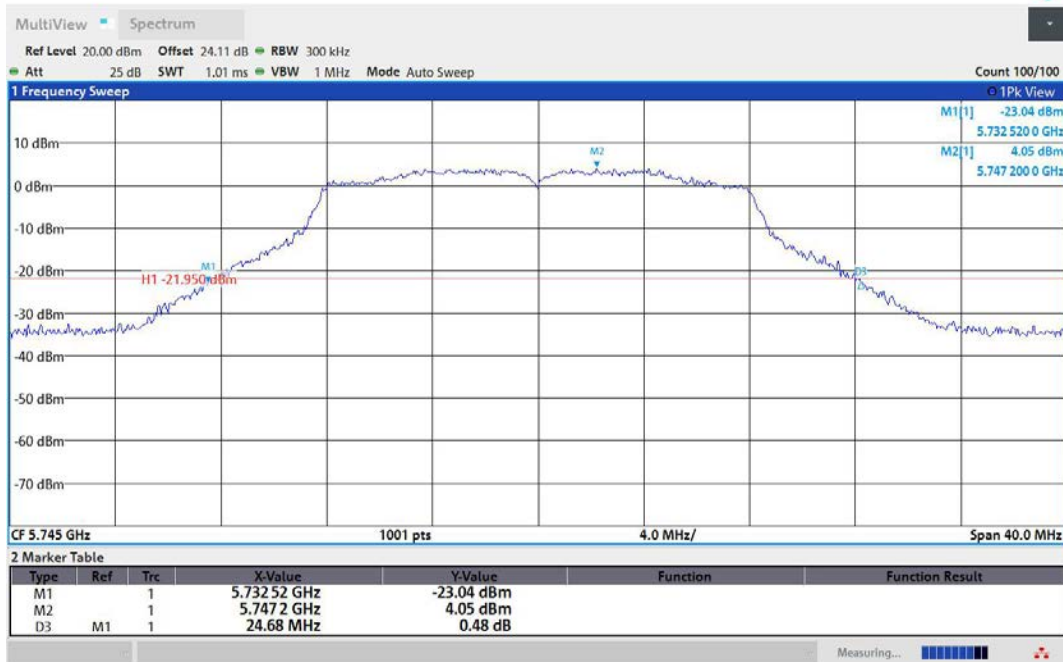
11A-Ant2-5745
