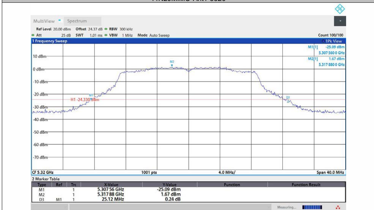
11N20MIMO-Ant2-5320
