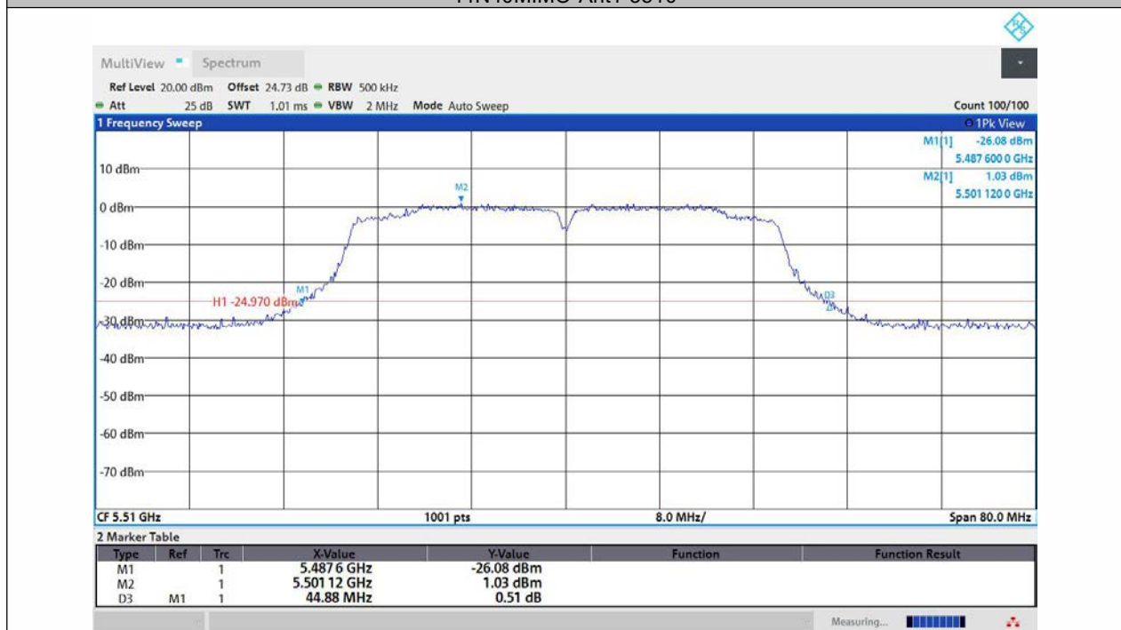
11N40MIMO-Ant2-5510
