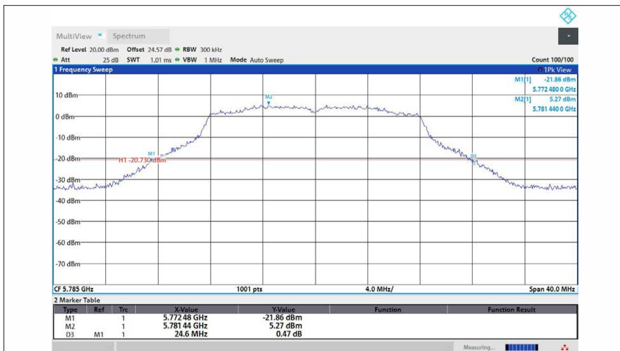
11A-Ant1-5785
