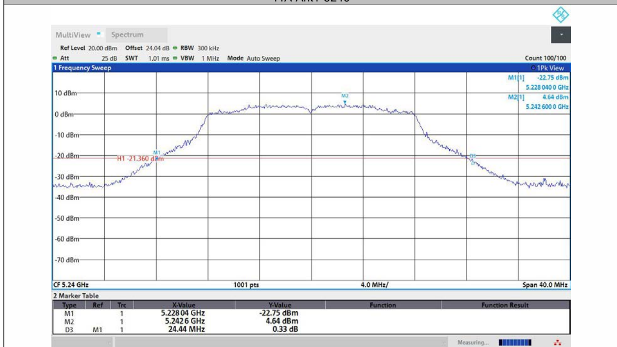
11A-Ant2-5240
