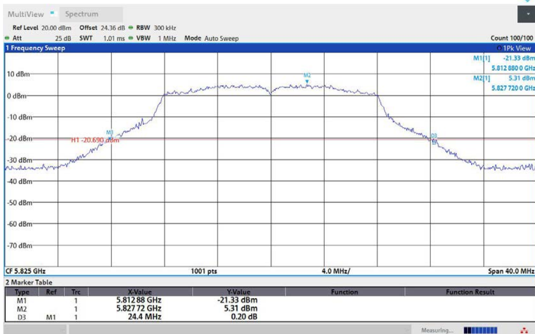
11A-Ant1-5825
