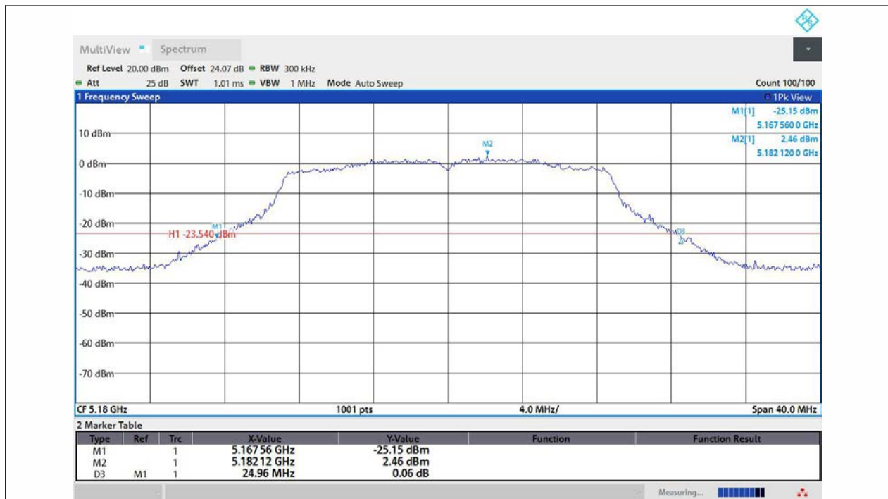
11AC20MIMO-Ant1-5180
