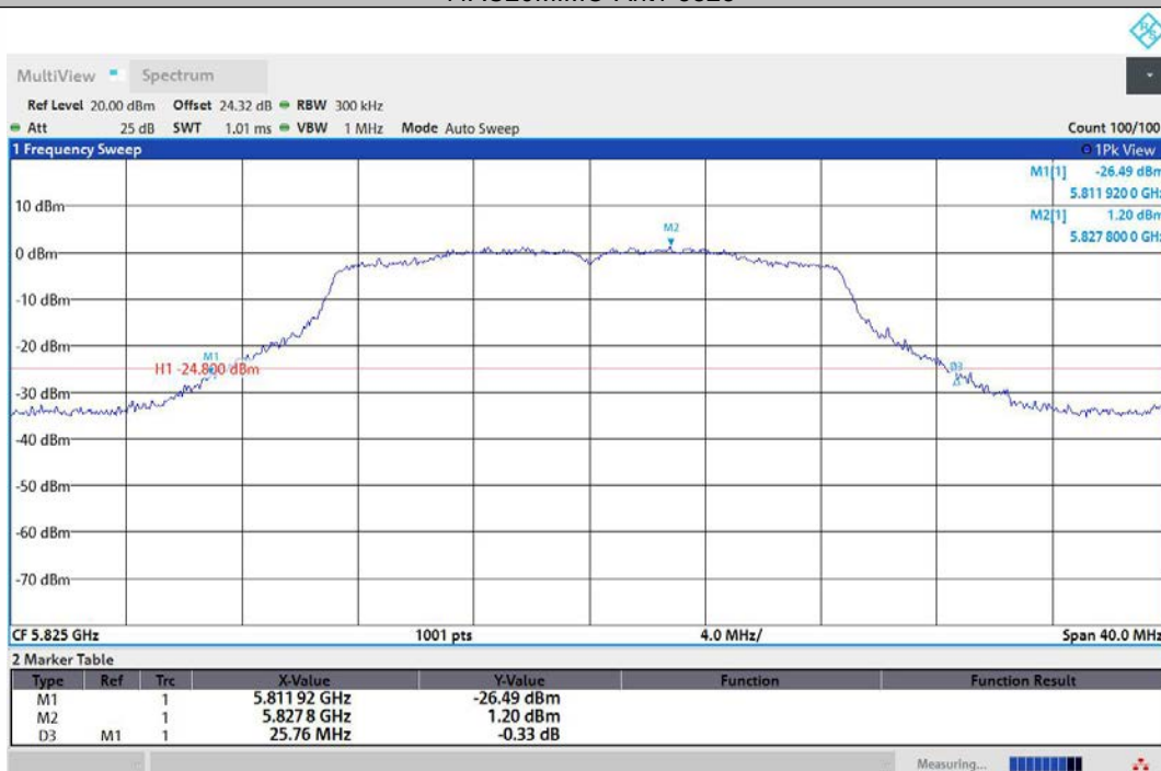
11AC20MIMO-Ant2-5825
