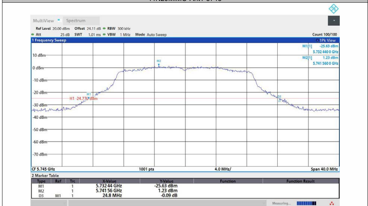
11N20MIMO-Ant2-5745
