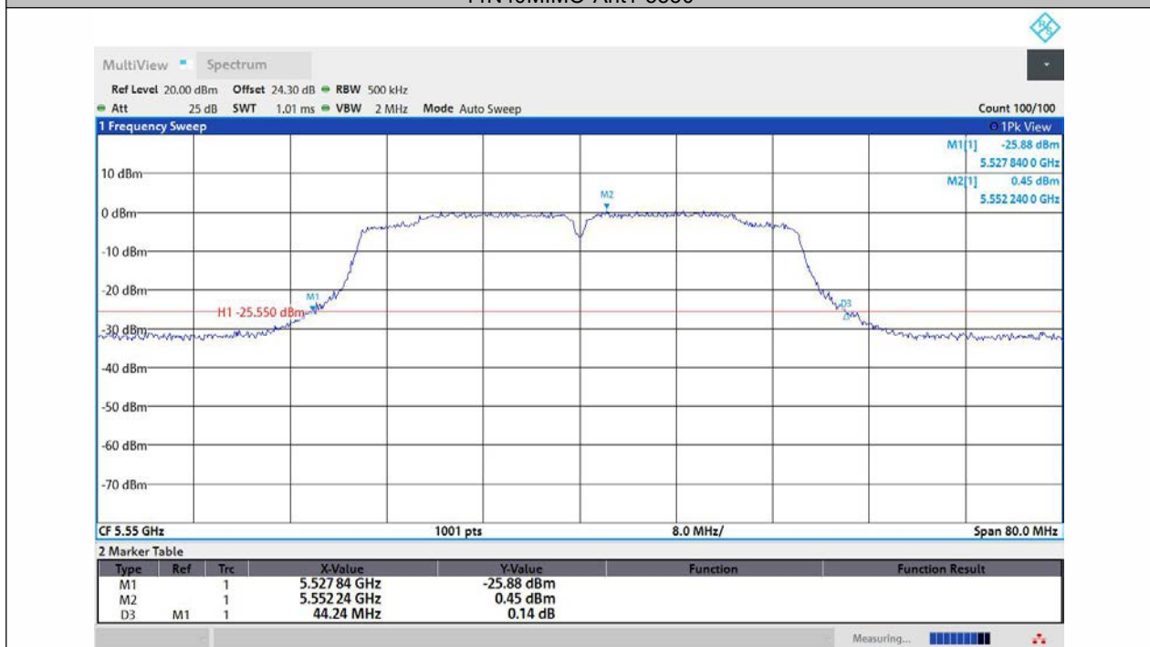
11N40MIMO-Ant2-5550
