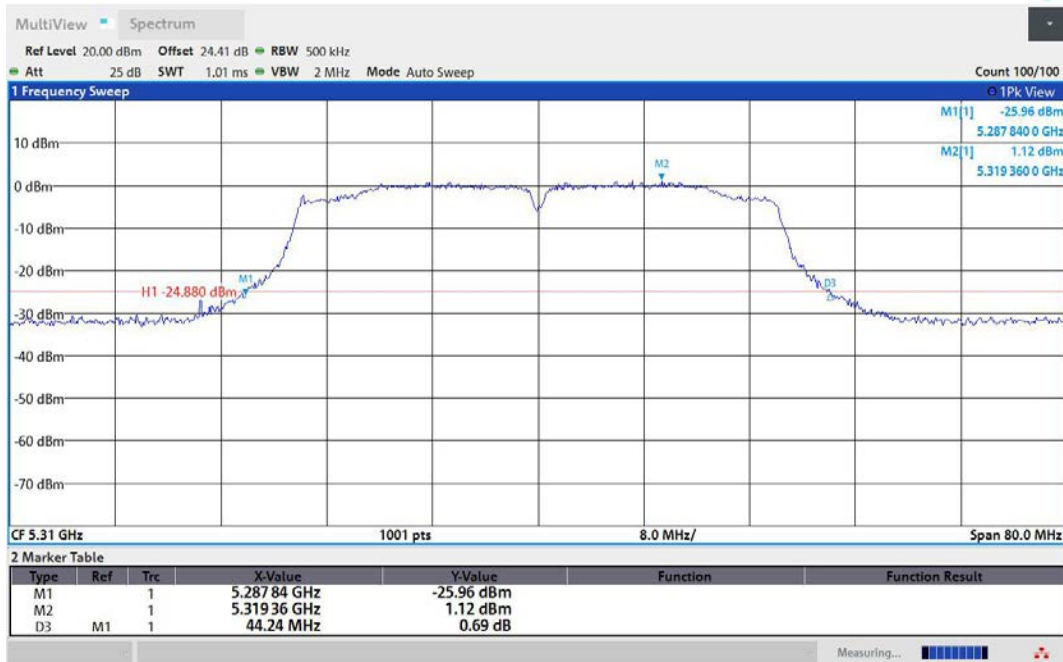
11N40MIMO-Ant2-5310
