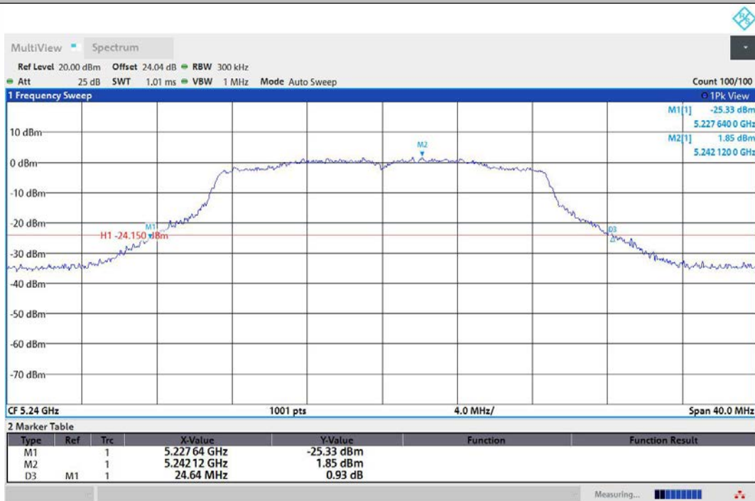
11N20MIMO-Ant2-5240
