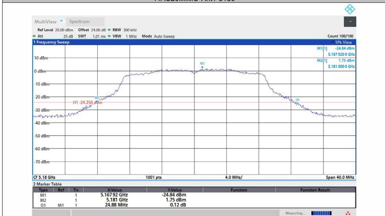
11AC20MIMO-Ant2-5180
