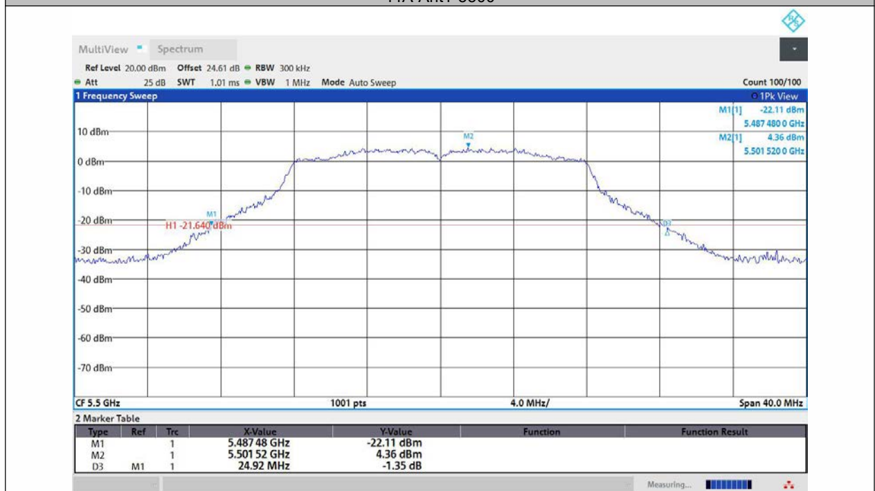
11A-Ant2-5500
