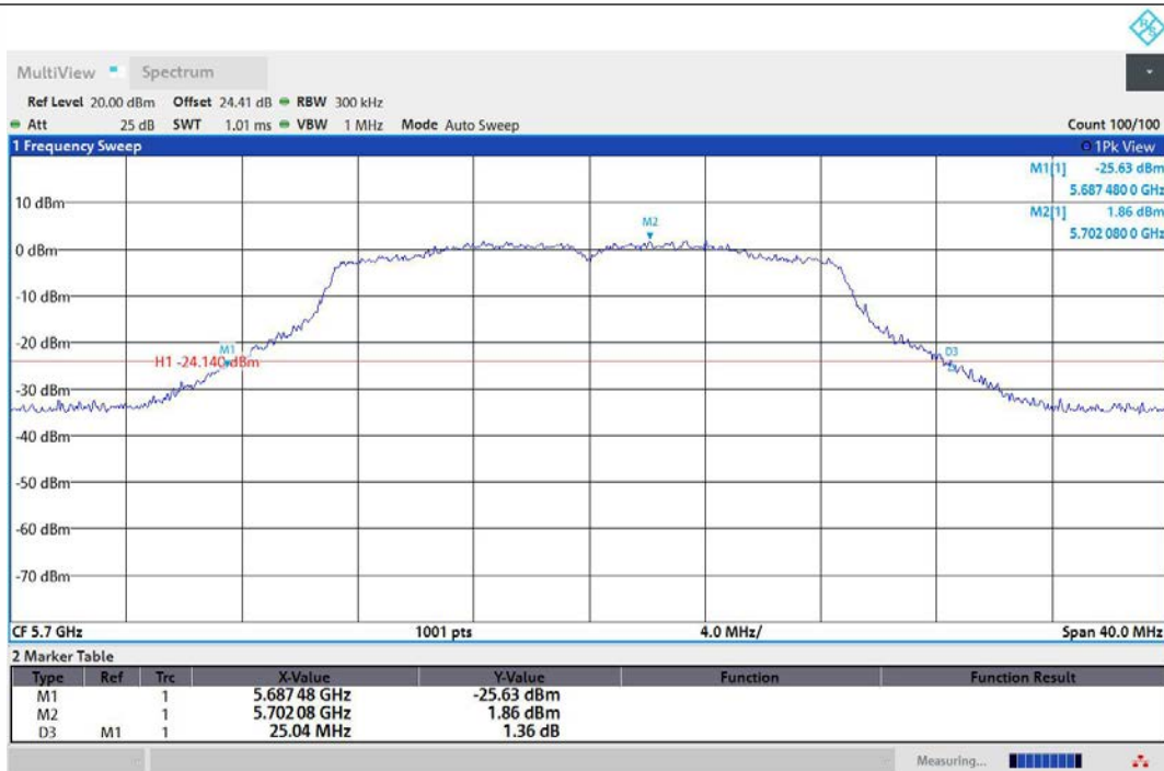
11AC20MIMO-Ant1-5700
