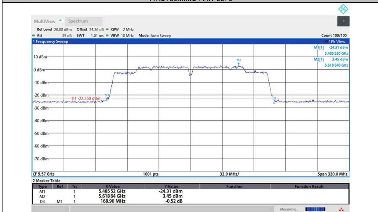
11AC160MIMO-Ant2-5570
