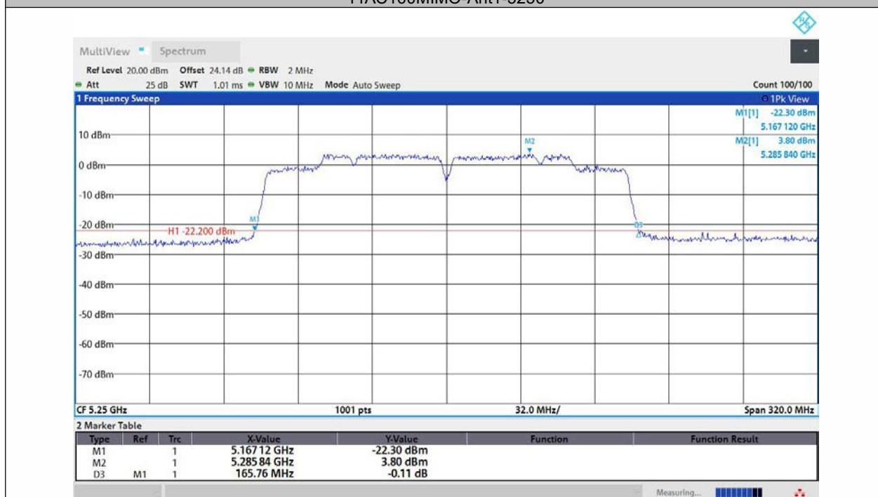
11AC160MIMO-Ant2-5250
