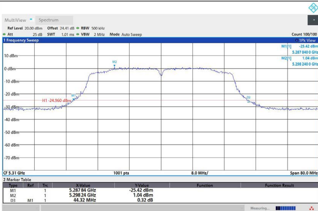
11AC40MIMO-Ant2-5310
