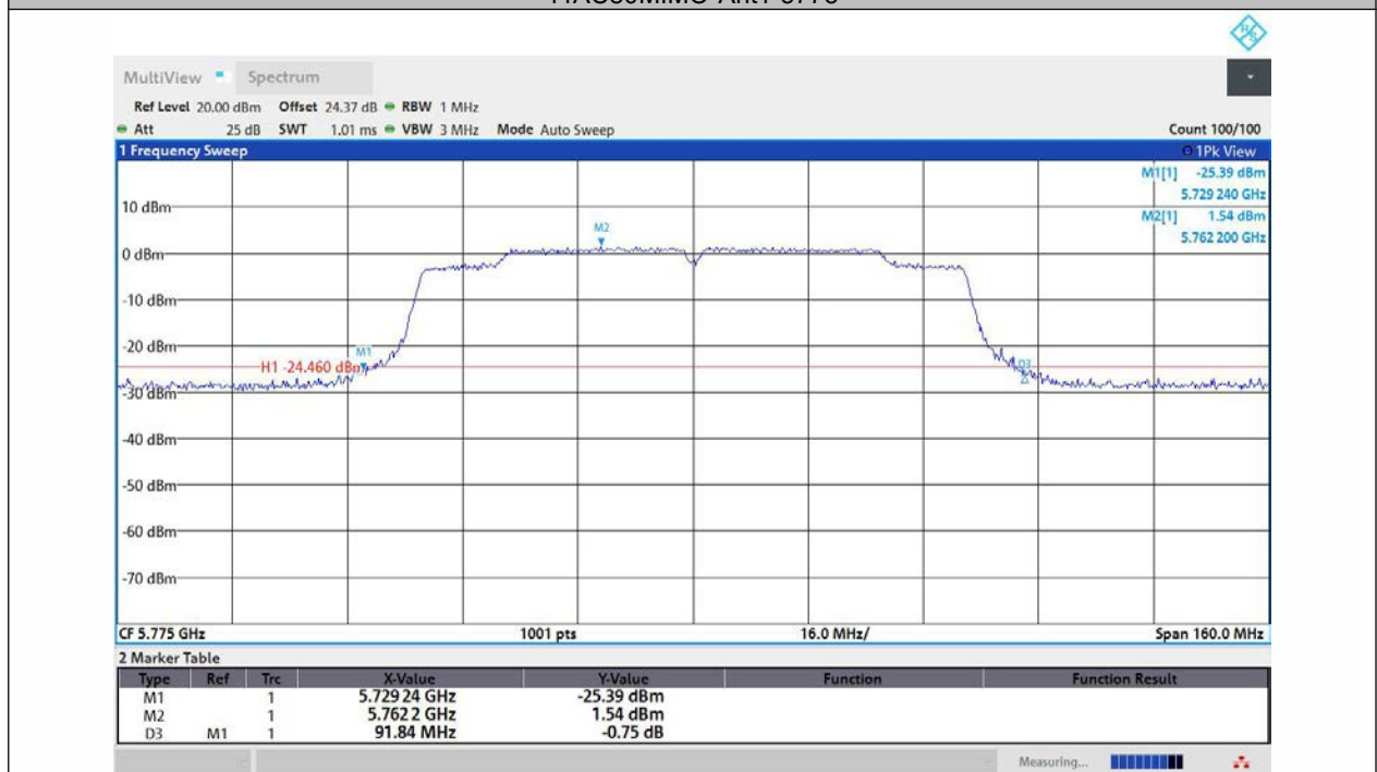
11AC80MIMO-Ant2-5775
