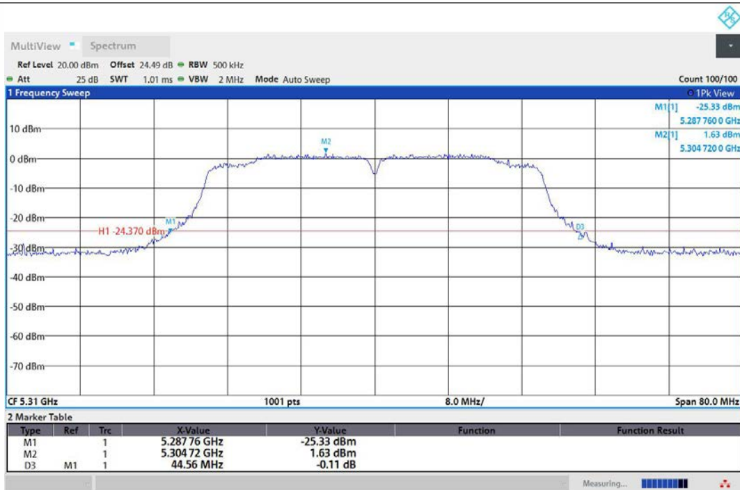
11AC40MIMO-Ant1-5310
