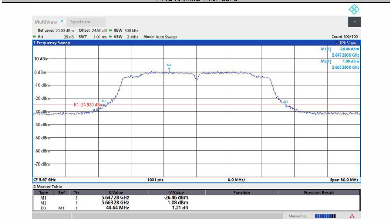
11AC40MIMO-Ant2-5670
