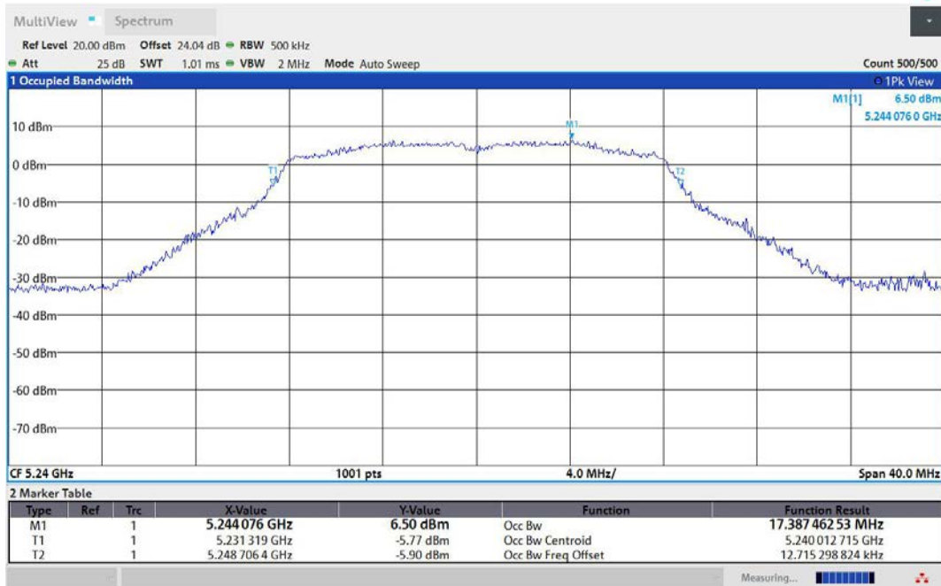
11A-Ant2-5240
