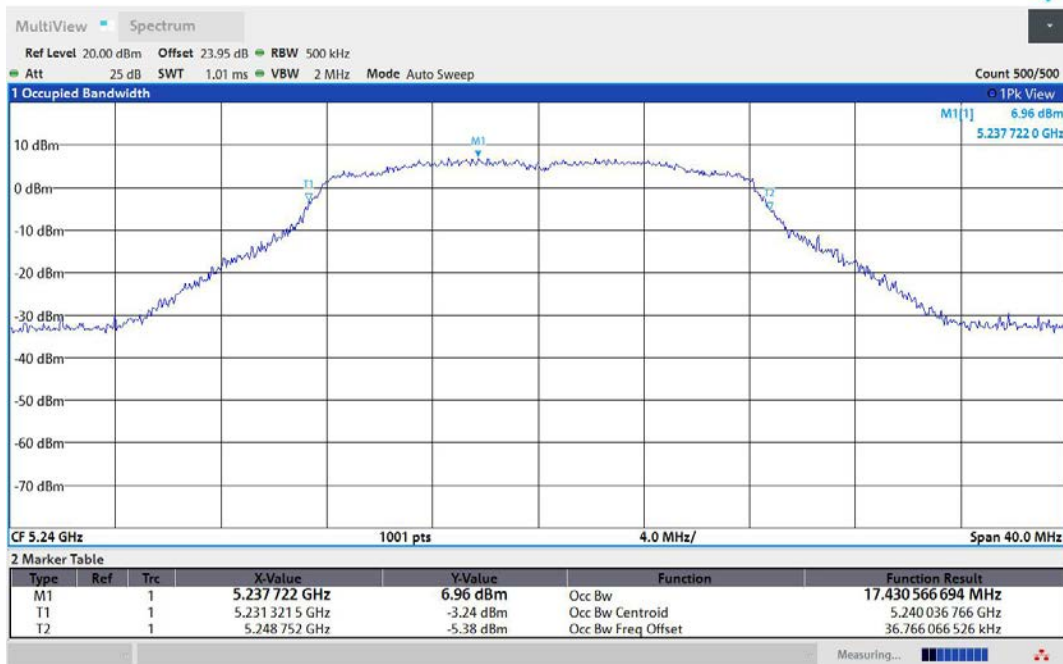
11A-Ant1-5240
