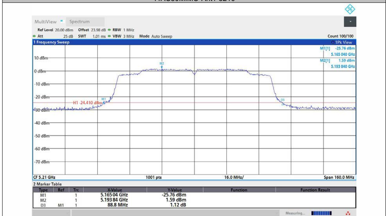
11AC80MIMO-Ant2-5210
