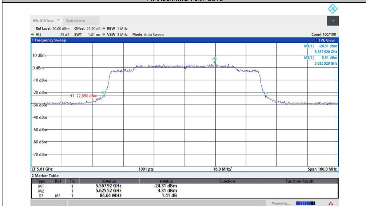
11AX80MIMO-Ant2-5610
