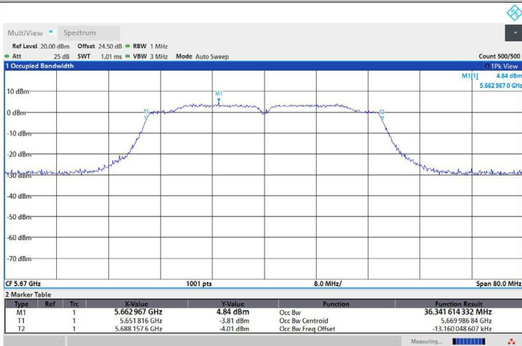
11AC40MIMO-Ant2-5670
