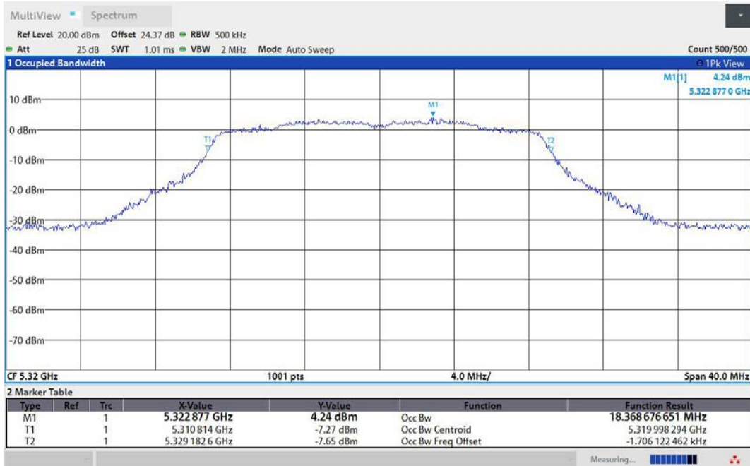
11AC20MIMO-Ant2-5320
