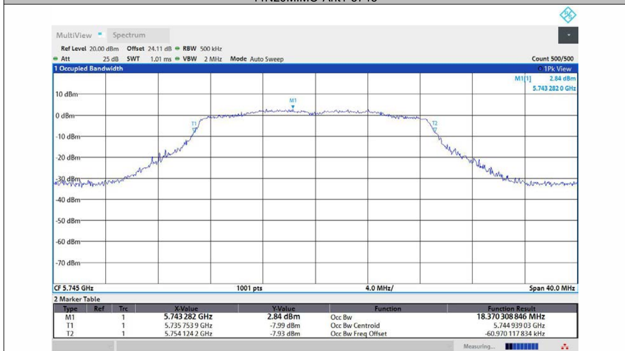
11N20MIMO-Ant2-5745
