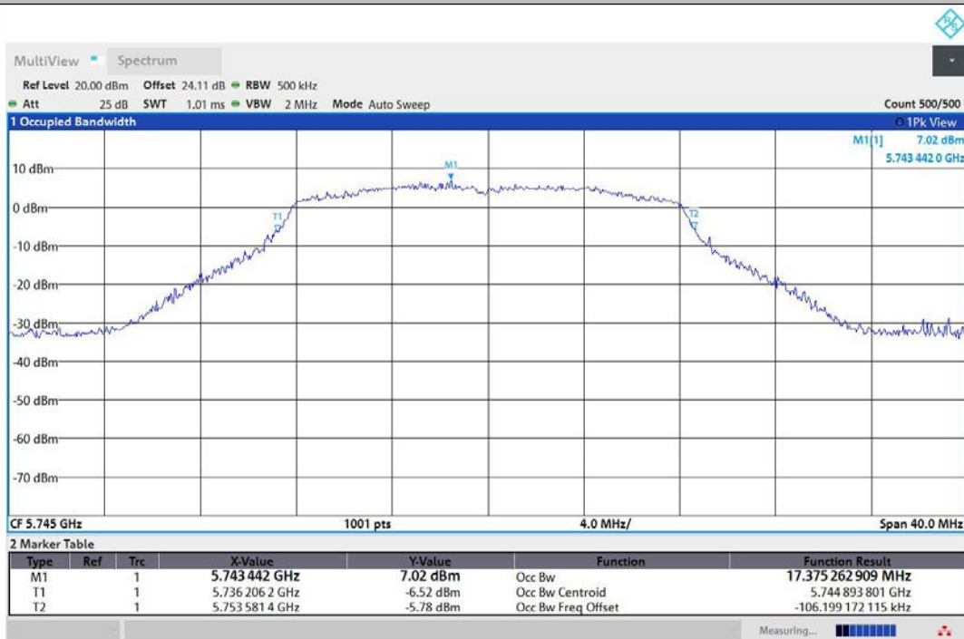
11A-Ant2-5745
