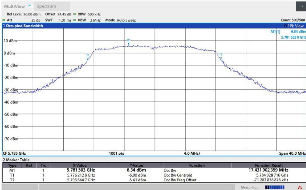
11A-Ant2-5785
