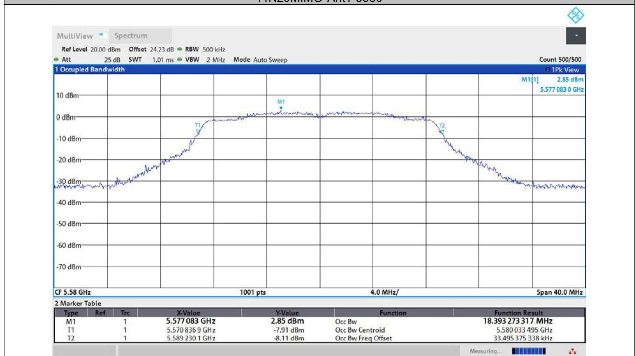
11N20MIMO-Ant2-5580
