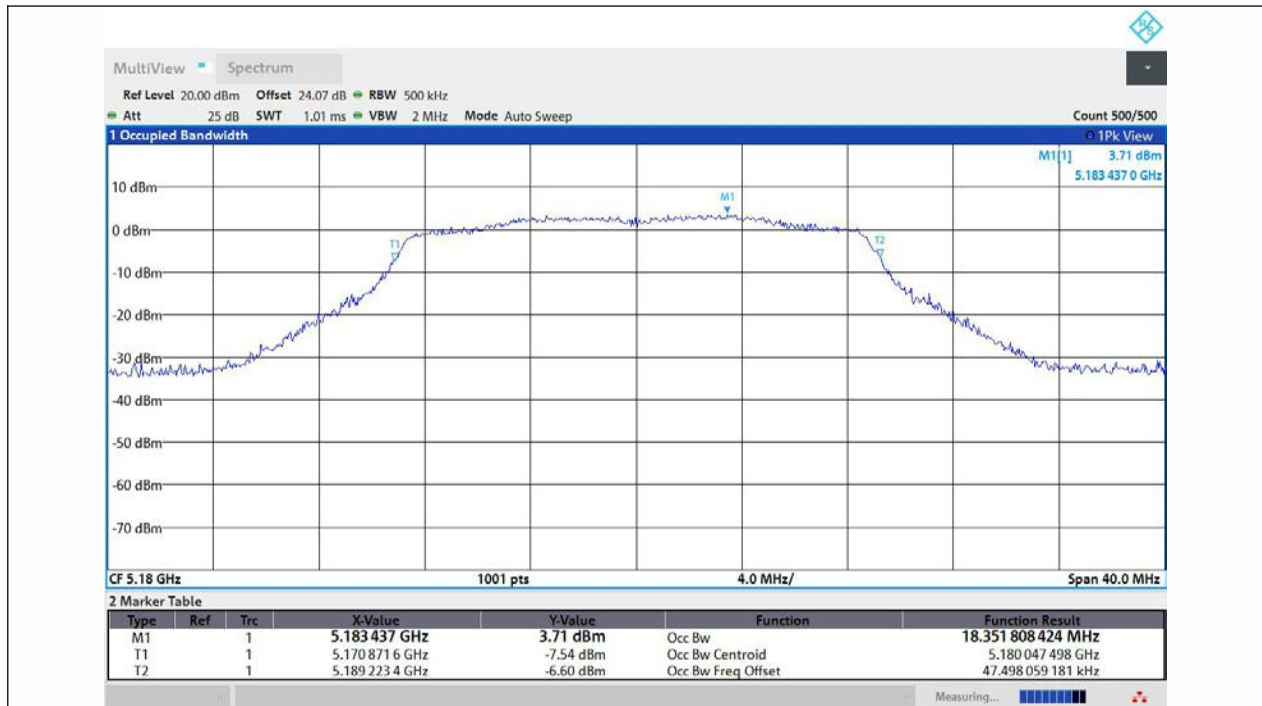
11N20MIMO-Ant1-5180
