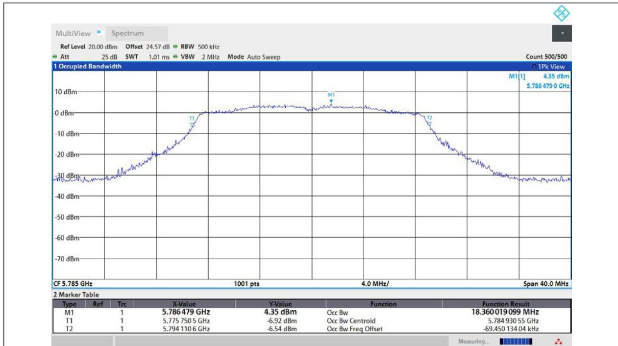
11N20MIMO-Ant1-5785
