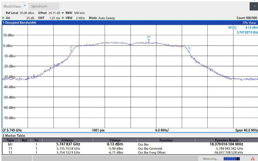
11AC20MIMO-Ant1-5745
