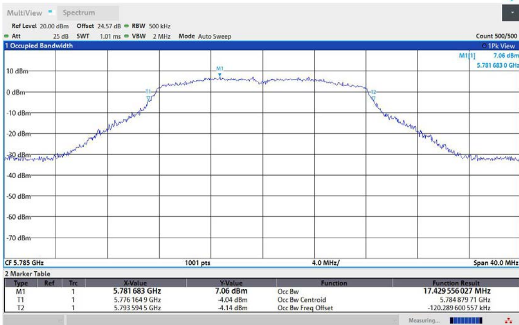
11A-Ant1-5785
