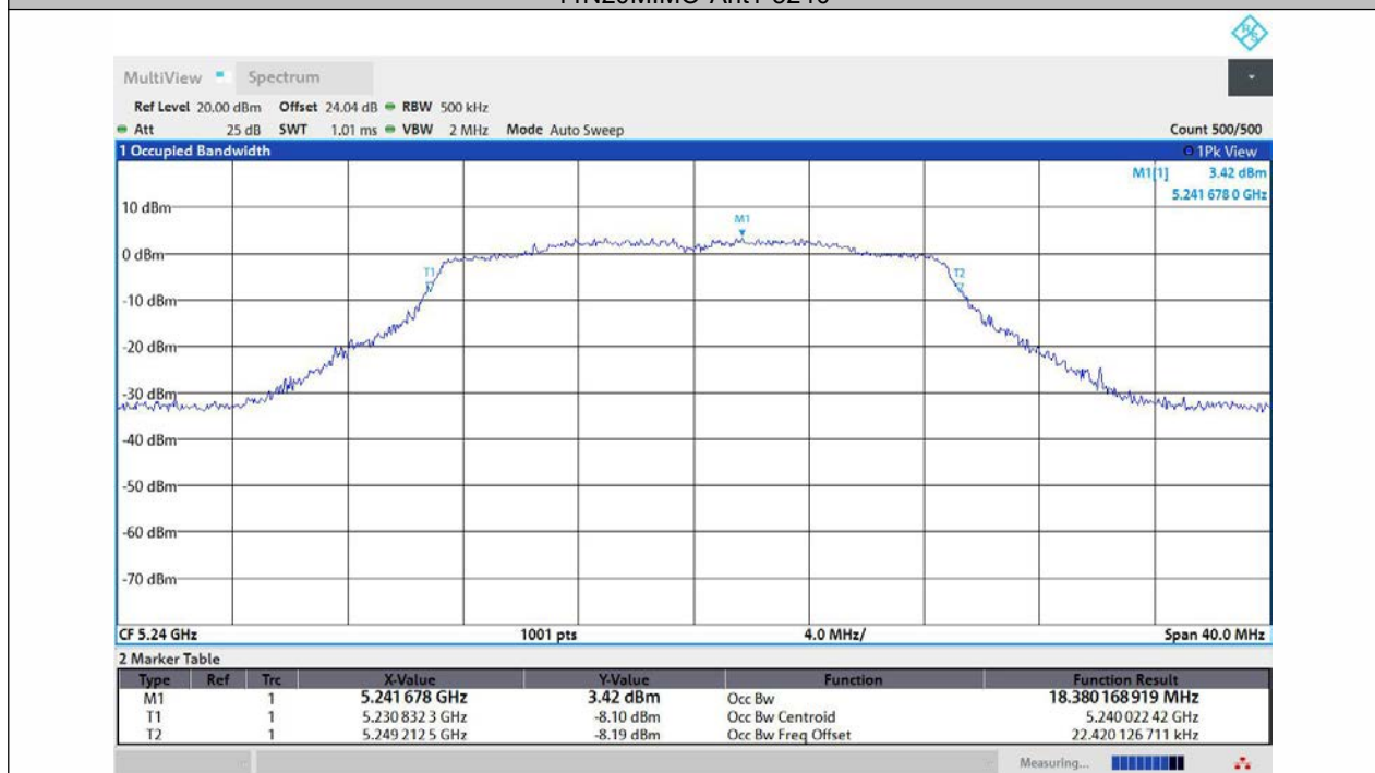
11N20MIMO-Ant2-5240
