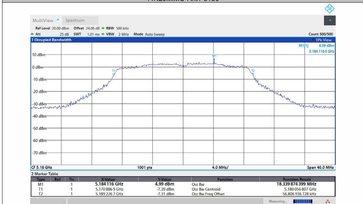
11N20MIMO-Ant2-5180
