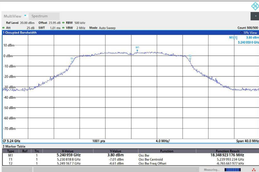
11AC20MIMO-Ant1-5240
