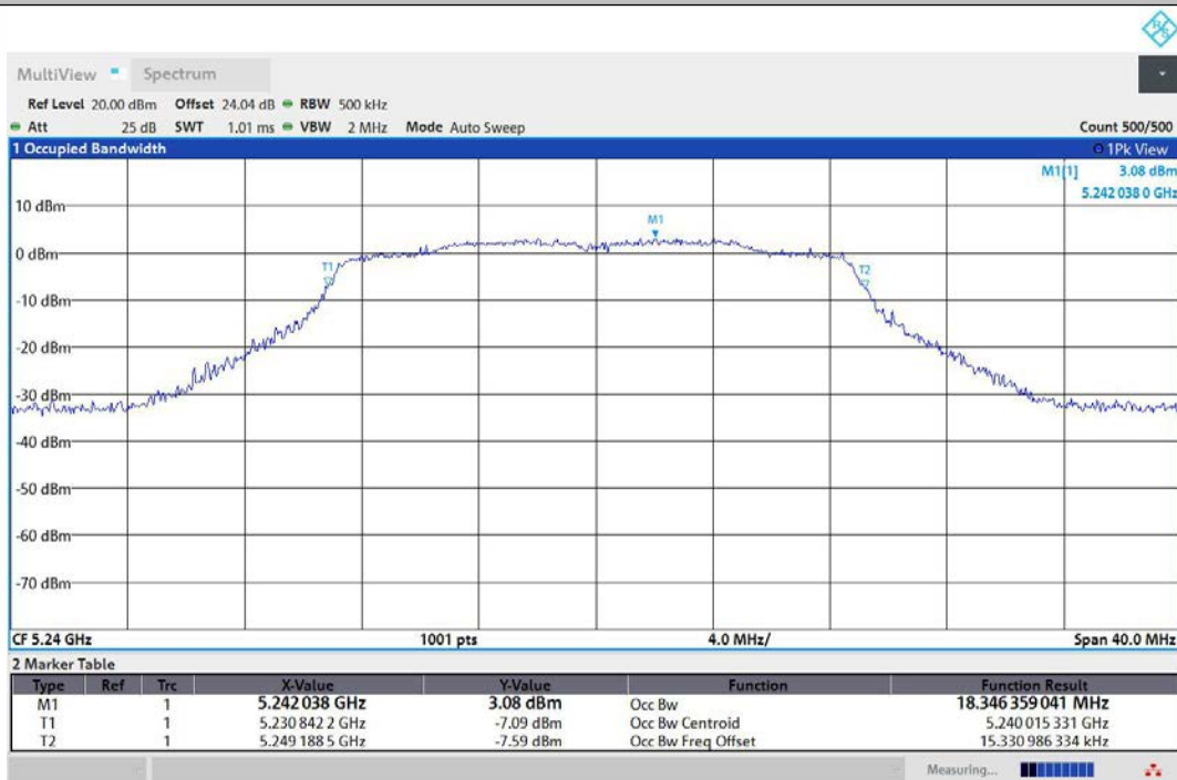
11AC20MIMO-Ant2-5240
