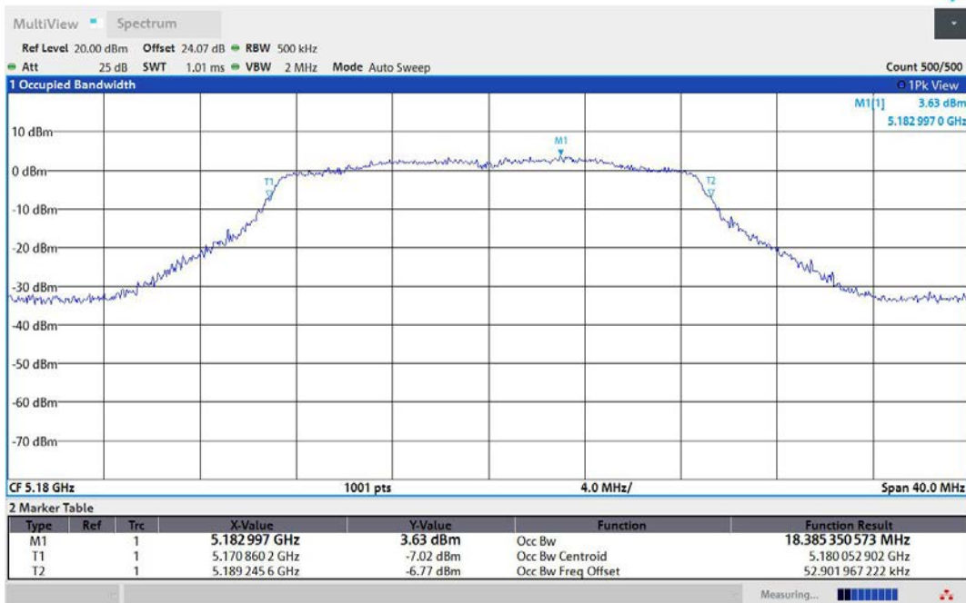
11AC20MIMO-Ant1-5180
