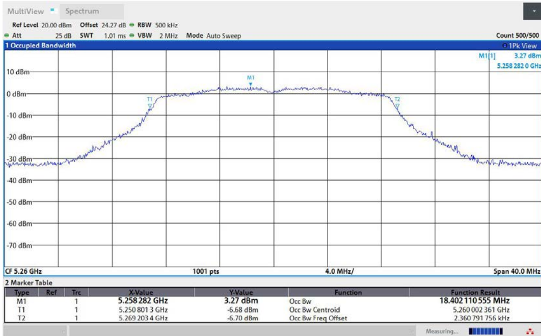
11AC20MIMO-Ant2-5260
