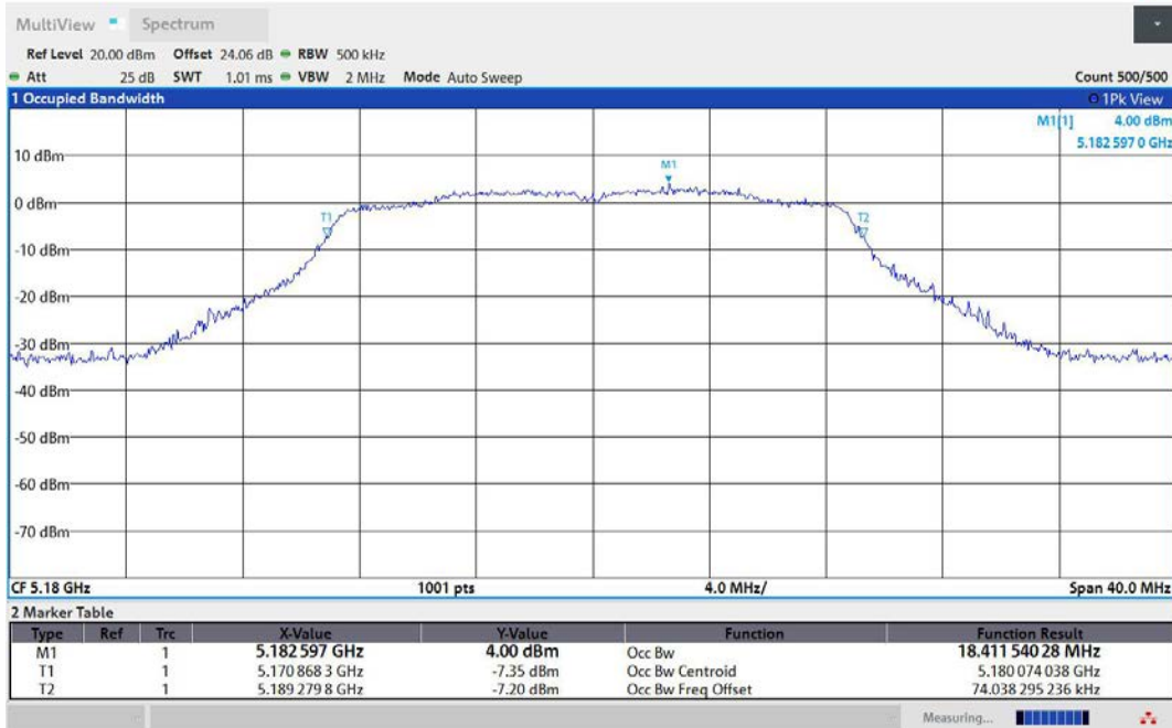
11AC20MIMO-Ant2-5180
