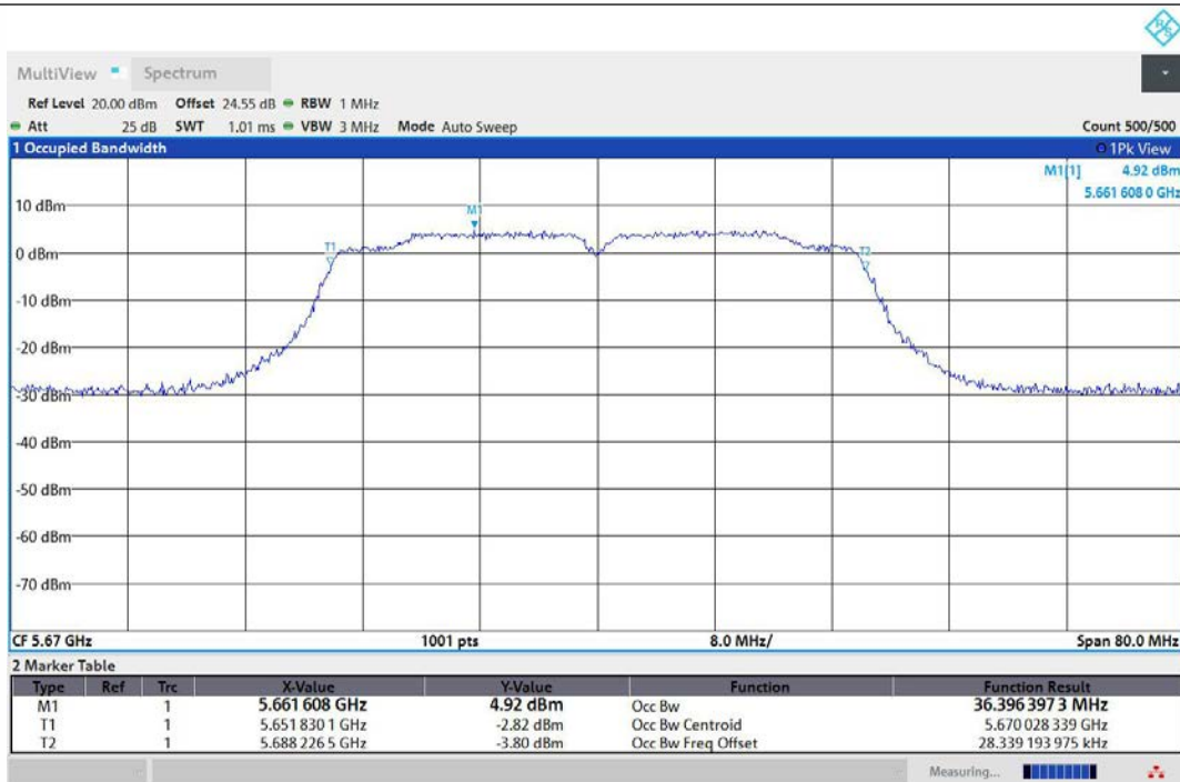
11AC40MIMO-Ant1-5670
