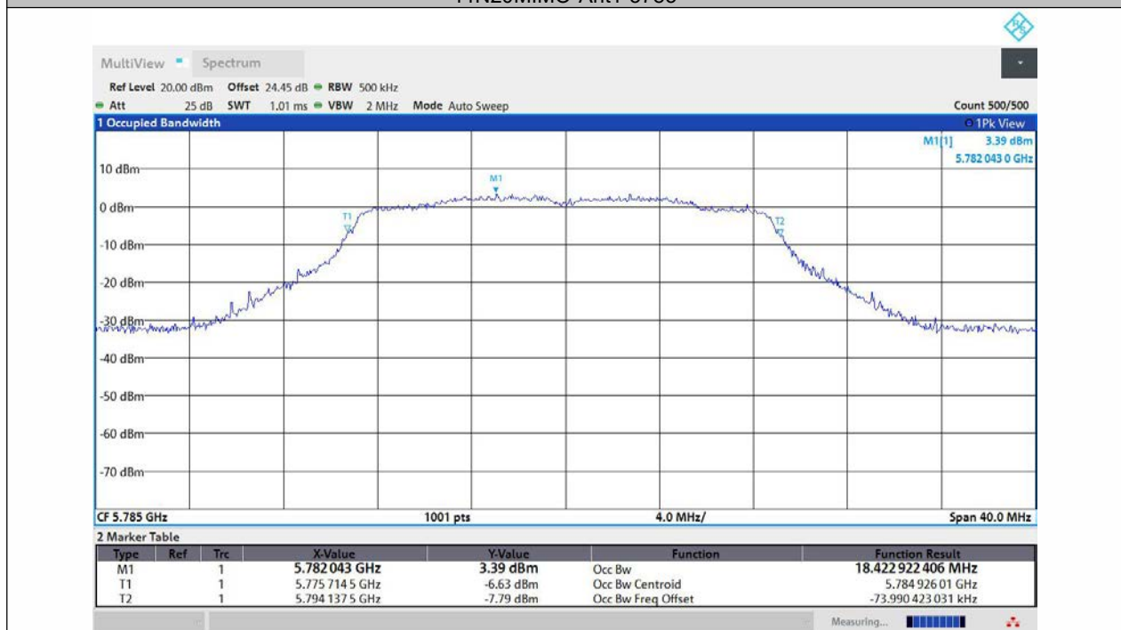
11N20MIMO-Ant2-5785
