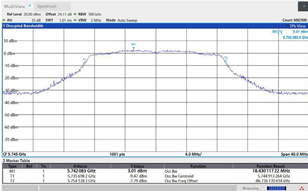
11AC20MIMO-Ant2-5745
