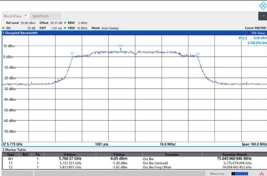
11AC80MIMO-Ant2-5775
