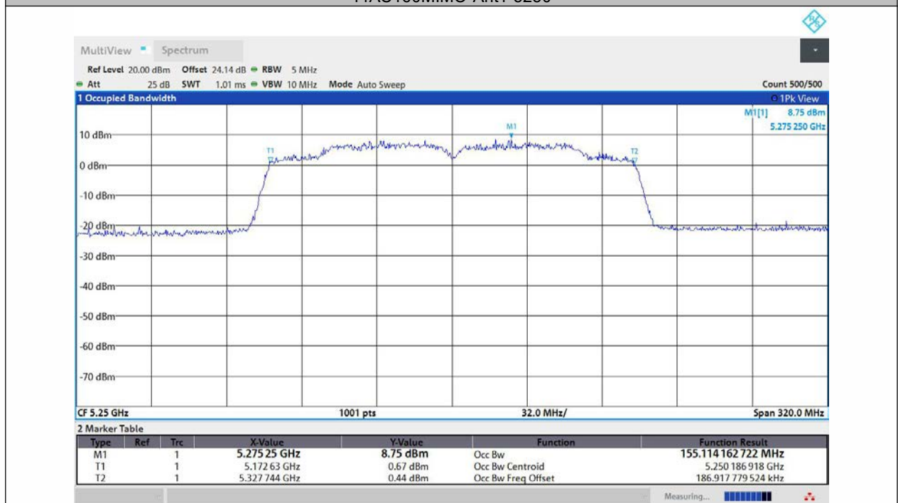
11AC160MIMO-Ant2-5250
