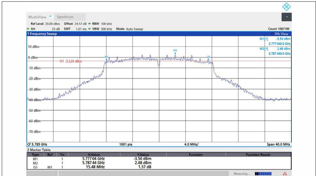
11A-Ant1-5785-PASS
