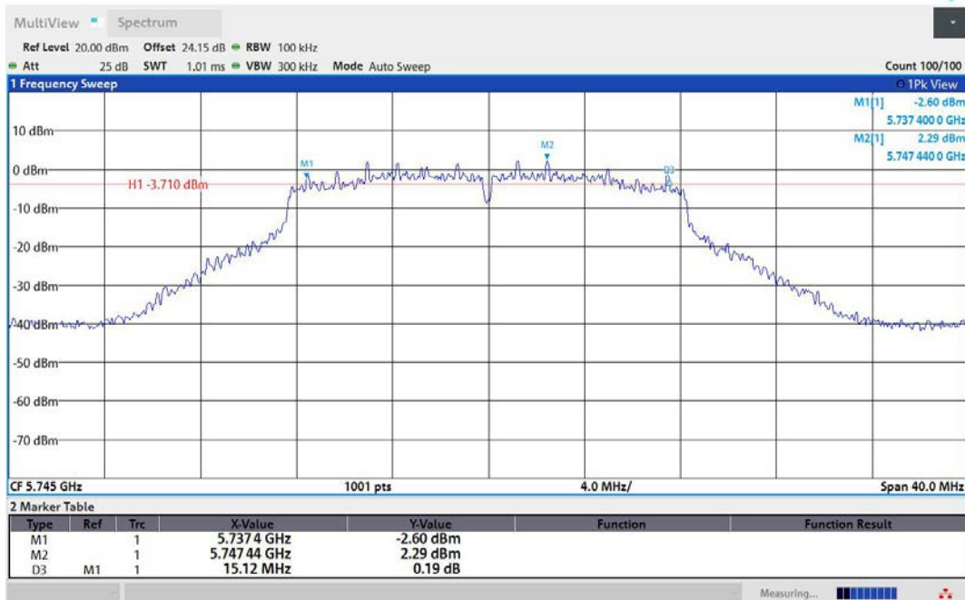
11A-Ant1-5745-PASS
