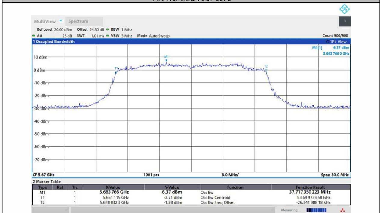
11AX40MIMO-Ant2-5670
