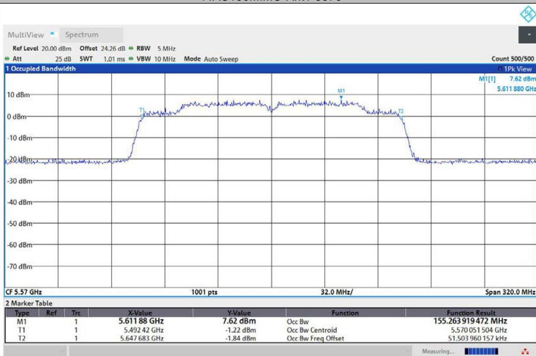
11AC160MIMO-Ant2-5570
