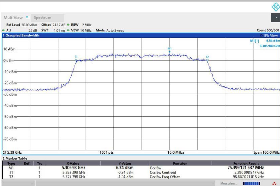
11AC80MIMO-Ant2-5290
