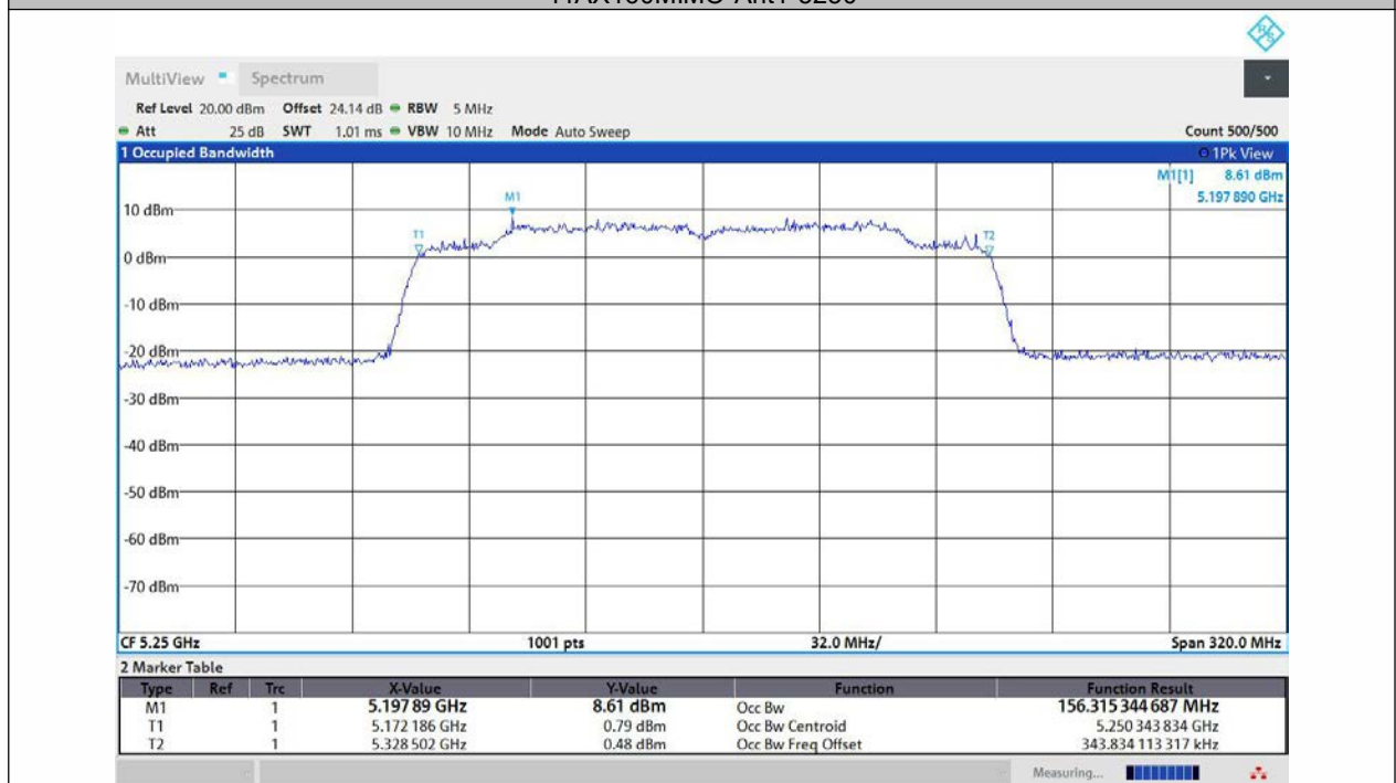
11AX160MIMO-Ant2-5250
