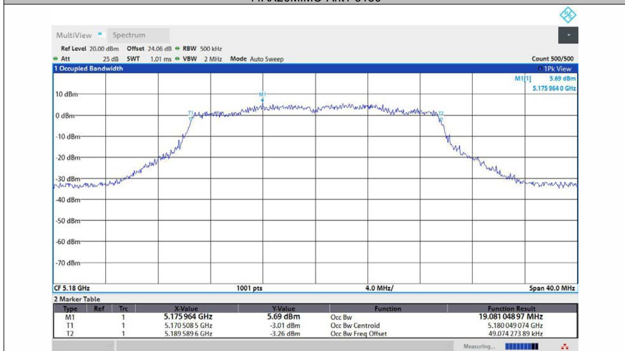
11AX20MIMO-Ant2-5180
