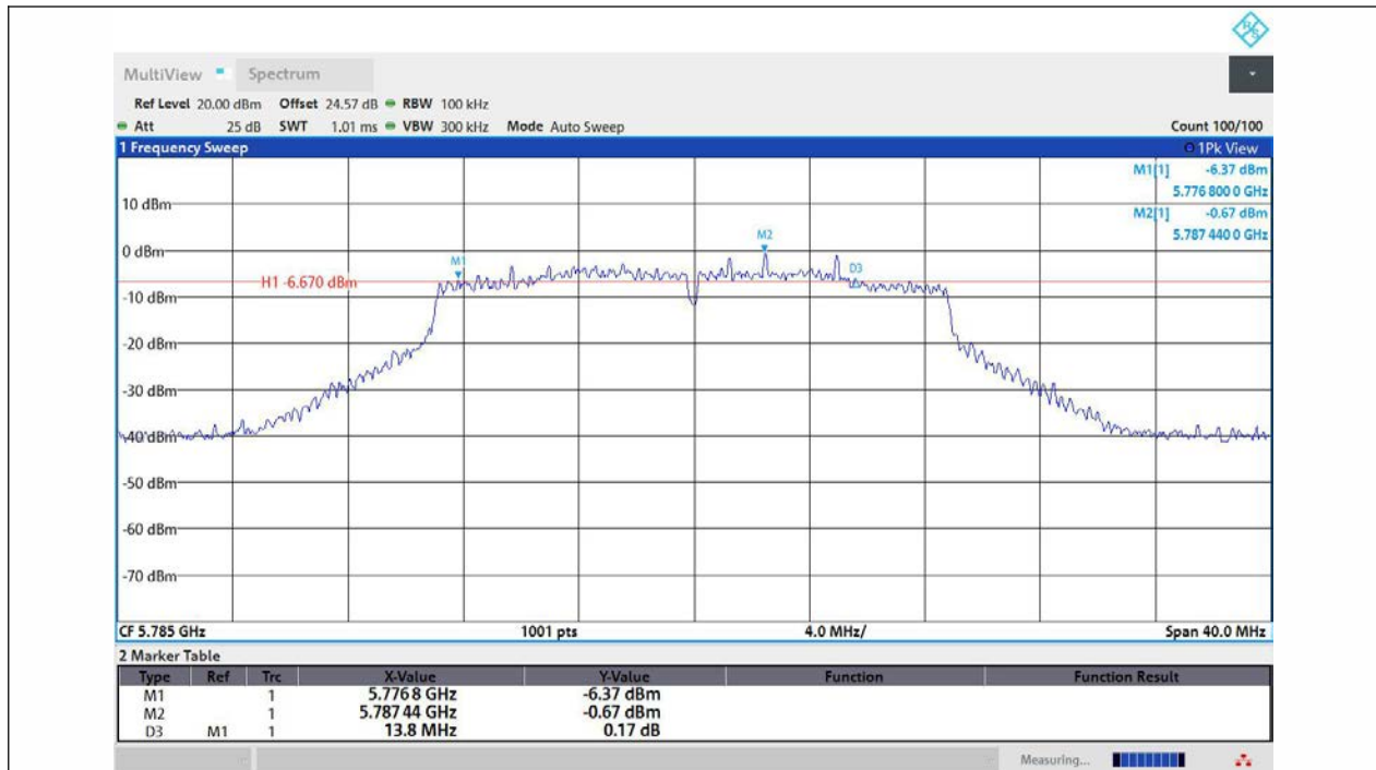
11AC20MIMO-Ant1-5785-PASS
