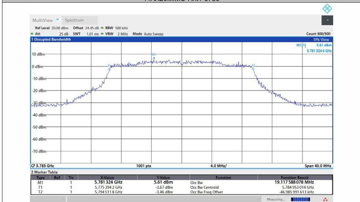
11AX20MIMO-Ant2-5785
