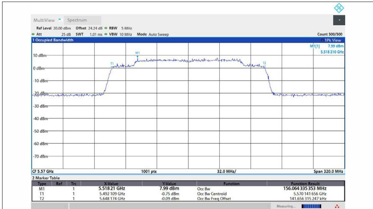
11AX160MIMO-Ant1-5570
