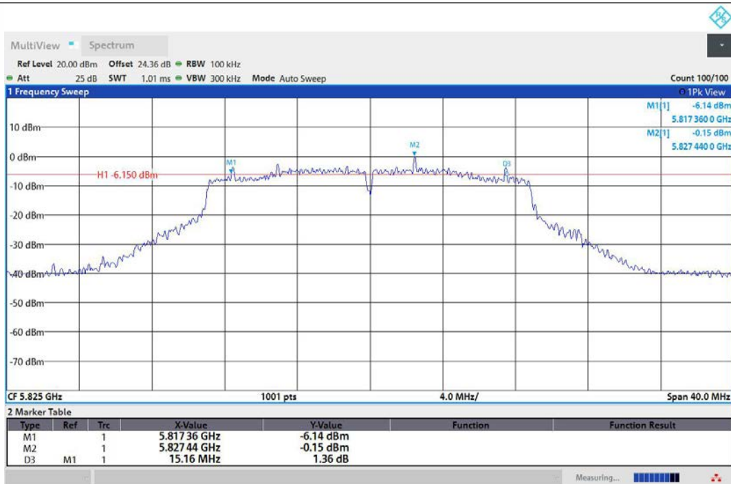
11N20MIMO-Ant1-5825-PASS
