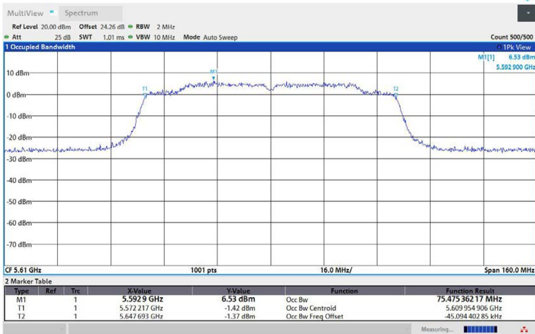
11AC80MIMO-Ant1-5610
