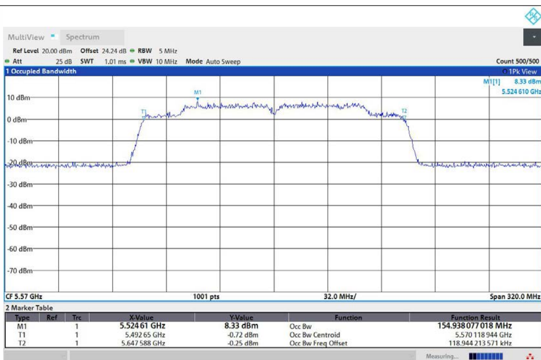
11AC160MIMO-Ant1-5570
