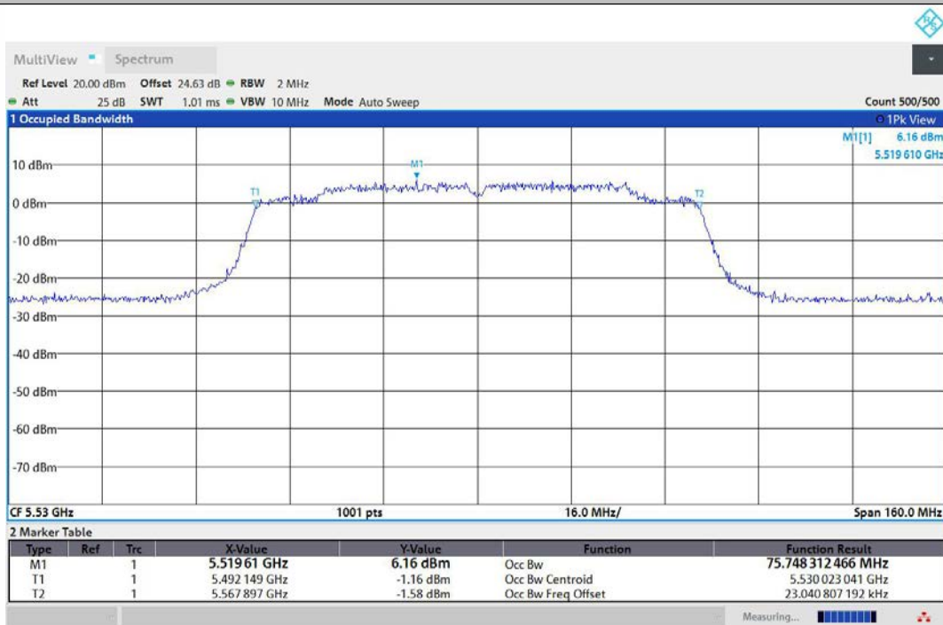
11AC80MIMO-Ant2-5530
