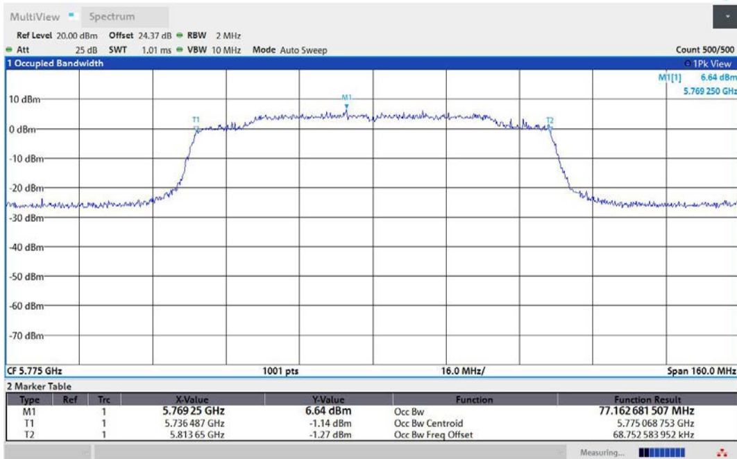
11AX80MIMO-Ant2-5775
