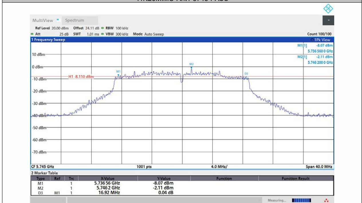
11N20MIMO-Ant2-5745-PASS
