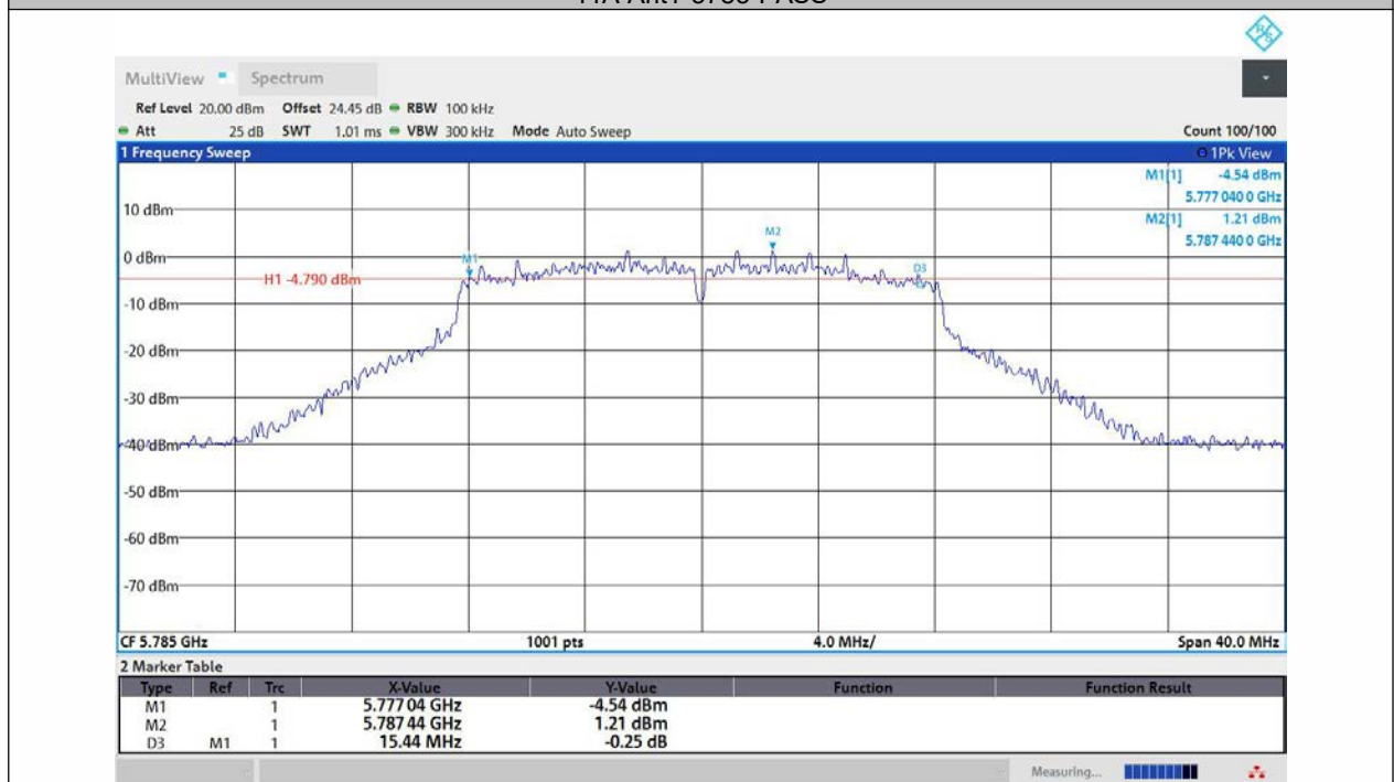
11A-Ant2-5785-PASS
