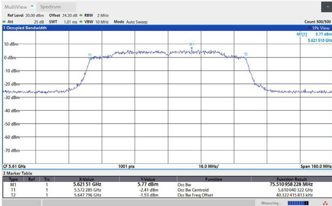
11AC80MIMO-Ant2-5610
