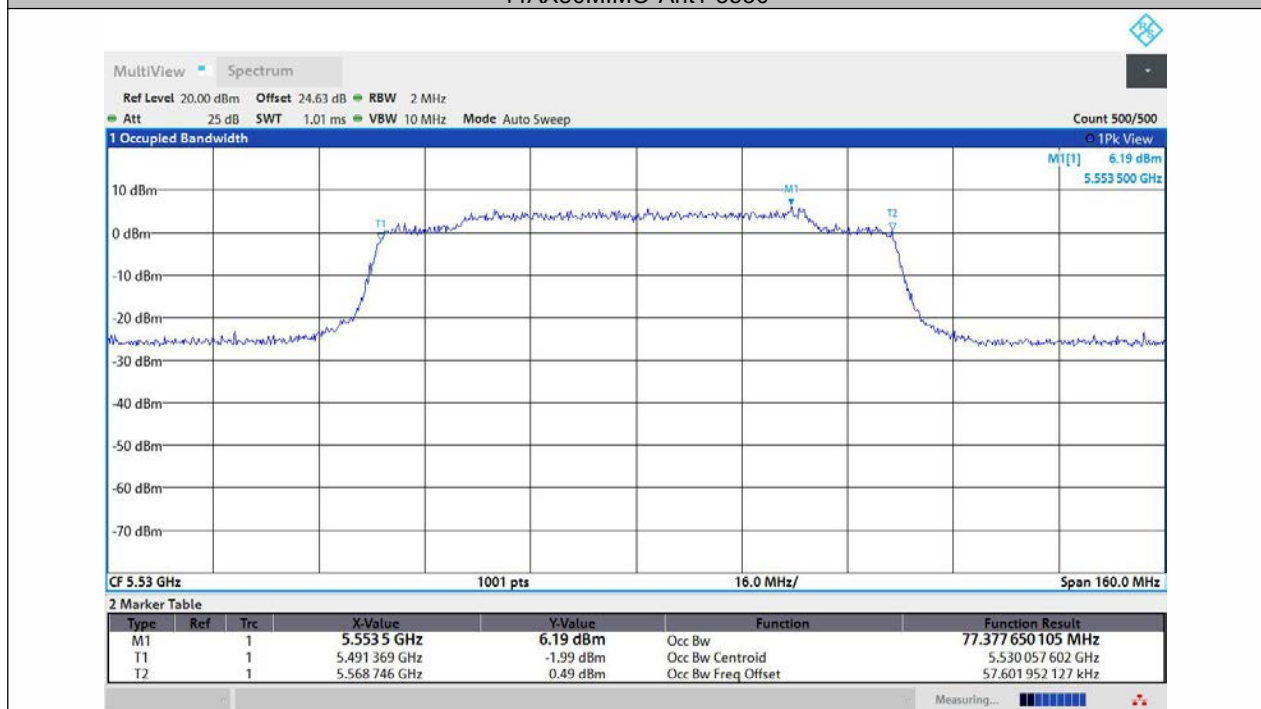
11AX80MIMO-Ant2-5530
