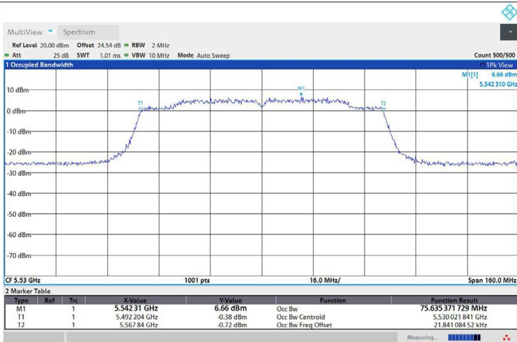
11AC80MIMO-Ant1-5530
