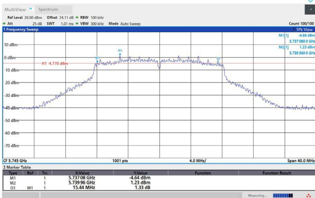
11A-Ant2-5745-PASS
