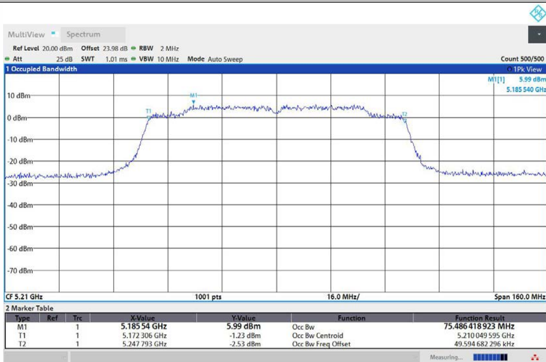
11AC80MIMO-Ant2-5210
