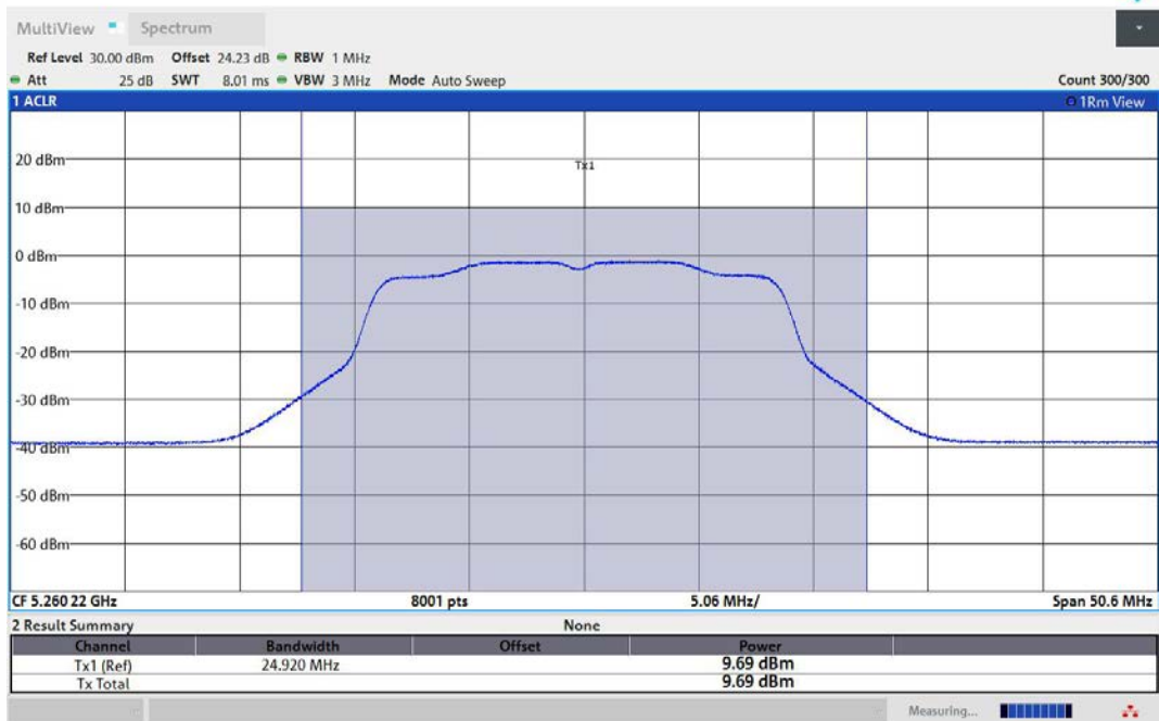
11N20MIMO-Ant1-5260-PASS
