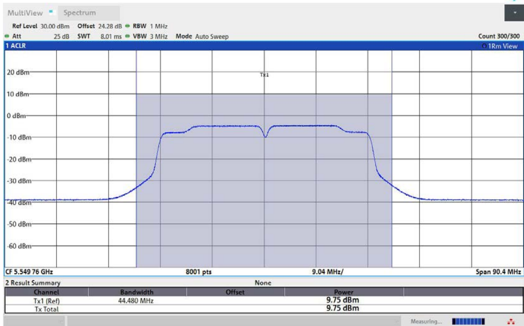
11N40MIMO-Ant1-5550-PASS
