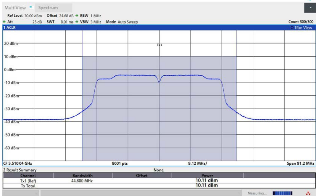
11N40MIMO-Ant1-5510-PASS
