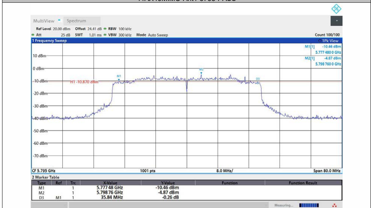
11AX40MIMO-Ant2-5795-PASS
