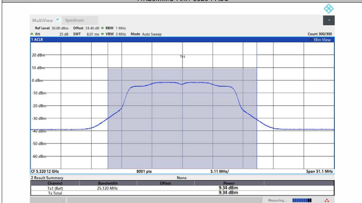
11N20MIMO-Ant2-5320-PASS
