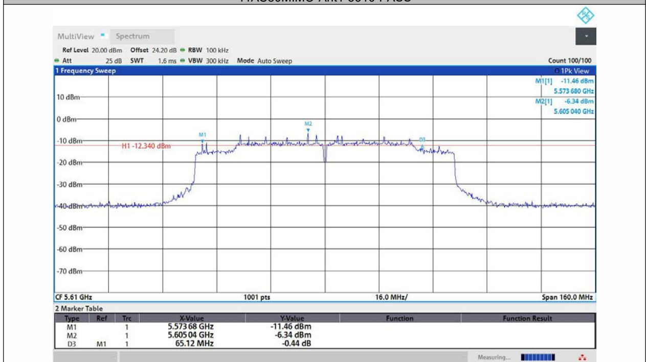
11AC80MIMO-Ant2-5610-PASS
