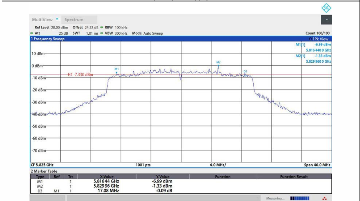
11AX20MIMO-Ant2-5825-PASS
