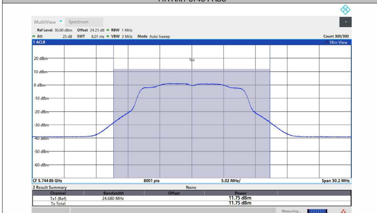
11A-Ant2-5745-PASS
