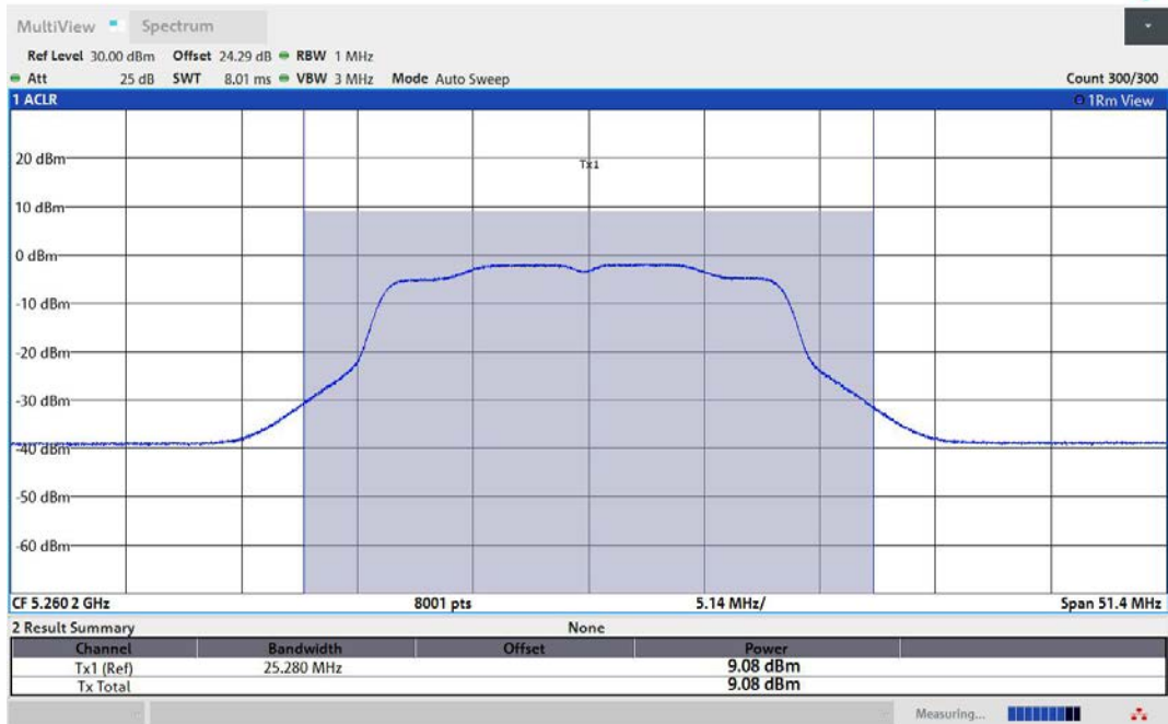
11N20MIMO-Ant2-5260-PASS
