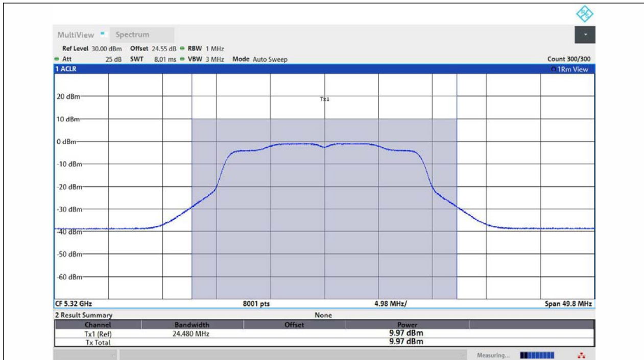
11N20MIMO-Ant1-5320-PASS
