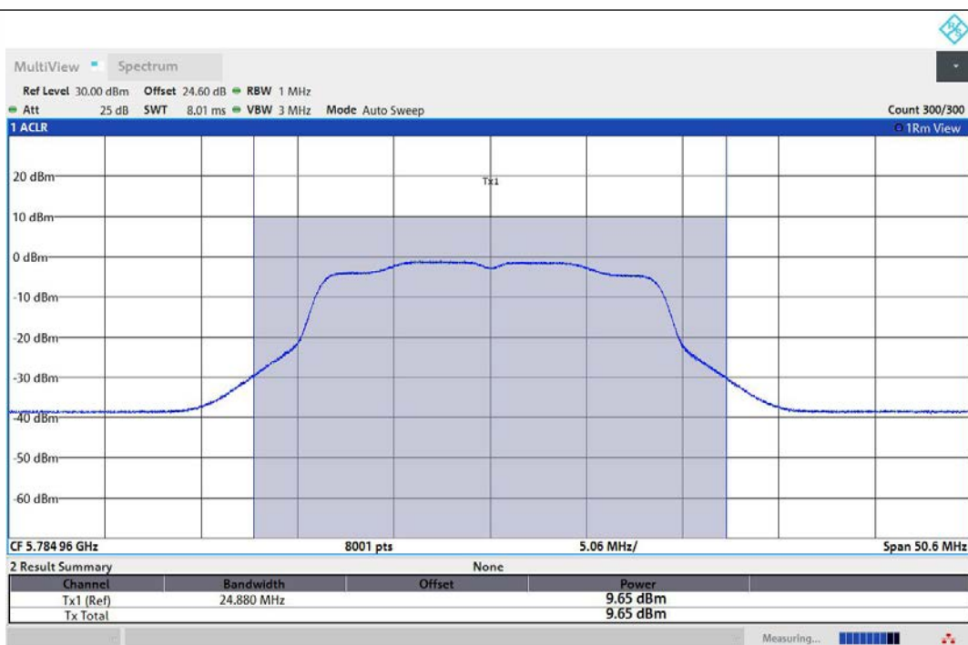
11N20MIMO-Ant1-5785-PASS
