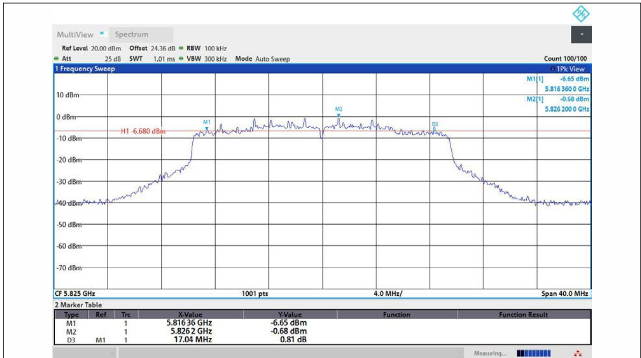
11AX20MIMO-Ant1-5825-PASS
