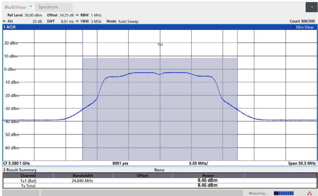
11N20MIMO-Ant2-5580-PASS
