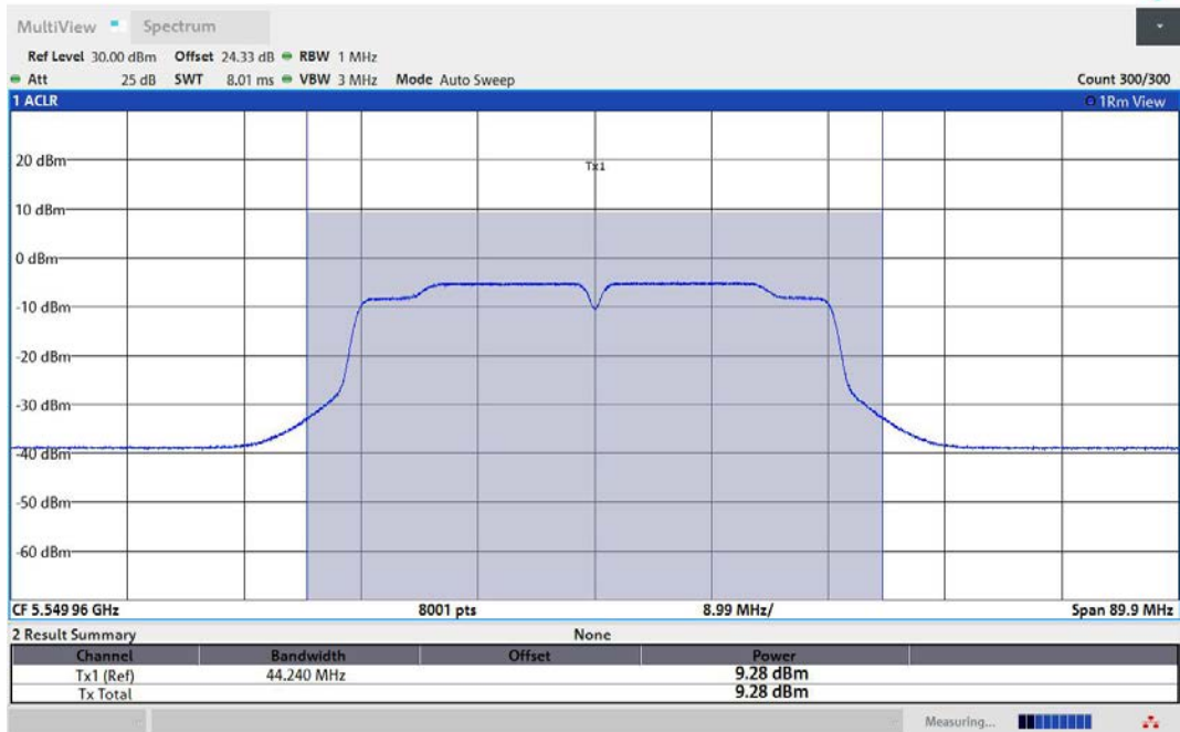
11N40MIMO-Ant2-5550-PASS
