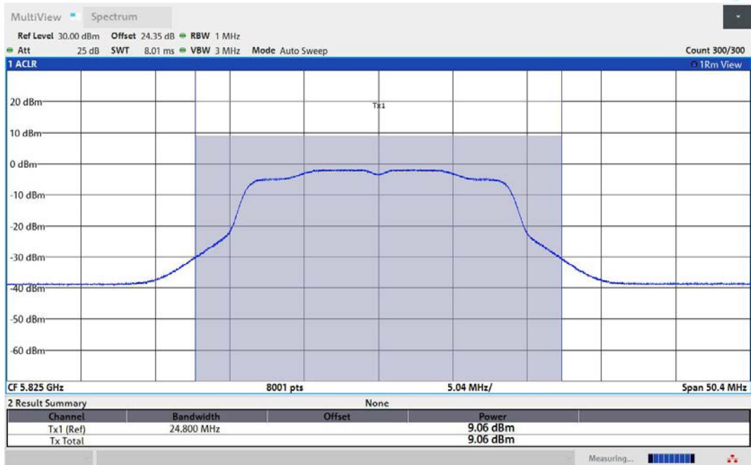
11N20MIMO-Ant2-5825-PASS
