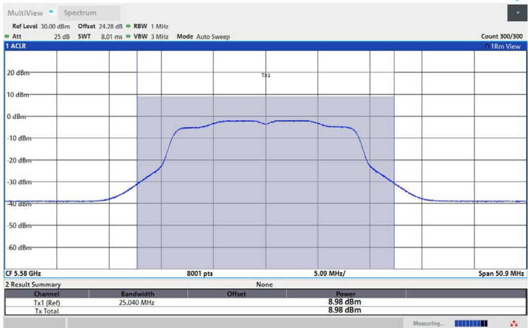
11N20MIMO-Ant1-5580-PASS
