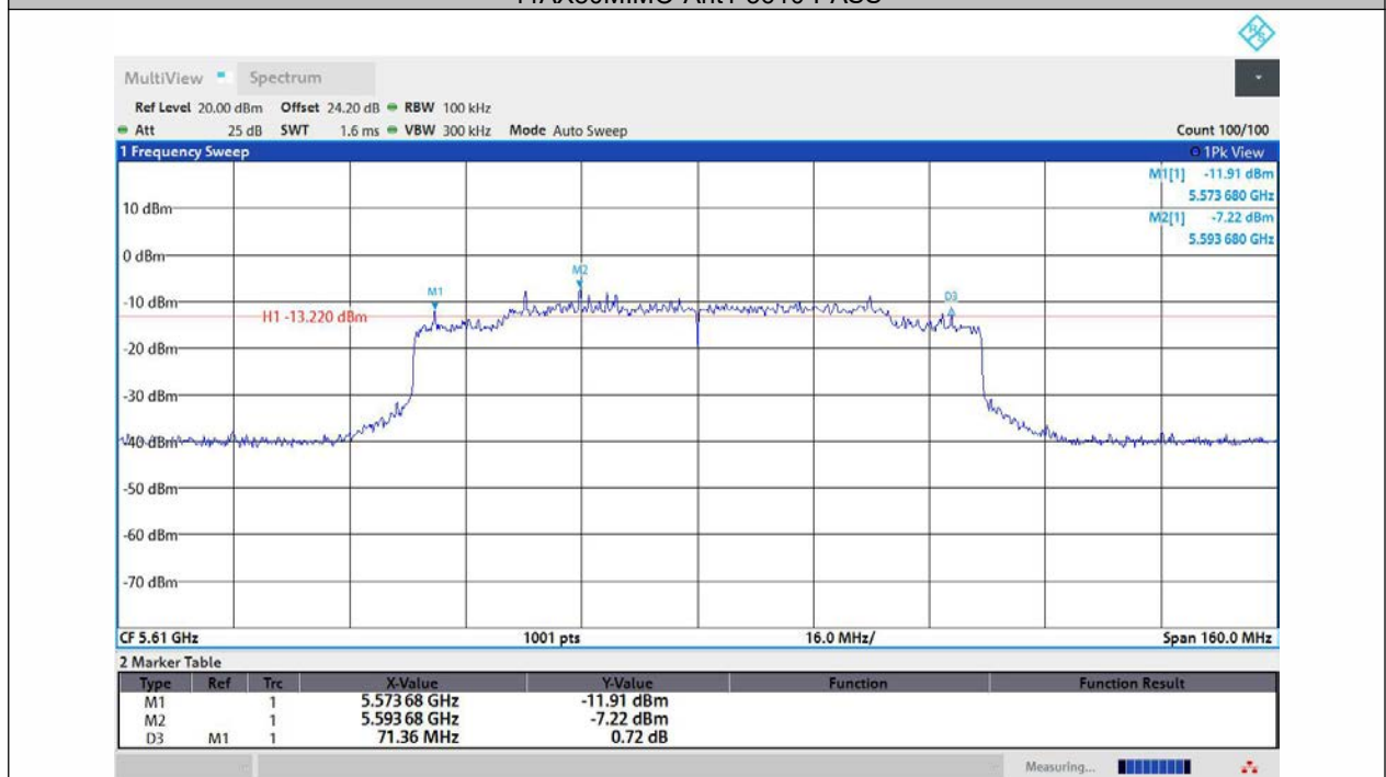
11AX80MIMO-Ant2-5610-PASS
