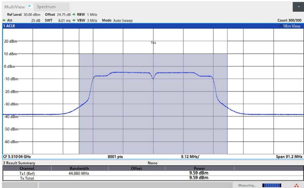
11N40MIMO-Ant2-5510-PASS
