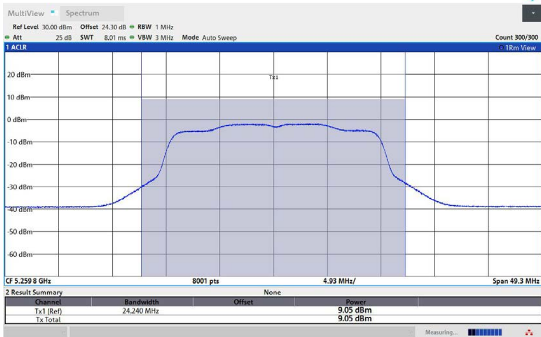
11AX20MIMO-Ant2-5260-PASS
