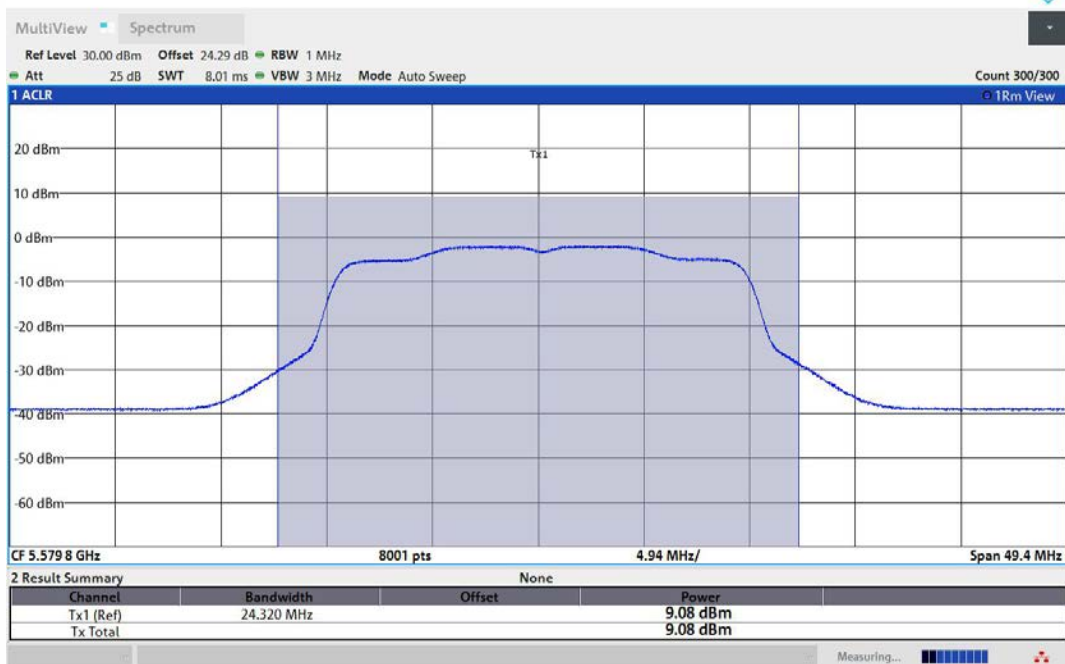
11AX20MIMO-Ant1-5580-PASS
