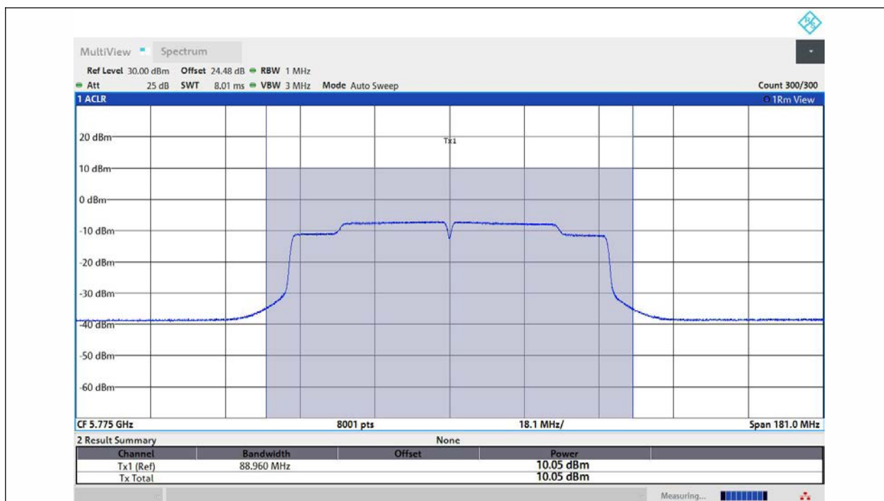
11AC80MIMO-Ant1-5775-PASS
