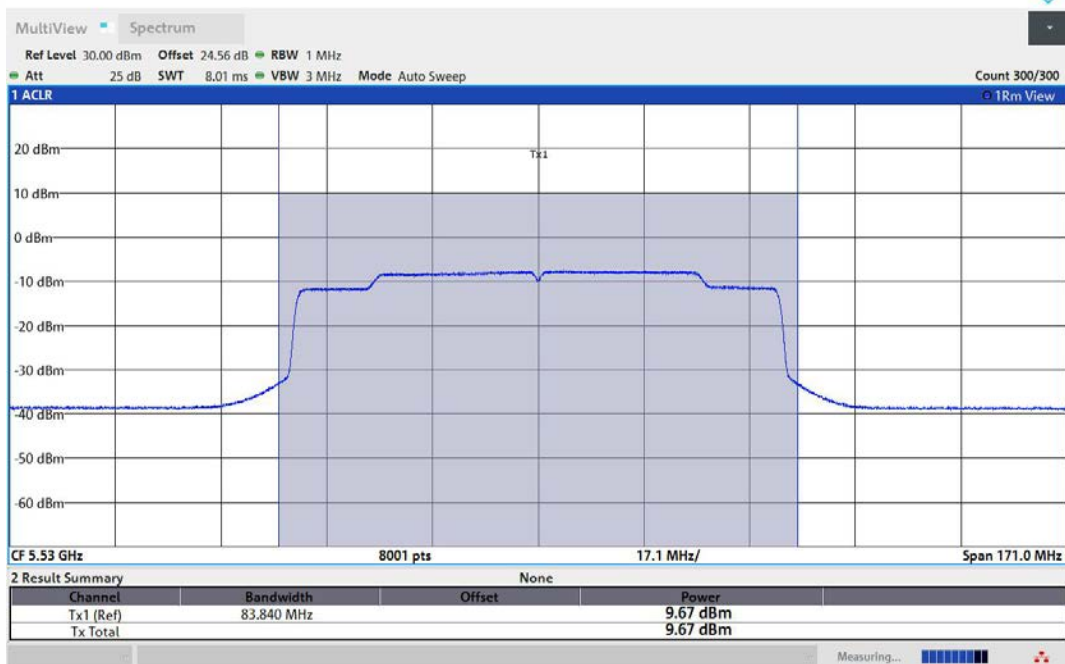
11AX80MIMO-Ant1-5530-PASS
