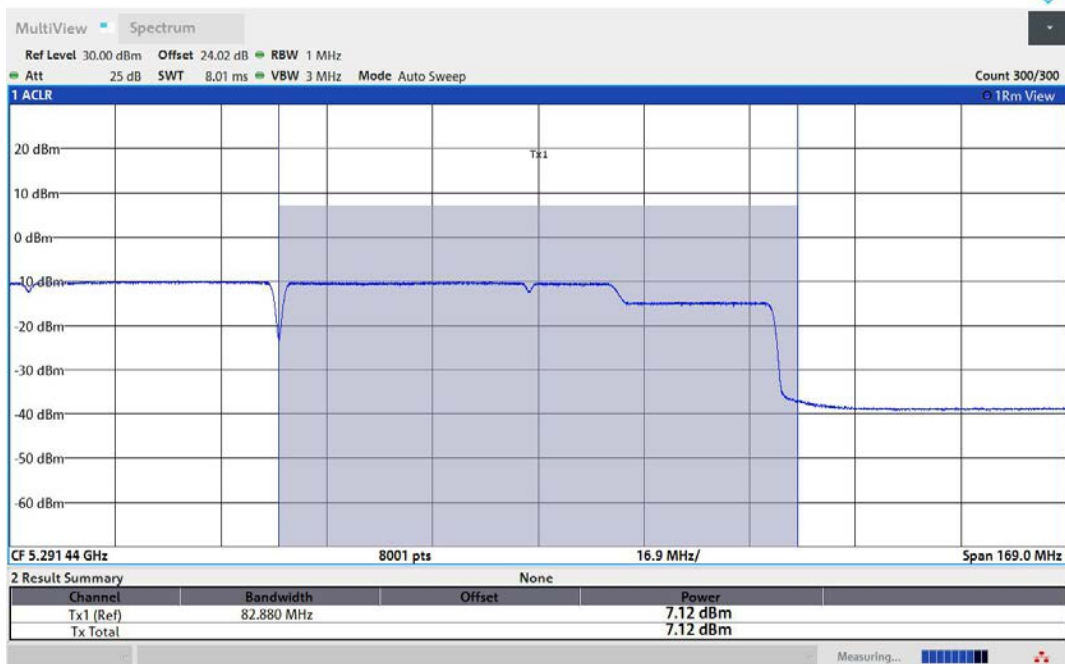
11AX160MIMO-Ant1-5250_UNII-2A-PASS
