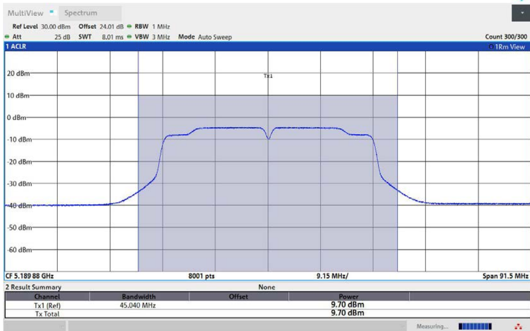
11AC40MIMO-Ant2-5190-PASS
