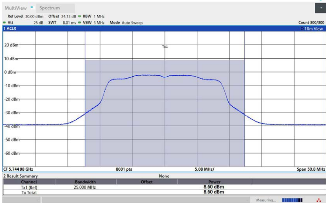
11AC20MIMO-Ant2-5745-PASS
