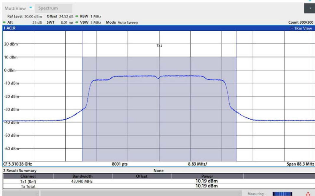
11AX40MIMO-Ant1-5310-PASS
