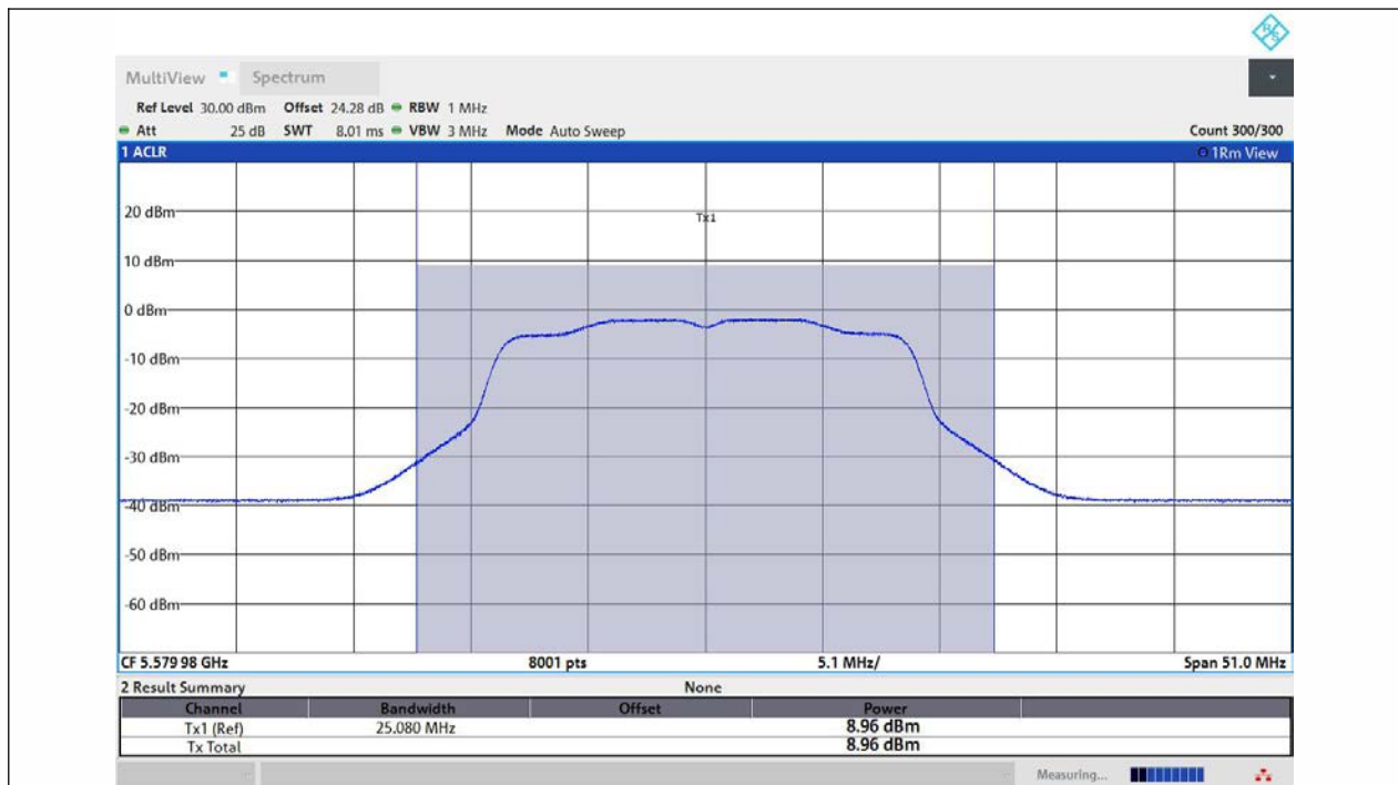
11AC20MIMO-Ant1-5580-PASS
