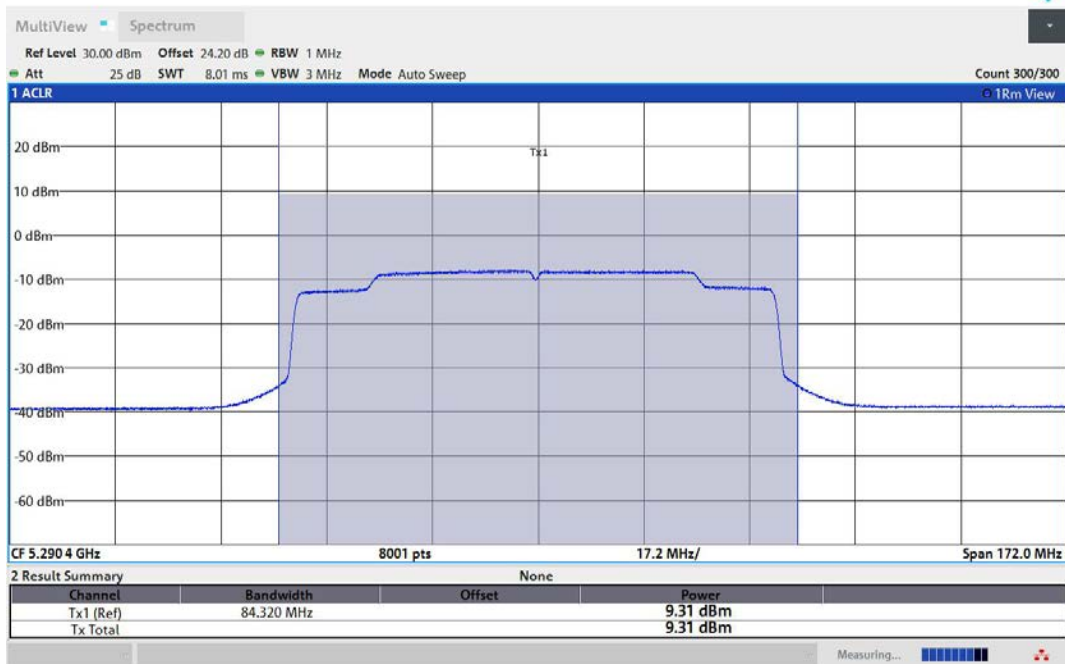
11AX80MIMO-Ant2-5290-PASS
