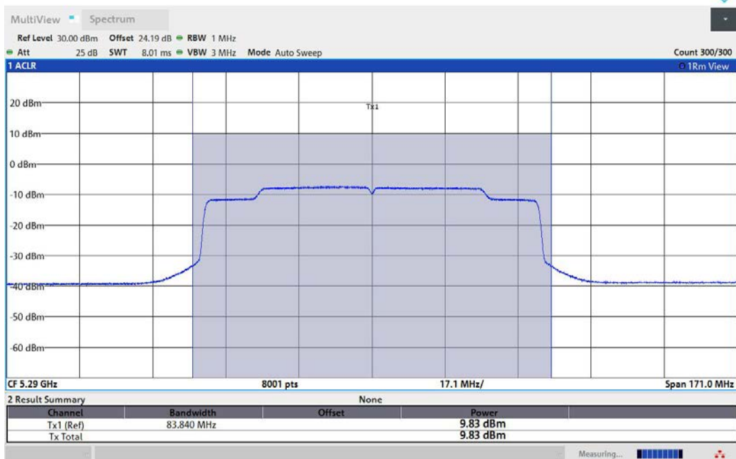
11AX80MIMO-Ant1-5290-PASS
