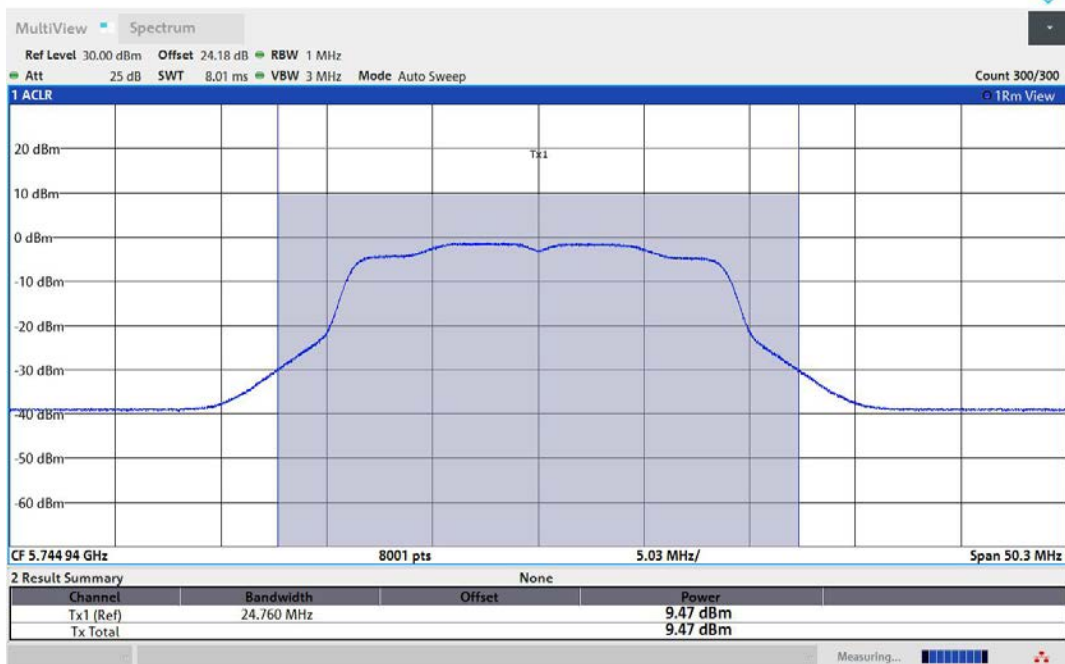
11AC20MIMO-Ant1-5745-PASS
