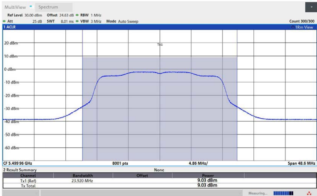
11AX20MIMO-Ant2-5500-PASS
