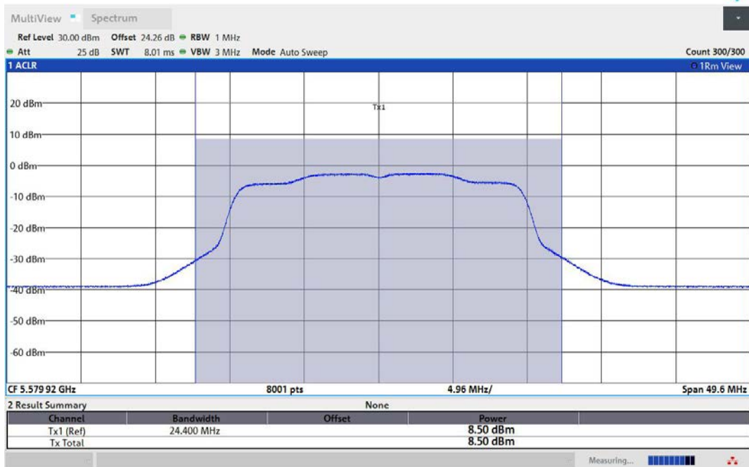
11AX20MIMO-Ant2-5580-PASS
