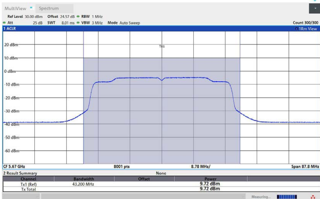
11AX40MIMO-Ant1-5670-PASS
