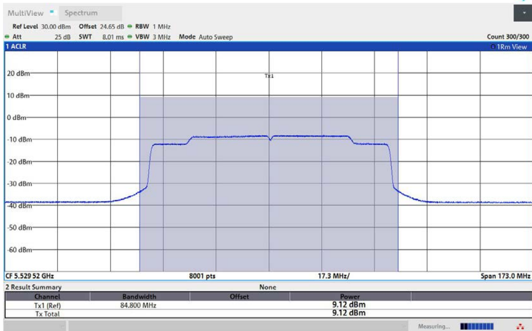
11AX80MIMO-Ant2-5530-PASS
