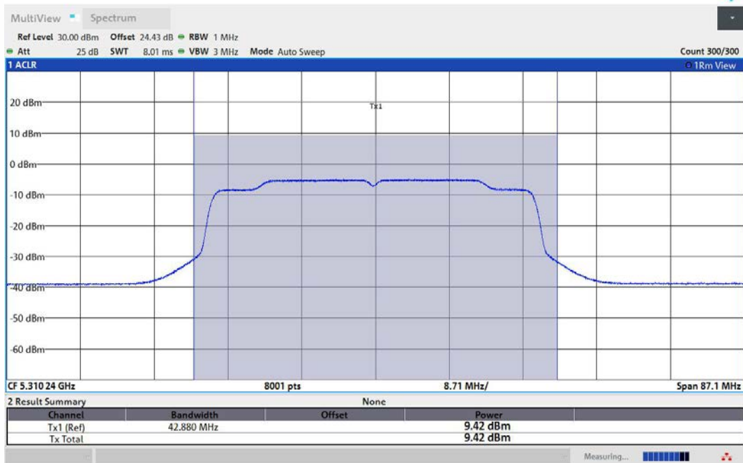
11AX40MIMO-Ant2-5310-PASS
