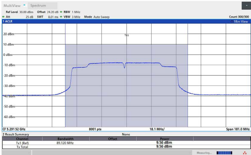
11AC80MIMO-Ant2-5290-PASS
