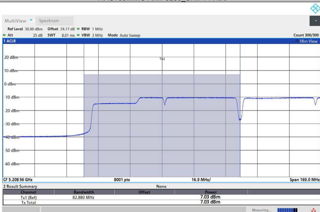
11AC160MIMO-Ant2-5250_UNII-1-PASS
