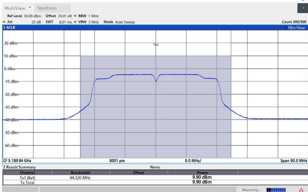
11AC40MIMO-Ant1-5190-PASS
