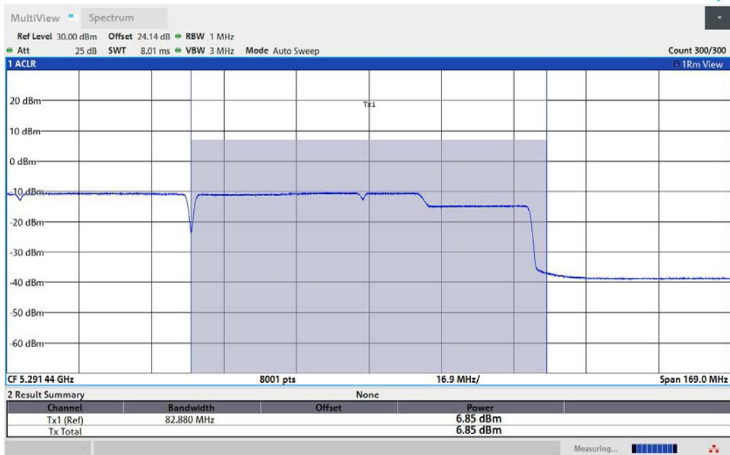
11AX160MIMO-Ant2-5250_UNII-2A-PASS
