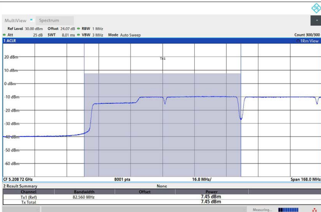
11AC160MIMO-Ant1-5250_UNII-1-PASS
