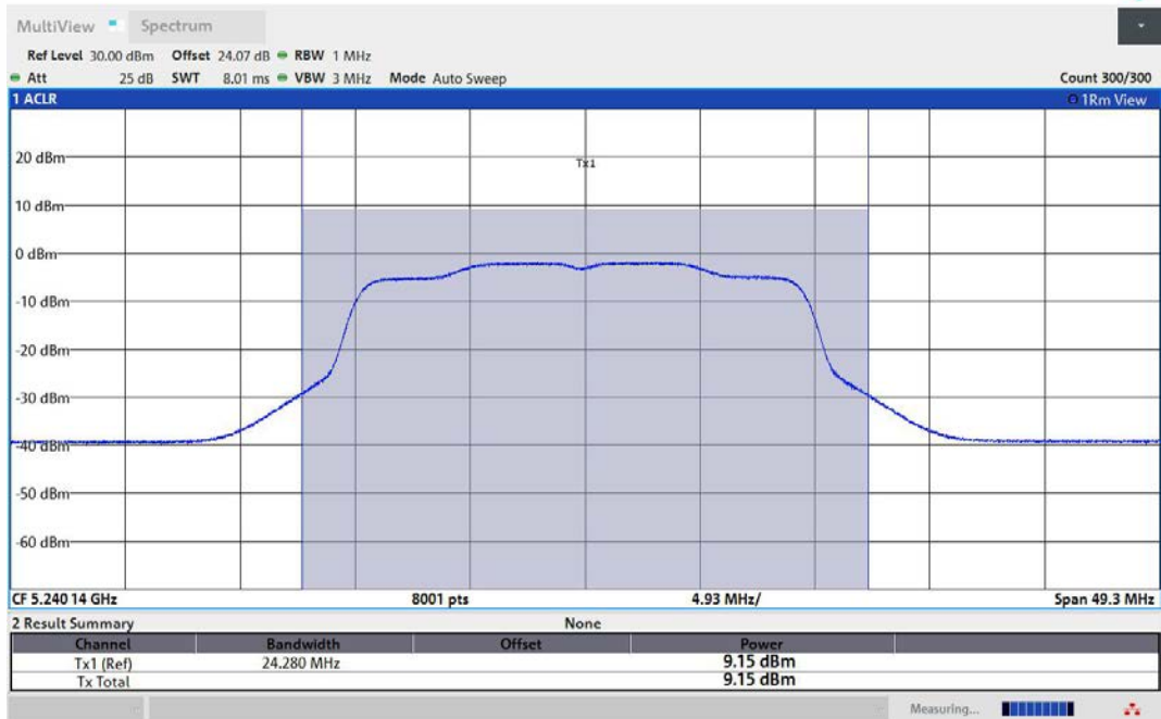
11AX20MIMO-Ant2-5240-PASS
