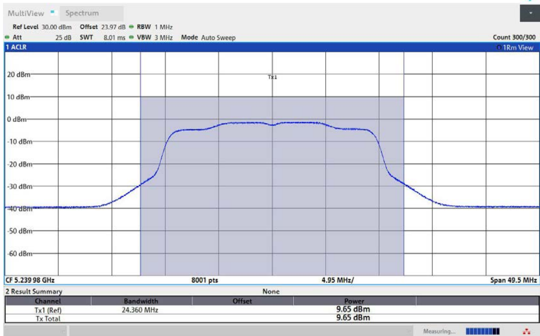
11AX20MIMO-Ant1-5240-PASS
