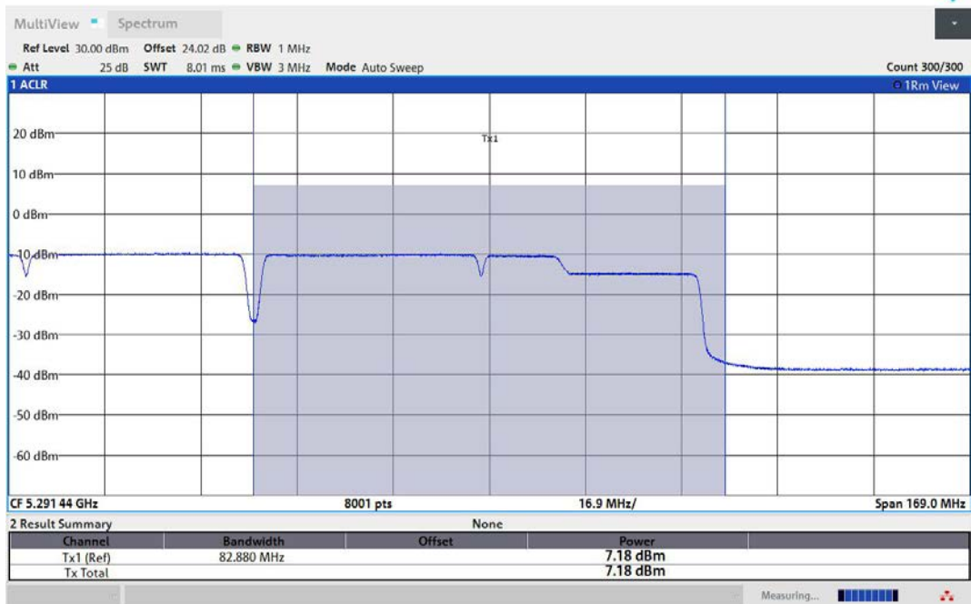
11AC160MIMO-Ant1-5250_UNII-2A-PASS
