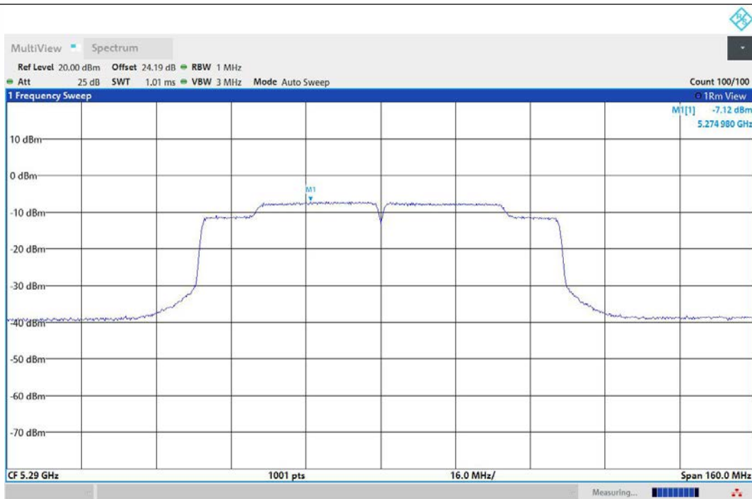
11AC80MIMO-Ant1-5290-PASS
