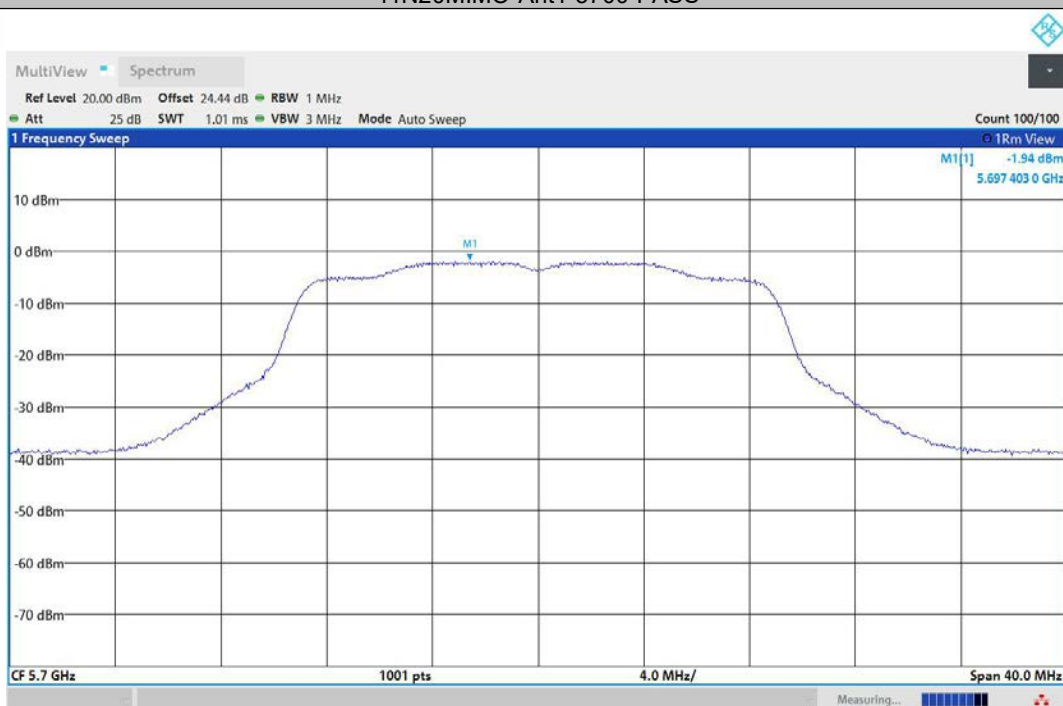
11N20MIMO-Ant2-5700-PASS
