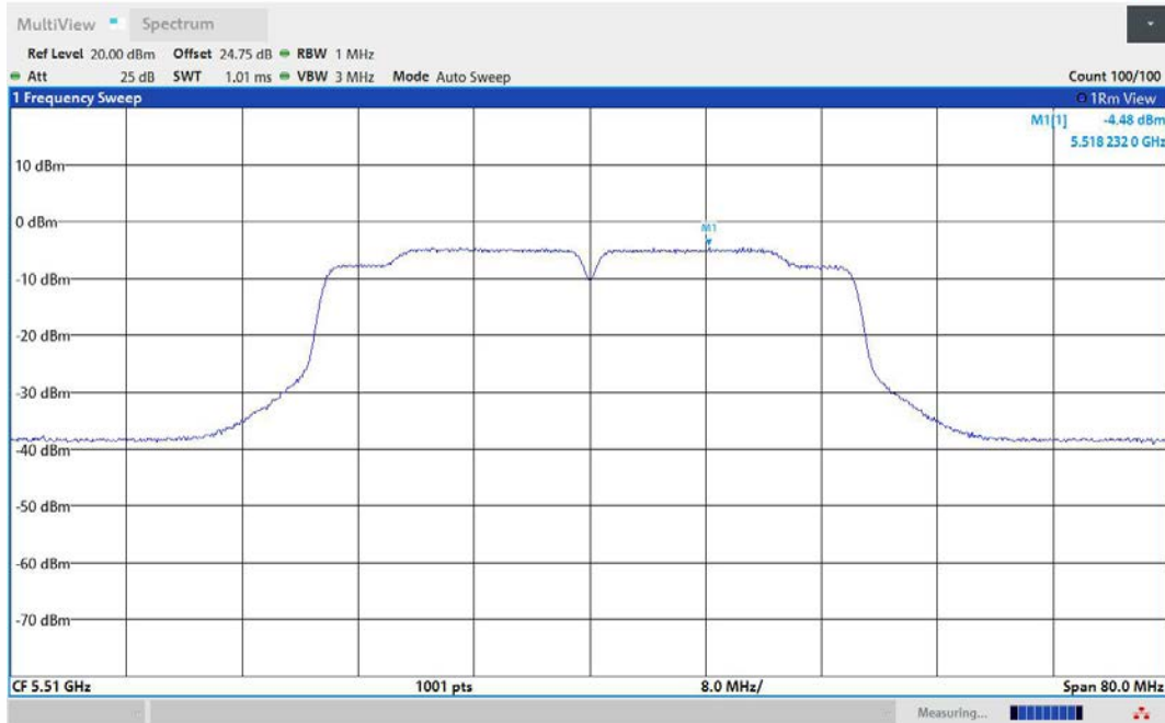
11N40MIMO-Ant2-5510-PASS
