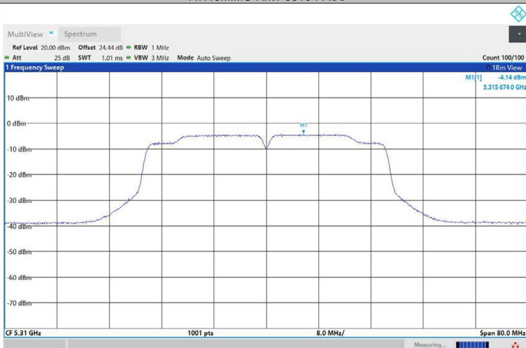
11N40MIMO-Ant2-5310-PASS
