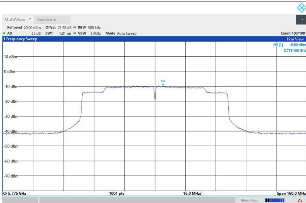
11AC80MIMO-Ant1-5775-PASS
