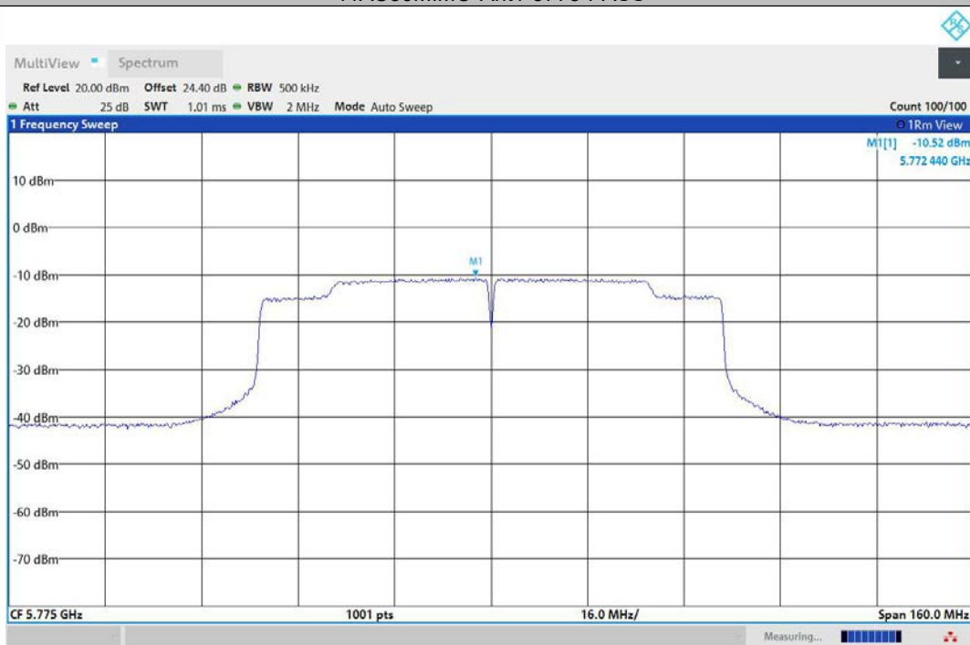
11AC80MIMO-Ant2-5775-PASS
