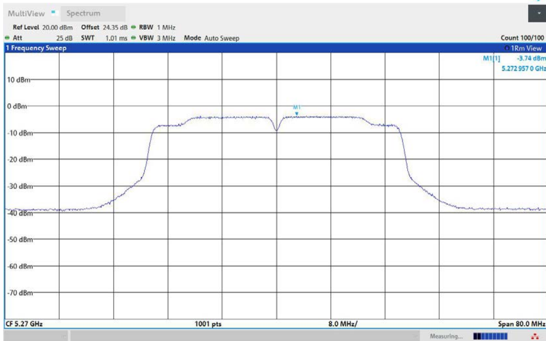
11AC40MIMO-Ant1-5270-PASS
