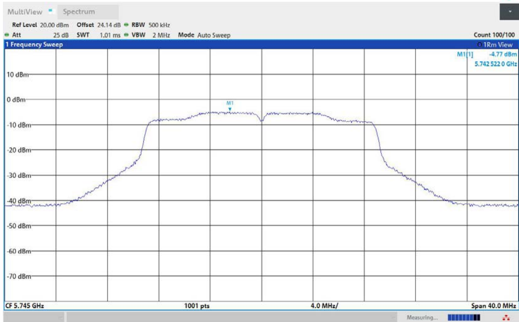
11N20MIMO-Ant2-5745-PASS
