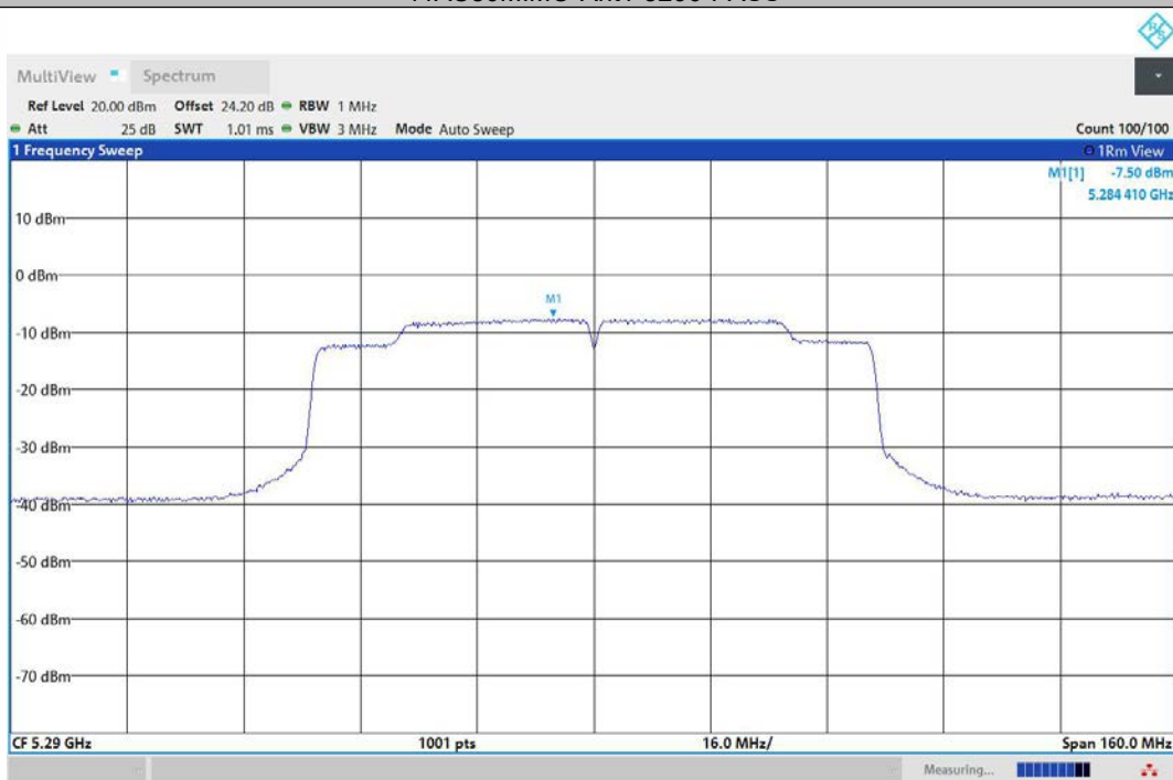
11AC80MIMO-Ant2-5290-PASS
