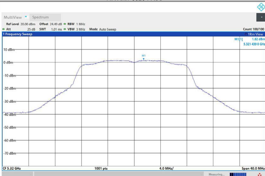
11A-Ant2-5320-PASS
