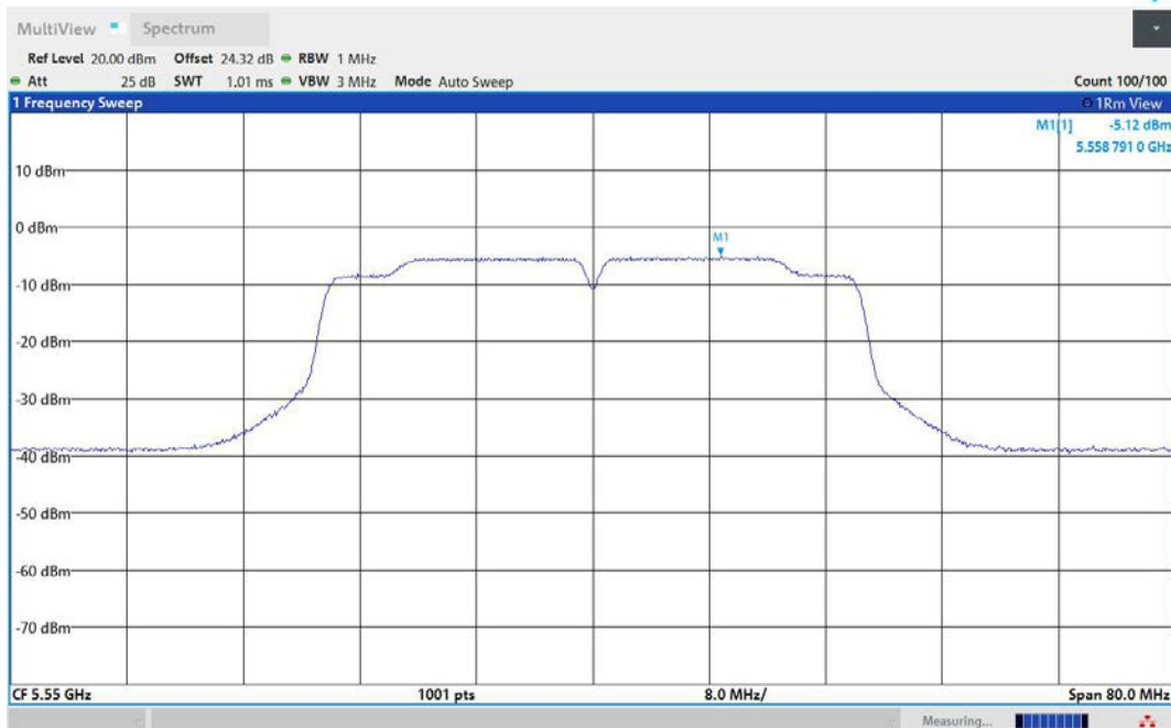
11AC40MIMO-Ant2-5550-PASS
