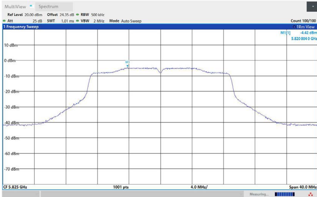
11N20MIMO-Ant2-5825-PASS
