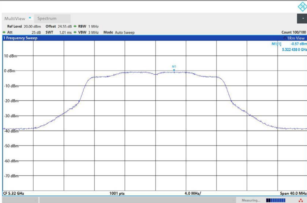
11N20MIMO-Ant1-5320-PASS
