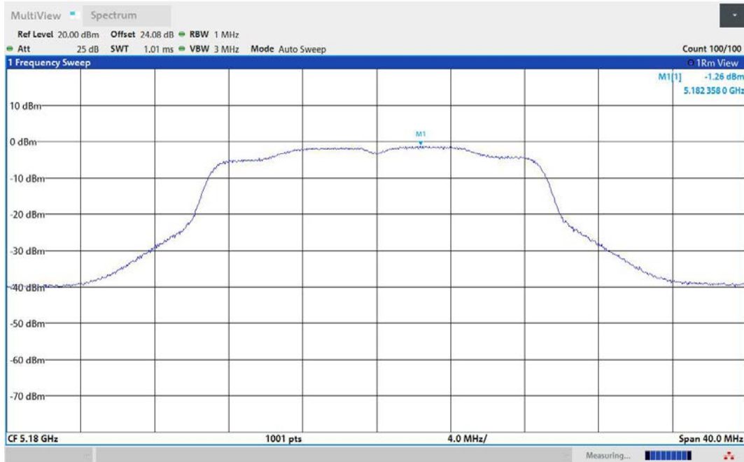
11N20MIMO-Ant2-5180-PASS
