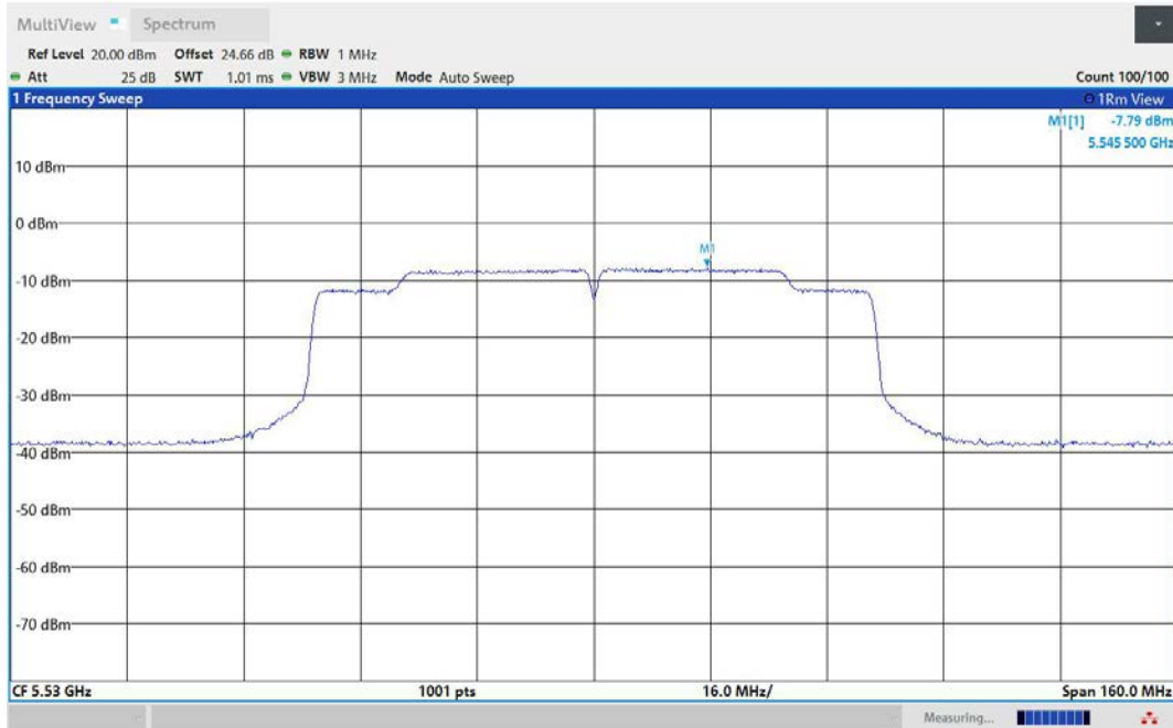
11AC80MIMO-Ant2-5530-PASS
