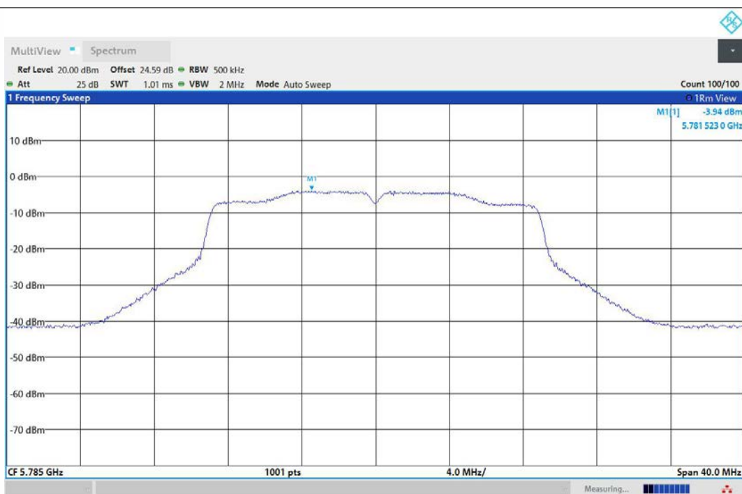
11AC20MIMO-Ant1-5785-PASS
