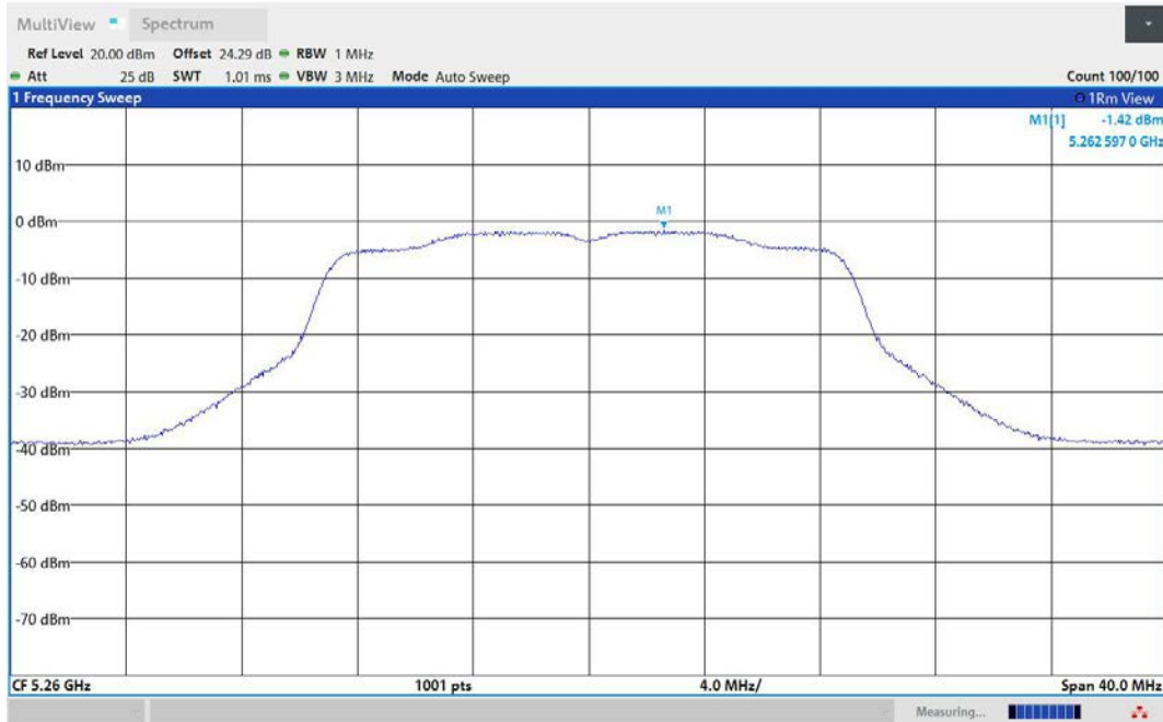
11N20MIMO-Ant2-5260-PASS
