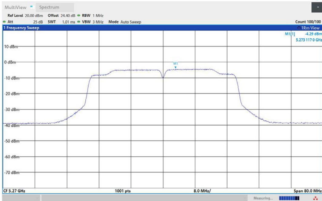
11AC40MIMO-Ant2-5270-PASS
