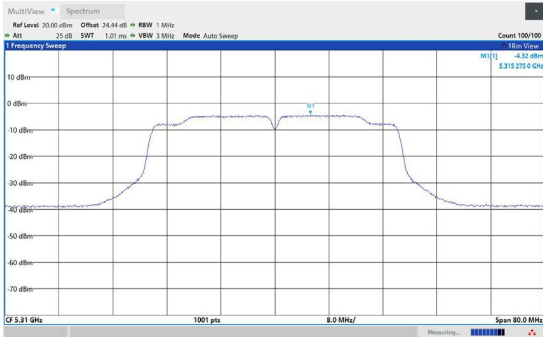
11AC40MIMO-Ant2-5310-PASS
