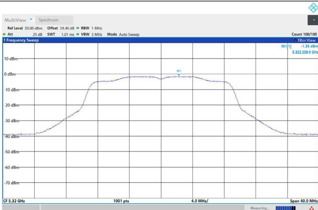
11N20MIMO-Ant2-5320-PASS
