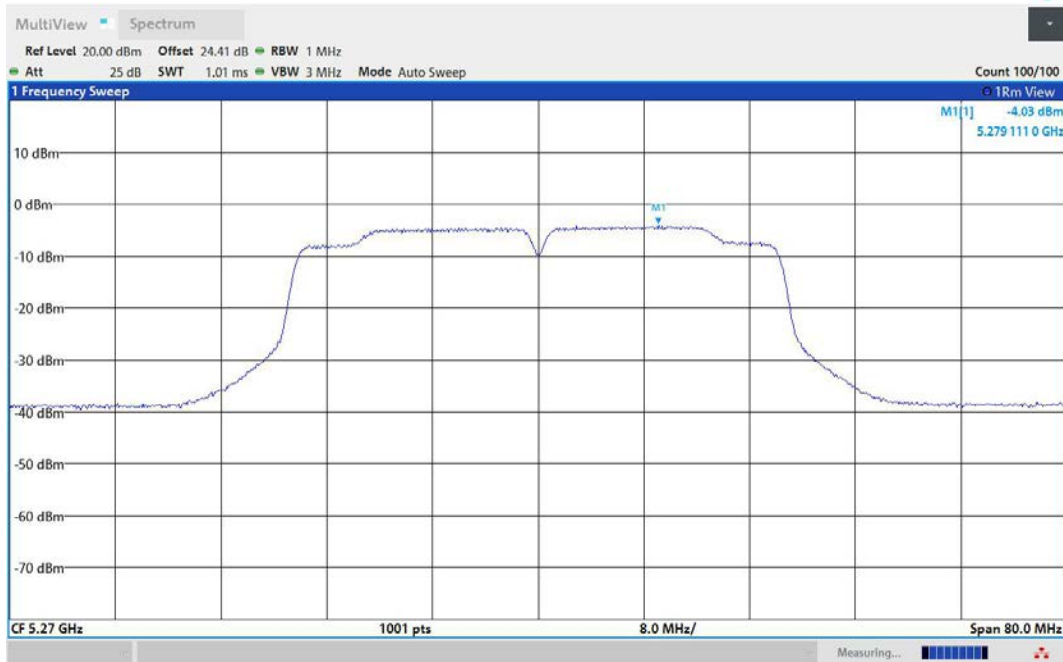
11N40MIMO-Ant2-5270-PASS
