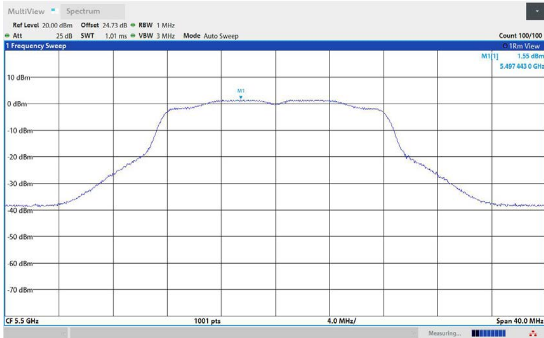
11A-Ant2-5500-PASS
