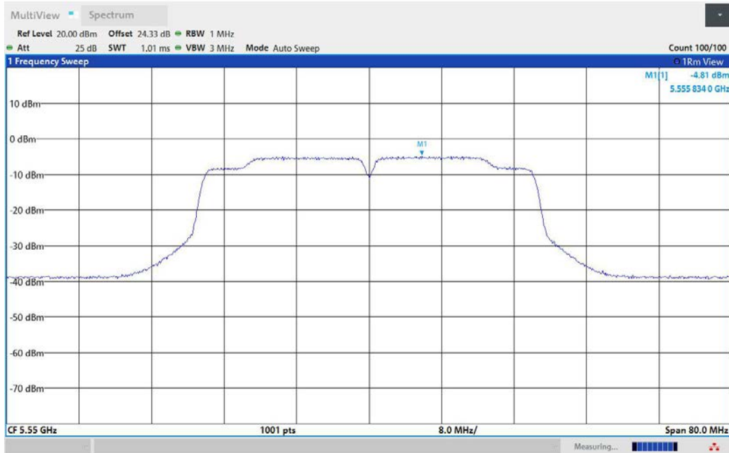
11N40MIMO-Ant2-5550-PASS
