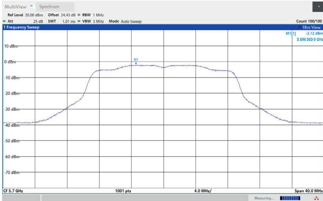
11AC20MIMO-Ant2-5700-PASS
