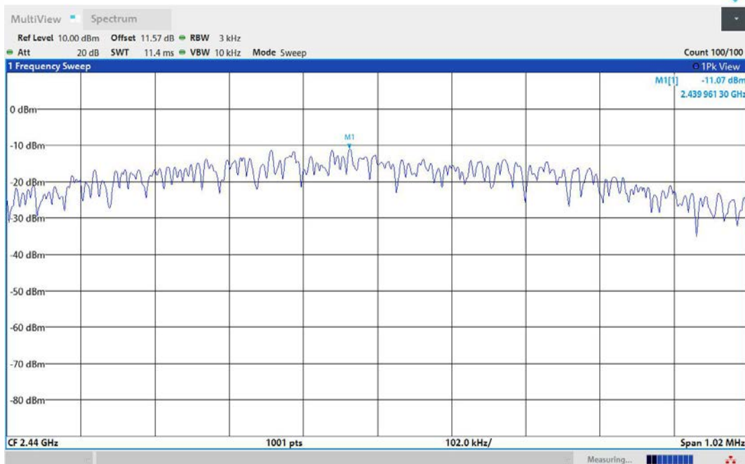
BLE_1M-Ant1-2440-PASS
