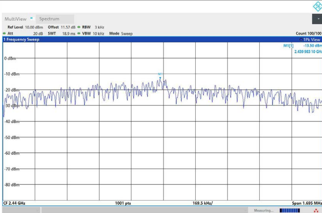
BLE_2M-Ant1-2440-PASS
