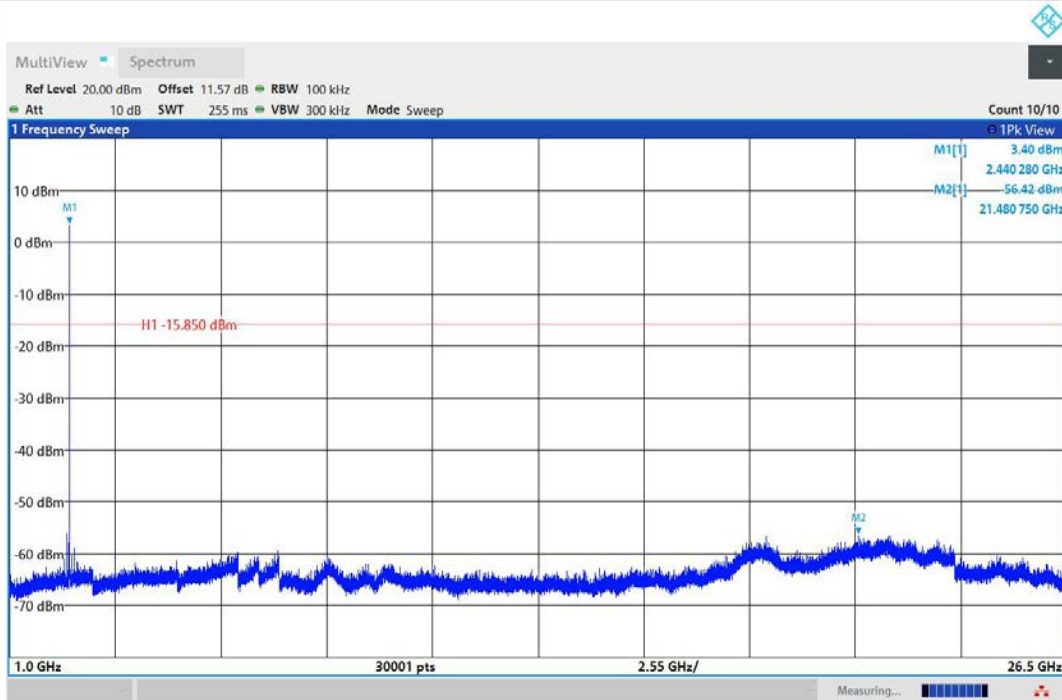
BLE_1M-Ant1-2440-1000~26500-PASS
