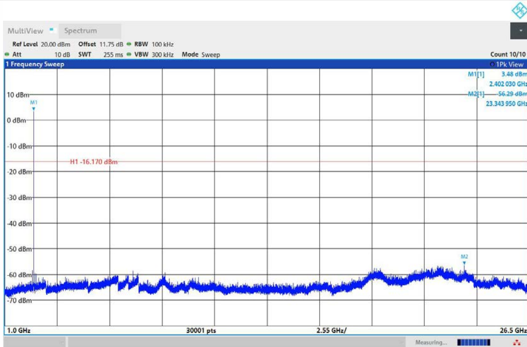
BLE_2M-Ant1-2402-1000~26500-PASS
