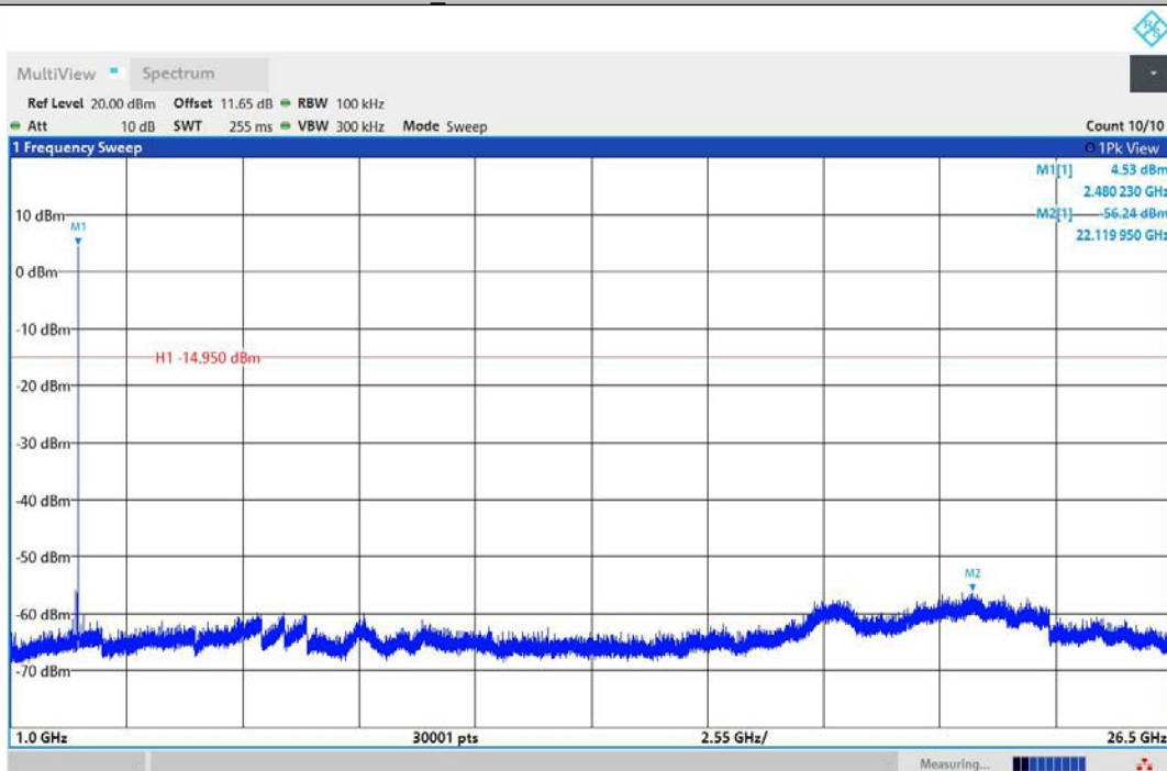
BLE_1M-Ant1-2480-1000~26500-PASS
