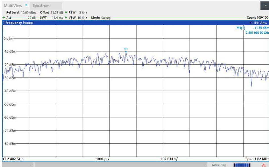
BLE_1M-Ant1-2402-PASS
