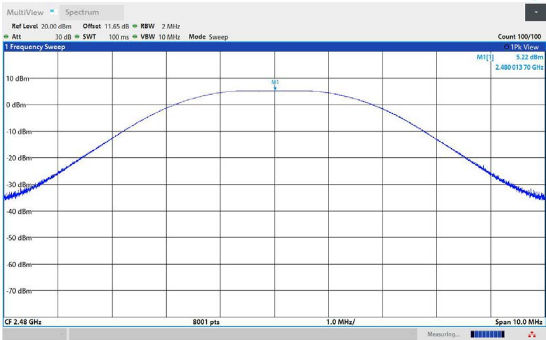
BLE_2M-Ant1-2480-PASS
