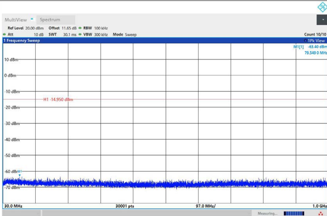
BLE_1M-Ant1-2480-30~1000-PASS
