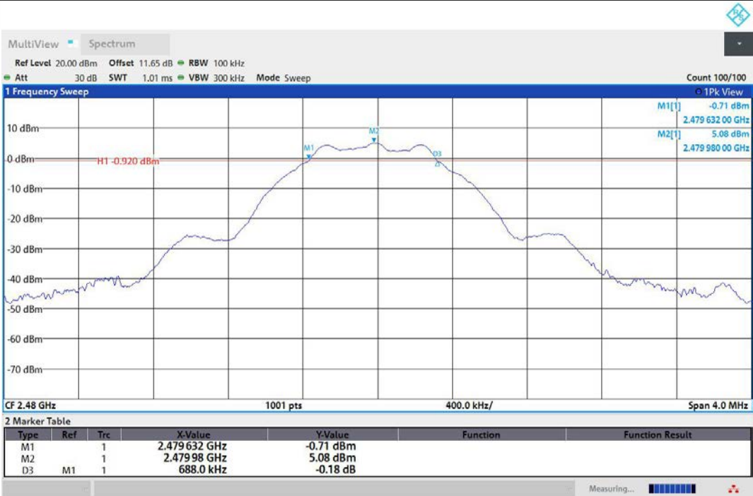
BLE_1M-Ant1-2480-PASS
