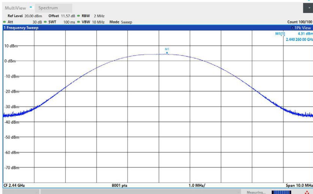
BLE_1M-Ant1-2440-PASS
