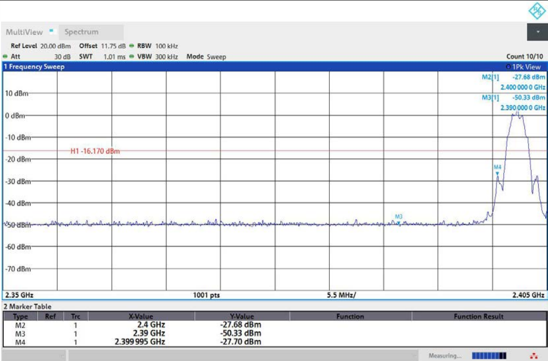
BLE_2M-Ant1-2402-PASS
