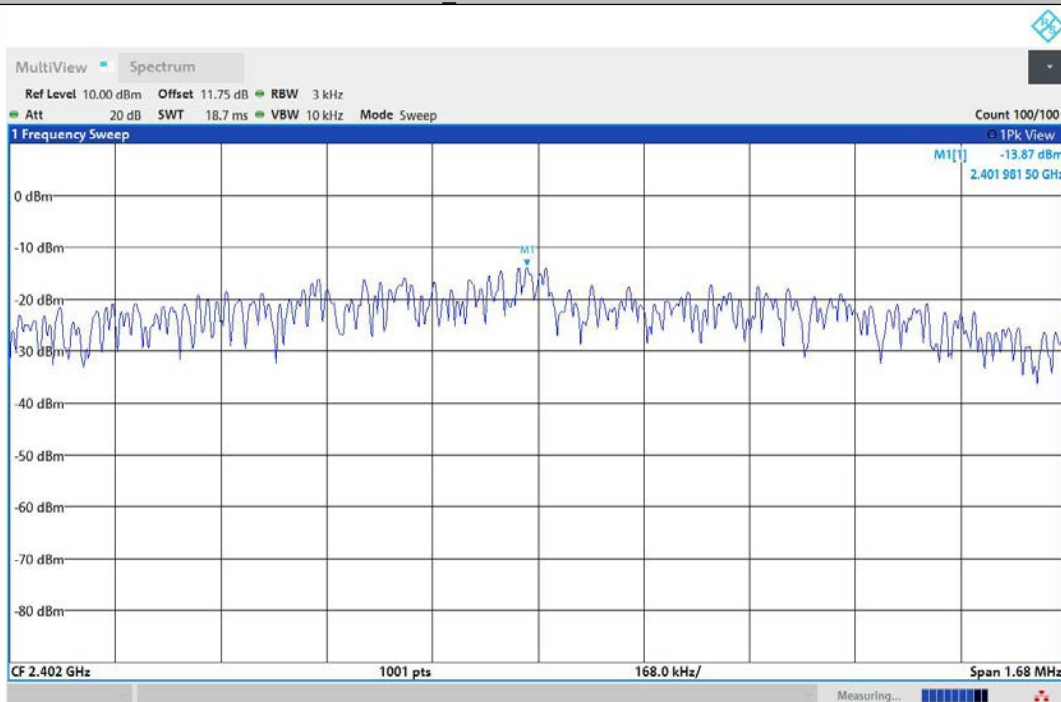
BLE_2M-Ant1-2402-PASS
