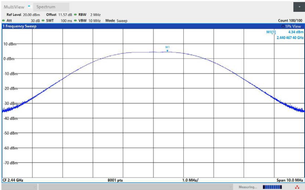
BLE_2M-Ant1-2440-PASS
