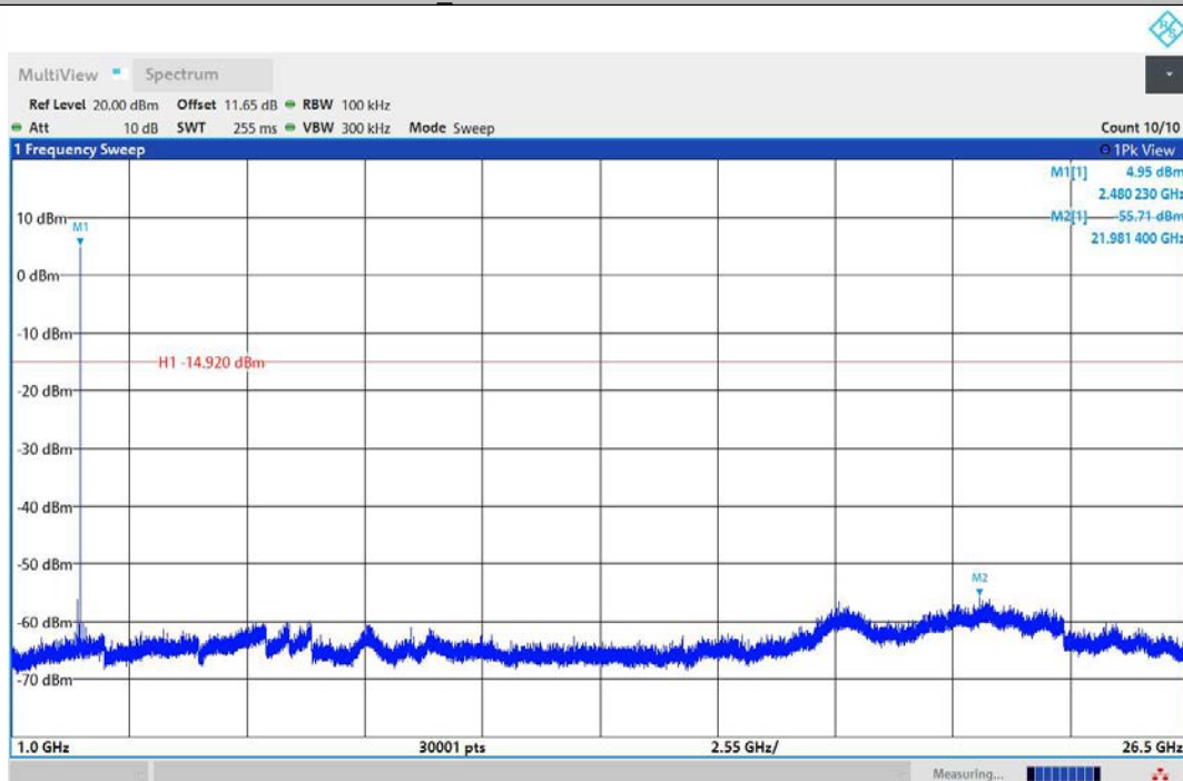
BLE_2M-Ant1-2480-1000~26500-PASS
