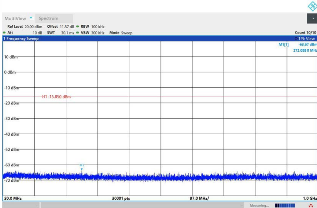
BLE_1M-Ant1-2440-30~1000-PASS
