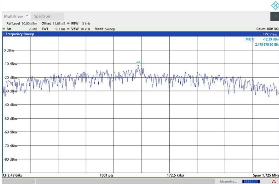
BLE_2M-Ant1-2480-PASS
