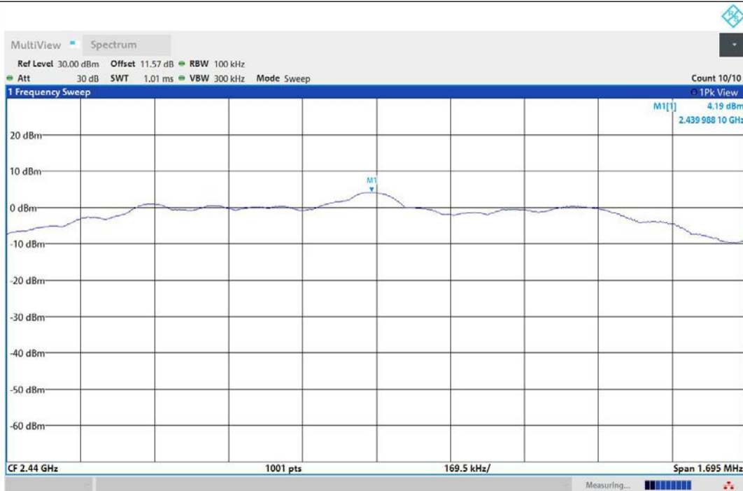
BLE_2M-Ant1-2440-PASS
