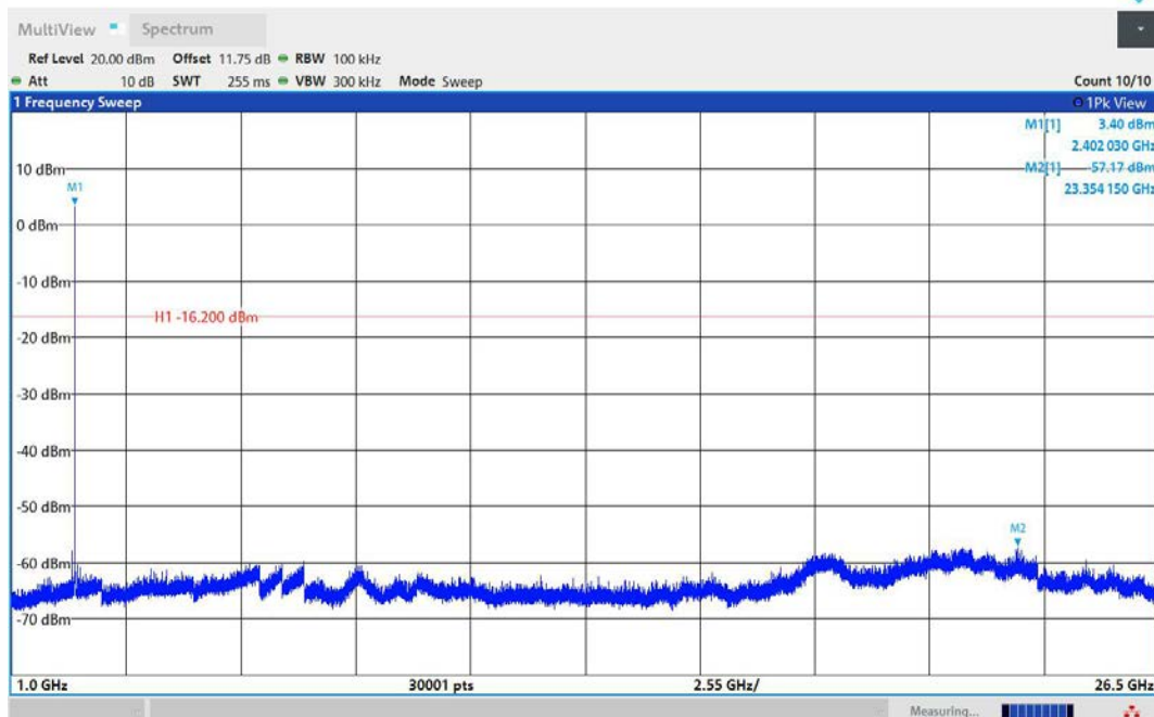
BLE_1M-Ant1-2402-1000~26500-PASS
