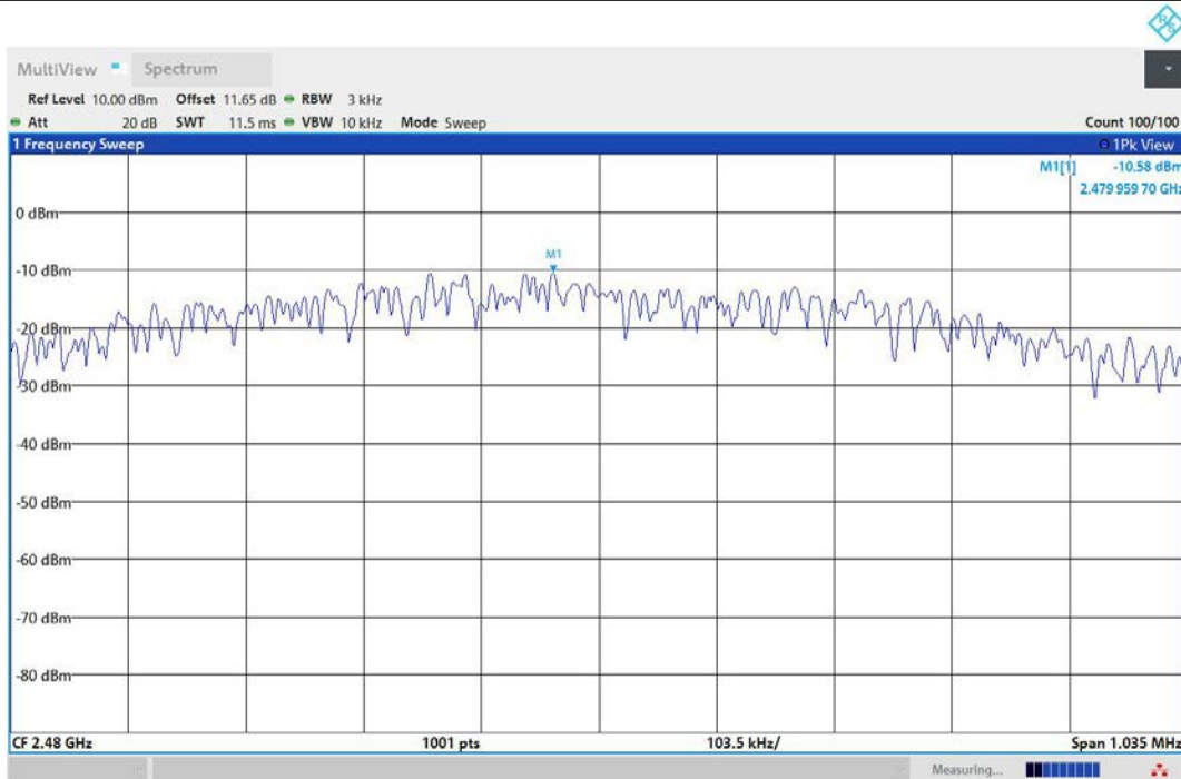
BLE_1M-Ant1-2480-PASS
