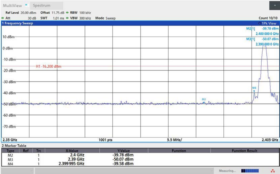
BLE_1M-Ant1-2402-PASS
