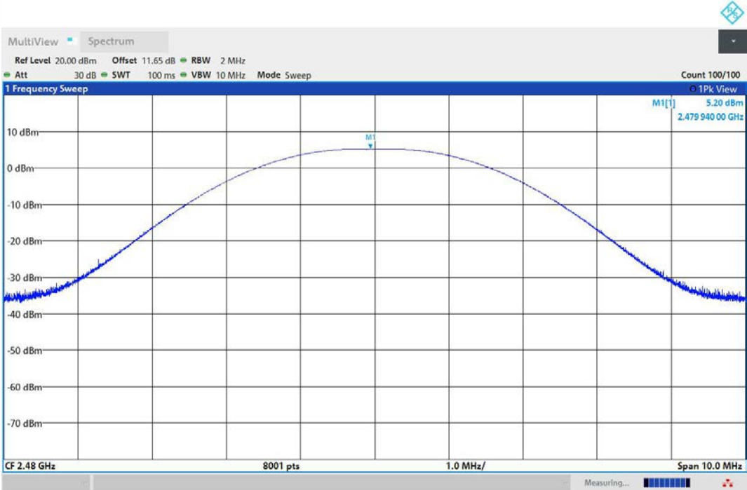
BLE_1M-Ant1-2480-PASS
