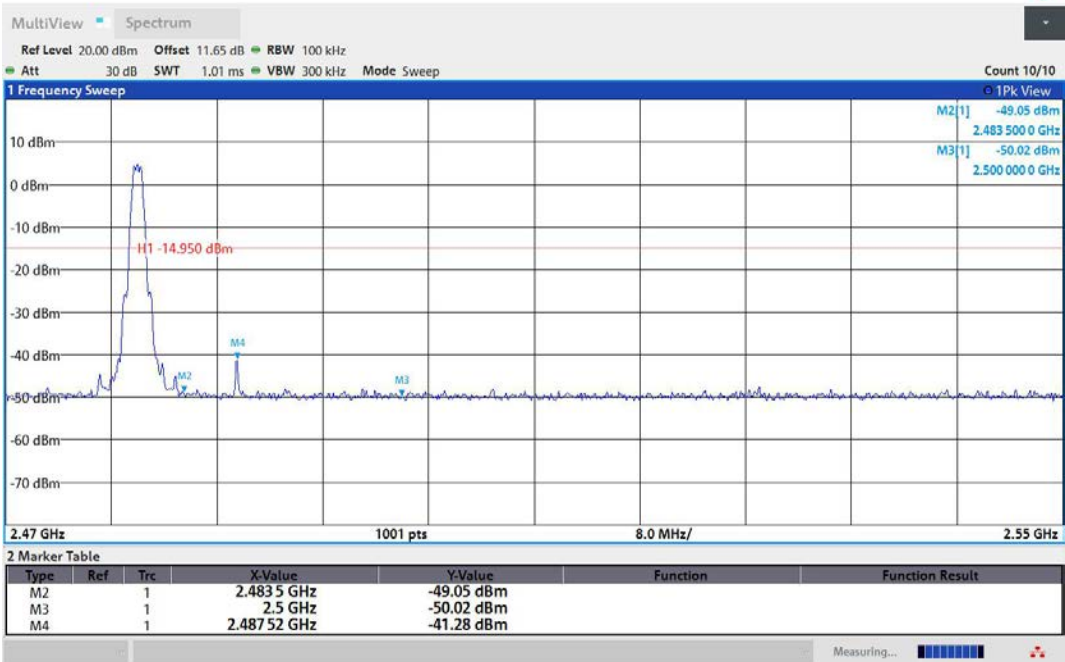
BLE_1M-Ant1-2480-PASS
