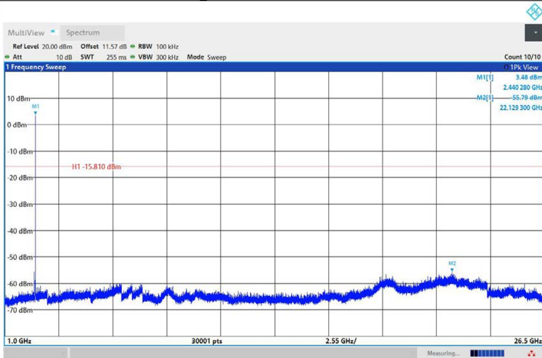
BLE_2M-Ant1-2440-1000~26500-PASS
