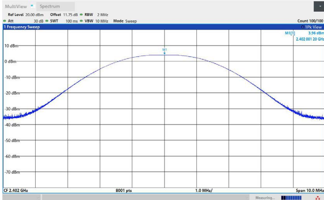
BLE_1M-Ant1-2402-PASS
