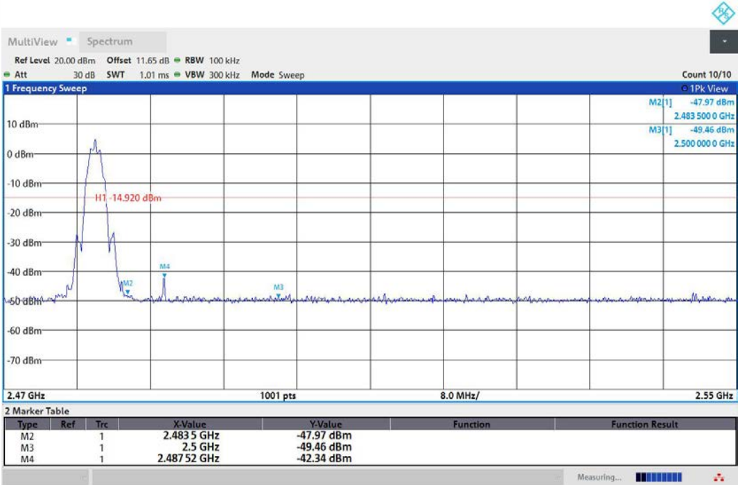
BLE_2M-Ant1-2480-PASS
