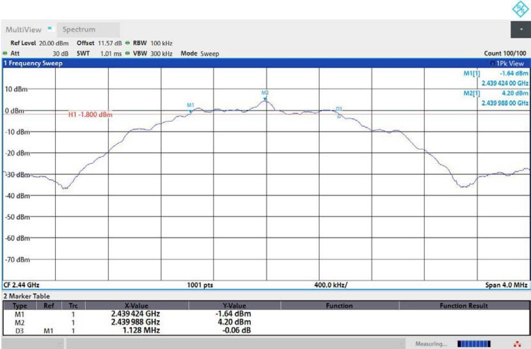
BLE_2M-Ant1-2440-PASS
