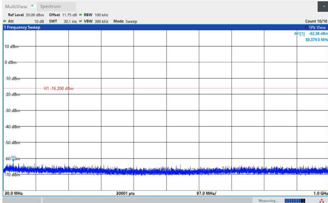
BLE_1M-Ant1-2402-30~1000-PASS
