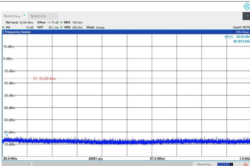
3DH5-Ant1-2402-30~1000-PASS
