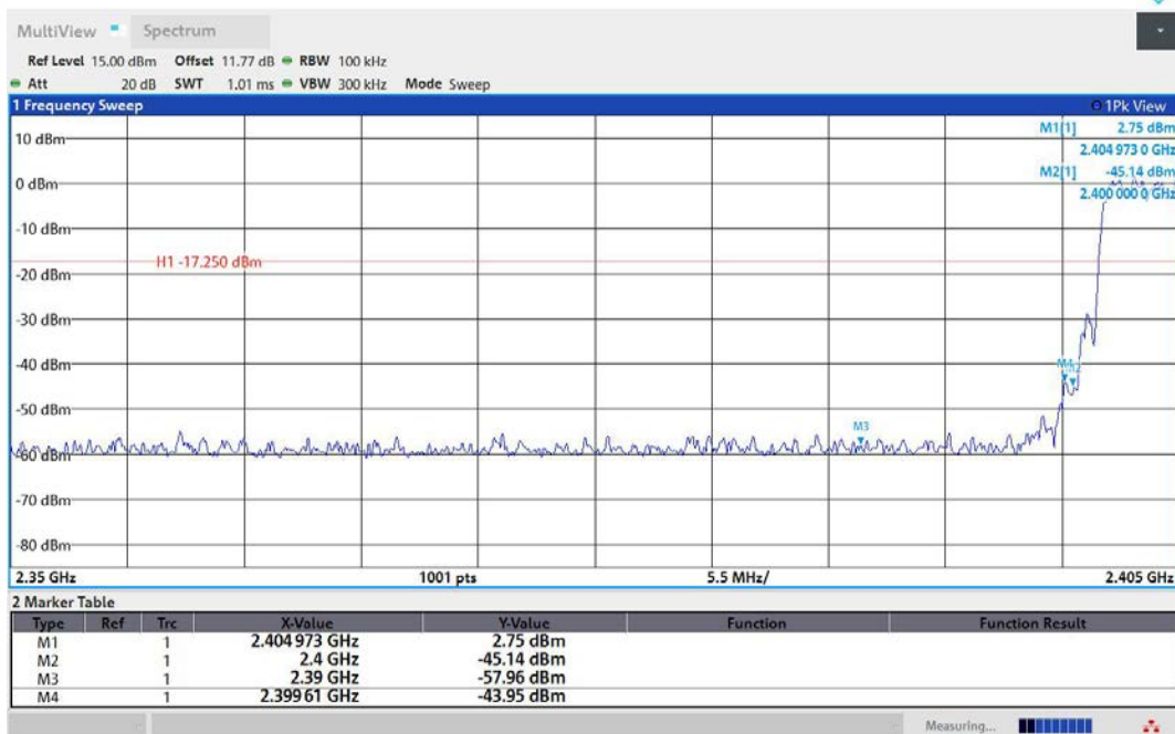
2DH5-Ant1-Hop_2402-PASS
