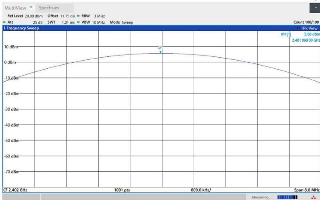
3DH5-Ant1-2402-PASS
