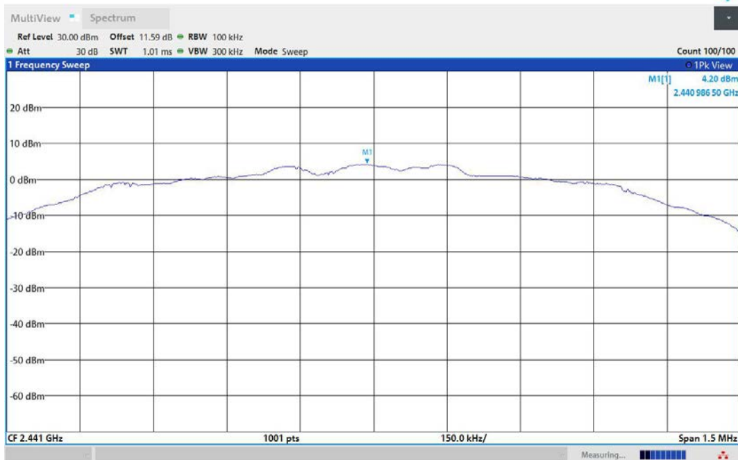
2DH5-Ant1-2441-PASS
