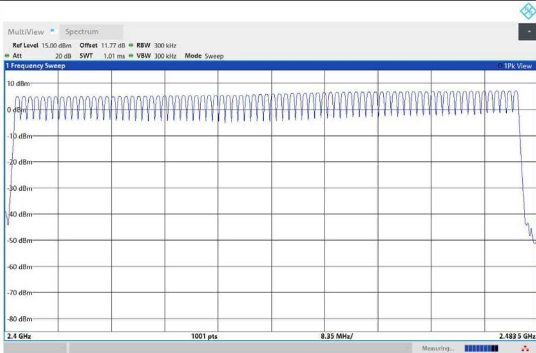
DH5-Ant1-Hop-PASS
