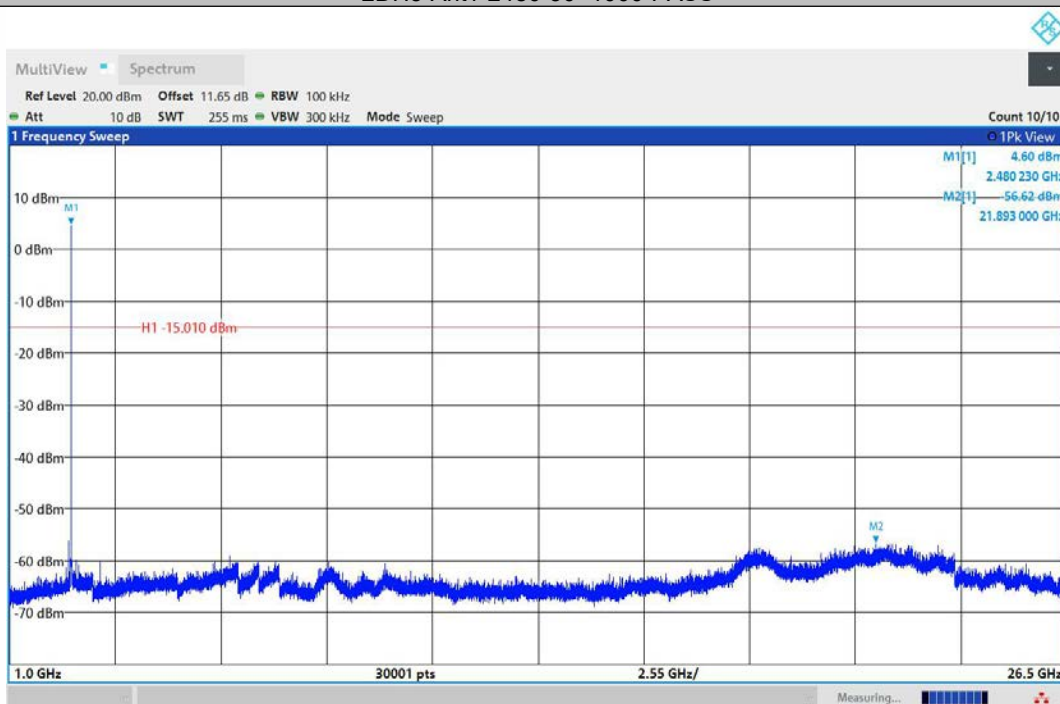
2DH5-Ant1-2480-1000~26500-PASS
