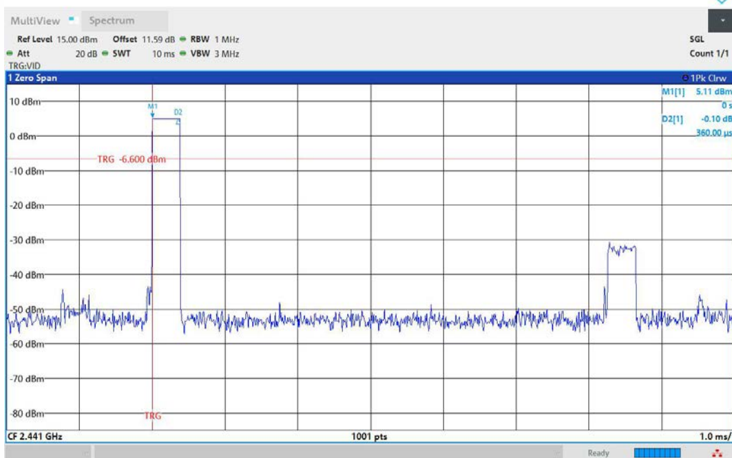
DH1-Ant1-Hop-PASS
