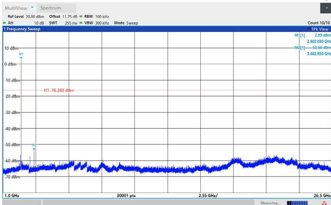
2DH5-Ant1-2402-1000~26500-PASS
