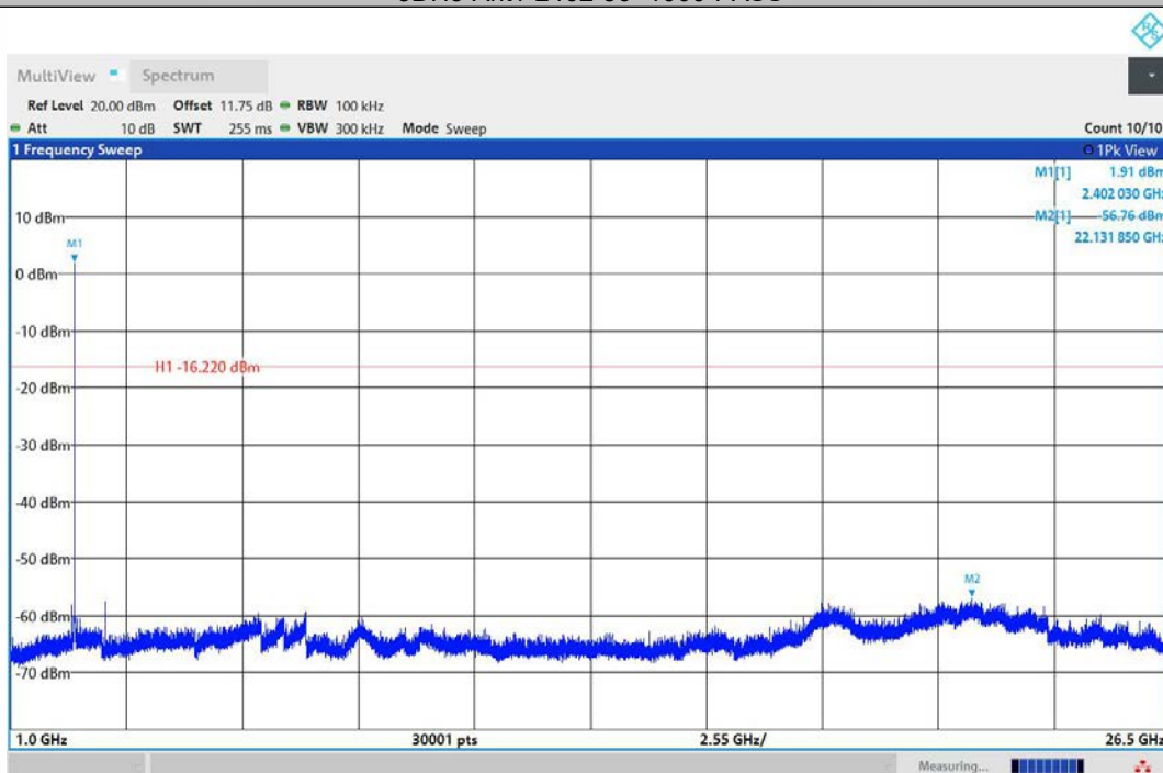
3DH5-Ant1-2402-1000~26500-PASS
