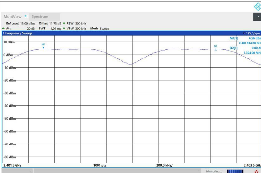
DH5-Ant1-Hop_2402-PASS
