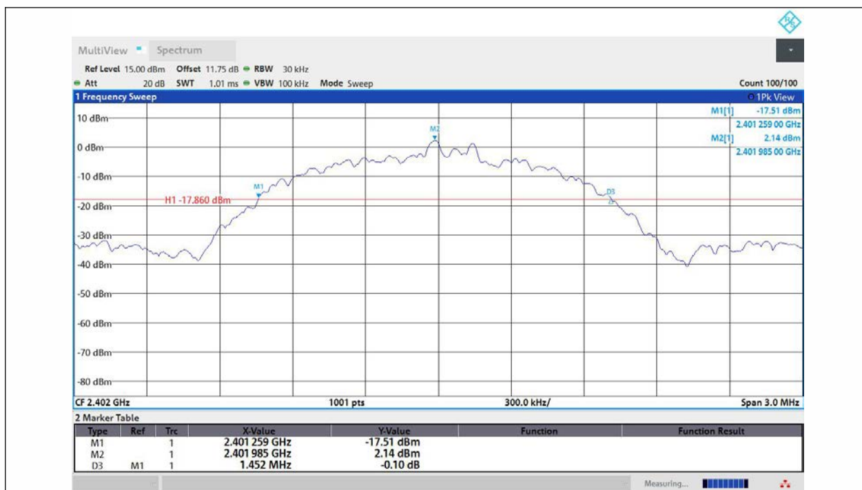
3DH5-Ant1-2402
