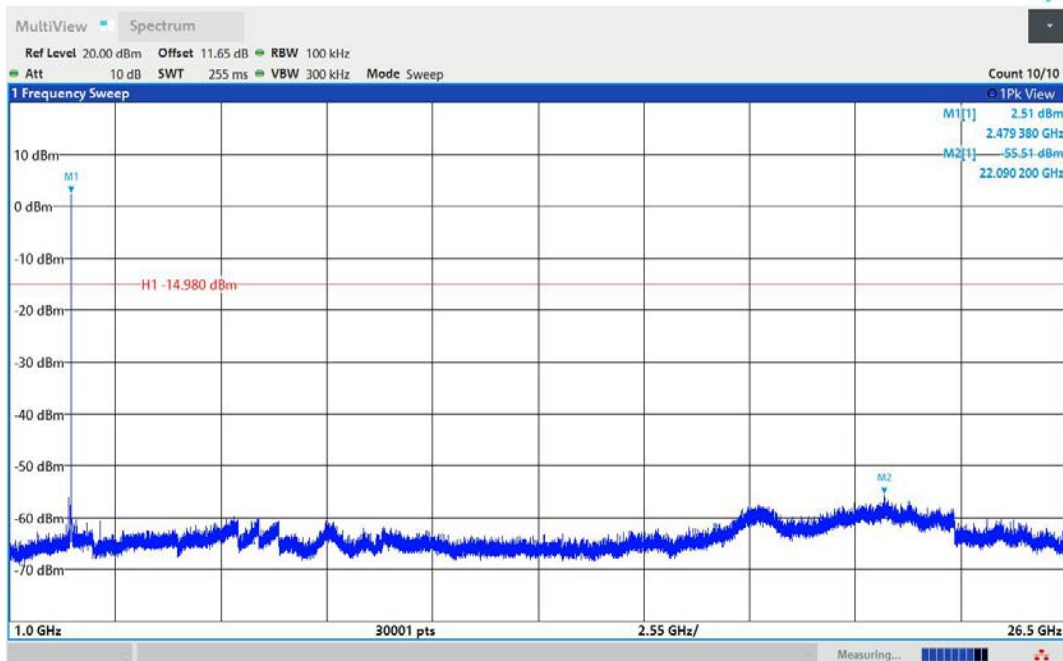
3DH5-Ant1-2480-1000~26500-PASS
