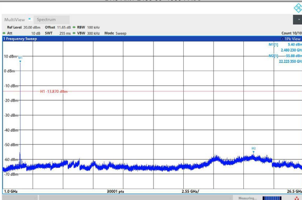
DH5-Ant1-2480-1000~26500-PASS
