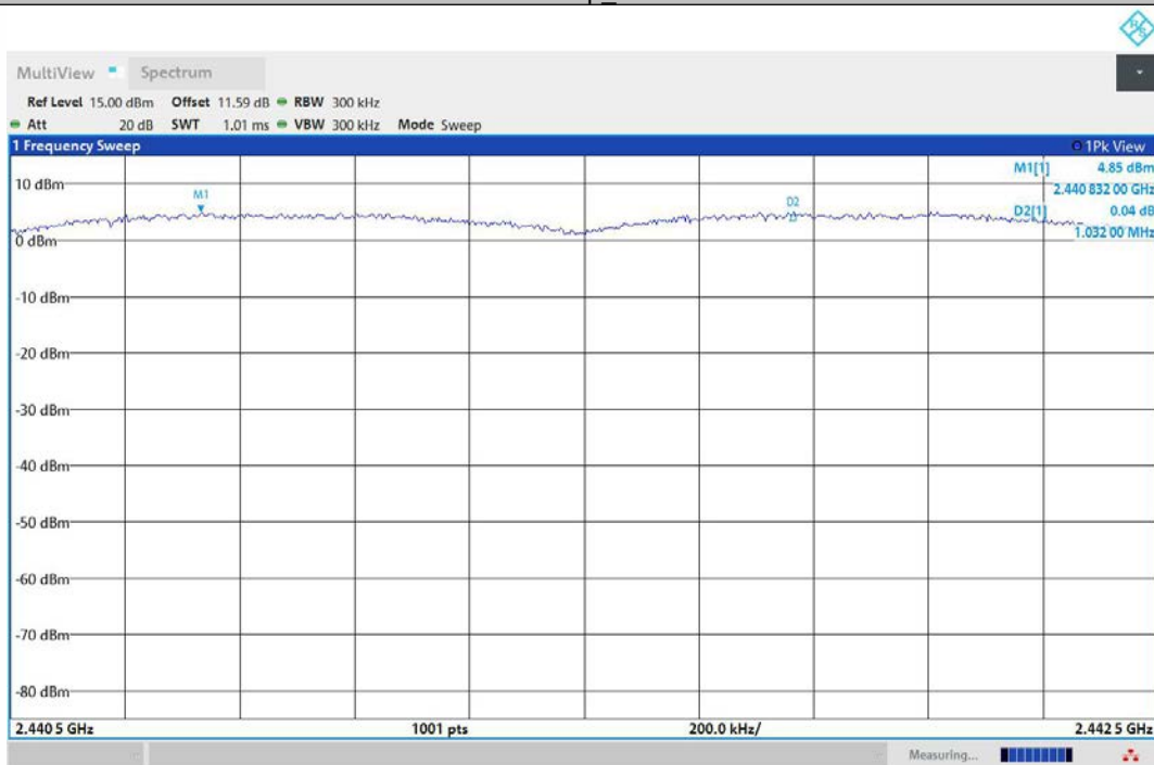
3DH5-Ant1-Hop_2441-PASS
