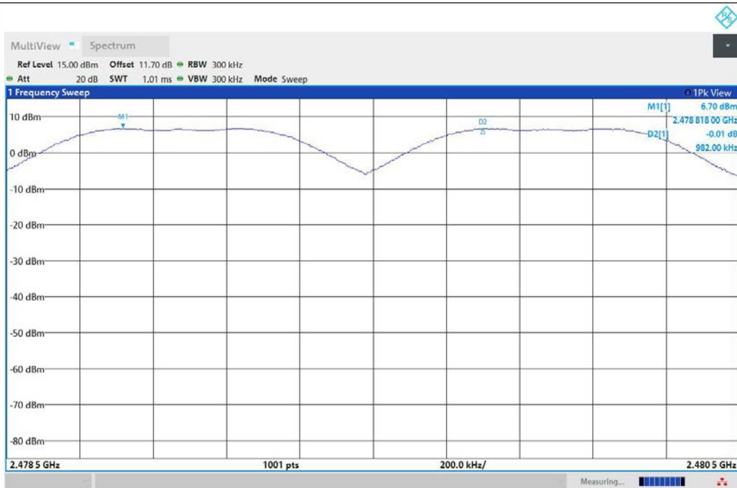
DH5-Ant1-Hop_2480-PASS
