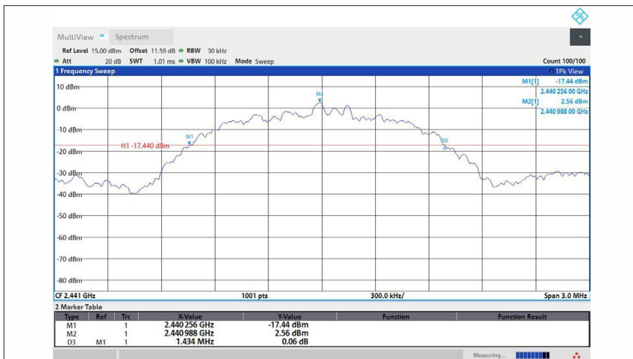
2DH5-Ant1-2441
