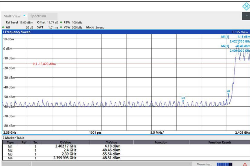
DH5-Ant1-Hop_2402-PASS
