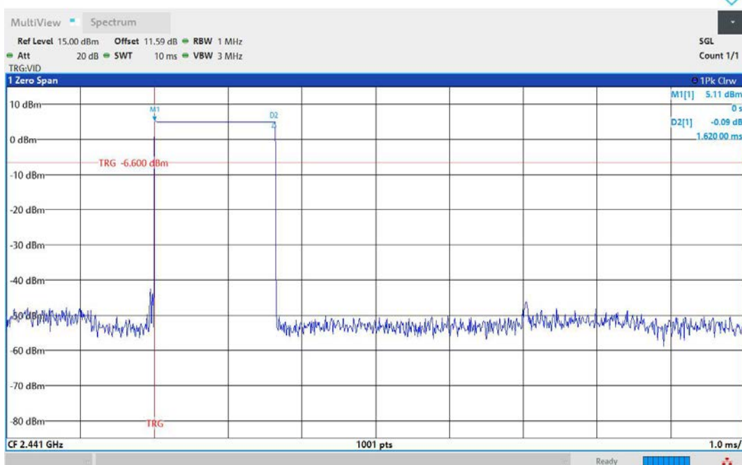
DH3-Ant1-Hop-PASS
