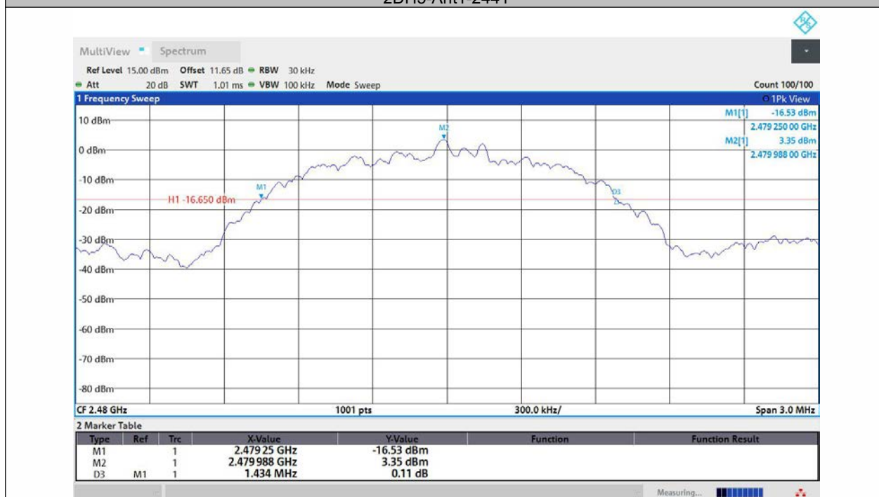
2DH5-Ant1-2480
