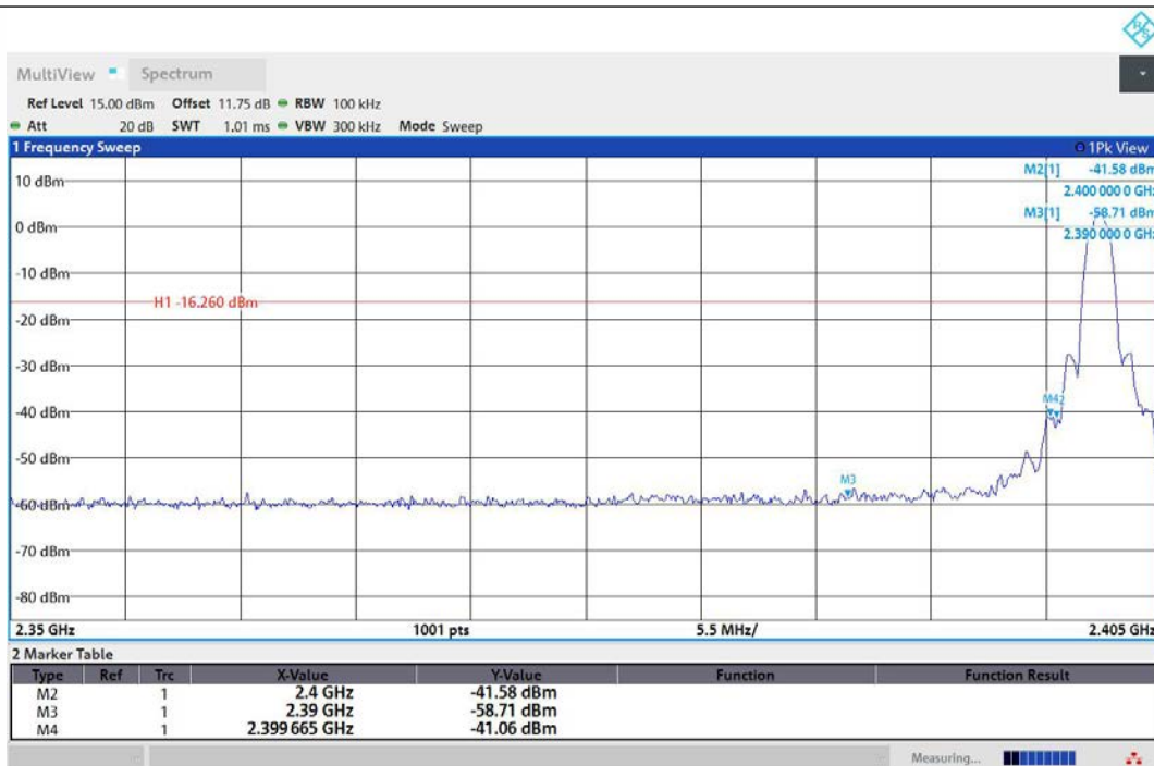
2DH5-Ant1-2402-PASS
