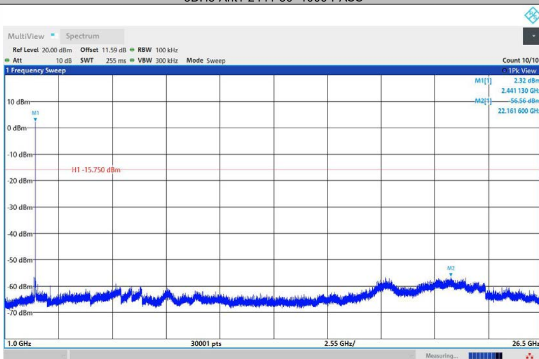
3DH5-Ant1-2441-1000~26500-PASS
