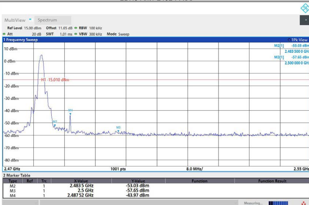
2DH5-Ant1-2480-PASS
