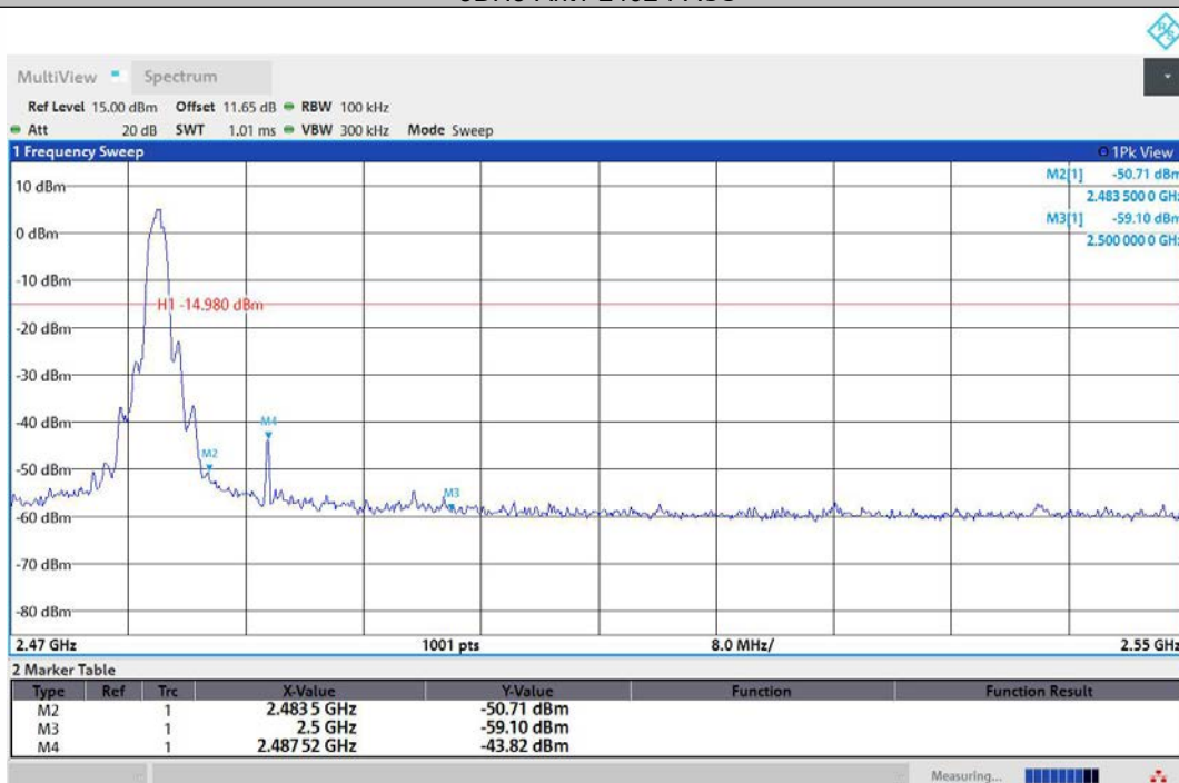
3DH5-Ant1-2480-PASS
