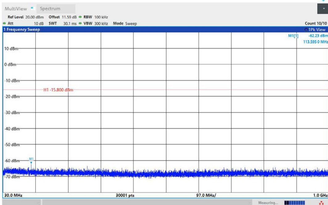
2DH5-Ant1-2441-30~1000-PASS
