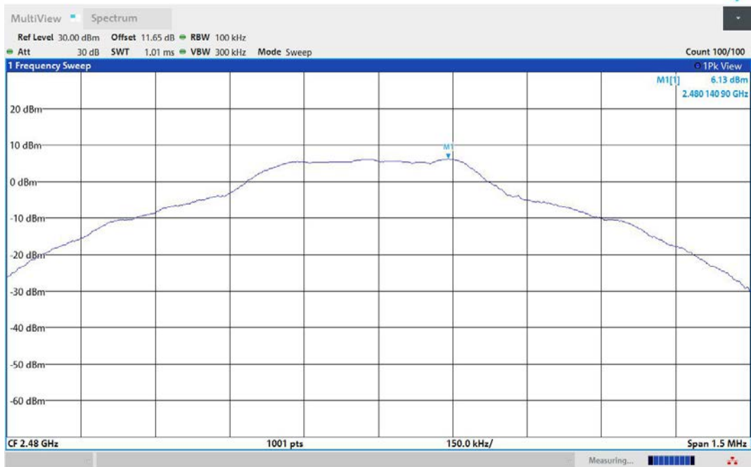
DH5-Ant1-2480-PASS
