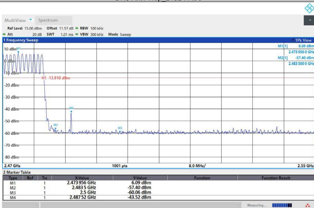
DH5-Ant1-Hop_2480-PASS
