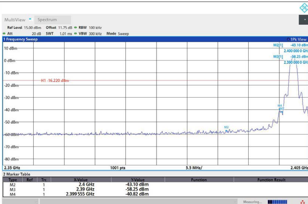
3DH5-Ant1-2402-PASS
