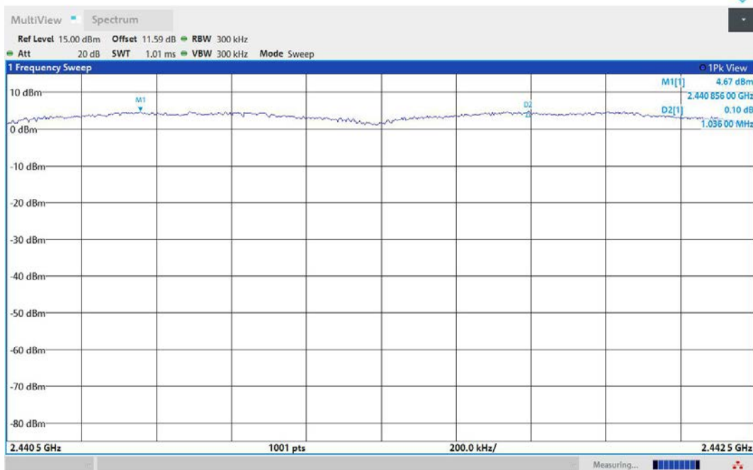
2DH5-Ant1-Hop_2441-PASS
