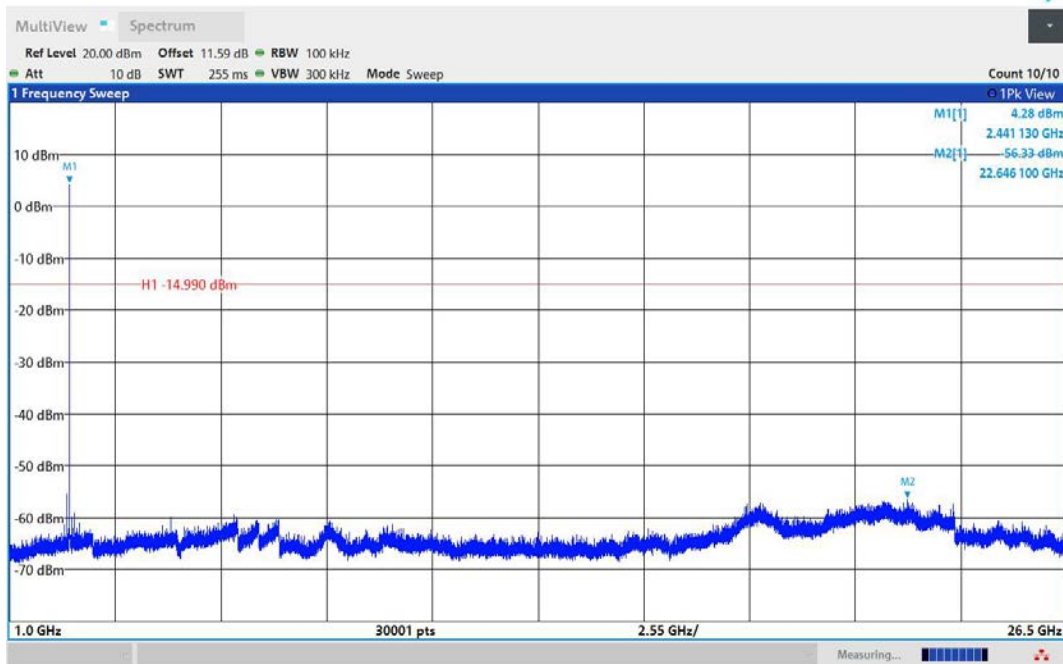
DH5-Ant1-2441-1000~26500-PASS
