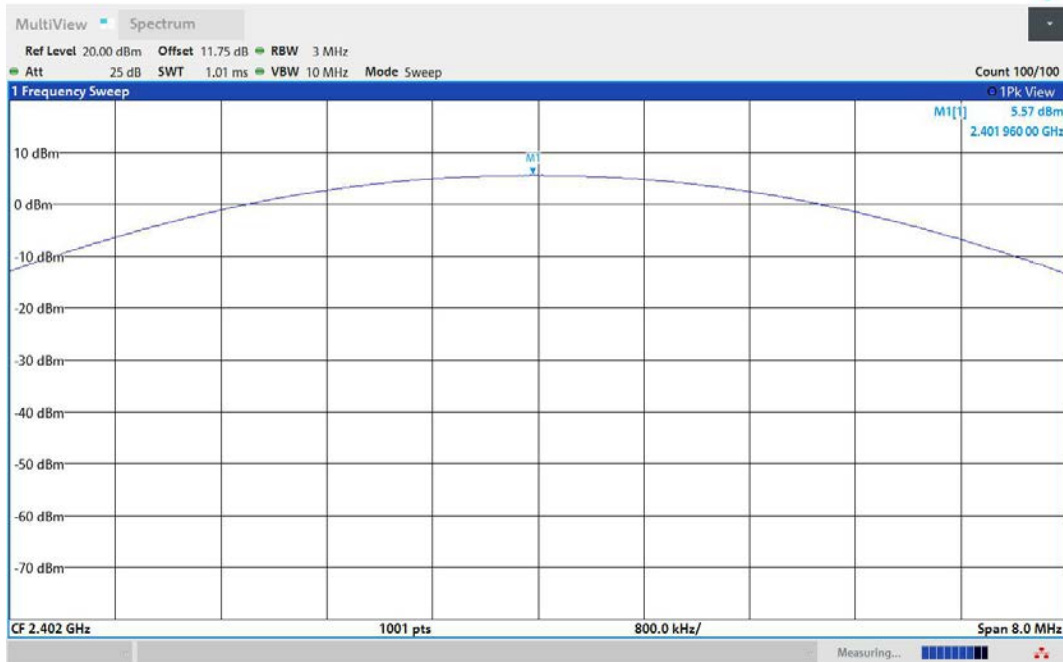
2DH5-Ant1-2402-PASS
