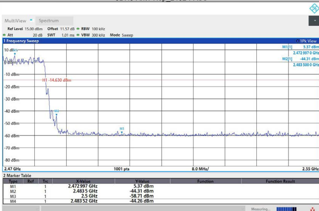
3DH5-Ant1-Hop_2480-PASS
