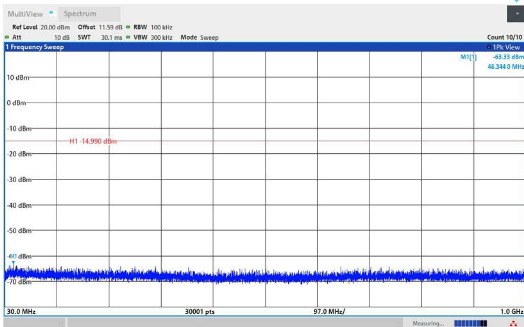
DH5-Ant1-2441-30~1000-PASS
