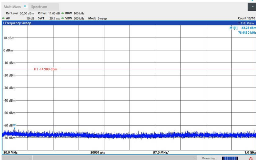
3DH5-Ant1-2480-30~1000-PASS
