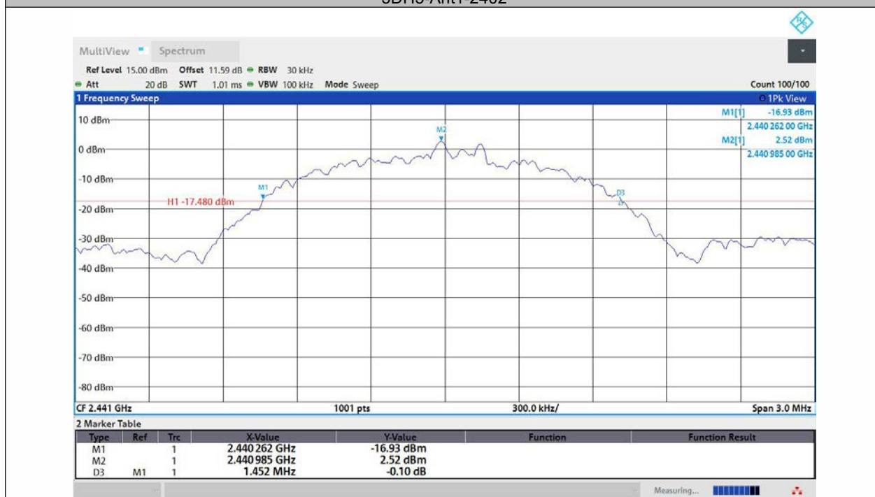
3DH5-Ant1-2441
