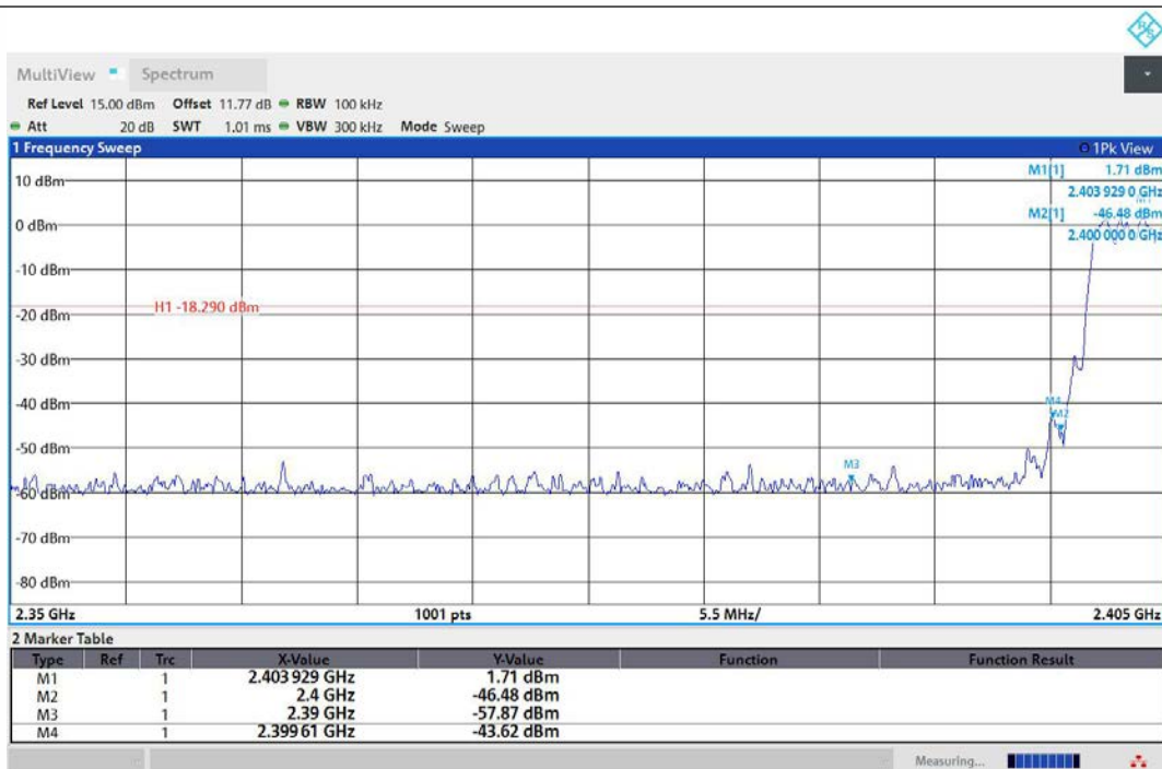
3DH5-Ant1-Hop_2402-PASS
