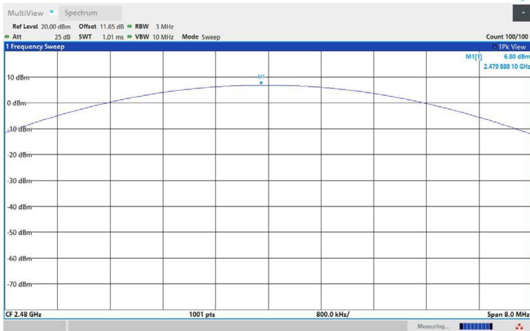
2DH5-Ant1-2480-PASS
