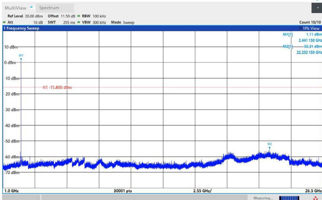
2DH5-Ant1-2441-1000~26500-PASS
