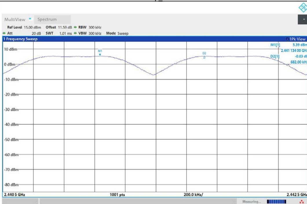
DH5-Ant1-Hop_2441-PASS
