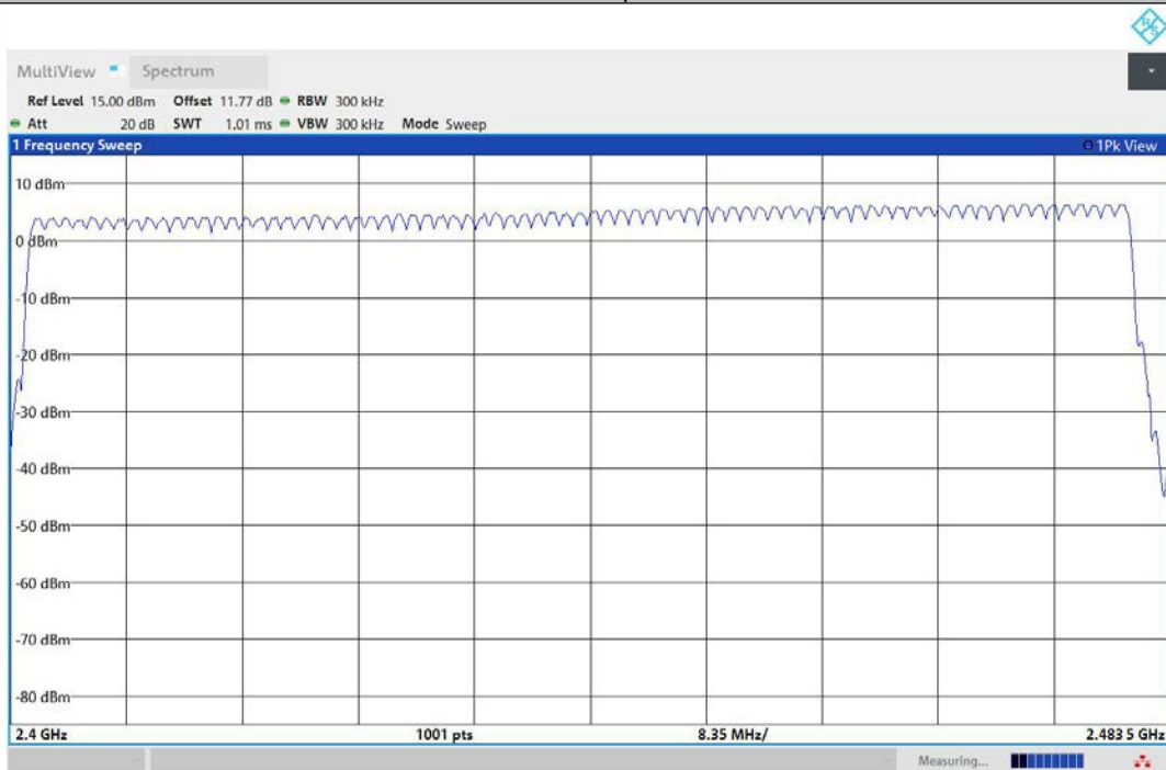
2DH5-Ant1-Hop-PASS
