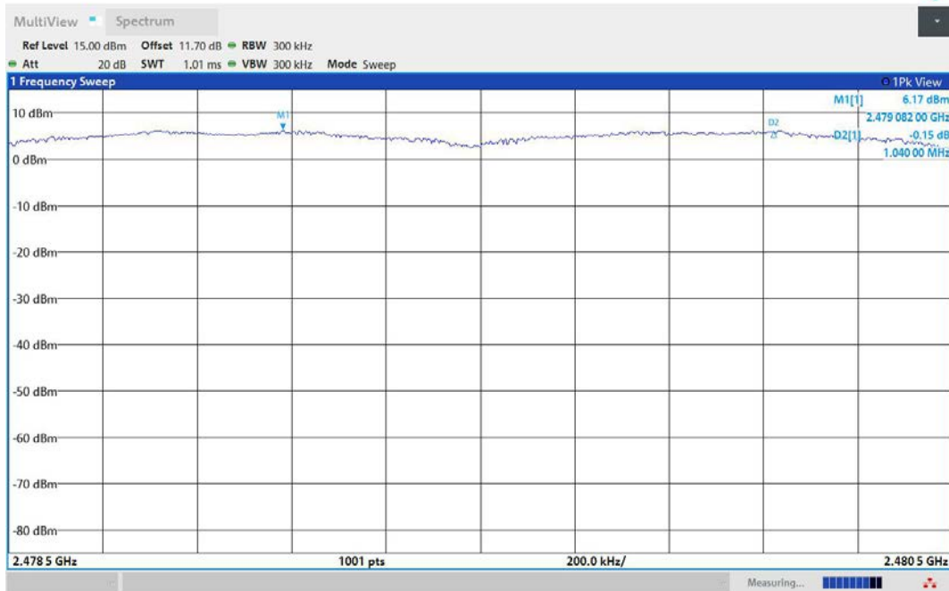
2DH5-Ant1-Hop_2480-PASS
