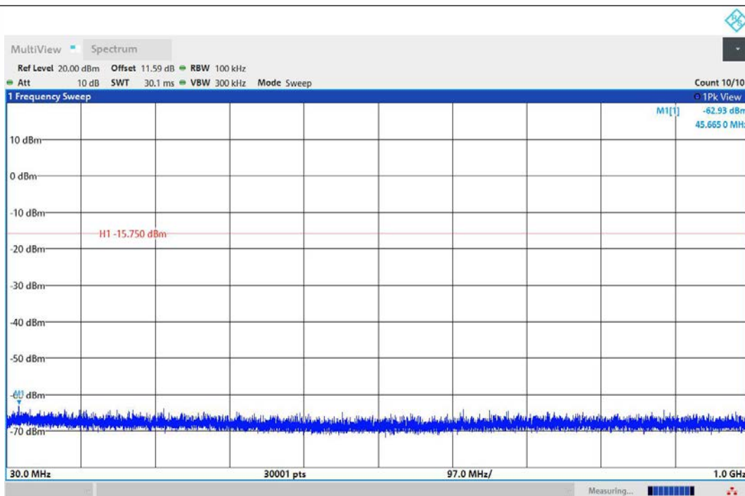
3DH5-Ant1-2441-30~1000-PASS
