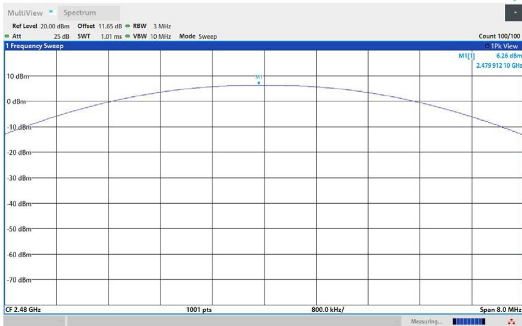
DH5-Ant1-2480-PASS
