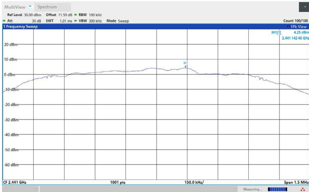
3DH5-Ant1-2441-PASS
