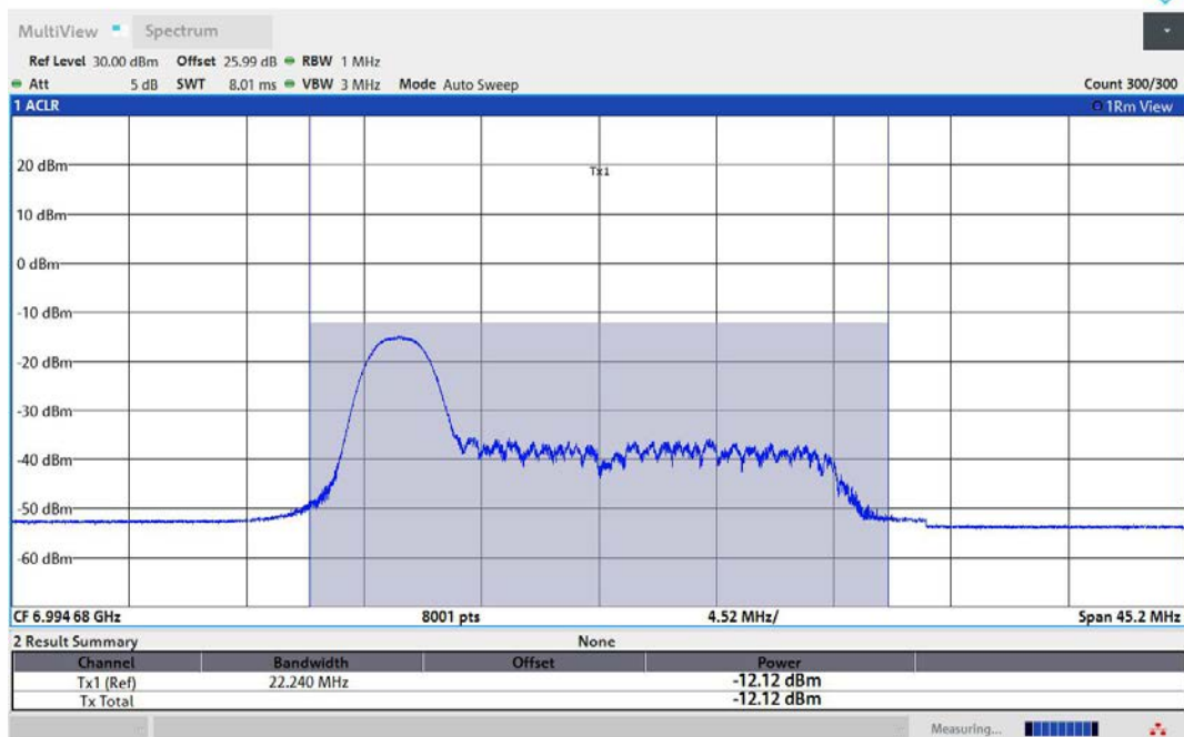
11AX80MIMO-Ant1-7025-26Tone-RU0-PASS
