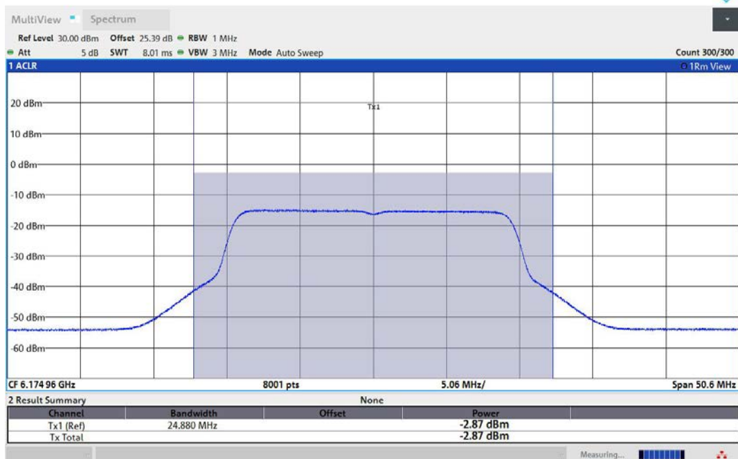
11AX20MIMO-Ant2-6175-PASS
