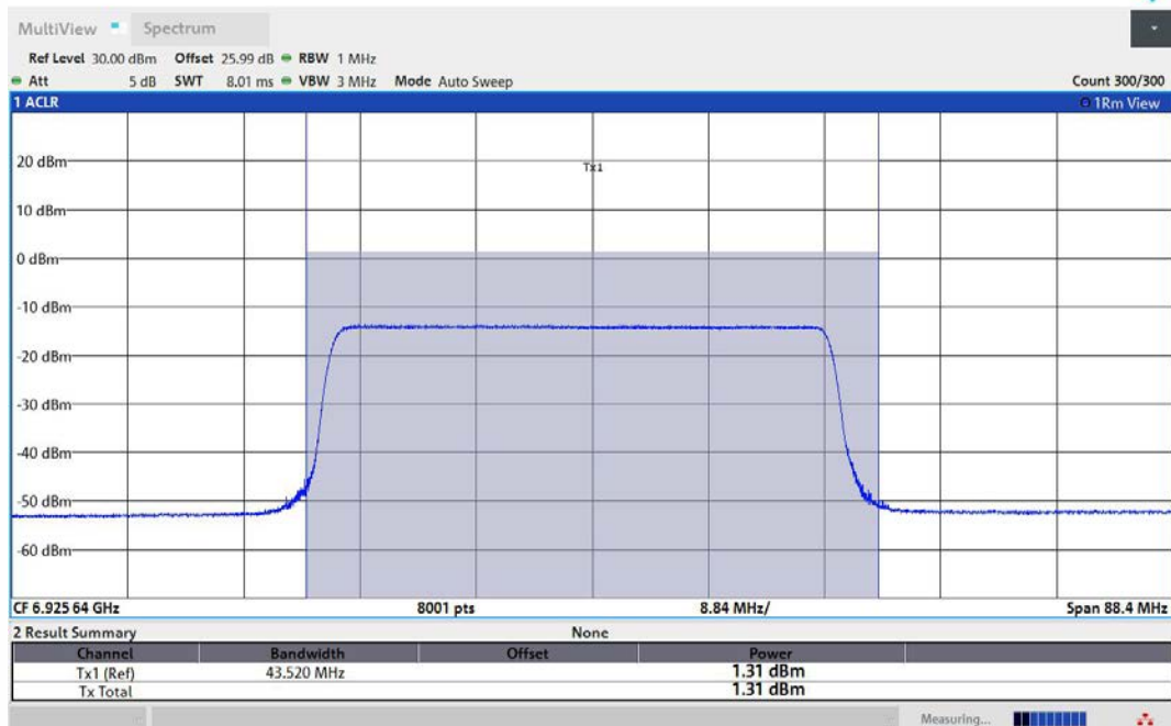
11AX80MIMO-Ant2-6945-484Tone-RU65-PASS
