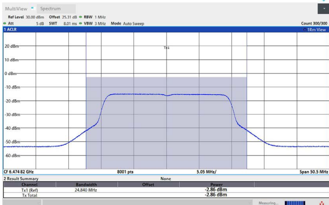
11AX20MIMO-Ant2-6475-PASS
