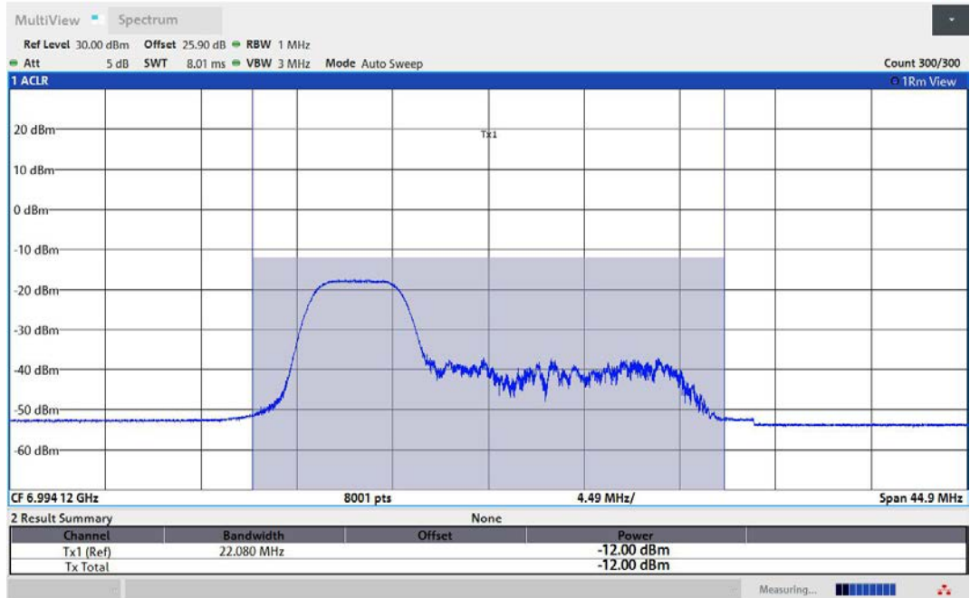
11AX80MIMO-Ant2-7025-52Tone-RU37-PASS
