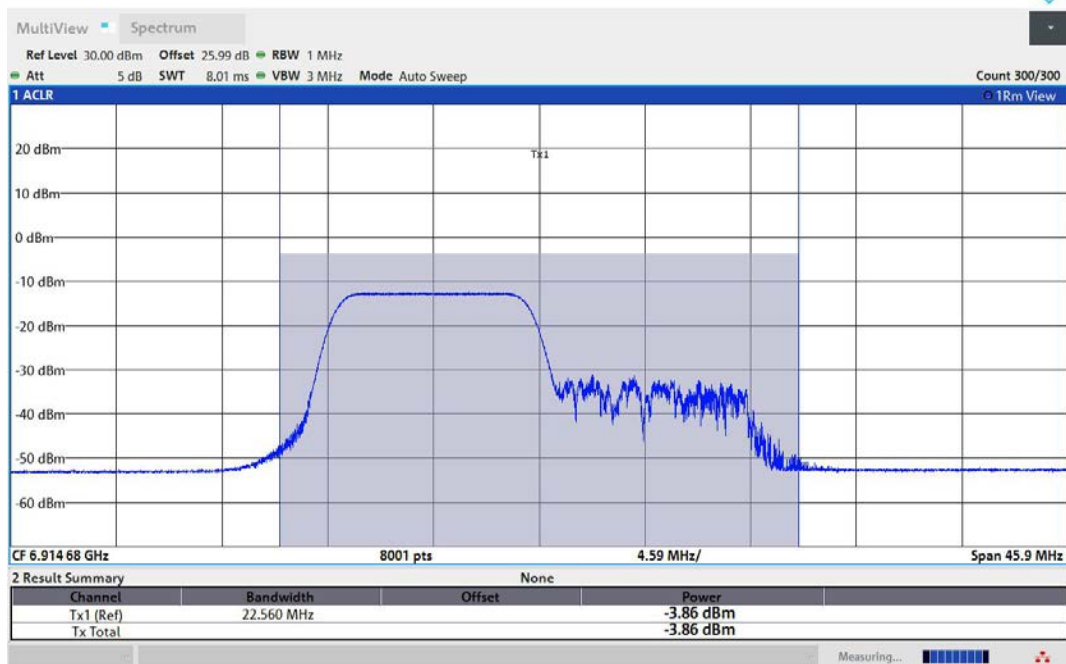
11AX80MIMO-Ant1-6945-106Tone-RU53-PASS
