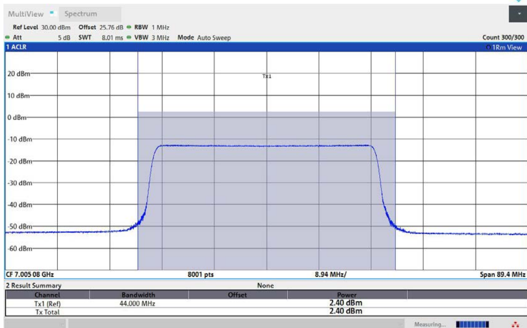
11AX80MIMO-Ant1-7025-484Tone-RU65-PASS
