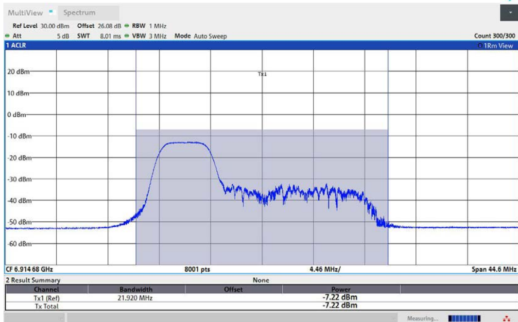
11AX80MIMO-Ant1-6945-52Tone-RU37-PASS
