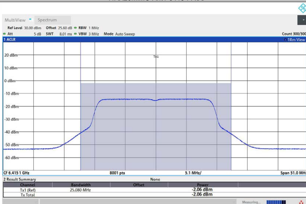
11AX20MIMO-Ant2-6415-PASS
