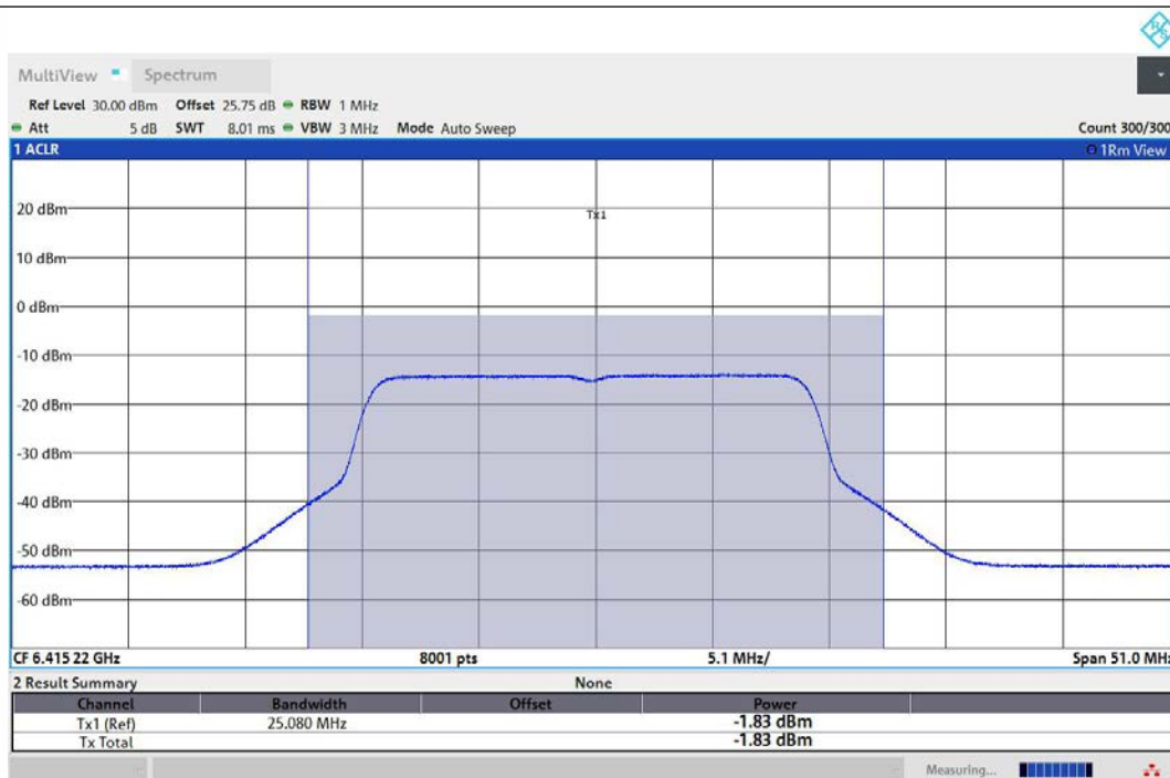
11AX20MIMO-Ant1-6415-PASS
