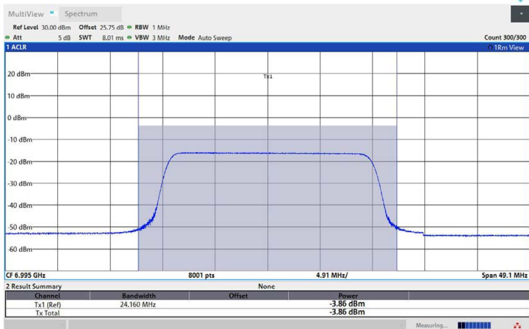
11AX80MIMO-Ant1-7025-242Tone-RU61-PASS
