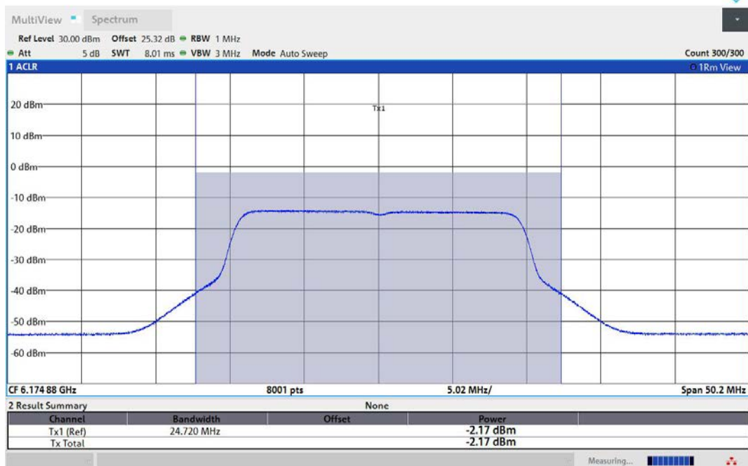
11AX20MIMO-Ant1-6175-PASS
