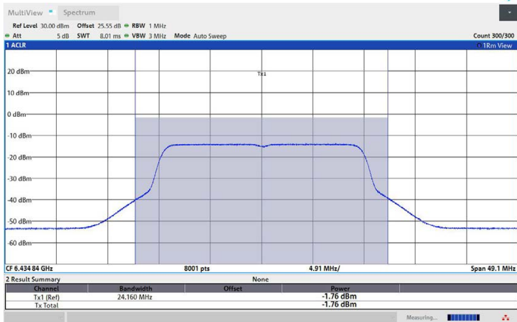
11AX20MIMO-Ant2-6435-PASS
