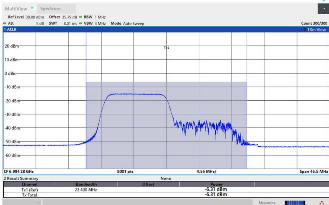
11AX80MIMO-Ant1-7025-106Tone-RU53-PASS
