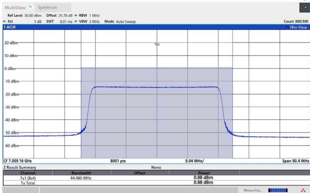
11AX80MIMO-Ant2-7025-484Tone-RU65-PASS
