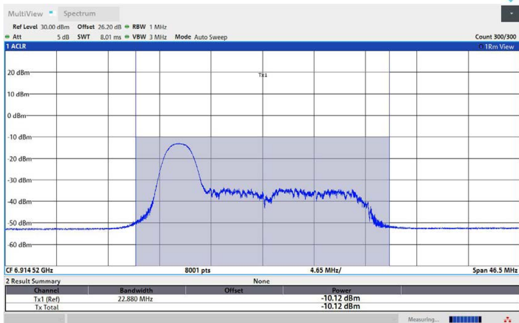
11AX80MIMO-Ant1-6945-26Tone-RU0-PASS
