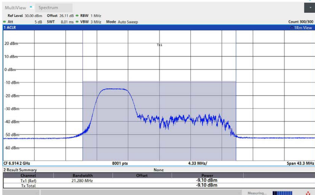
11AX80MIMO-Ant2-6945-52Tone-RU37-PASS
