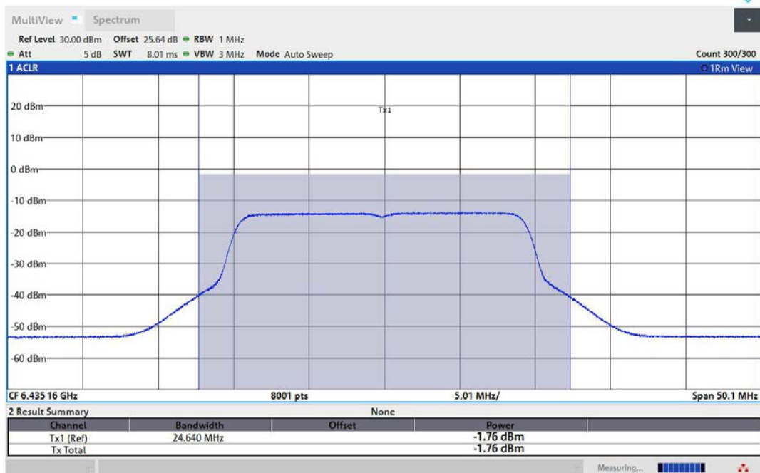
11AX20MIMO-Ant1-6435-PASS
