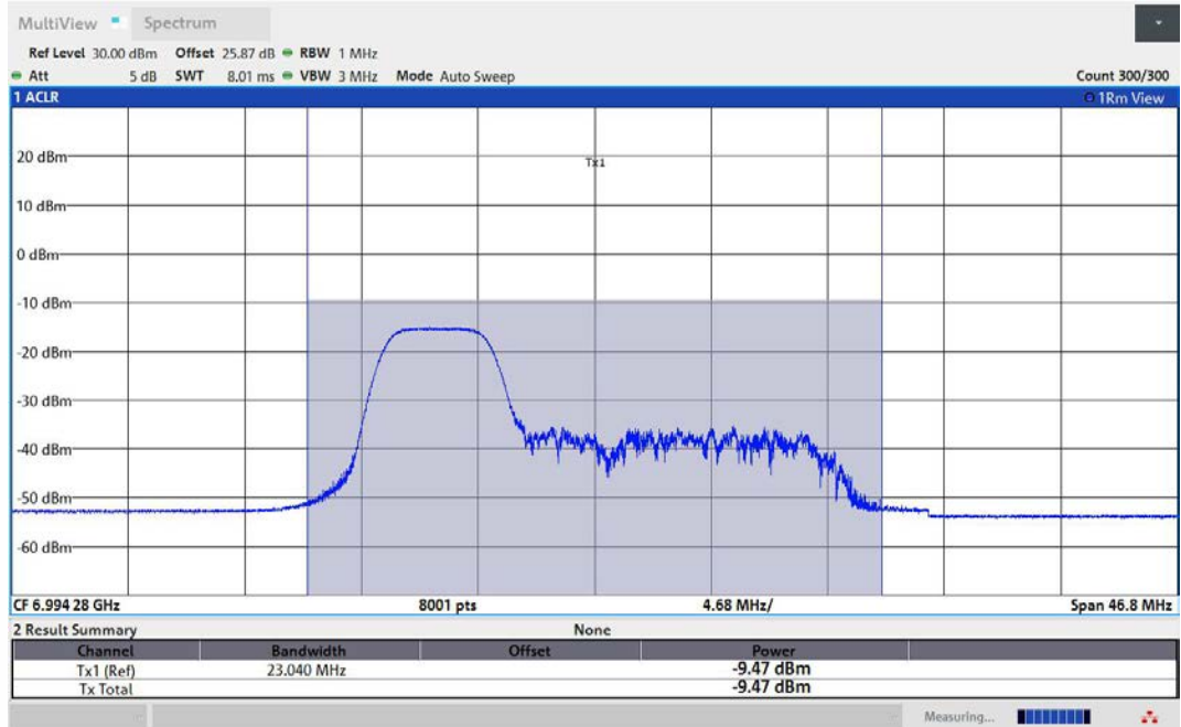
11AX80MIMO-Ant1-7025-52Tone-RU37-PASS
