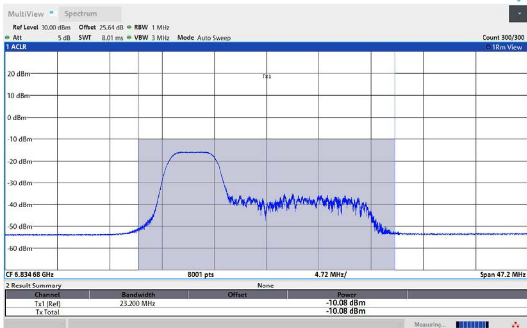
11AX80MIMO-Ant1-6865-52Tone-RU37-PASS
