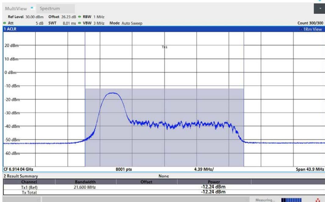
11AX80MIMO-Ant2-6945-26Tone-RU0-PASS
