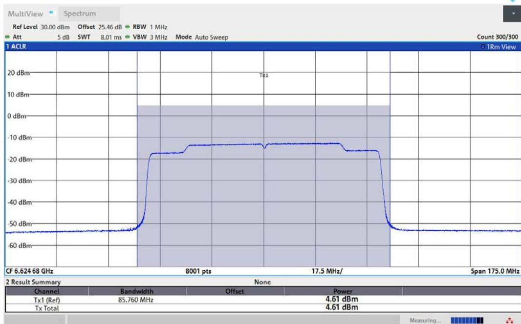
11AX160MIMO-Ant1-6665-996Tone-RU67-PASS
