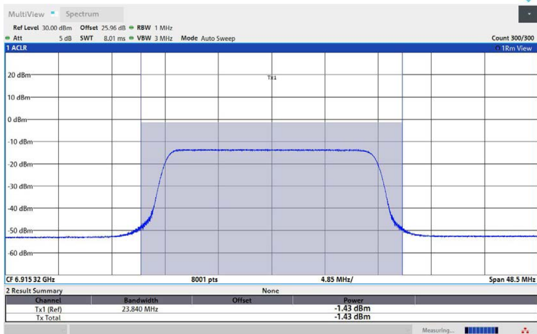
11AX80MIMO-Ant1-6945-242Tone-RU61-PASS
