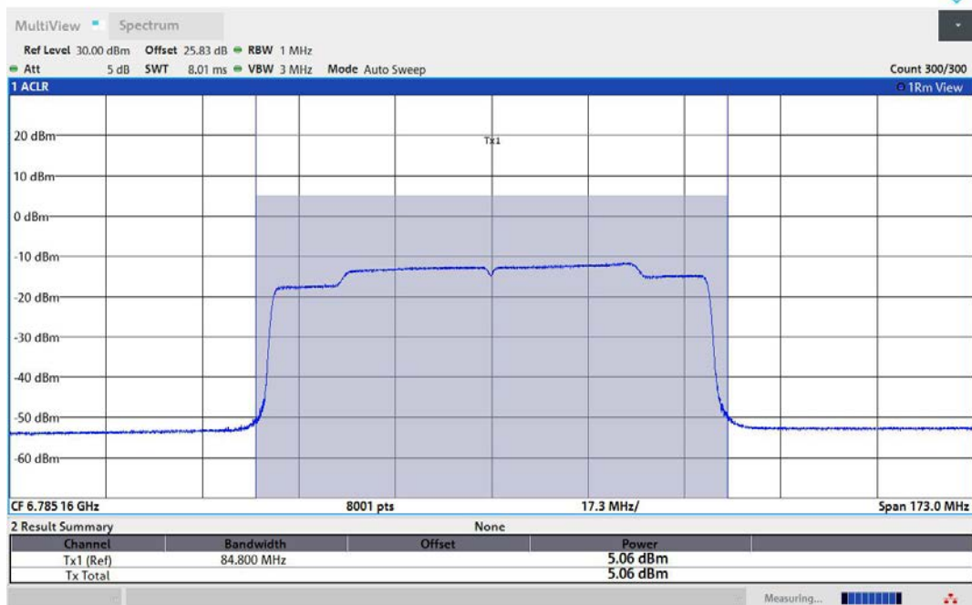
11AX160MIMO-Ant1-6825-996Tone-RU67-PASS
