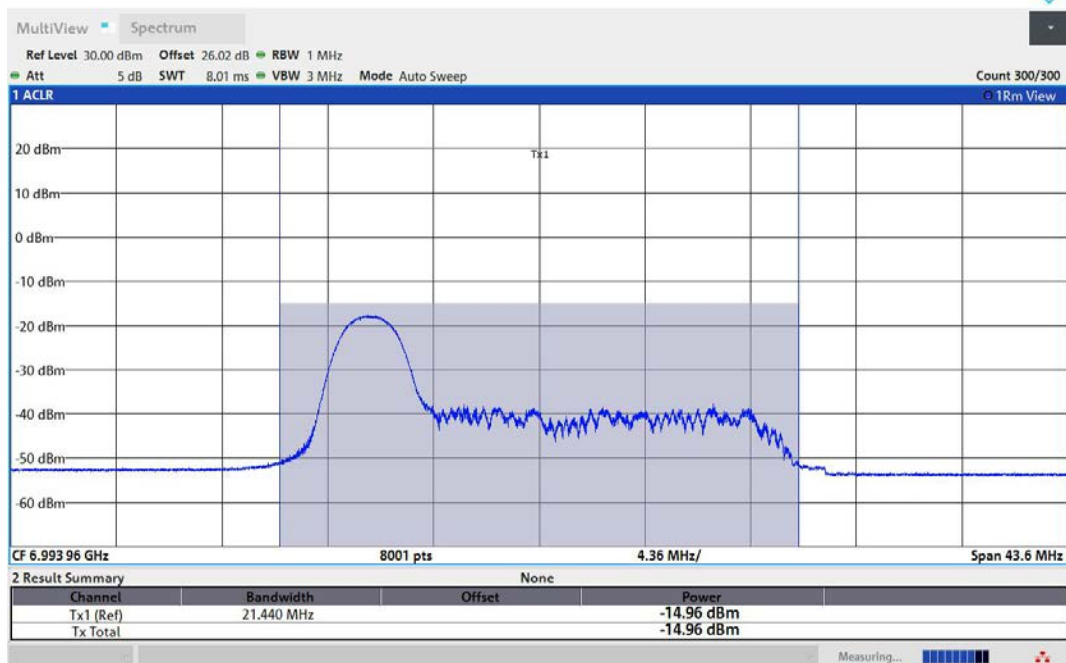
11AX80MIMO-Ant2-7025-26Tone-RU0-PASS
