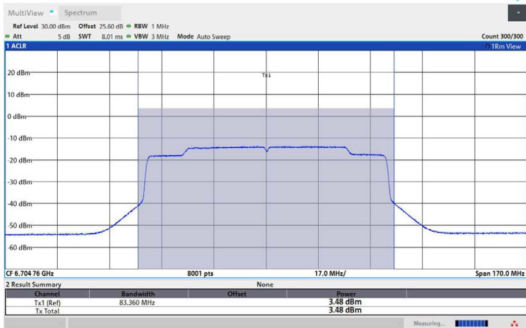
11AX80MIMO-Ant2-6705-PASS
