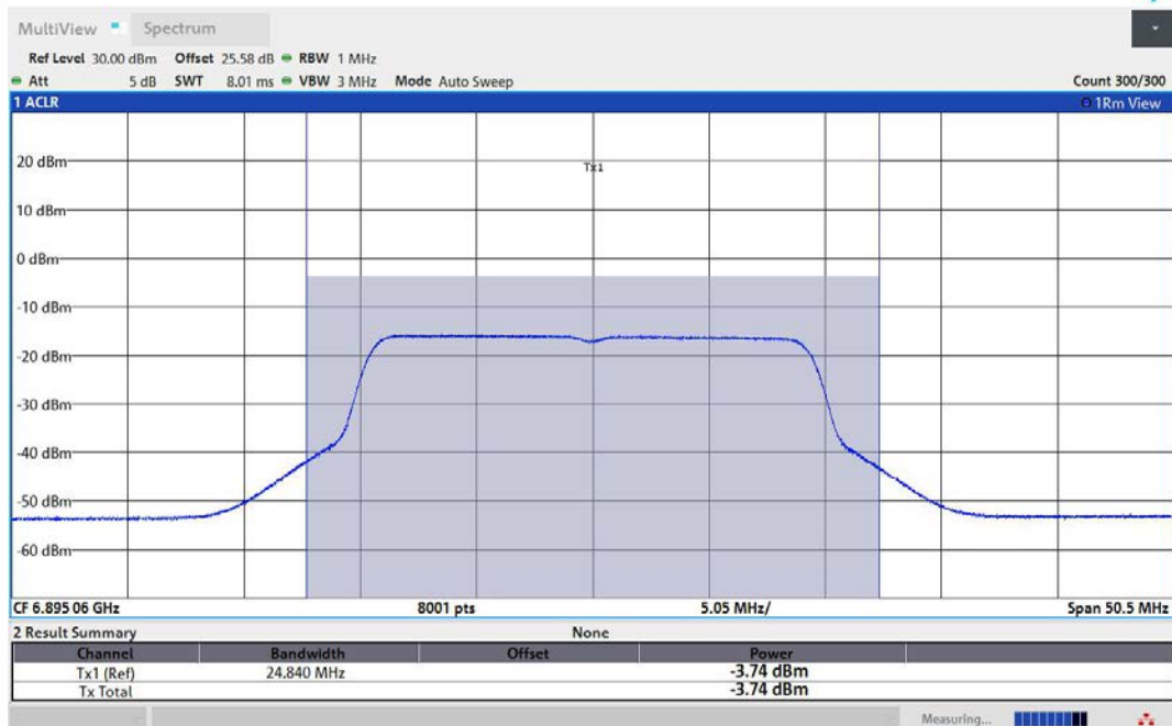
11AX20MIMO-Ant2-6895-PASS
