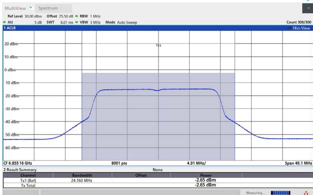
11AX20MIMO-Ant1-6855-PASS
