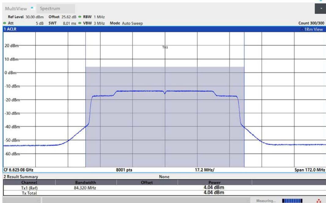
11AX80MIMO-Ant1-6625-PASS
