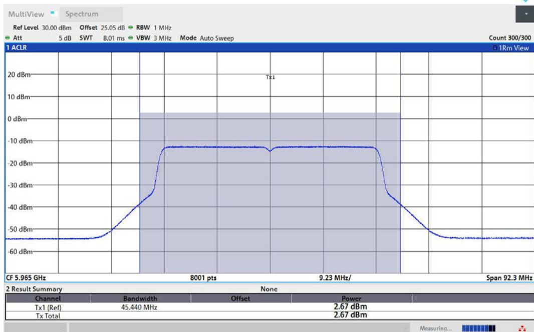
11AX40MIMO-Ant1-5965-PASS
