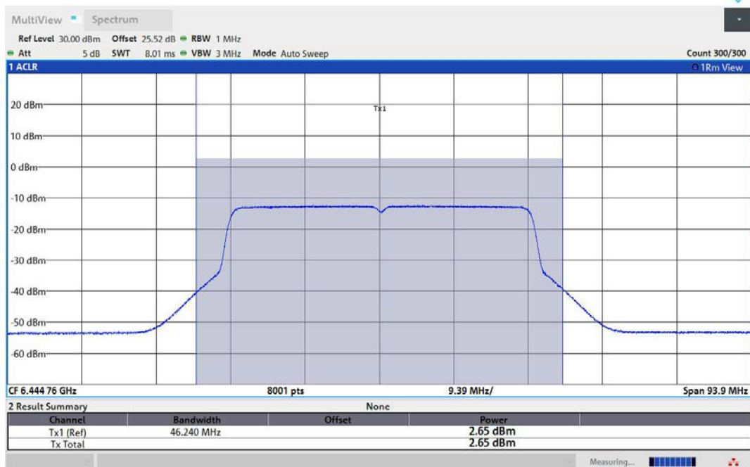
11AX40MIMO-Ant1-6445-PASS
