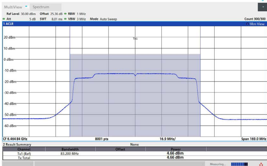
11AX80MIMO-Ant1-6465-PASS
