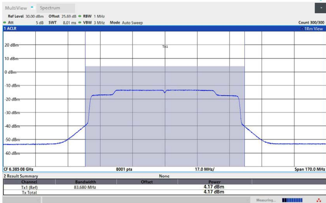
11AX80MIMO-Ant2-6385-PASS
