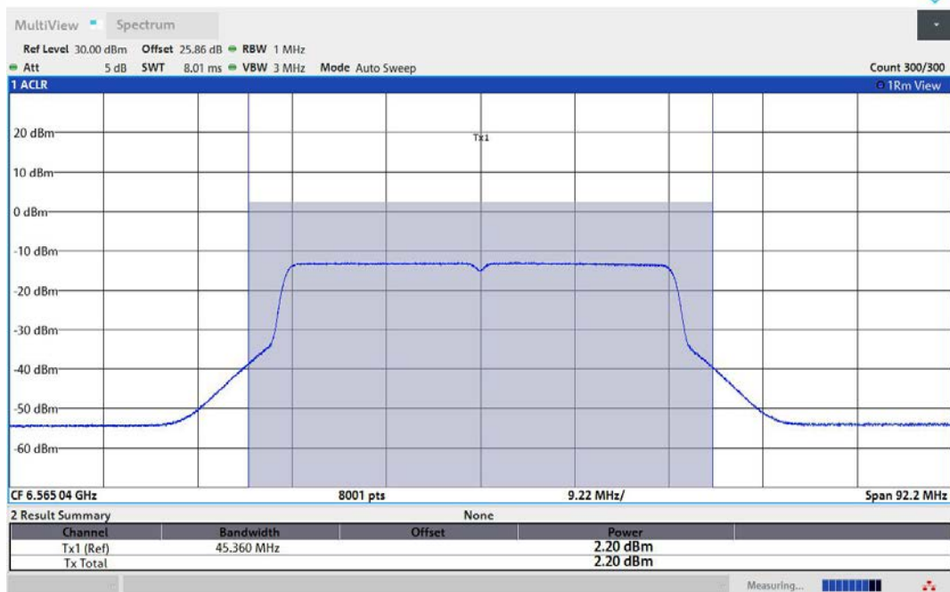
11AX40MIMO-Ant1-6565-PASS
