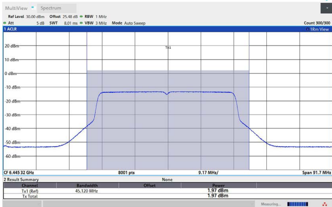
11AX40MIMO-Ant2-6445-PASS
