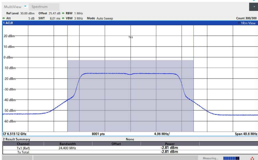
11AX20MIMO-Ant1-6515-PASS
