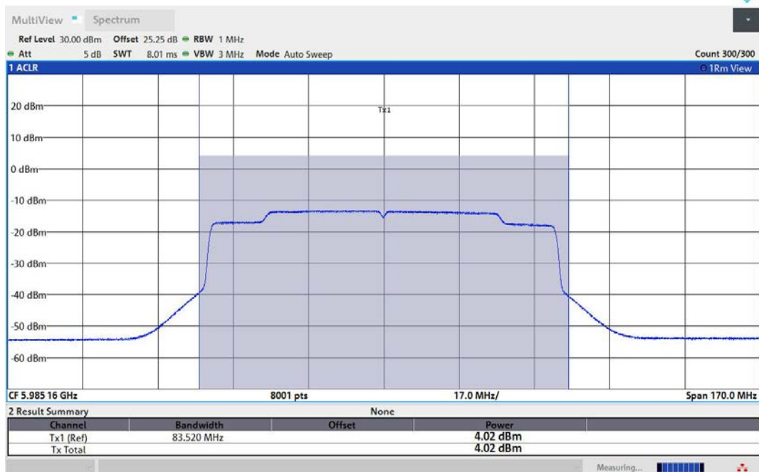
11AX80MIMO-Ant2-5985-PASS
