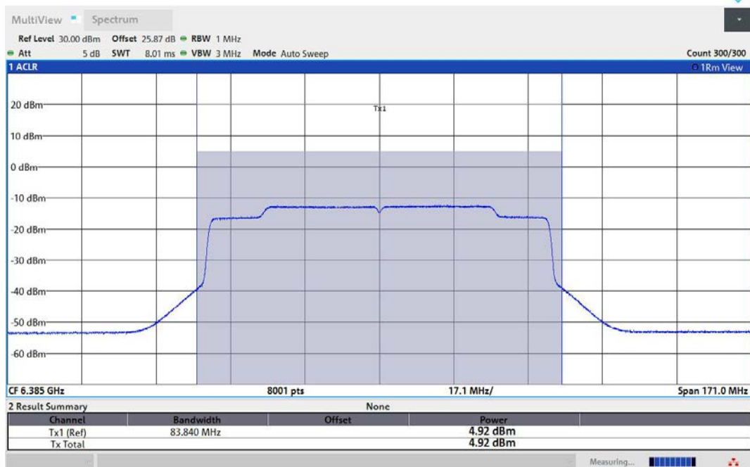
11AX80MIMO-Ant1-6385-PASS
