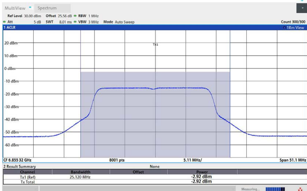
11AX20MIMO-Ant2-6855-PASS
