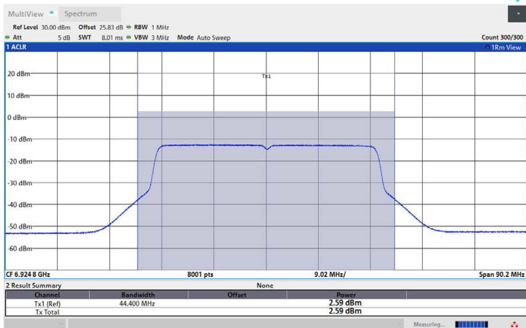
11AX40MIMO-Ant1-6925-PASS
