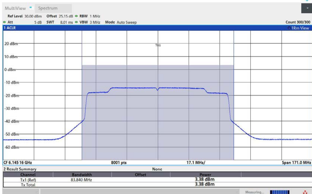
11AX80MIMO-Ant2-6145-PASS
