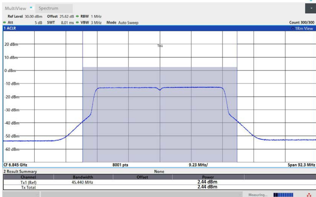
11AX40MIMO-Ant1-6845-PASS
