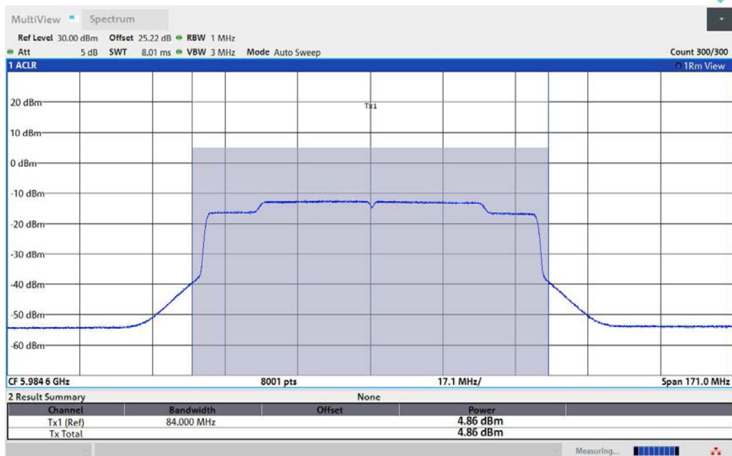
11AX80MIMO-Ant1-5985-PASS
