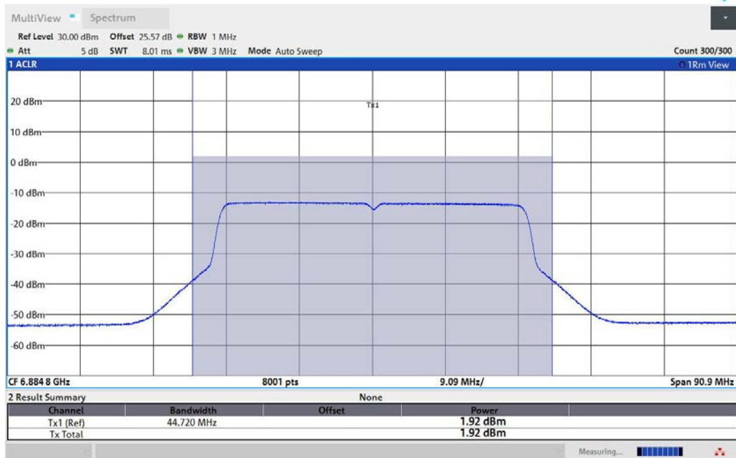
11AX40MIMO-Ant2-6885-PASS
