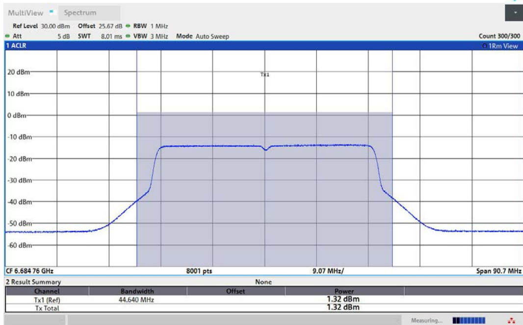
11AX40MIMO-Ant2-6685-PASS
