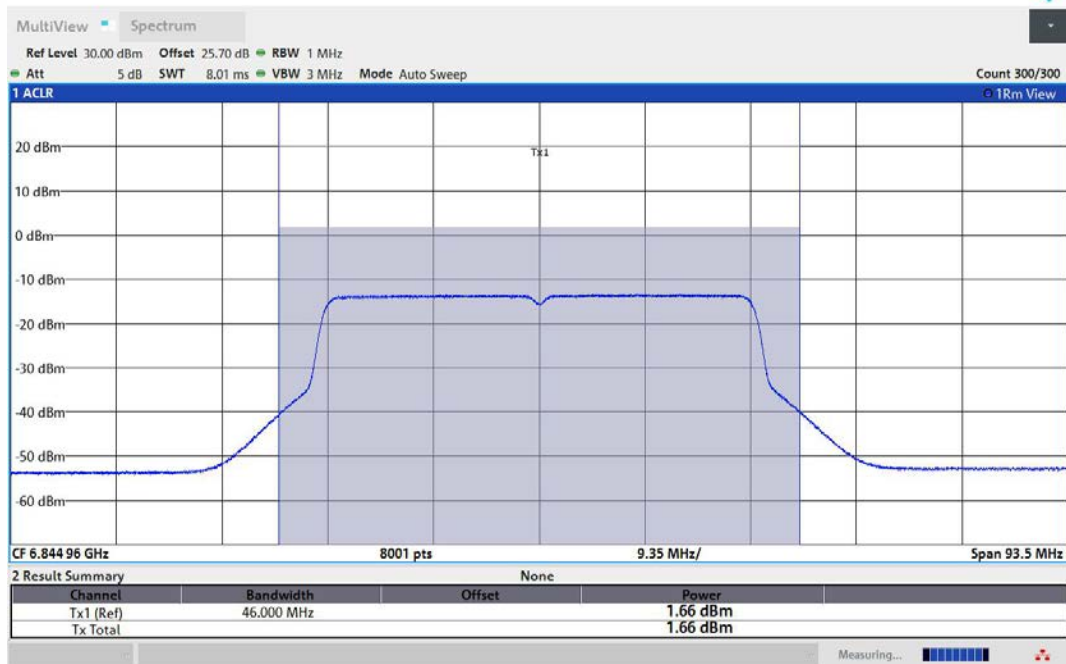
11AX40MIMO-Ant2-6845-PASS
