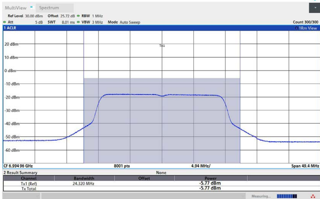
11AX20MIMO-Ant2-6995-PASS
