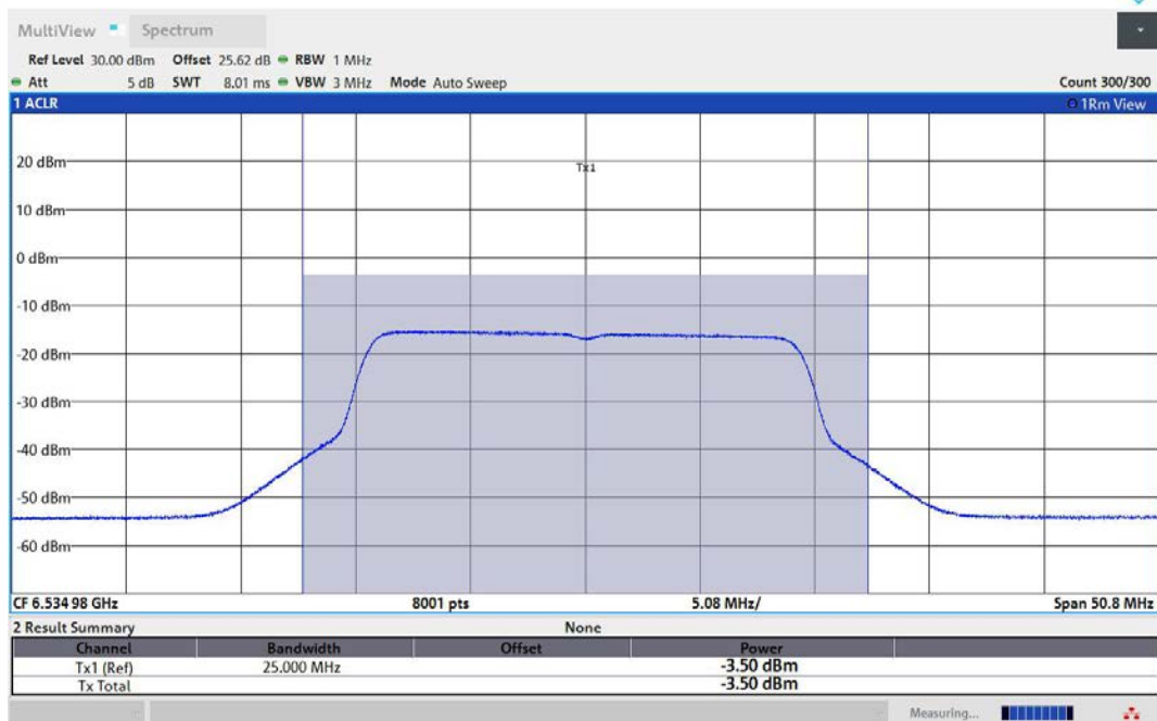
11AX20MIMO-Ant1-6535-PASS
