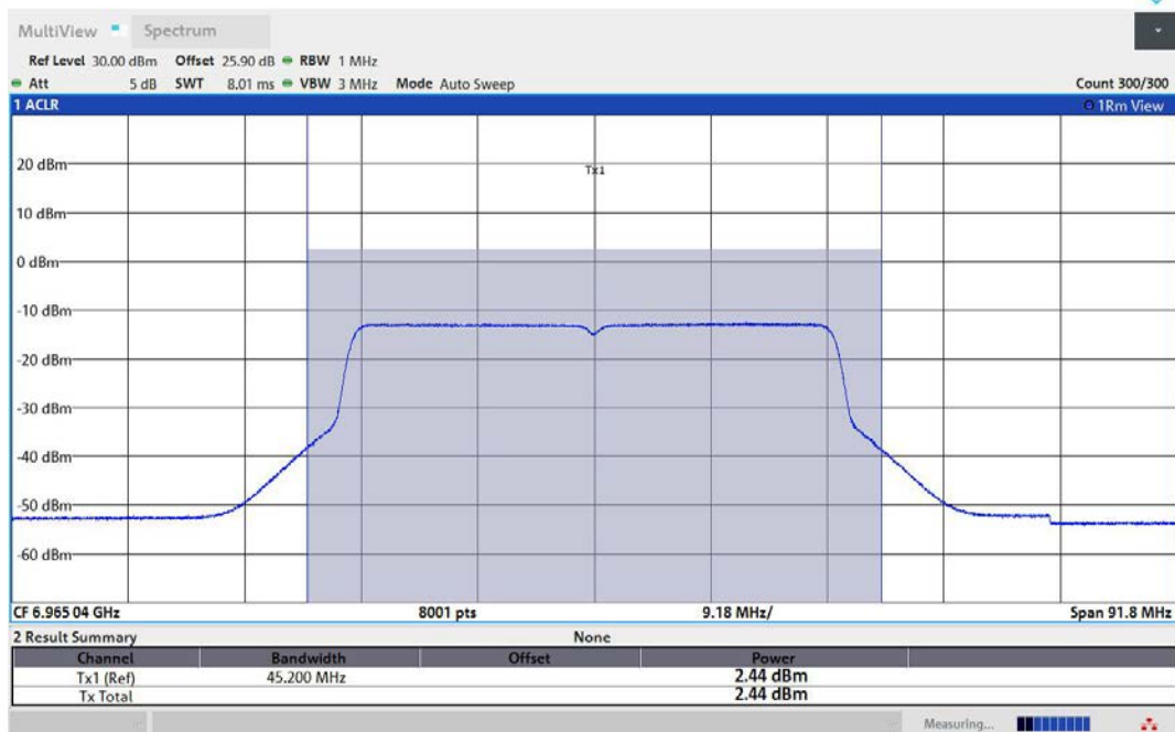
11AX40MIMO-Ant1-6965-PASS
