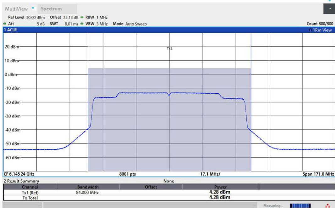
11AX80MIMO-Ant1-6145-PASS
