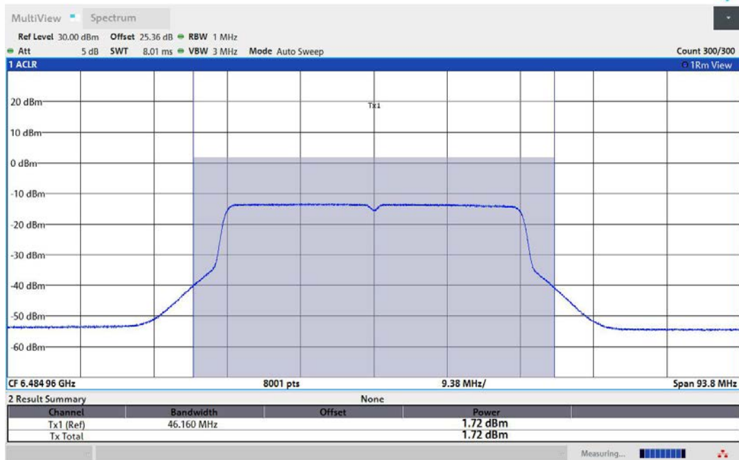
11AX40MIMO-Ant2-6485-PASS
