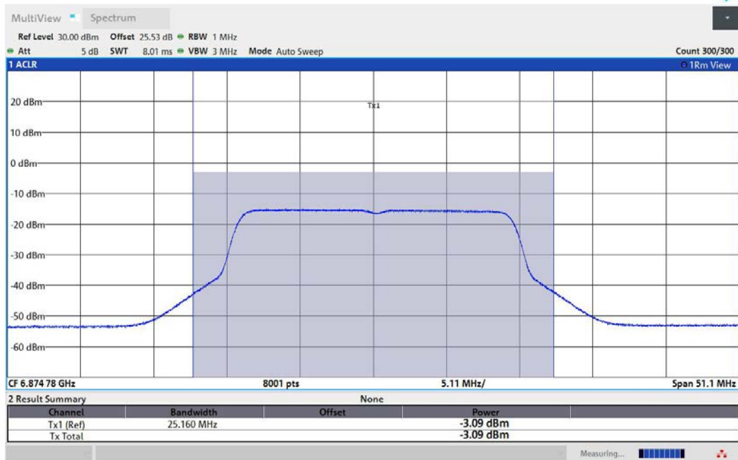
11AX20MIMO-Ant2-6875-PASS
