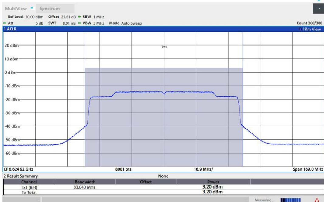
11AX80MIMO-Ant2-6625-PASS
