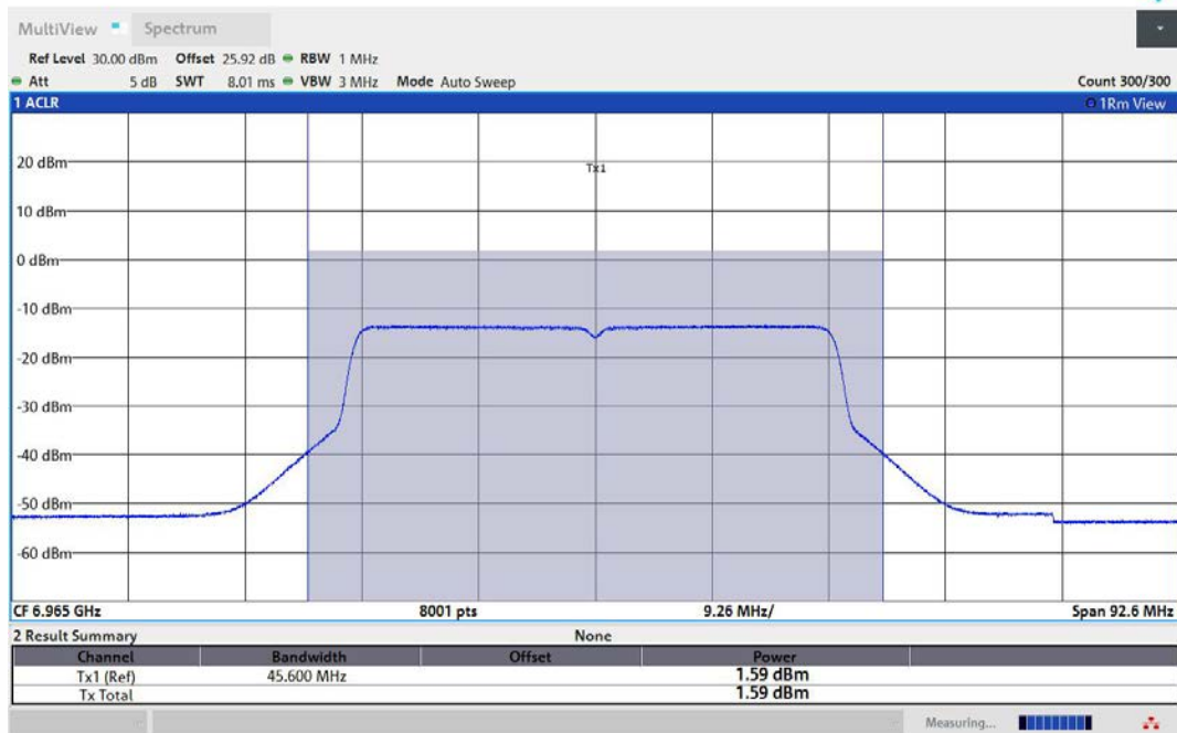
11AX40MIMO-Ant2-6965-PASS
