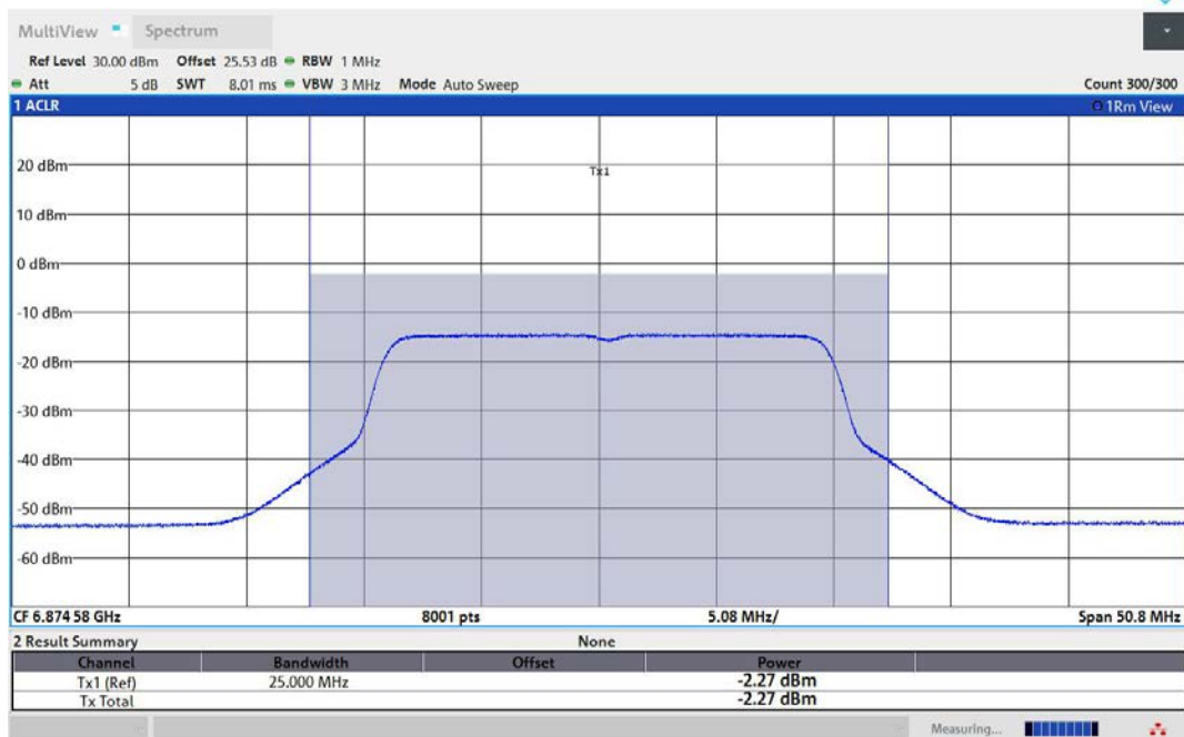
11AX20MIMO-Ant1-6875-PASS
