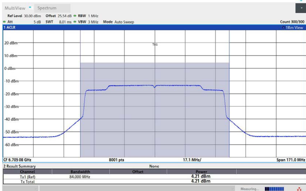
11AX80MIMO-Ant1-6705-PASS
