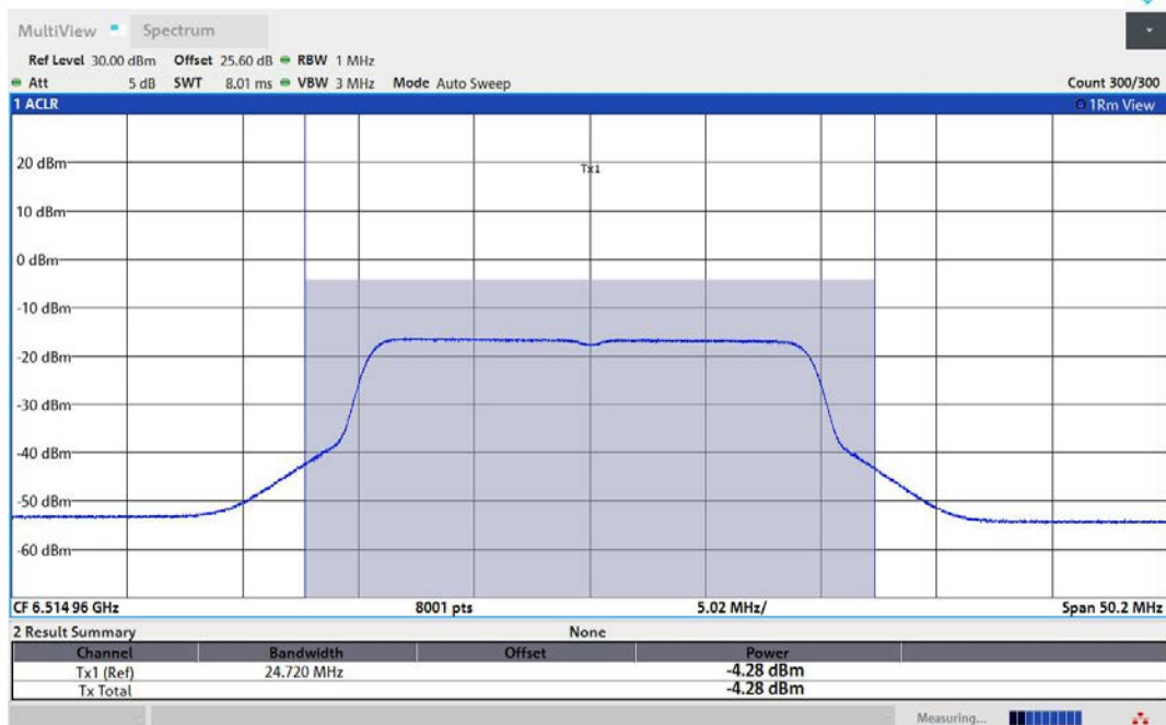
11AX20MIMO-Ant2-6515-PASS
