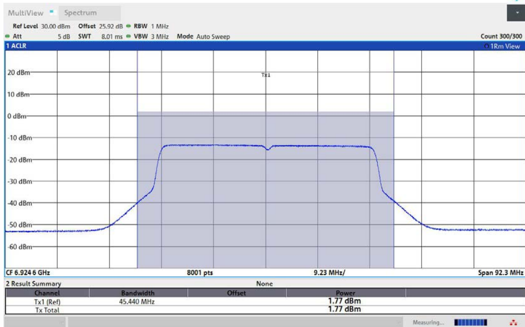
11AX40MIMO-Ant2-6925-PASS
