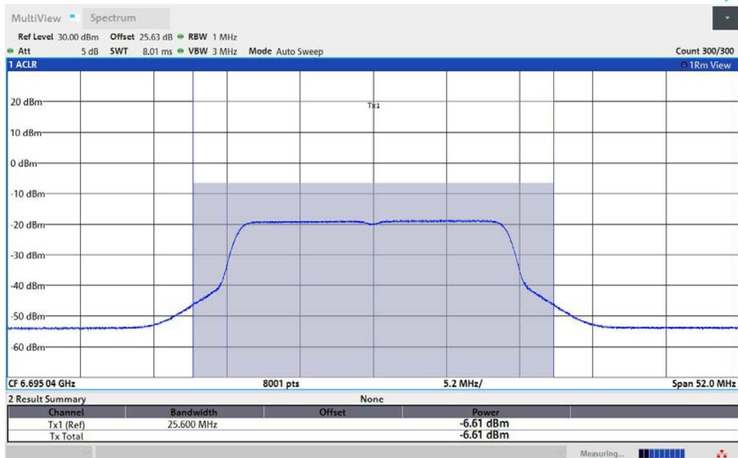
11AX20MIMO-Ant2-6695-PASS
