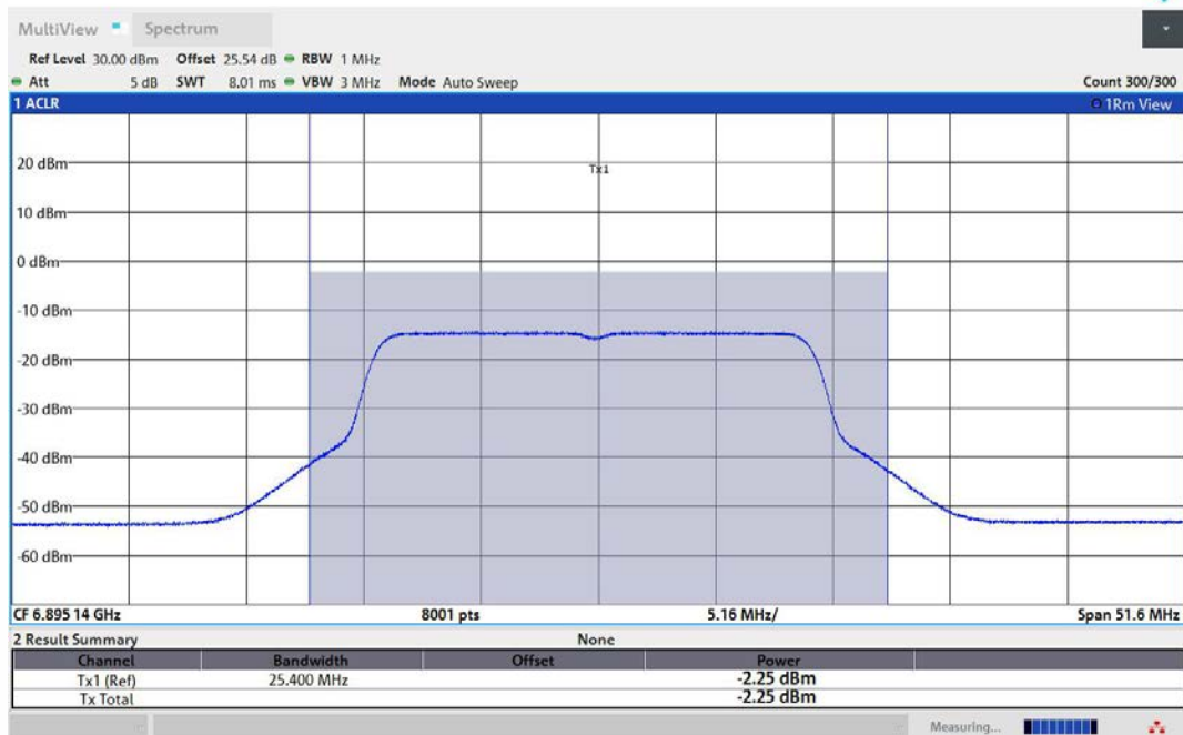
11AX20MIMO-Ant1-6895-PASS
