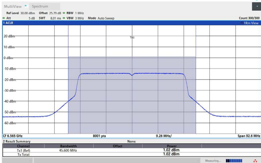
11AX40MIMO-Ant2-6565-PASS
