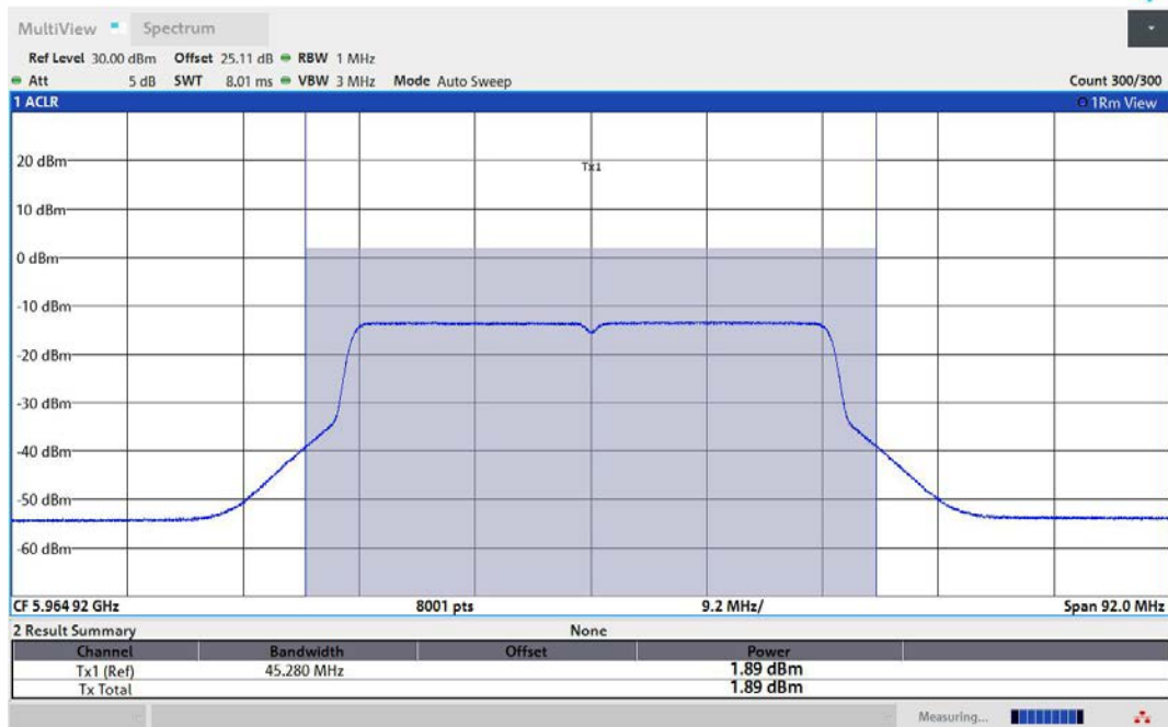
11AX40MIMO-Ant2-5965-PASS
