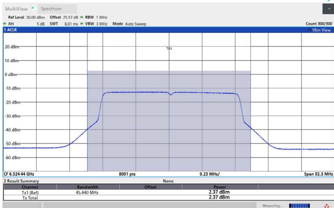
11AX40MIMO-Ant1-6525-PASS
