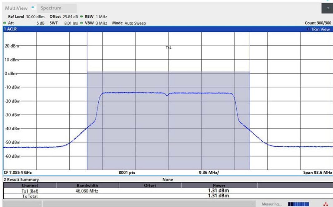
11AX40MIMO-Ant2-7085-PASS
