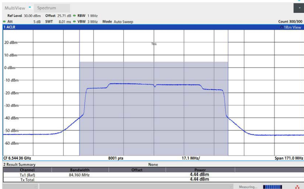
11AX80MIMO-Ant1-6545-PASS
