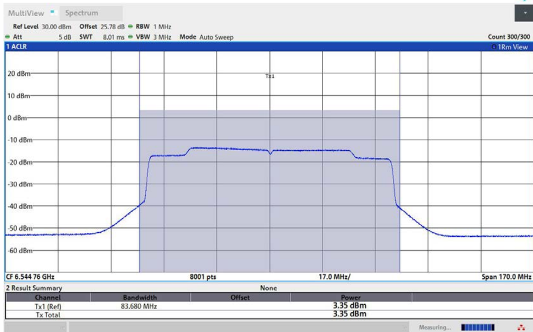
11AX80MIMO-Ant2-6545-PASS
