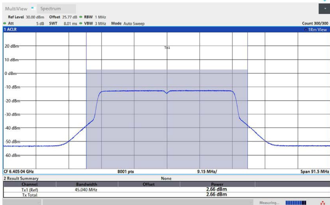
11AX40MIMO-Ant1-6405-PASS
