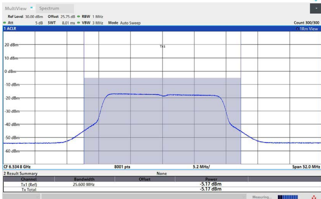
11AX20MIMO-Ant2-6535-PASS
