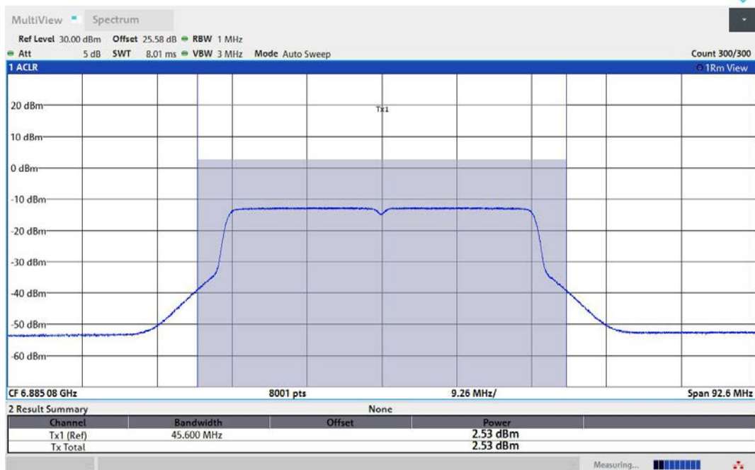
11AX40MIMO-Ant1-6885-PASS
