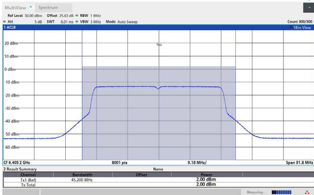
11AX40MIMO-Ant2-6405-PASS
