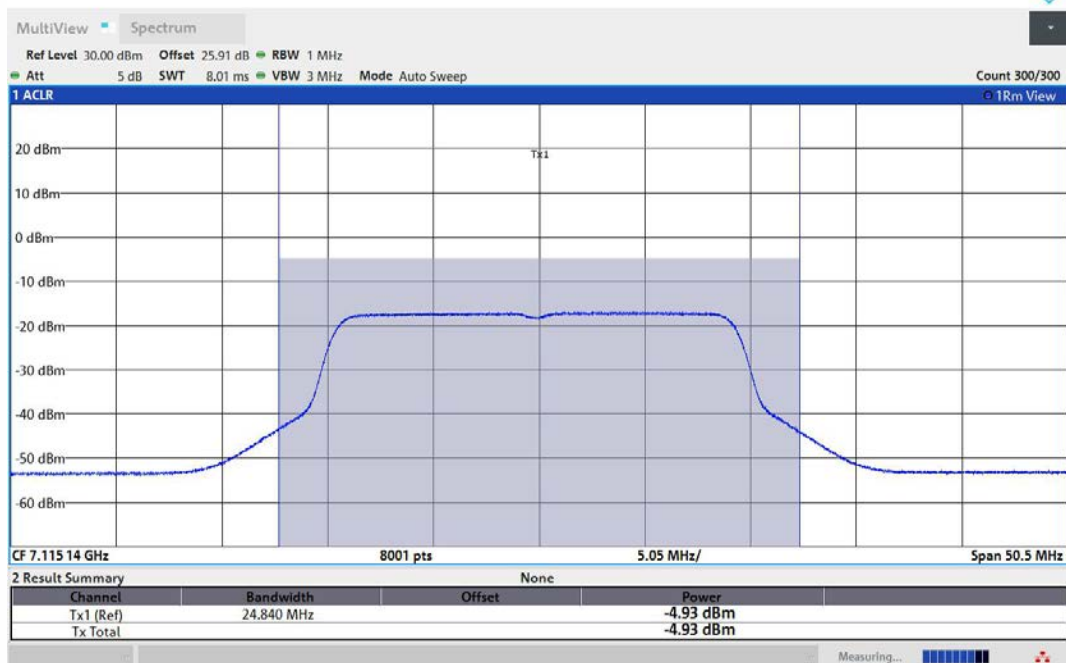
11AX20MIMO-Ant2-7115-PASS
