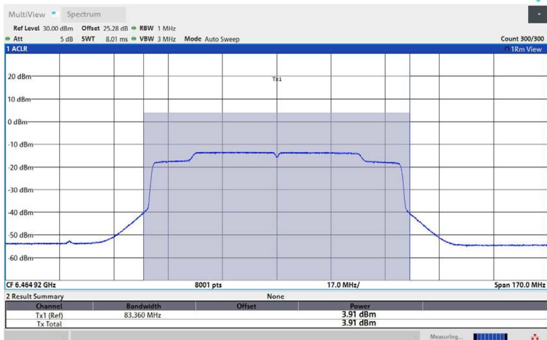
11AX80MIMO-Ant2-6465-PASS
