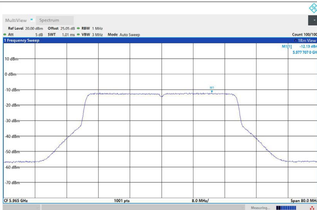
11AX40MIMO-Ant1-5965-PASS
