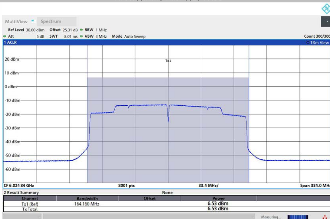
11AX160MIMO-Ant2-6025-PASS
