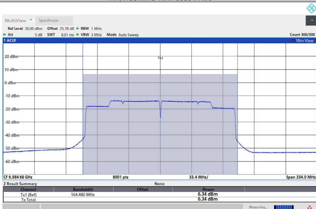
11AX160MIMO-Ant2-6985-PASS
