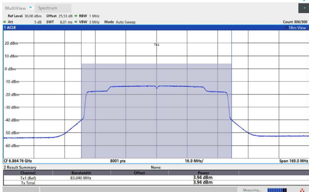
11AX80MIMO-Ant2-6865-PASS
