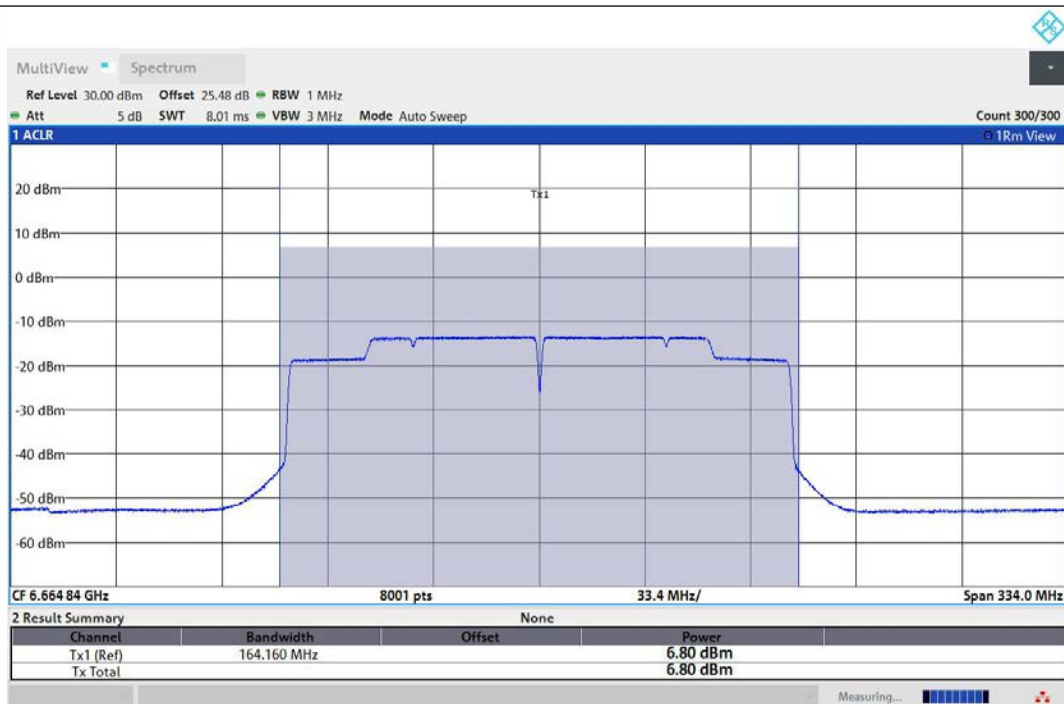
11AX160MIMO-Ant1-6665-PASS
