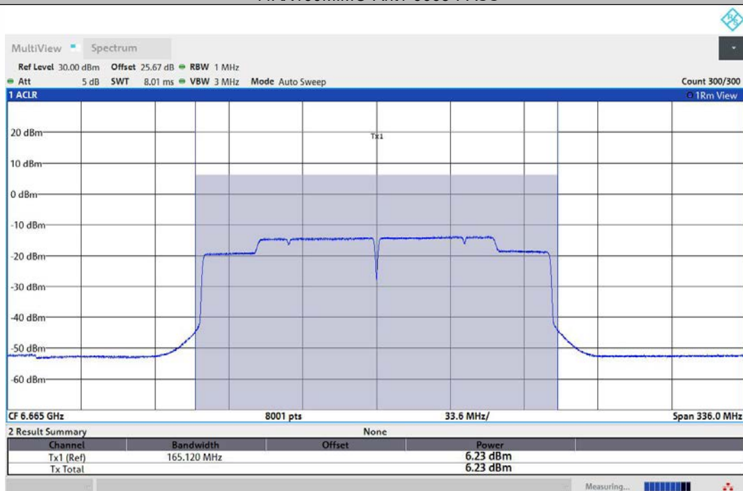
11AX160MIMO-Ant2-6665-PASS
