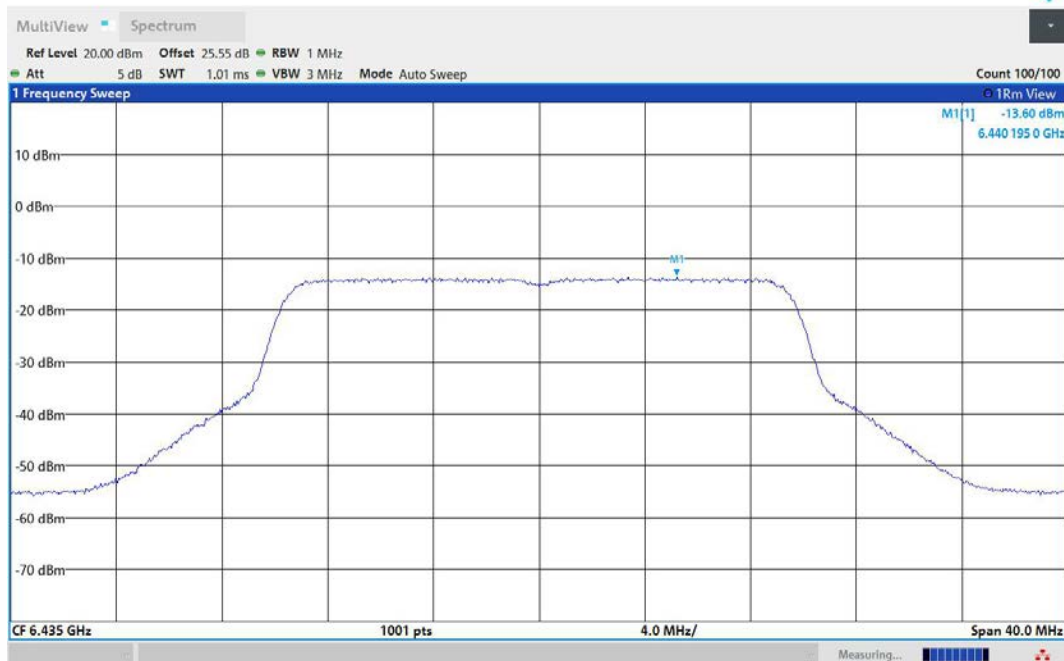
11AX20MIMO-Ant2-6435-PASS
