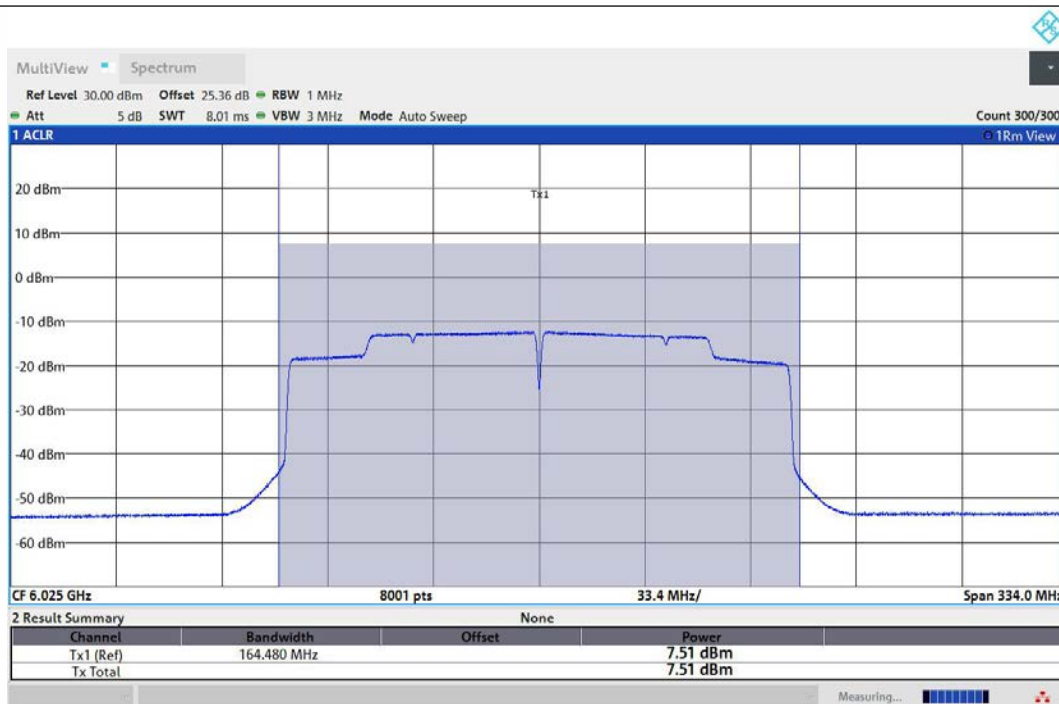
11AX160MIMO-Ant1-6025-PASS
