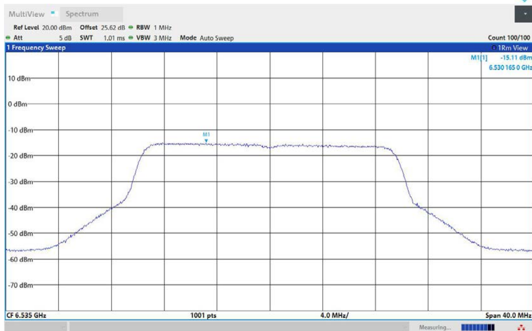
11AX20MIMO-Ant1-6535-PASS
