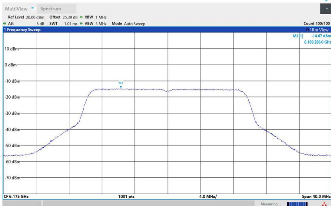
11AX20MIMO-Ant2-6175-PASS
