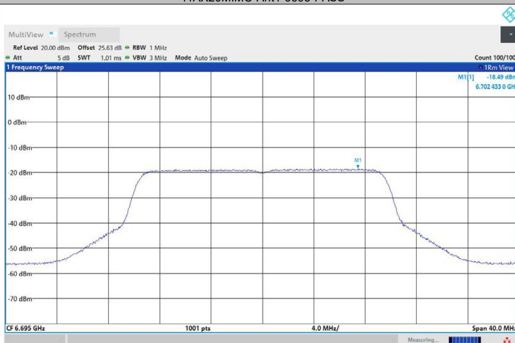
11AX20MIMO-Ant2-6695-PASS
