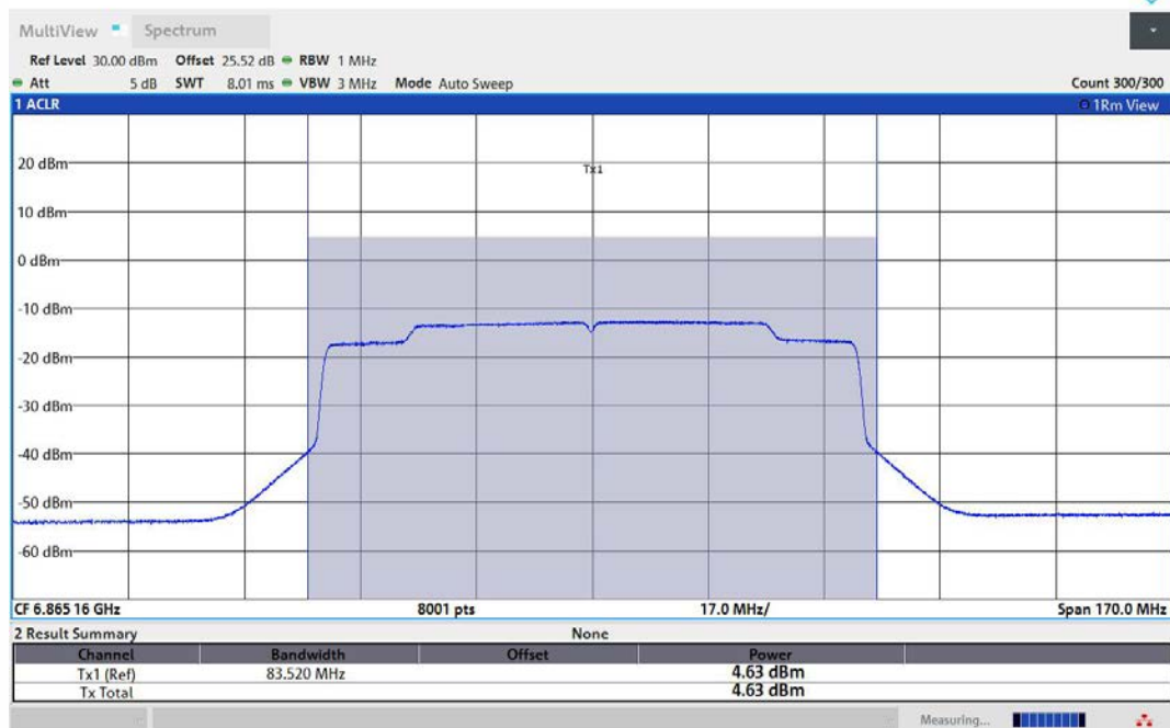
11AX80MIMO-Ant1-6865-PASS
