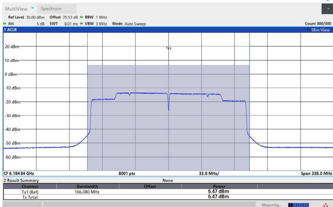
11AX160MIMO-Ant2-6185-PASS
