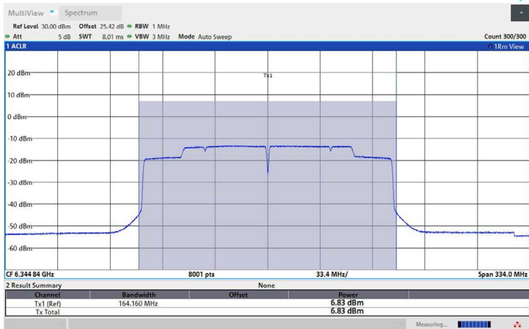
11AX160MIMO-Ant2-6345-PASS
