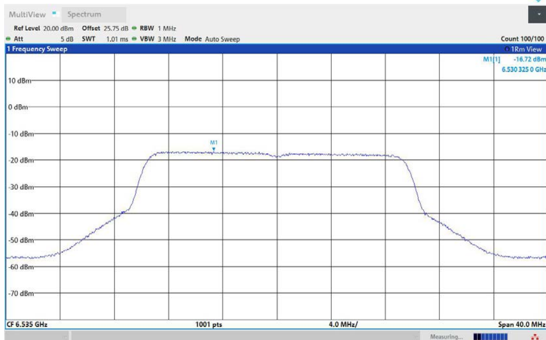
11AX20MIMO-Ant2-6535-PASS
