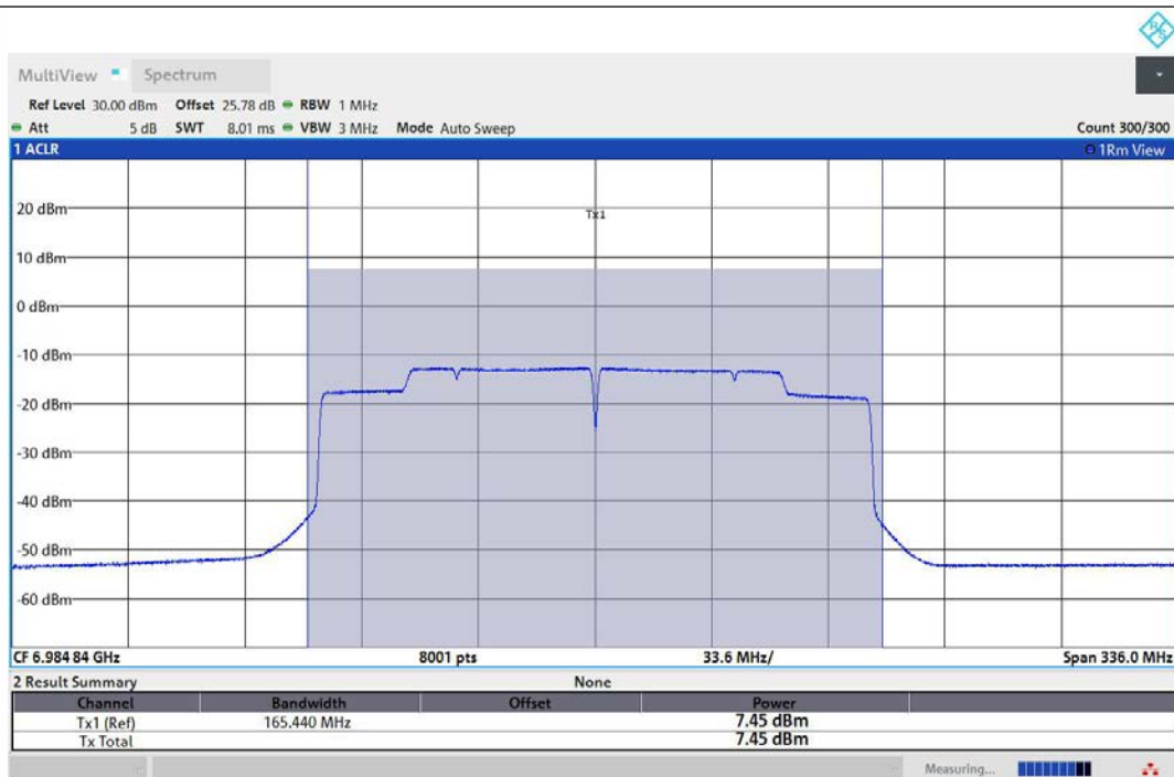
11AX160MIMO-Ant1-6985-PASS
