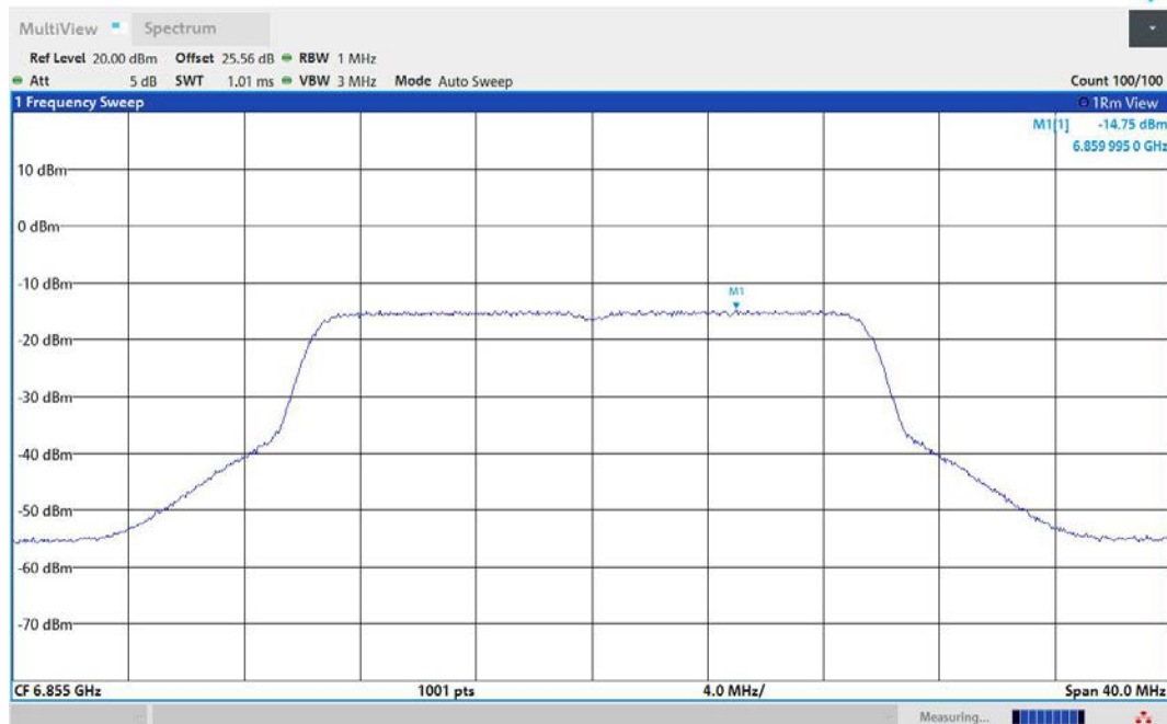
11AX20MIMO-Ant2-6855-PASS
