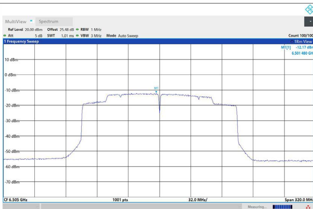
11AX160MIMO-Ant1-6505-PASS
