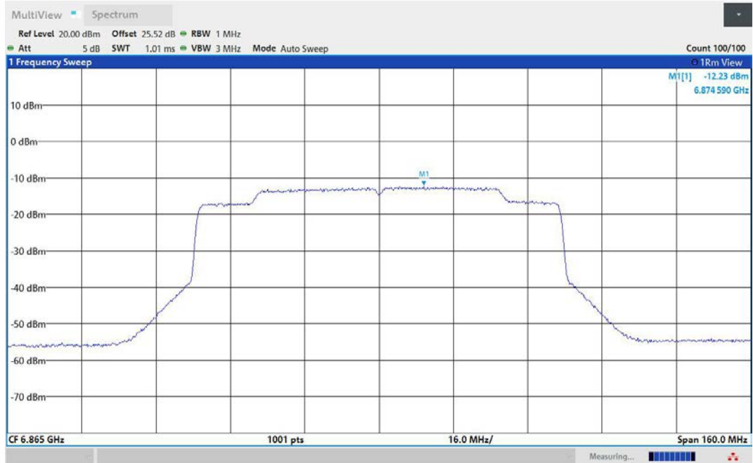
11AX80MIMO-Ant1-6865-PASS
