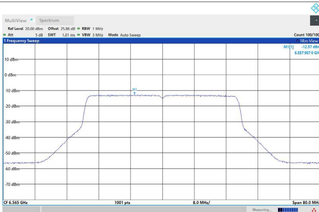
11AX40MIMO-Ant1-6565-PASS
