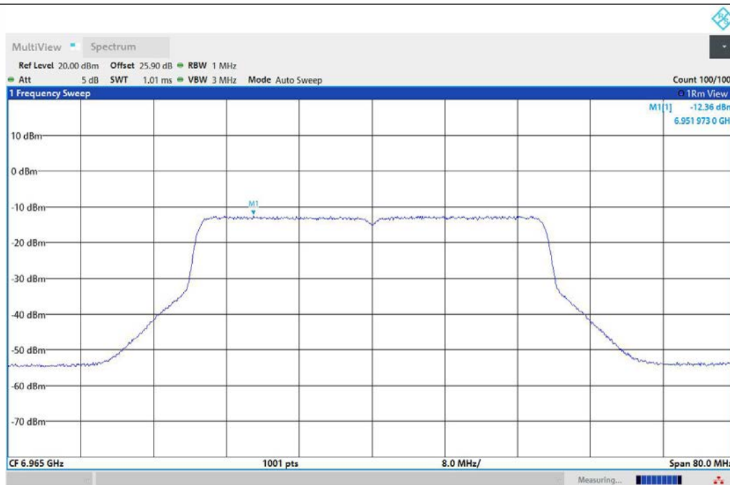
11AX40MIMO-Ant1-6965-PASS
