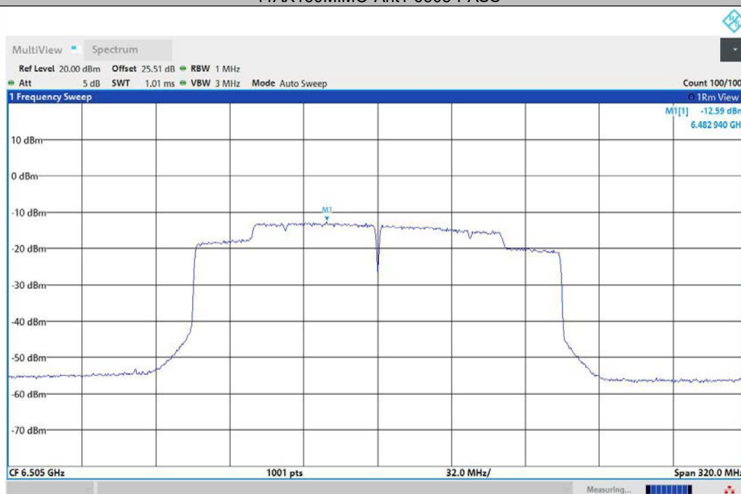
11AX160MIMO-Ant2-6505-PASS
