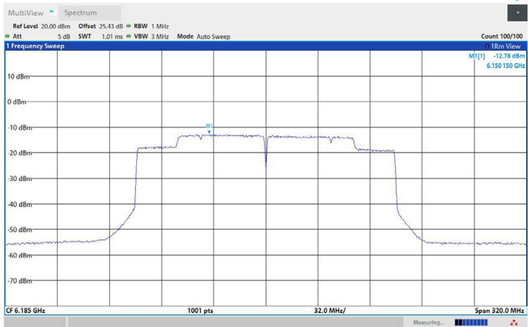
11AX160MIMO-Ant1-6185-PASS
