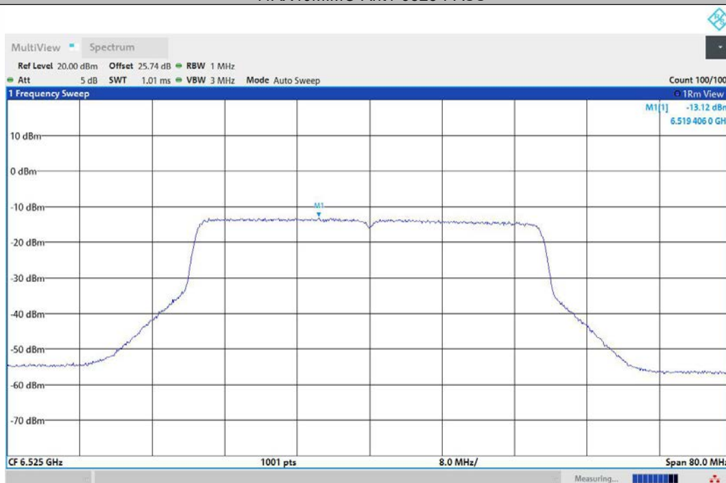
11AX40MIMO-Ant2-6525-PASS
