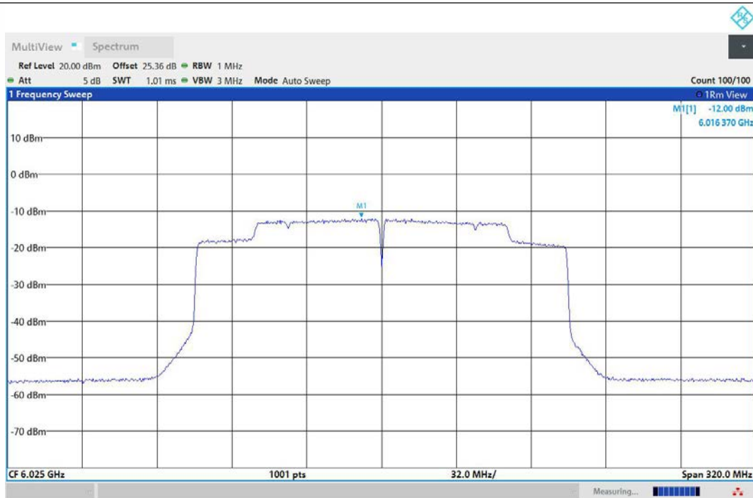
11AX160MIMO-Ant1-6025-PASS
