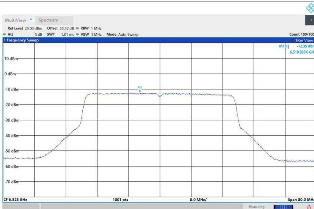
11AX40MIMO-Ant1-6525-PASS
