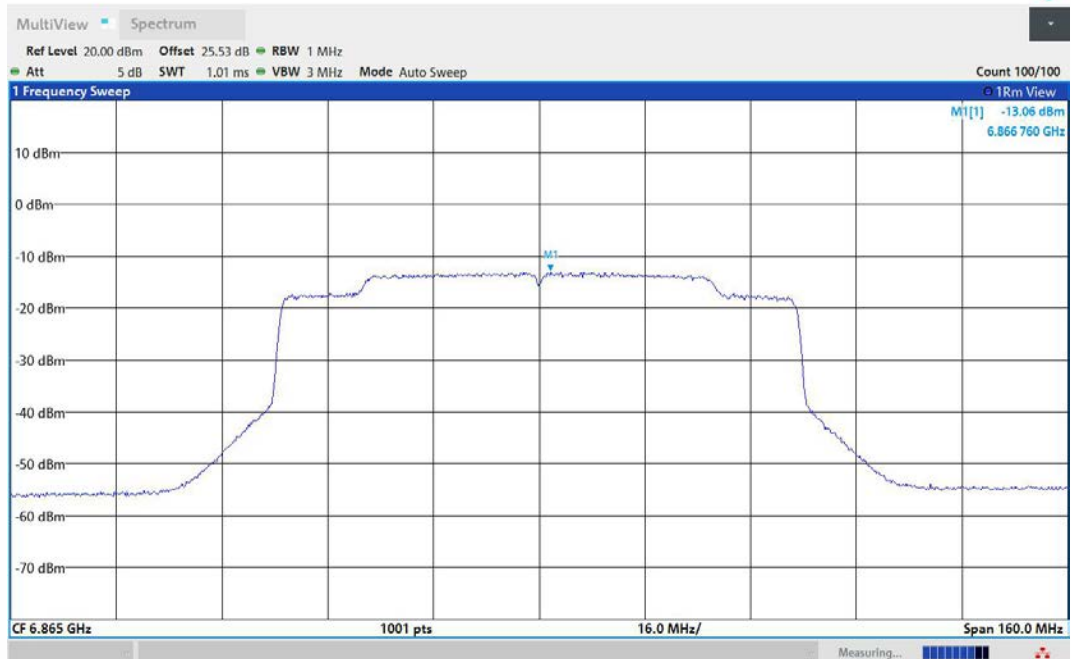
11AX80MIMO-Ant2-6865-PASS
