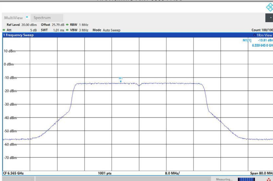
11AX40MIMO-Ant2-6565-PASS
