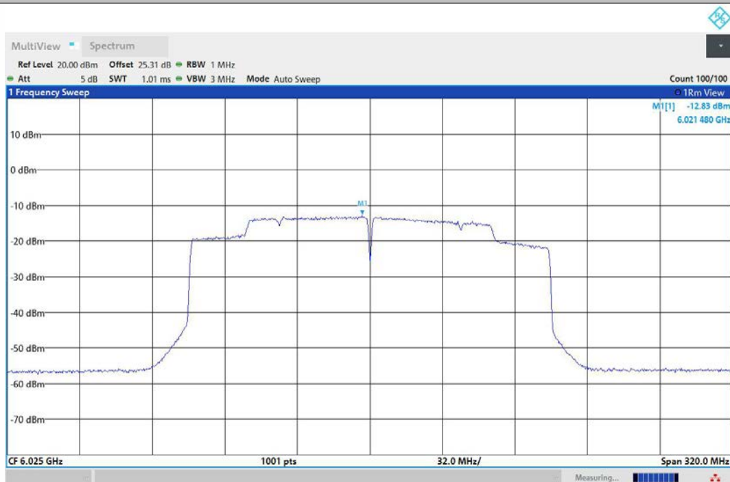
11AX160MIMO-Ant2-6025-PASS
