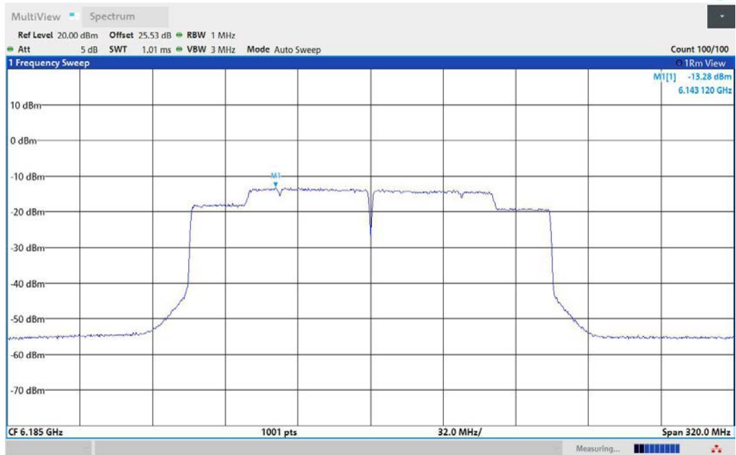
11AX160MIMO-Ant2-6185-PASS
