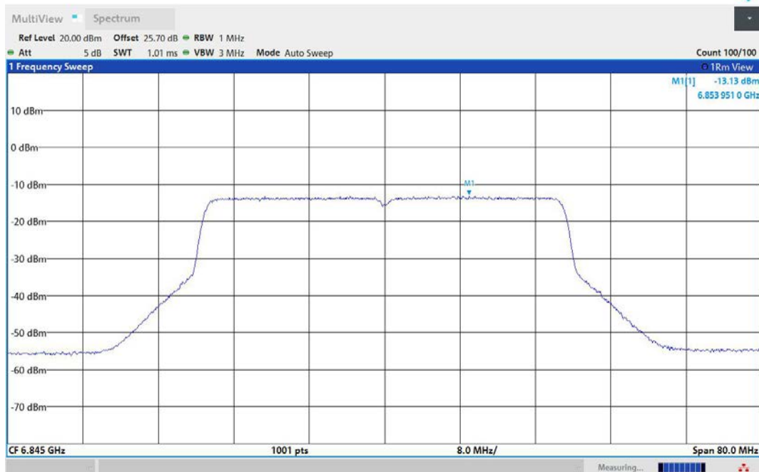
11AX40MIMO-Ant2-6845-PASS
