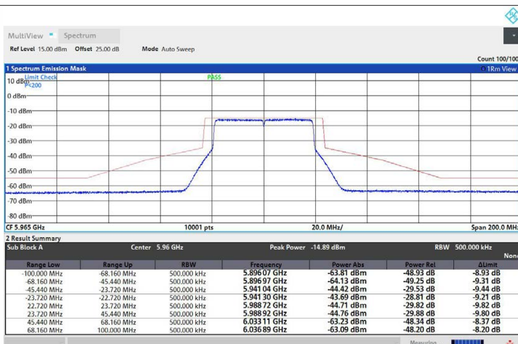
NTNV-11AX40MIMO-Ant1-5965-PASS
