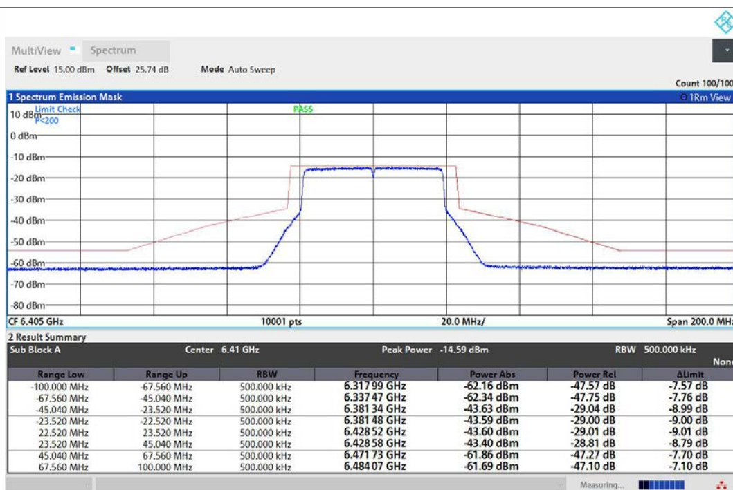
NTNV-11AX40MIMO-Ant1-6405-PASS
