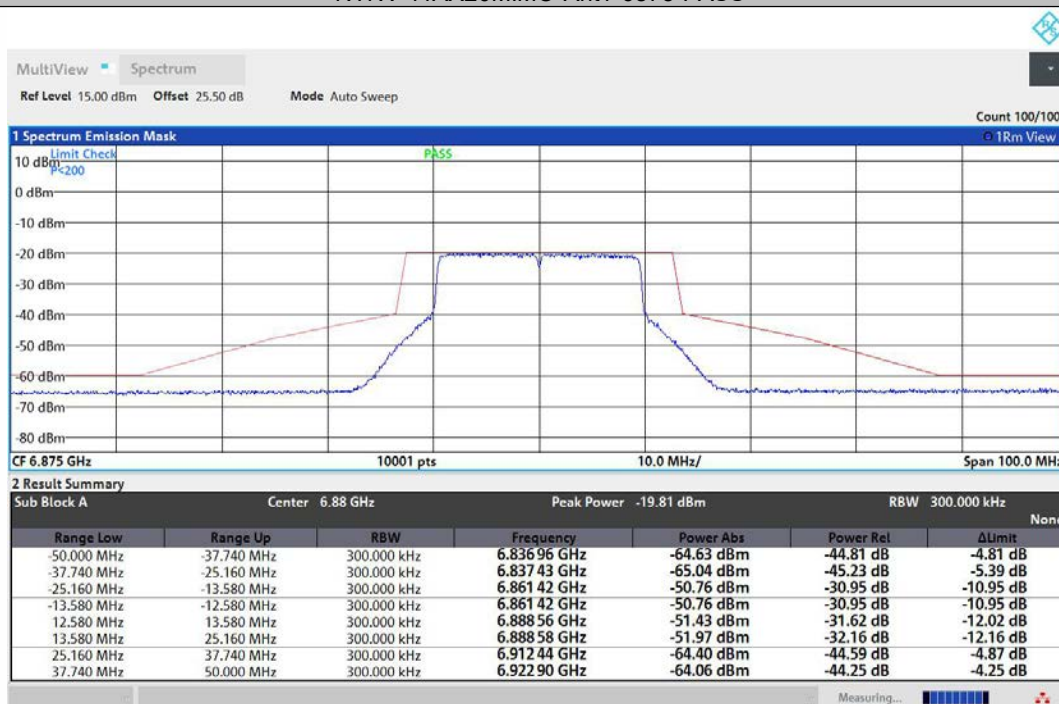
NTNV-11AX20MIMO-Ant2-6875-PASS
