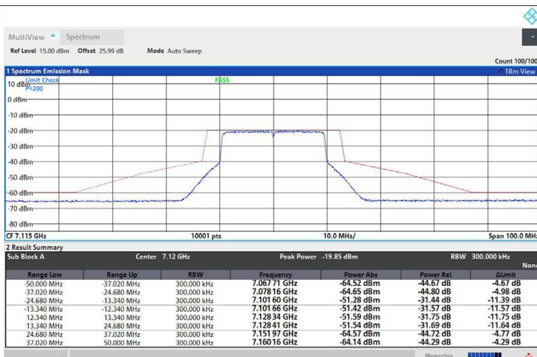
NTNV-11AX20MIMO-Ant1-7115-PASS
