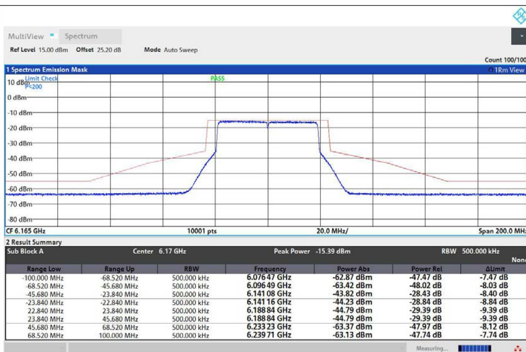
NTNV-11AX40MIMO-Ant1-6165-PASS
