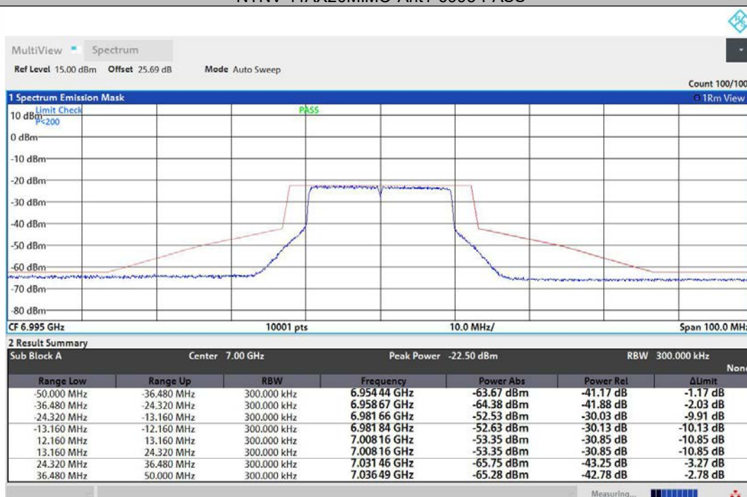
NTNV-11AX20MIMO-Ant2-6995-PASS
