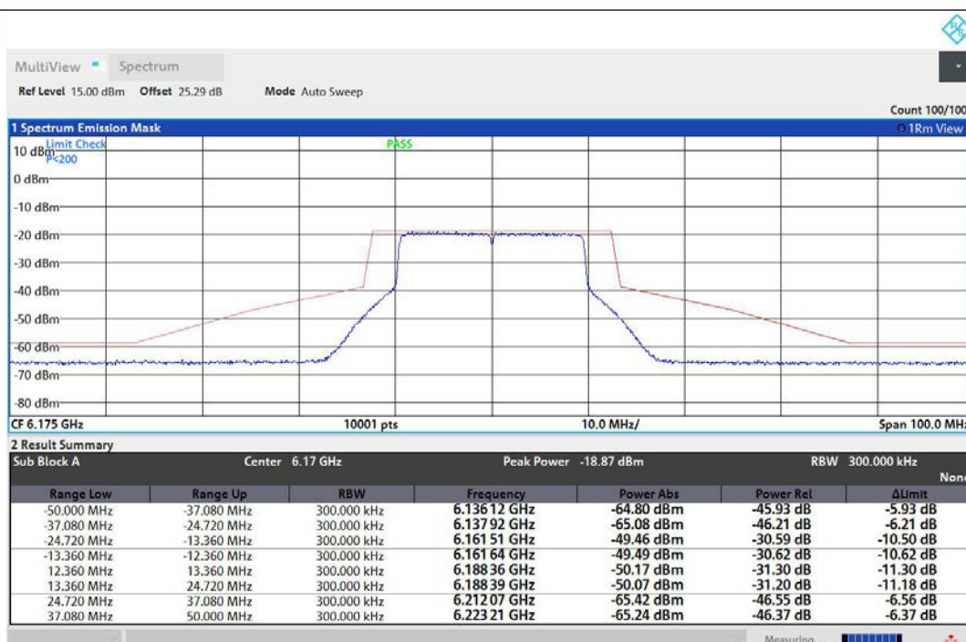
NTNV-11AX20MIMO-Ant1-6175-PASS
