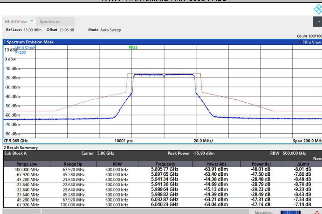
NTNV-11AX40MIMO-Ant2-5965-PASS
