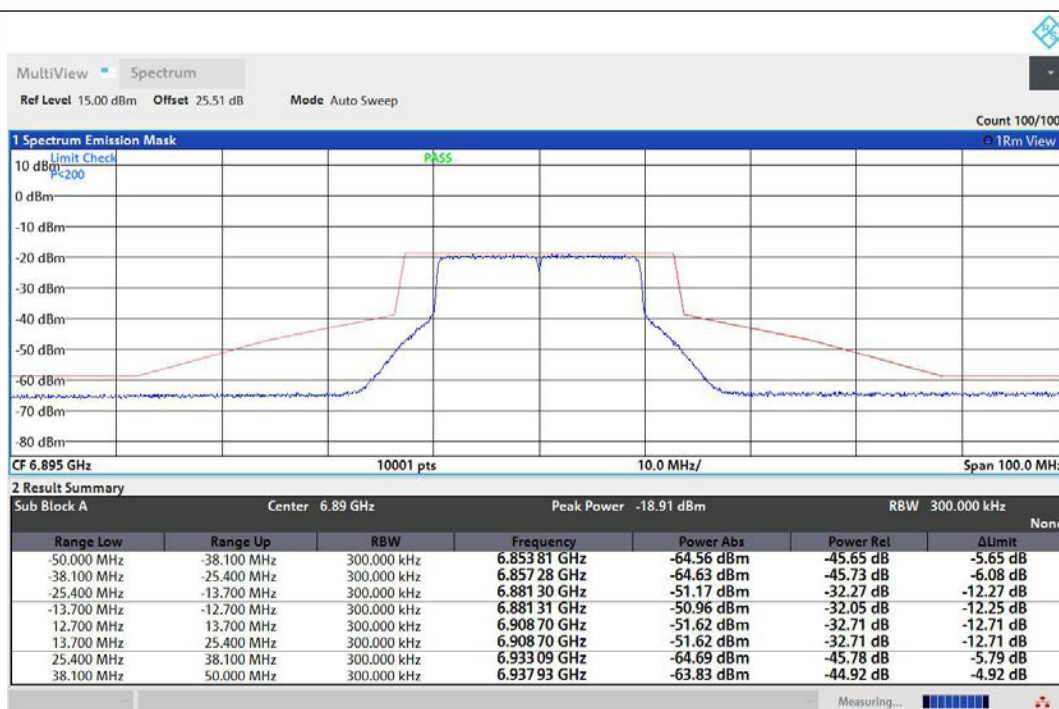
NTNV-11AX20MIMO-Ant1-6895-PASS
