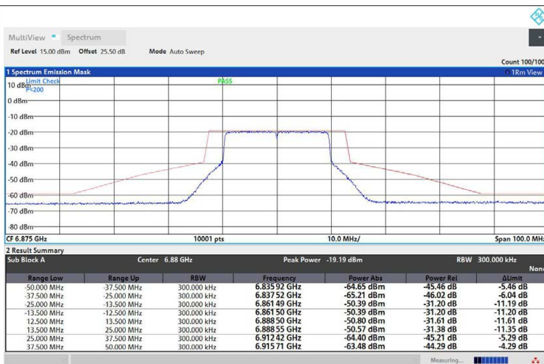
NTNV-11AX20MIMO-Ant1-6875-PASS
