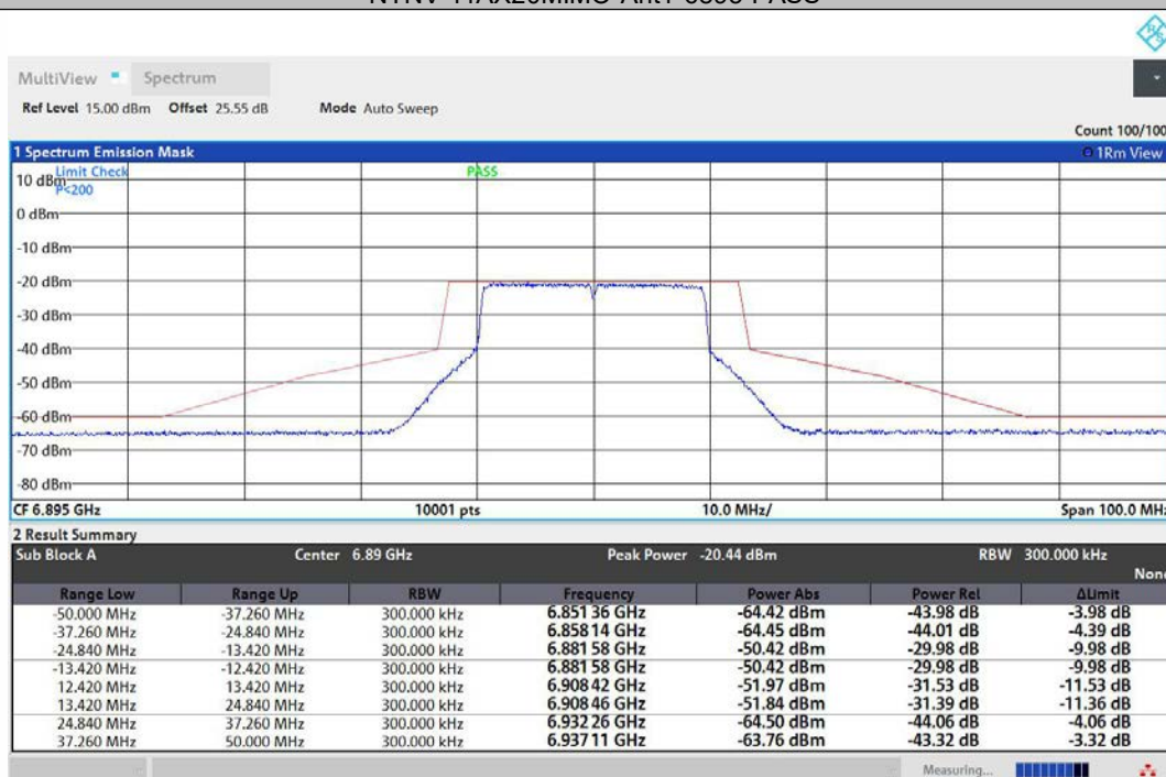
NTNV-11AX20MIMO-Ant2-6895-PASS
