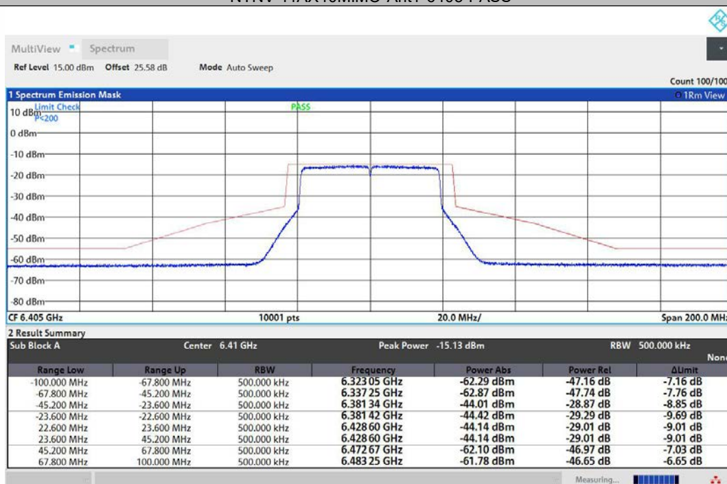
NTNV-11AX40MIMO-Ant2-6405-PASS
