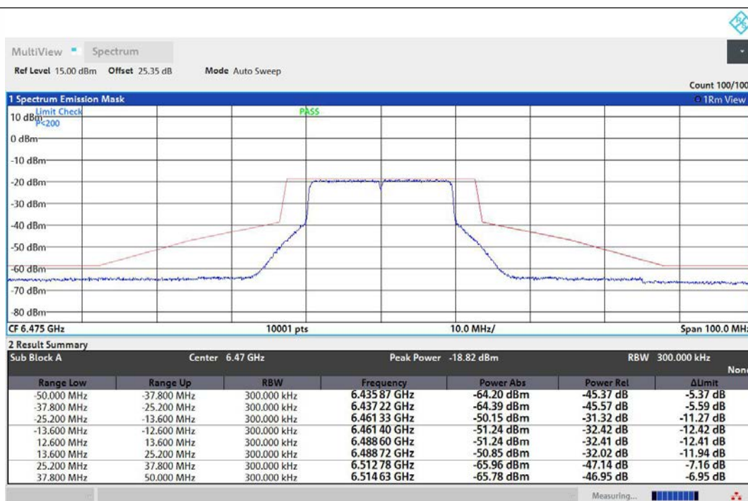
NTNV-11AX20MIMO-Ant1-6475-PASS
