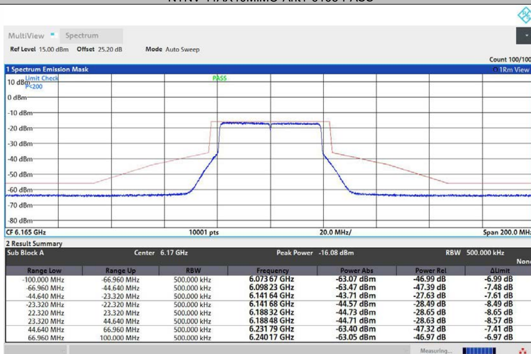
NTNV-11AX40MIMO-Ant2-6165-PASS
