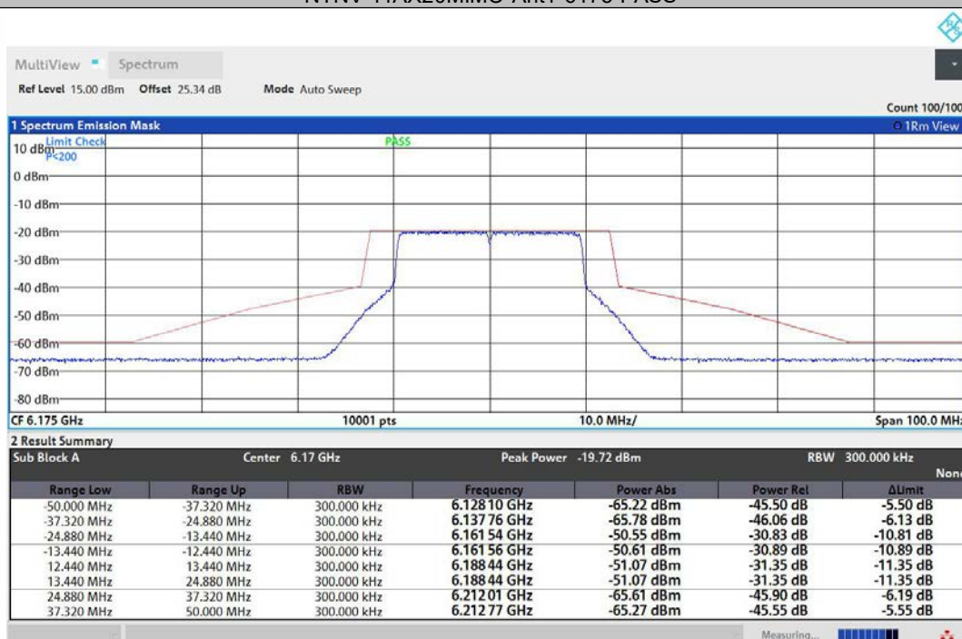
NTNV-11AX20MIMO-Ant2-6175-PASS
