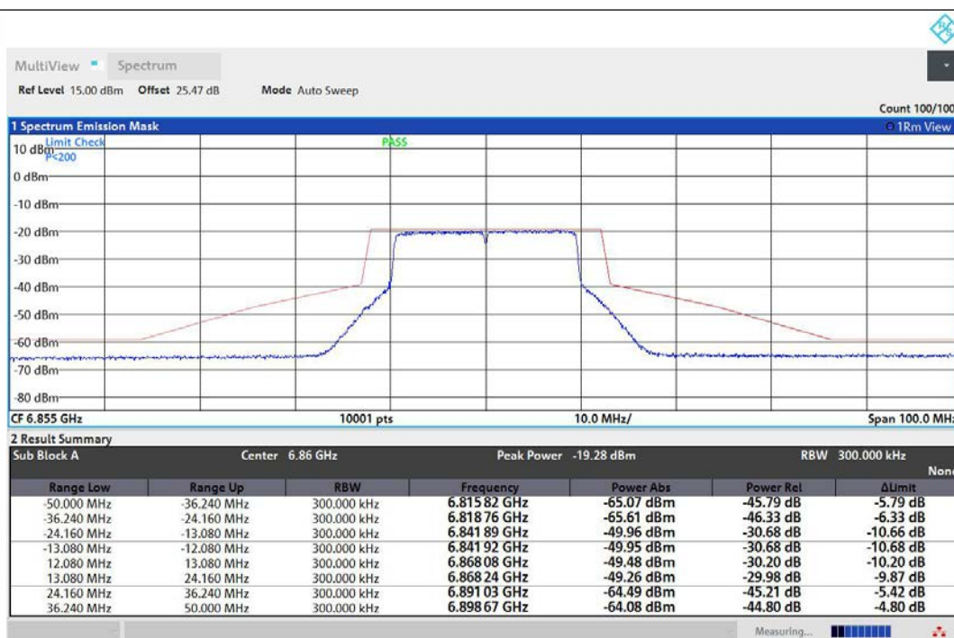
NTNV-11AX20MIMO-Ant1-6855-PASS
