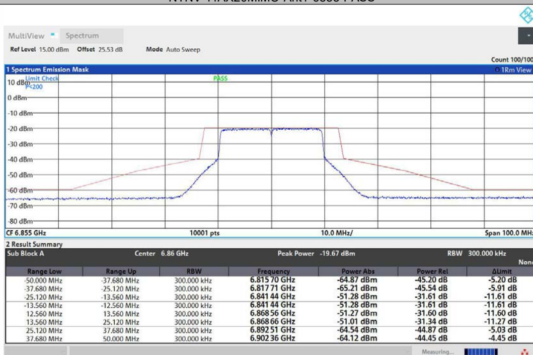
NTNV-11AX20MIMO-Ant2-6855-PASS
