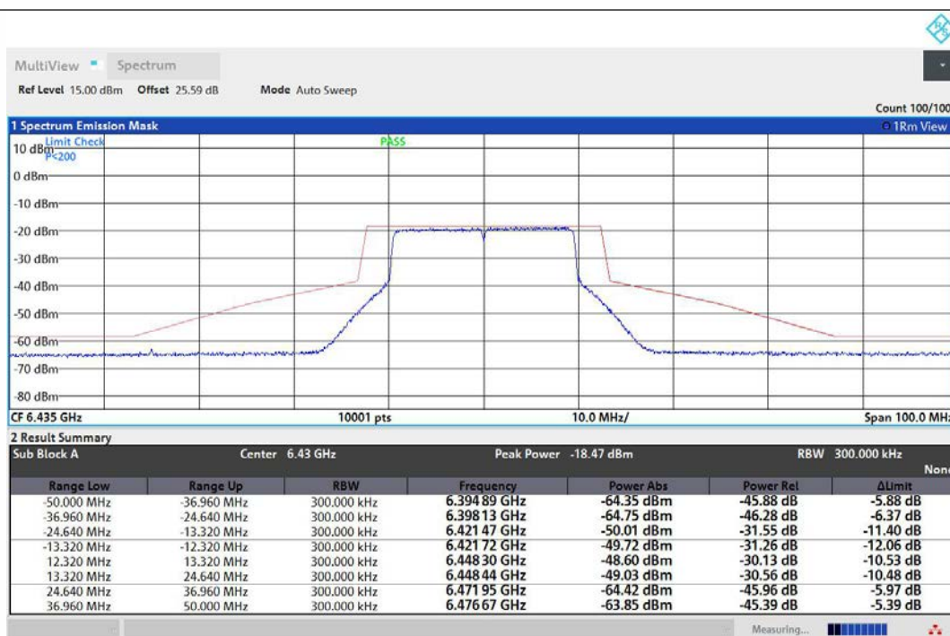
NTNV-11AX20MIMO-Ant1-6435-PASS
