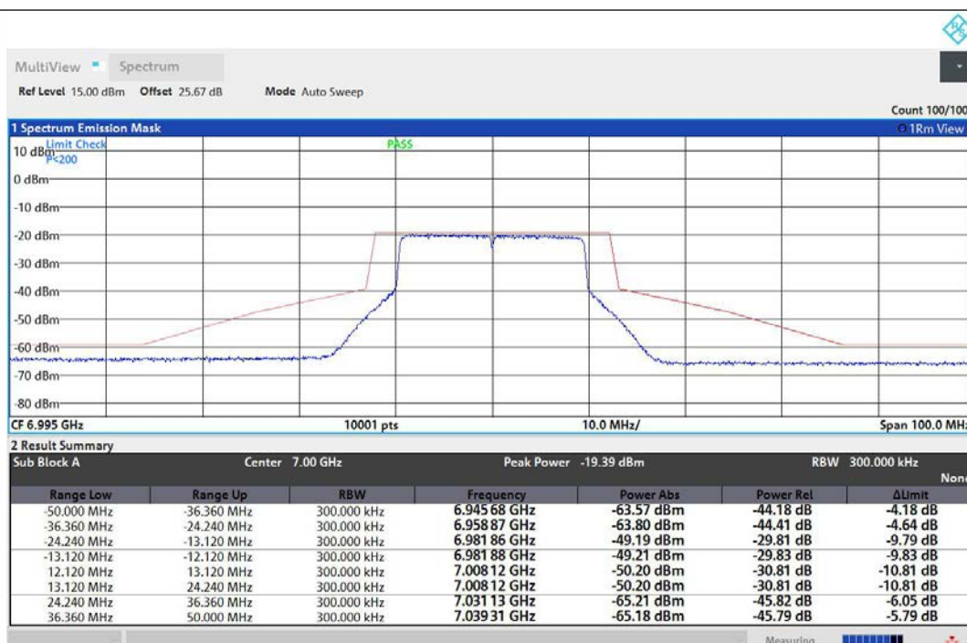
NTNV-11AX20MIMO-Ant1-6995-PASS
