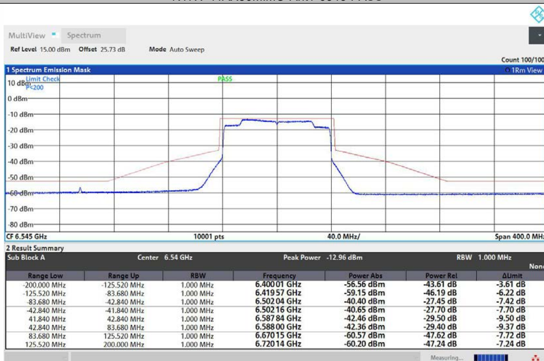
NTNV-11AX80MIMO-Ant2-6545-PASS
