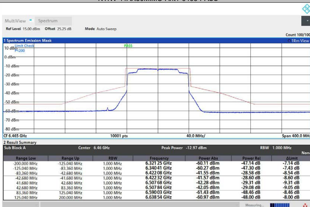
NTNV-11AX80MIMO-Ant2-6465-PASS
