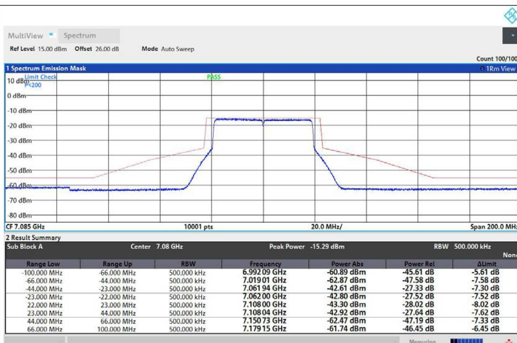
NTNV-11AX40MIMO-Ant1-7085-PASS
