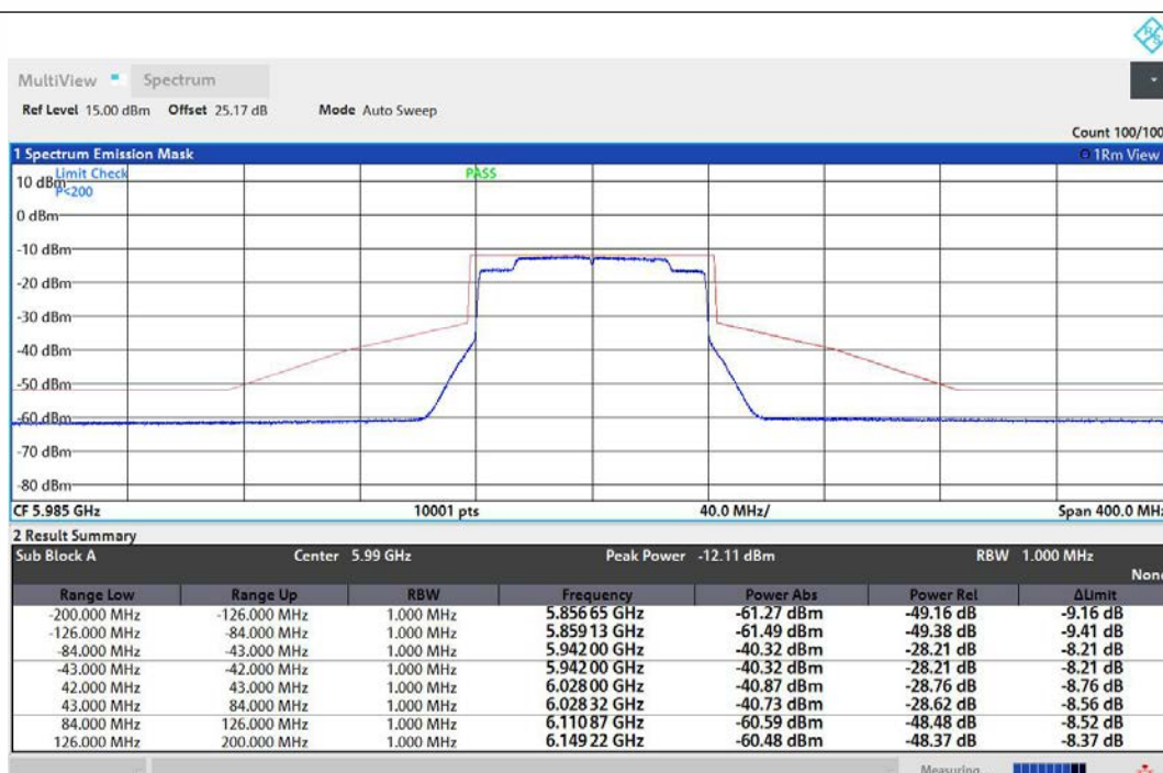
NTNV-11AX80MIMO-Ant1-5985-PASS
