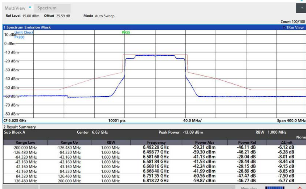
NTNV-11AX80MIMO-Ant1-6625-PASS
