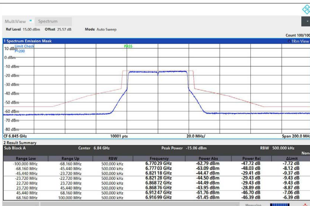
NTNV-11AX40MIMO-Ant1-6845-PASS
