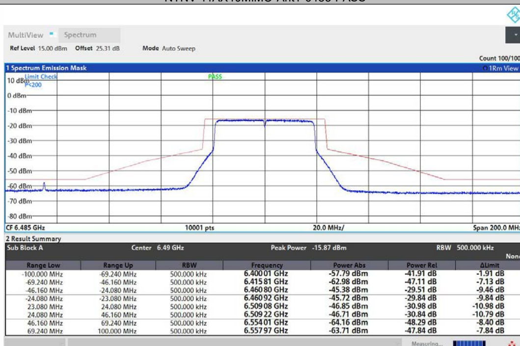
NTNV-11AX40MIMO-Ant2-6485-PASS
