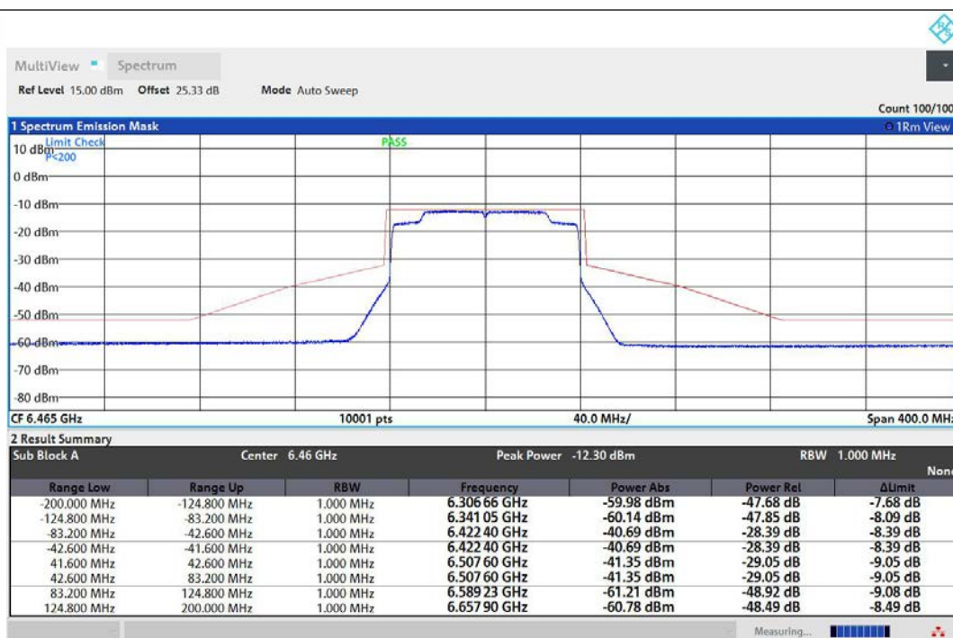
NTNV-11AX80MIMO-Ant1-6465-PASS
