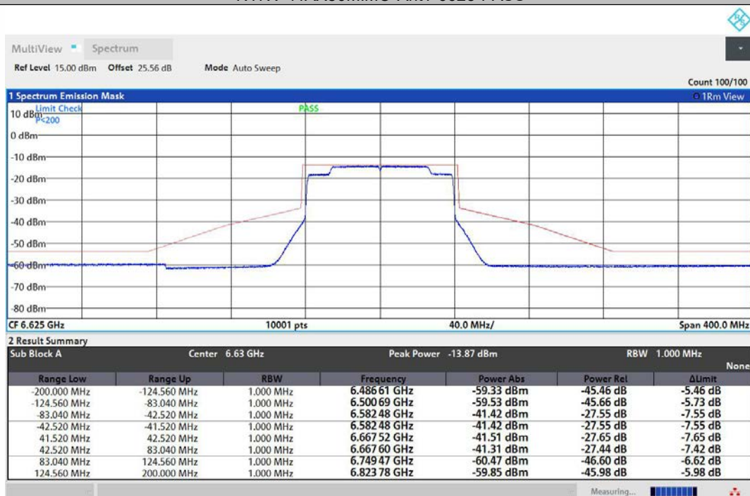
NTNV-11AX80MIMO-Ant2-6625-PASS
