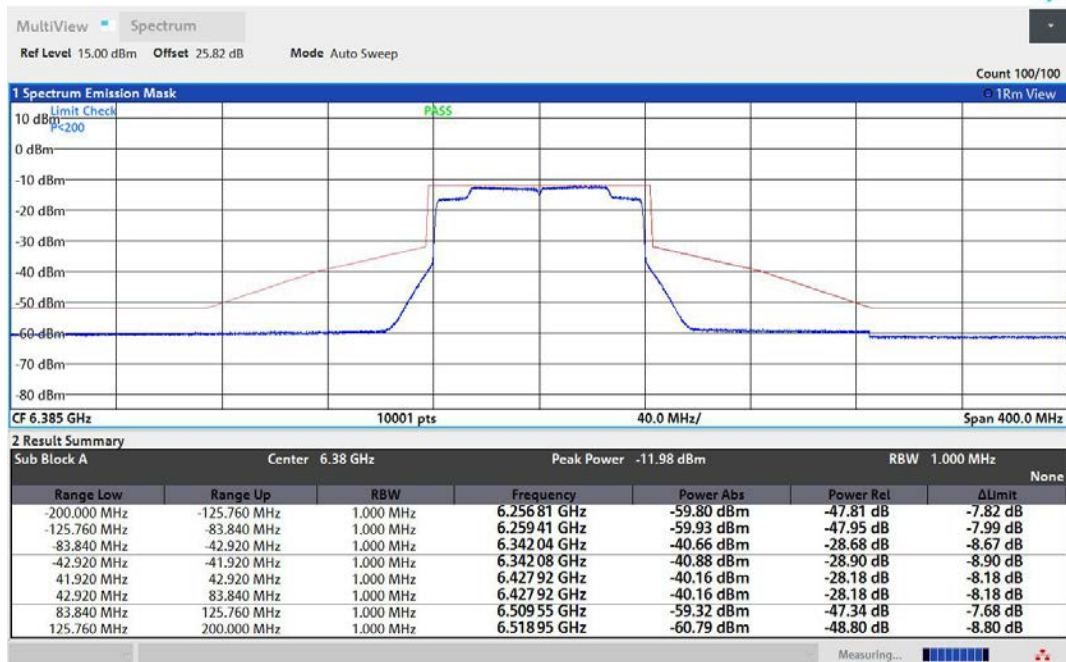
NTNV-11AX80MIMO-Ant1-6385-PASS
