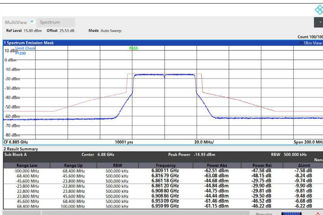
NTNV-11AX40MIMO-Ant1-6885-PASS
