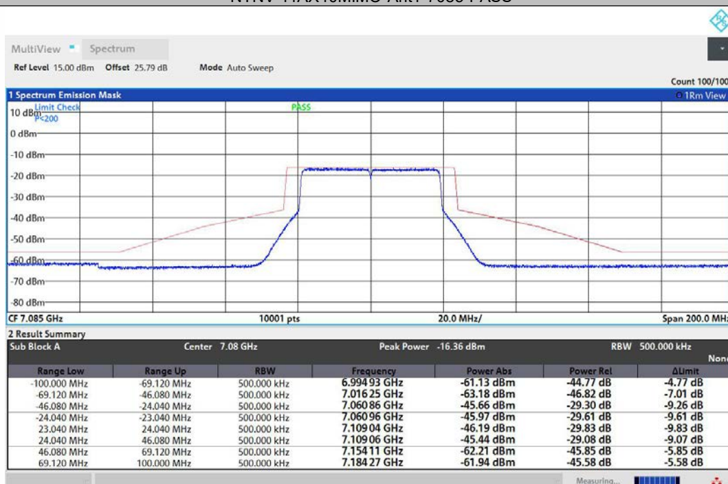
NTNV-11AX40MIMO-Ant2-7085-PASS
