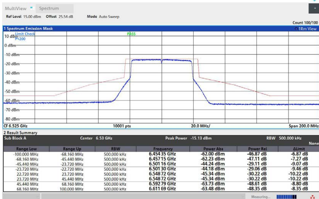
NTNV-11AX40MIMO-Ant1-6525-PASS
