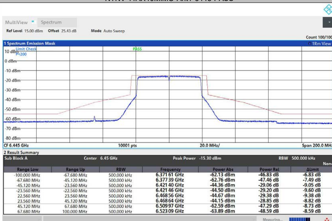
NTNV-11AX40MIMO-Ant2-6445-PASS
