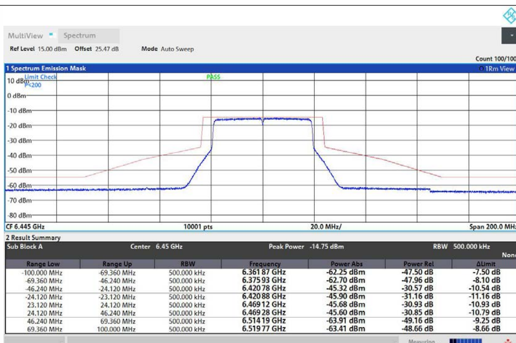
NTNV-11AX40MIMO-Ant1-6445-PASS
