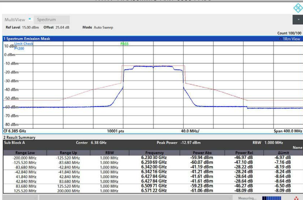
NTNV-11AX80MIMO-Ant2-6385-PASS
