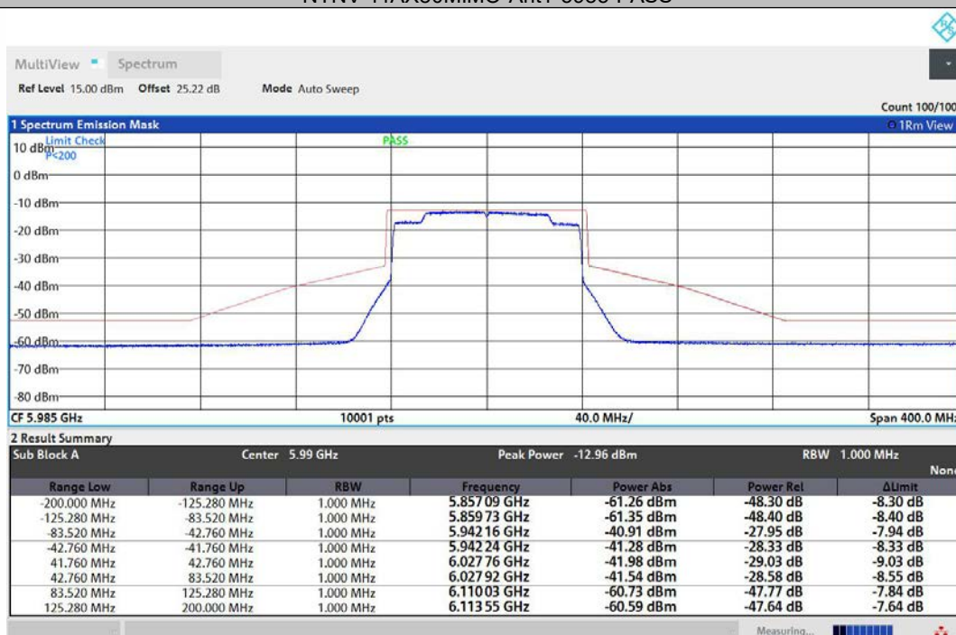
NTNV-11AX80MIMO-Ant2-5985-PASS
