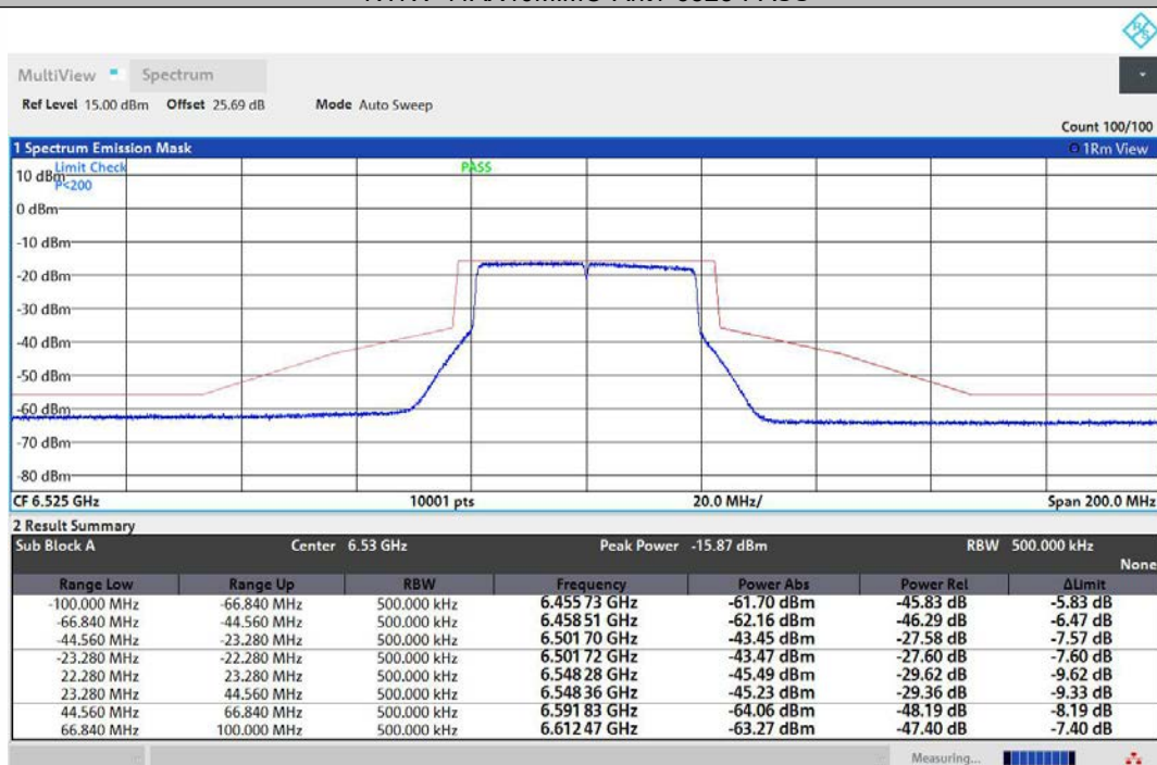
NTNV-11AX40MIMO-Ant2-6525-PASS
