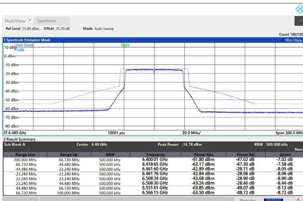
NTNV-11AX40MIMO-Ant1-6485-PASS
