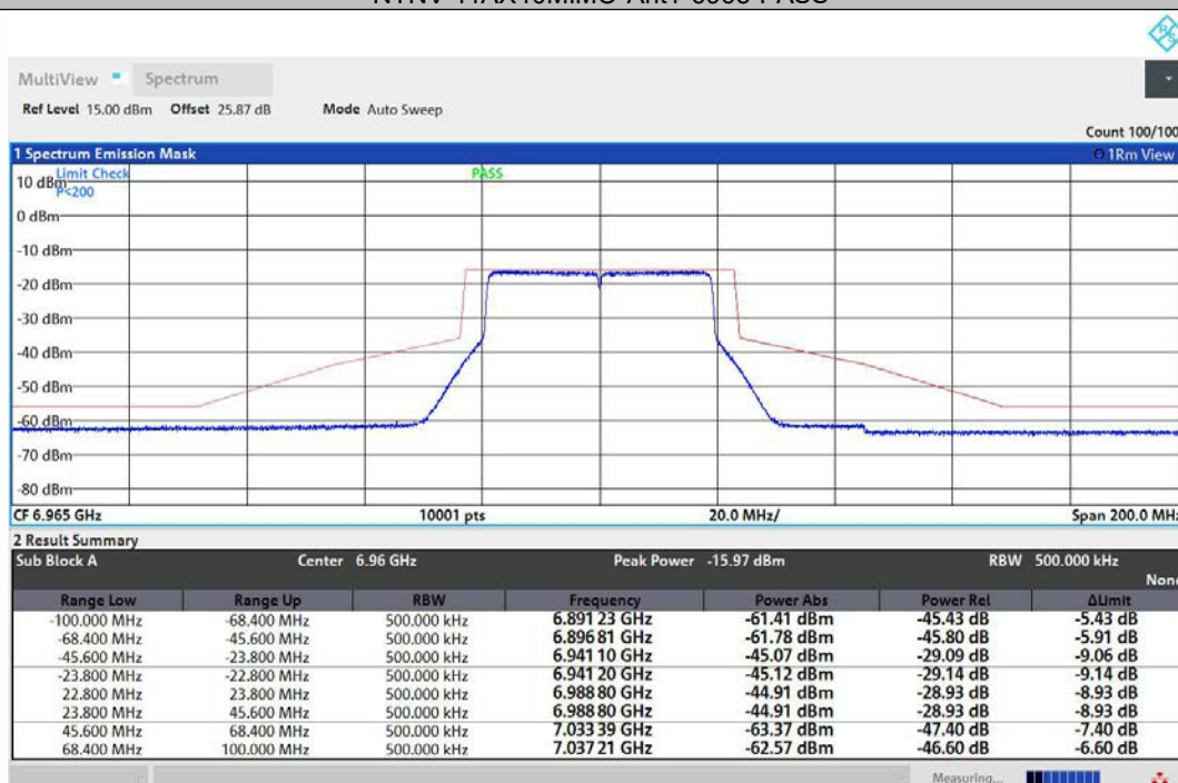
NTNV-11AX40MIMO-Ant2-6965-PASS
