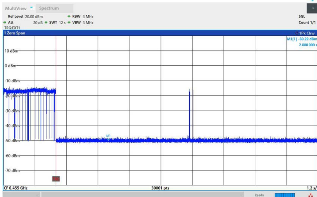
11AX20MIMO-Ant1-6455-Center-6455-Minimal
