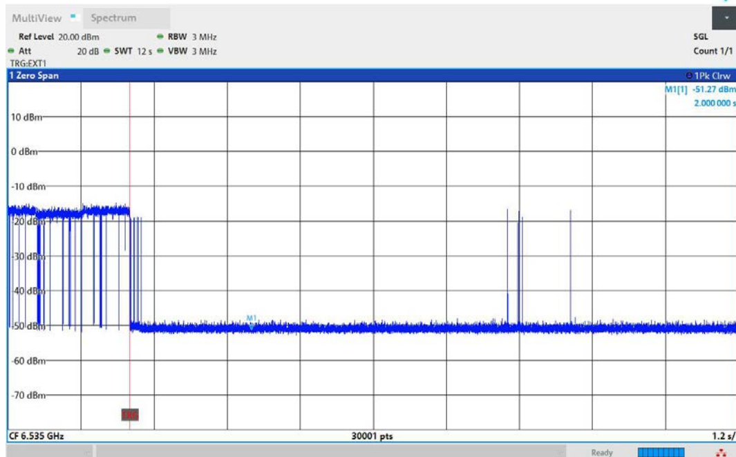
11AX20MIMO-Ant1-6535-Center-6535-Minimal
