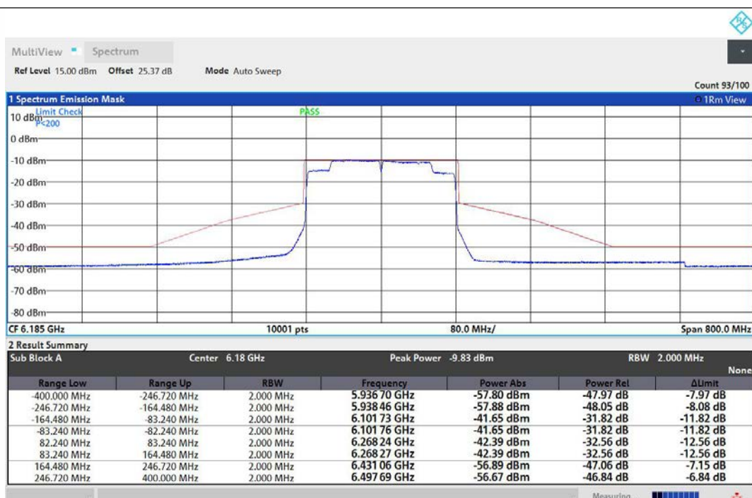
NTNV-11AX160MIMO-Ant1-6185-PASS
