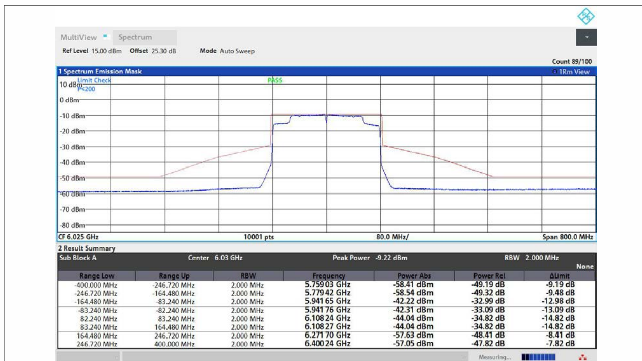
NTNV-11AX160MIMO-Ant1-6025-PASS
