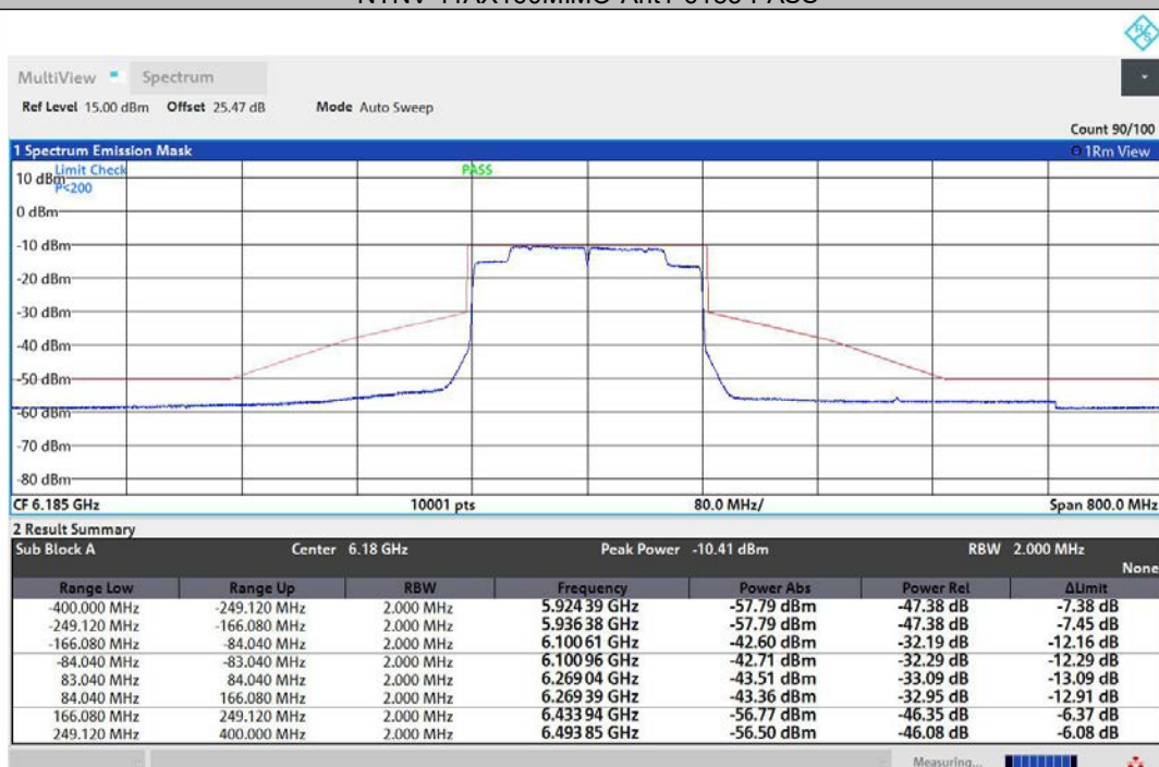
NTNV-11AX160MIMO-Ant2-6185-PASS
