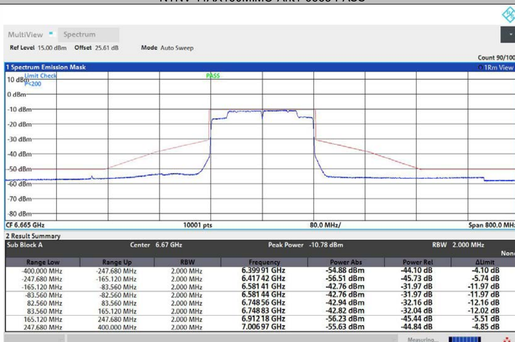
NTNV-11AX160MIMO-Ant2-6665-PASS
