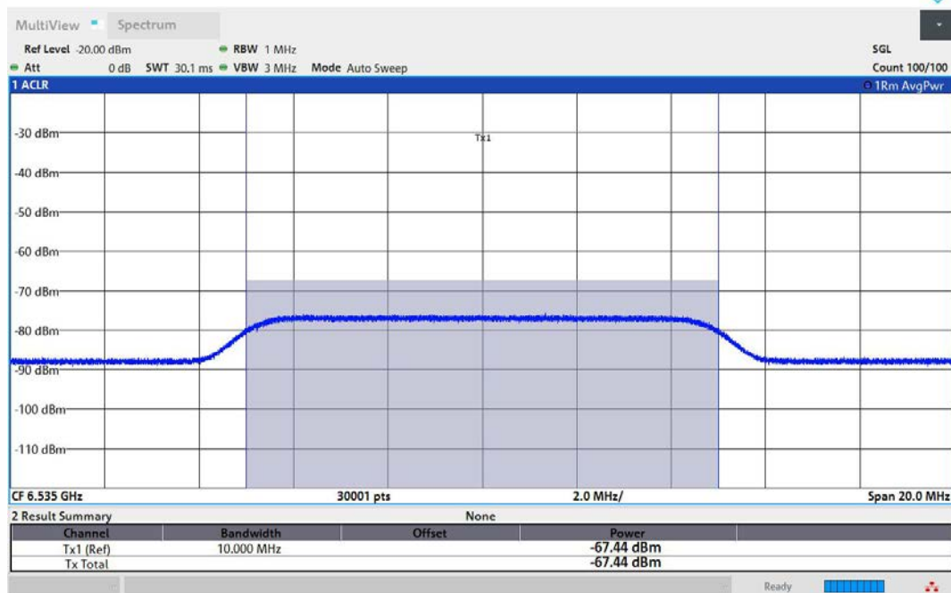
11AX20MIMO-Ant1-6535-Center-6535-Minimal
