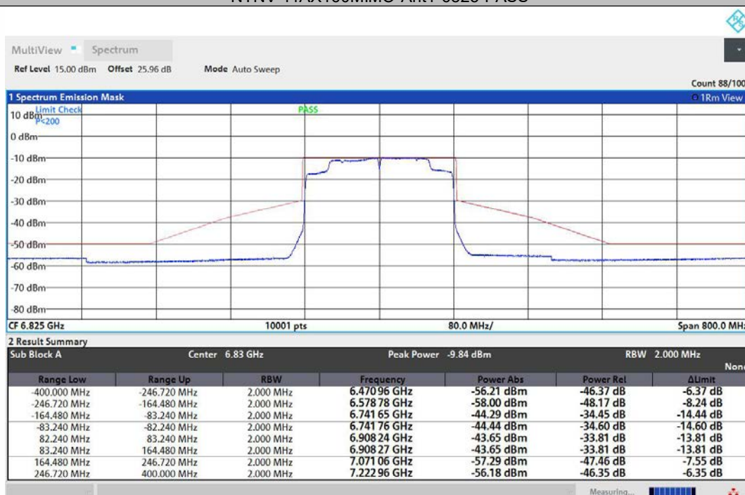
NTNV-11AX160MIMO-Ant2-6825-PASS
