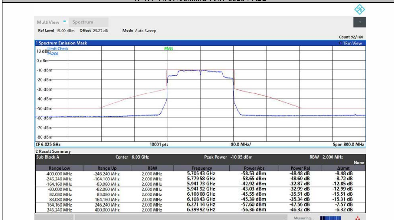
NTNV-11AX160MIMO-Ant2-6025-PASS
