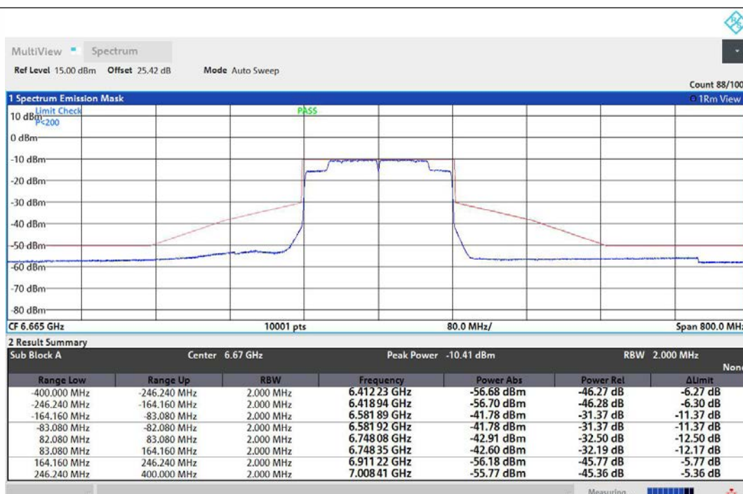
NTNV-11AX160MIMO-Ant1-6665-PASS
