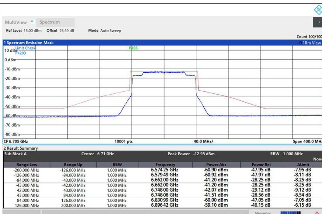
NTNV-11AX80MIMO-Ant1-6705-PASS
