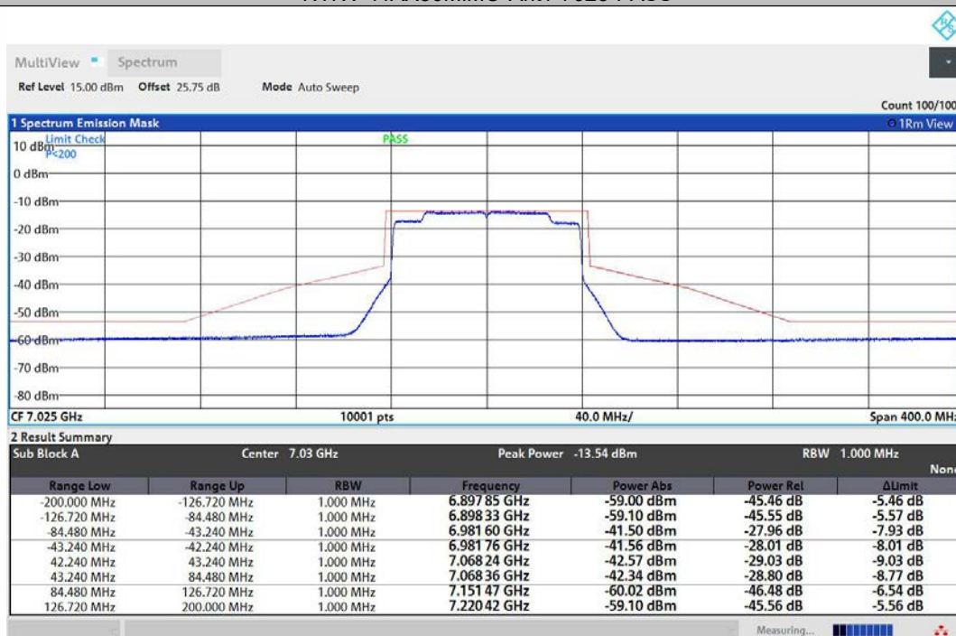
NTNV-11AX80MIMO-Ant2-7025-PASS
