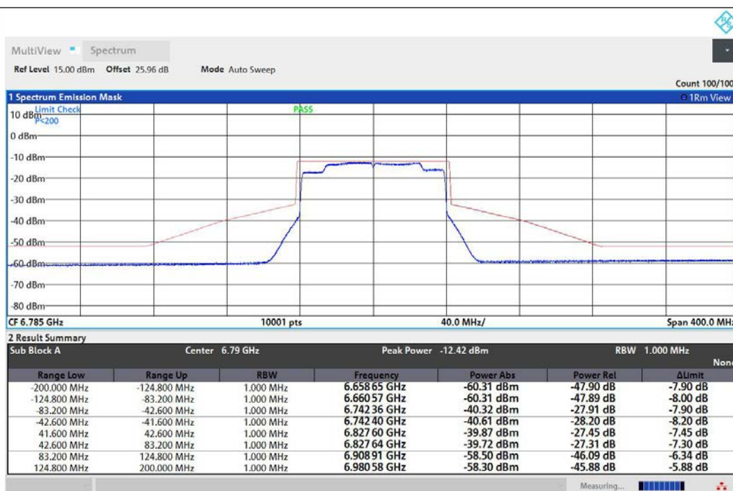
NTNV-11AX80MIMO-Ant1-6785-PASS
