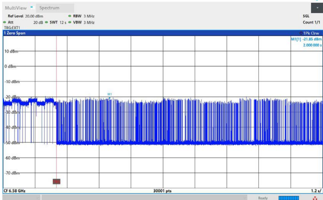
11AX160MIMO-Ant1-6505-High-6580-Minimal
