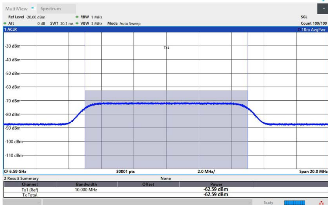
11AX160MIMO-Ant1-6665-Low-6590-Minimal
