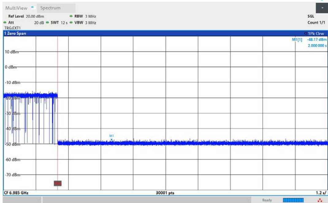
11AX160MIMO-Ant1-6985-Center-6985-OFF-PASS
