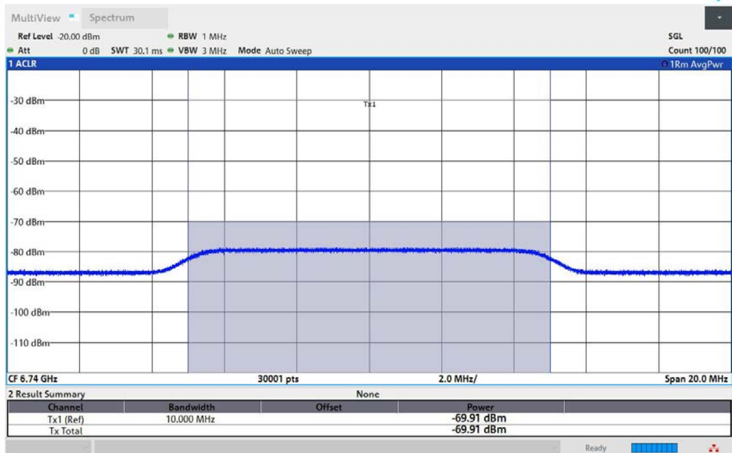
11AX160MIMO-Ant1-6665-High-6740-OFF-PASS
