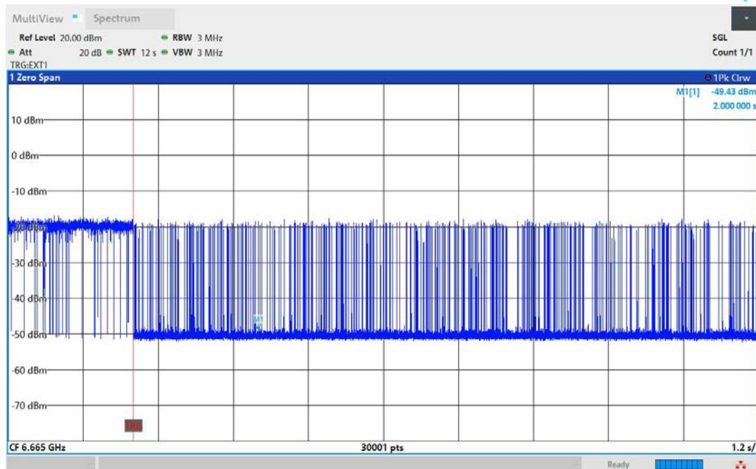
11AX160MIMO-Ant1-6665-Center-6665-Minimal
