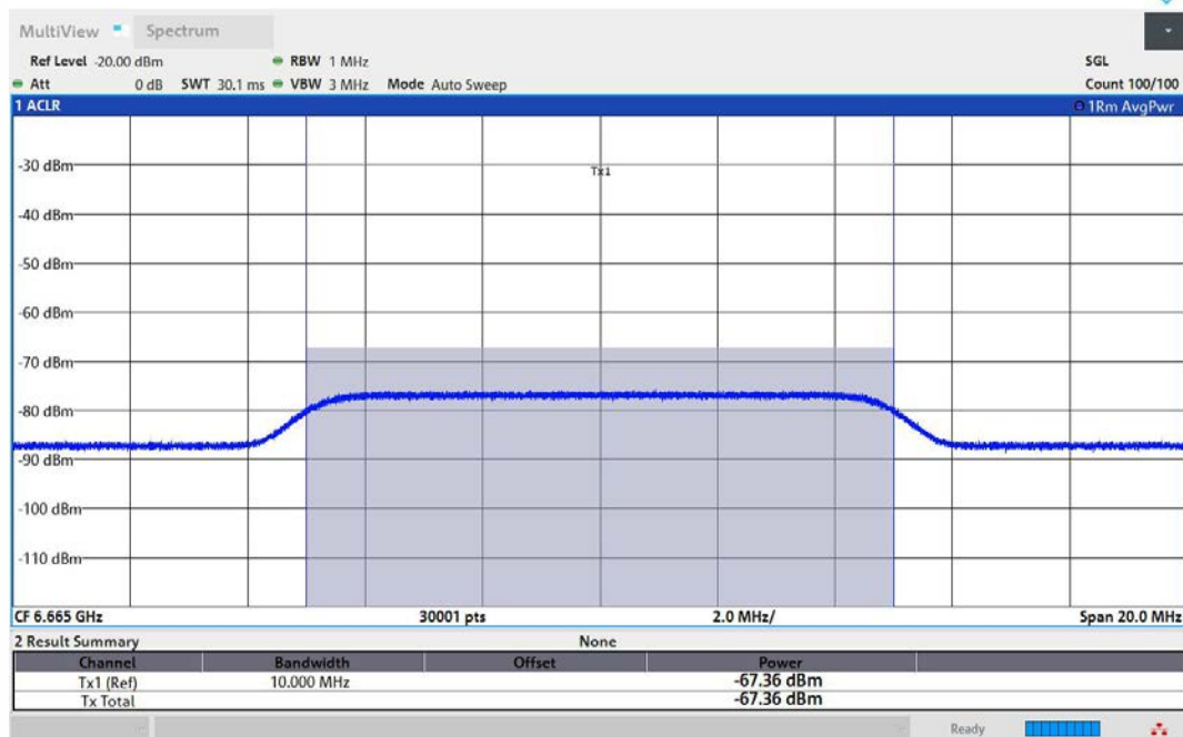
11AX160MIMO-Ant1-6665-Center-6665-Minimal
