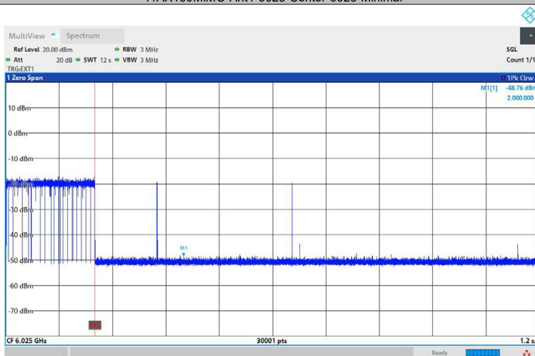
11AX160MIMO-Ant1-6025-Center-6025-Minimal
