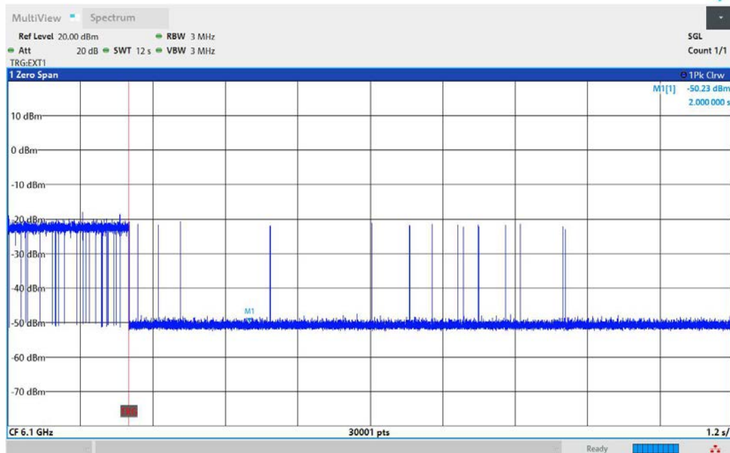
11AX160MIMO-Ant1-6025-High-6100-Minimal
