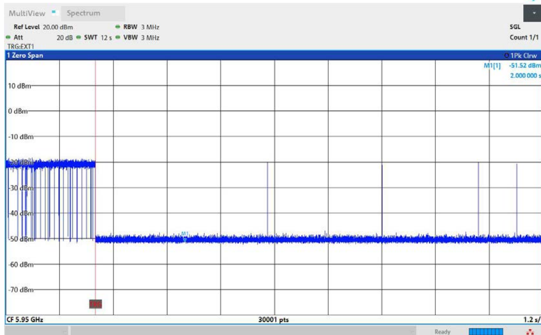
11AX160MIMO-Ant1-6025-Low-5950-Minimal
