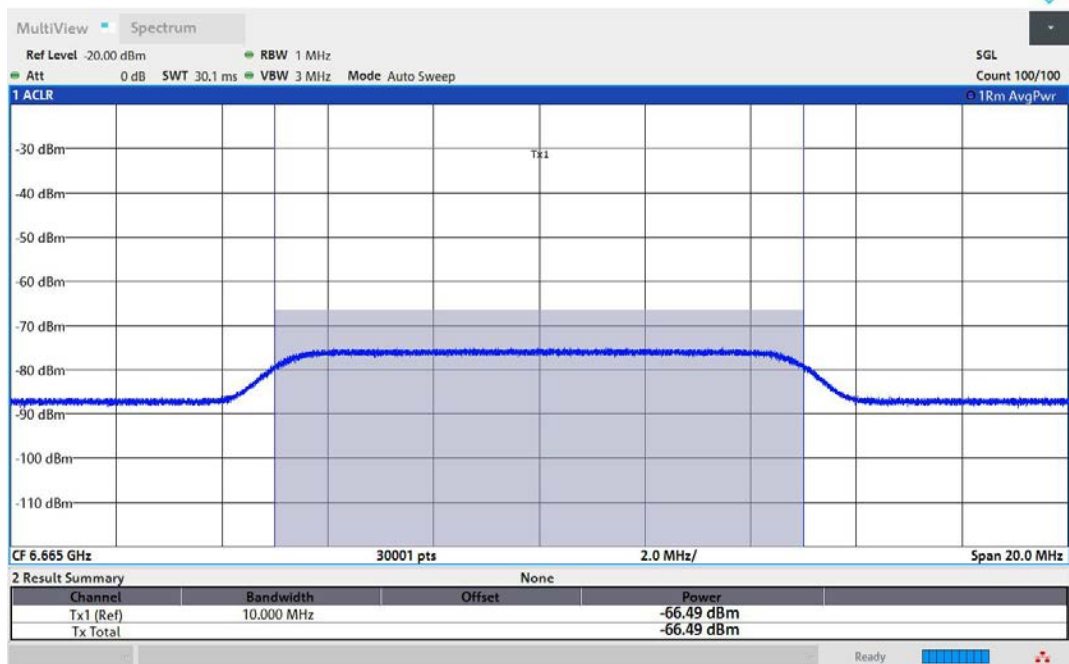
11AX160MIMO-Ant1-6665-Center-6665-OFF-PASS
