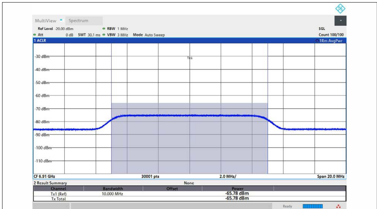
11AX160MIMO-Ant1-6985-Low-6910-Minimal
