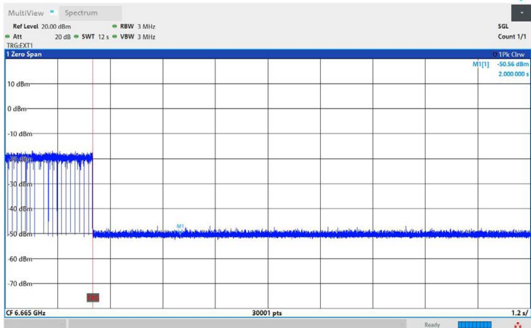
11AX160MIMO-Ant1-6665-Center-6665-OFF-PASS
