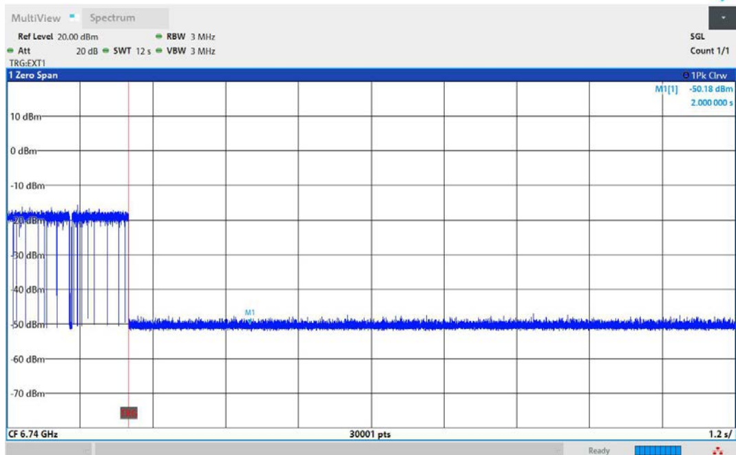
11AX160MIMO-Ant1-6665-High-6740-OFF-PASS
