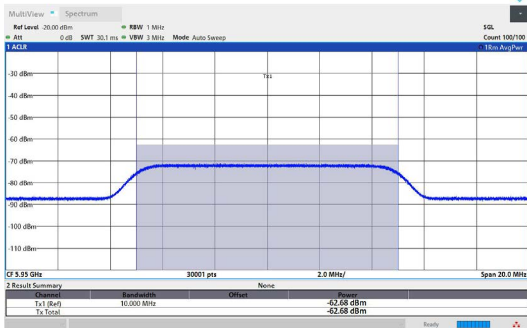
11AX160MIMO-Ant1-6025-Low-5950-Minimal
