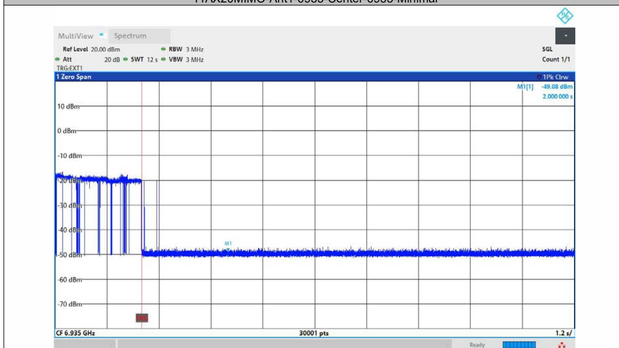
11AX20MIMO-Ant1-6935-Center-6935-Minimal
