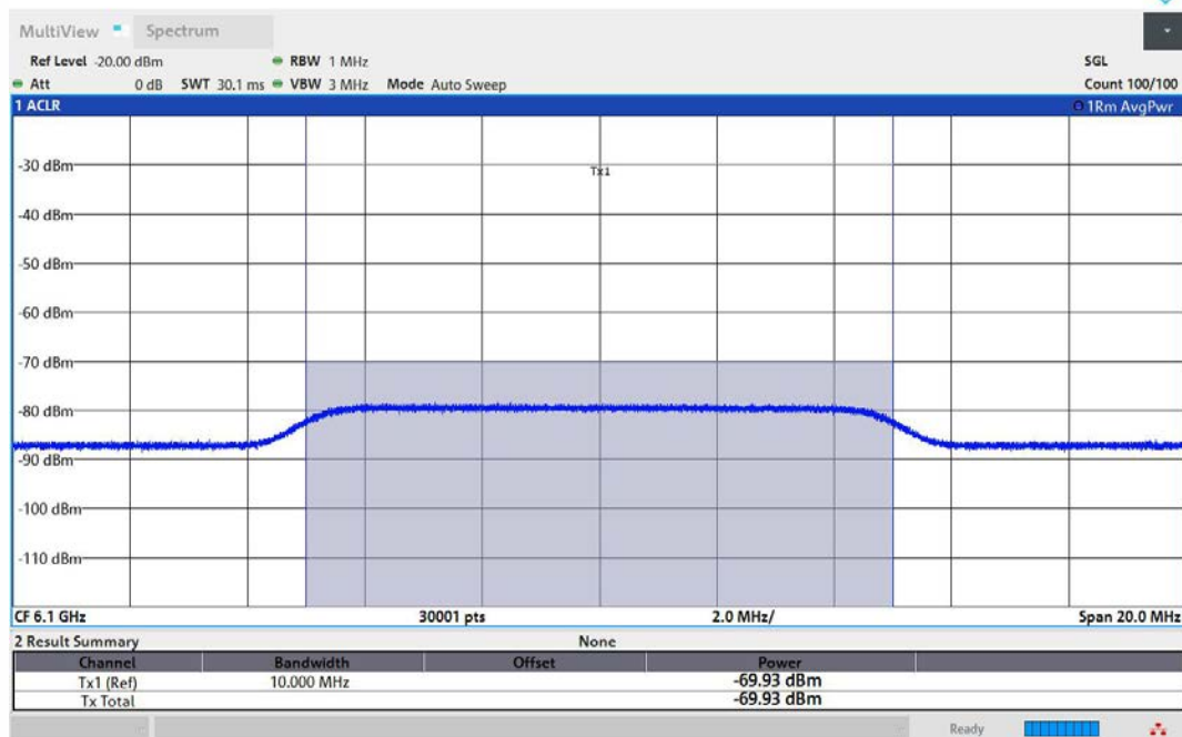
11AX160MIMO-Ant1-6025-High-6100-Minimal
