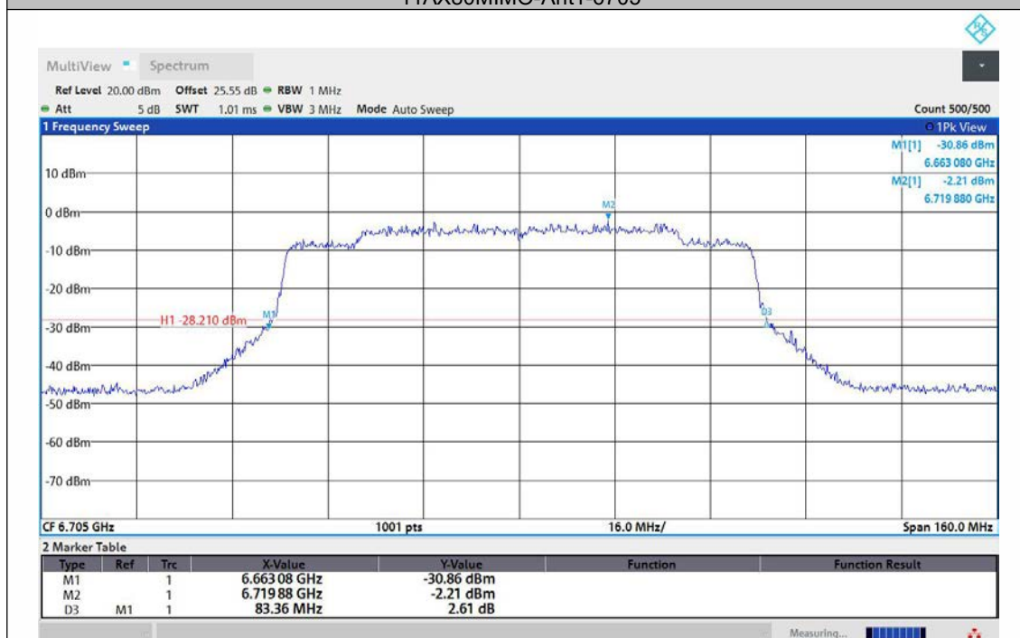
11AX80MIMO-Ant2-6705
