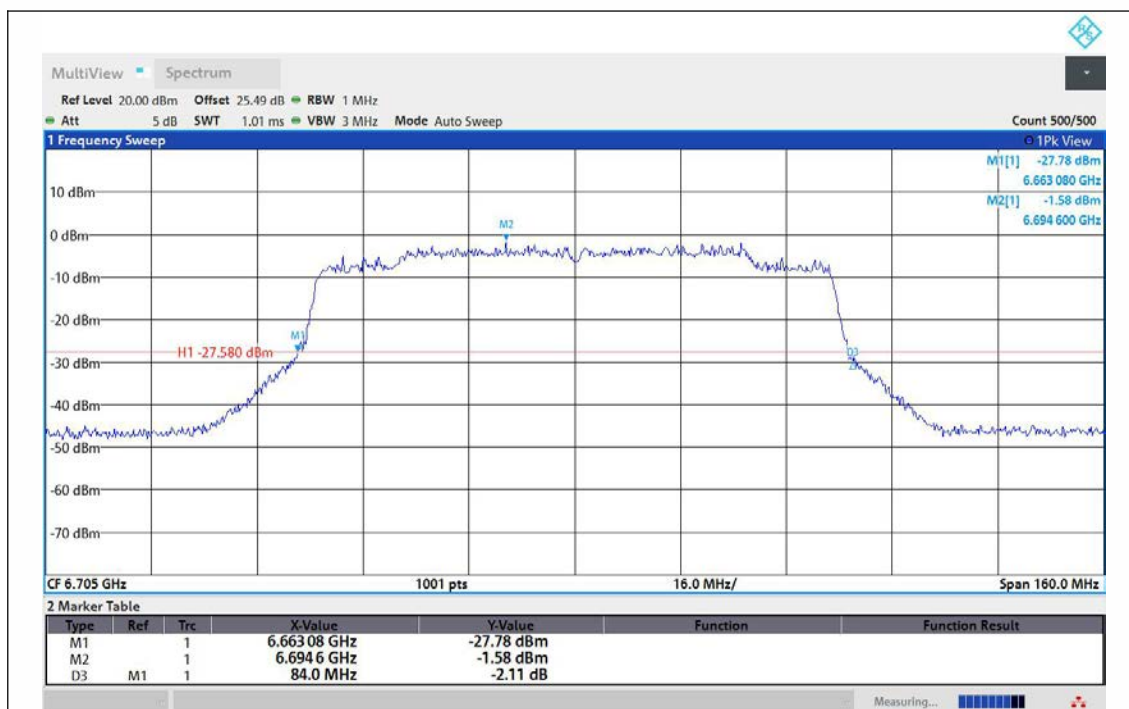
11AX80MIMO-Ant1-6705
