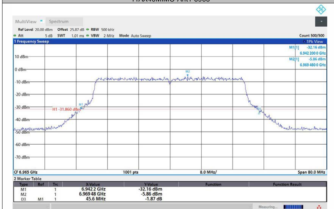
11AX40MIMO-Ant2-6965
