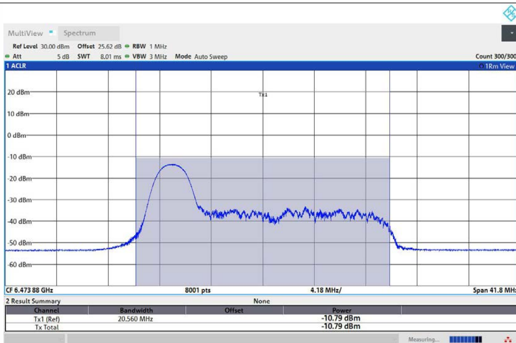
11AX20MIMO-Ant1-6475-26Tone-RU0-PASS
