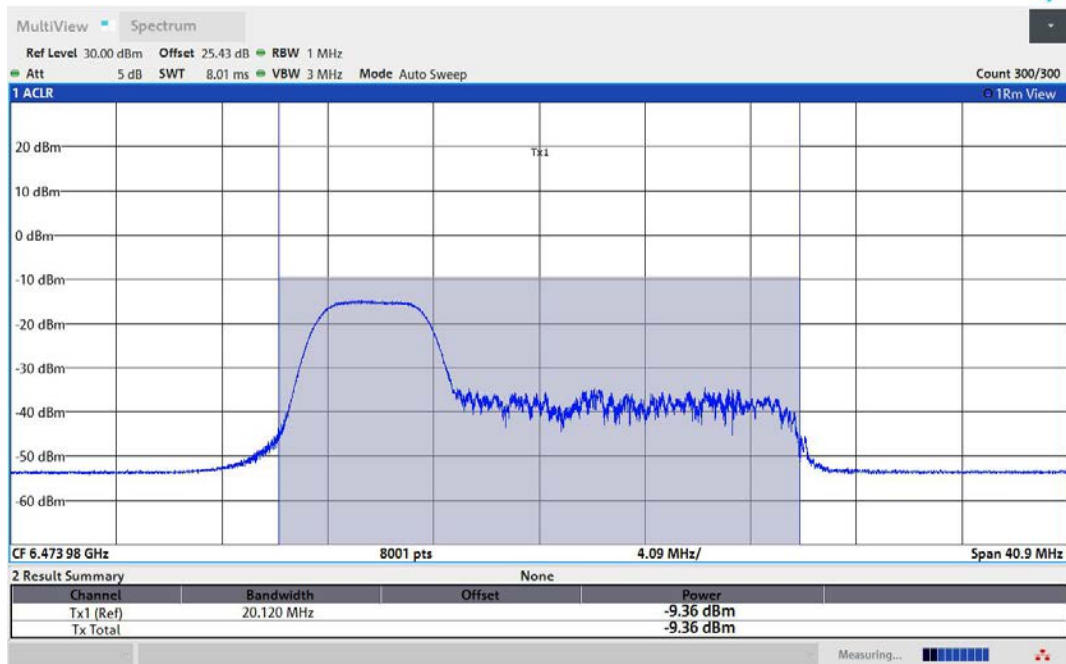
11AX20MIMO-Ant2-6475-52Tone-RU37-PASS
