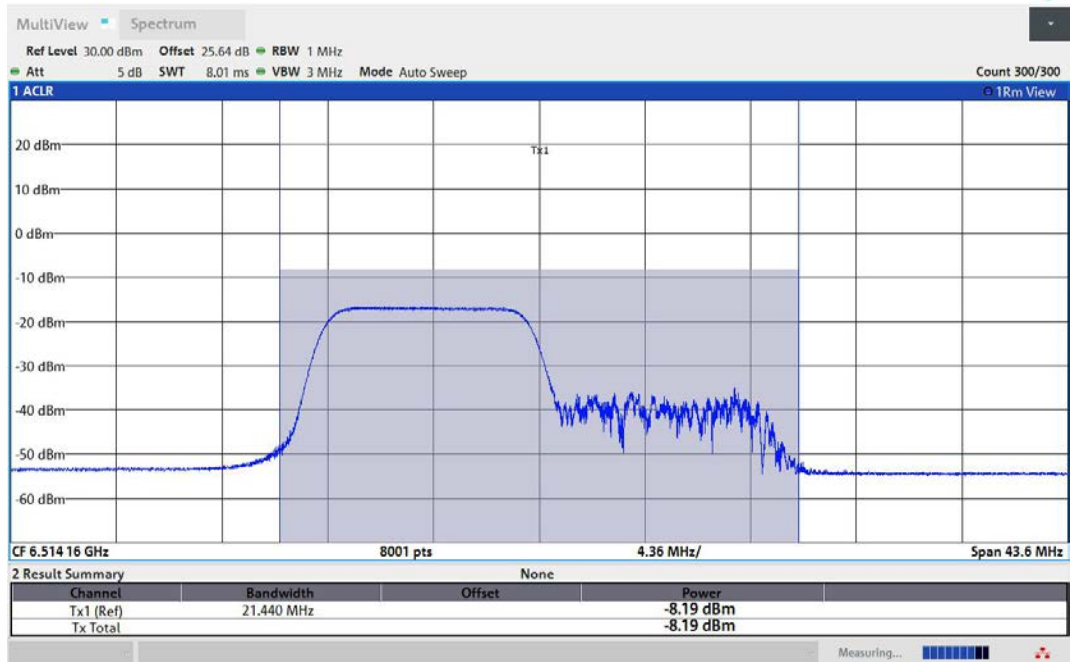
11AX20MIMO-Ant2-6515-106Tone-RU53-PASS
