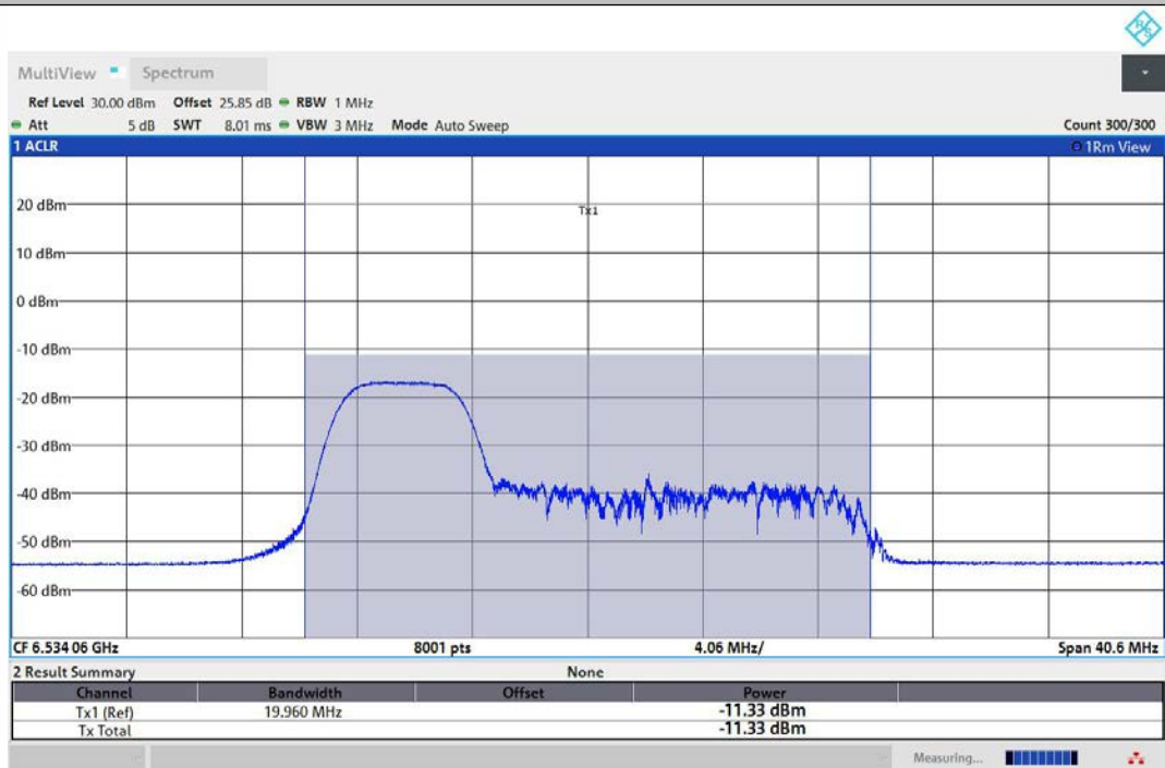
11AX20MIMO-Ant2-6535-52Tone-RU37-PASS
