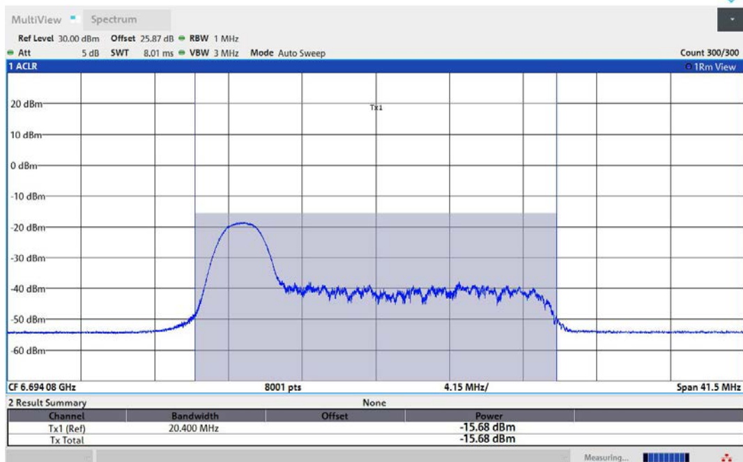
11AX20MIMO-Ant2-6695-26Tone-RU0-PASS
