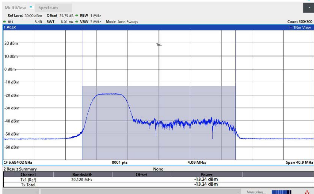
11AX20MIMO-Ant2-6695-52Tone-RU37-PASS
