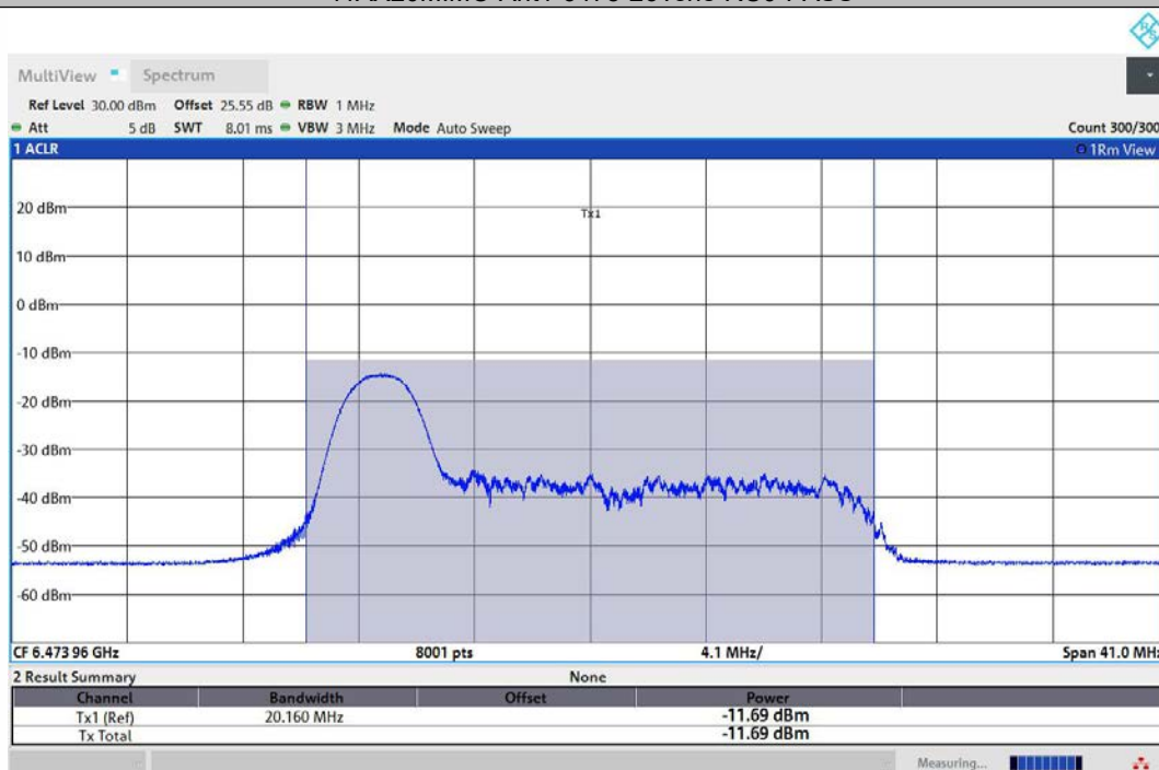
11AX20MIMO-Ant2-6475-26Tone-RU0-PASS
