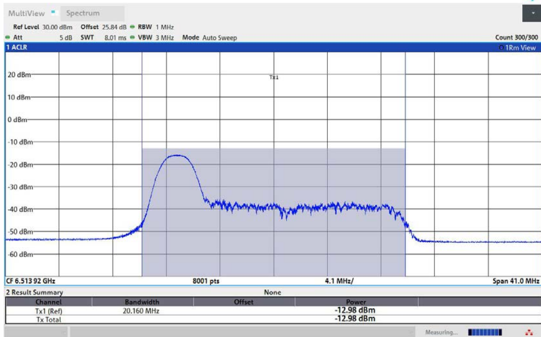
11AX20MIMO-Ant2-6515-26Tone-RU0-PASS
