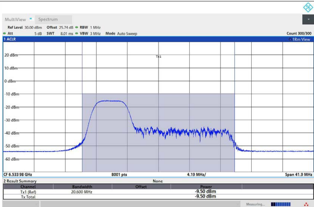
11AX20MIMO-Ant1-6535-52Tone-RU37-PASS
