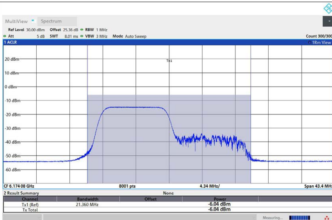
11AX20MIMO-Ant1-6175-106Tone-RU53-PASS
