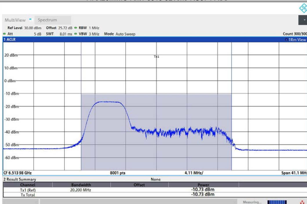
11AX20MIMO-Ant2-6515-52Tone-RU37-PASS
