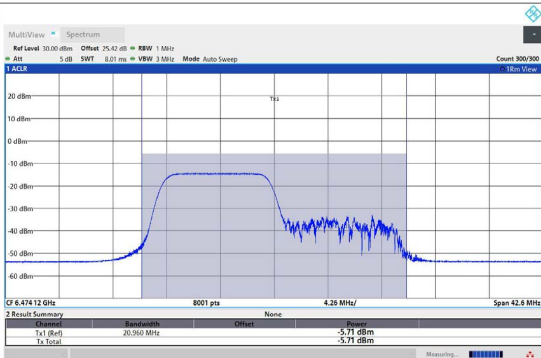
11AX20MIMO-Ant1-6475-106Tone-RU53-PASS
