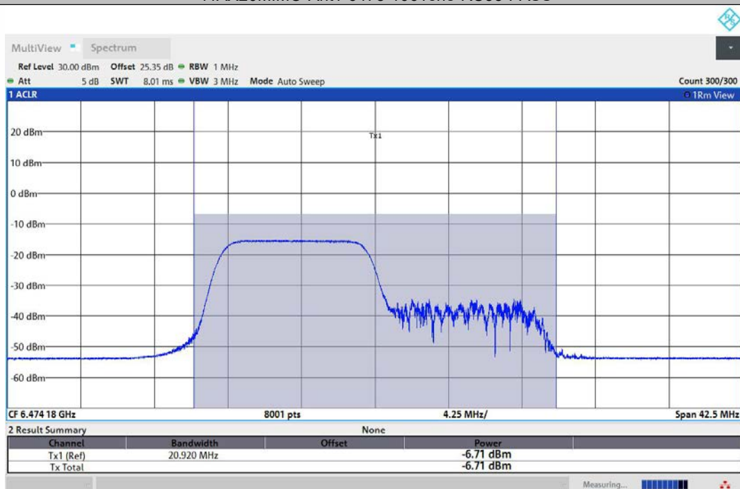
11AX20MIMO-Ant2-6475-106Tone-RU53-PASS
