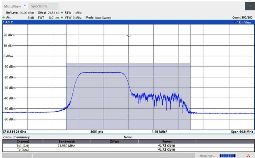
11AX20MIMO-Ant1-6515-106Tone-RU53-PASS
