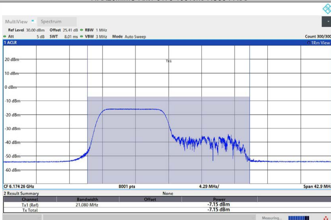
11AX20MIMO-Ant2-6175-106Tone-RU53-PASS
