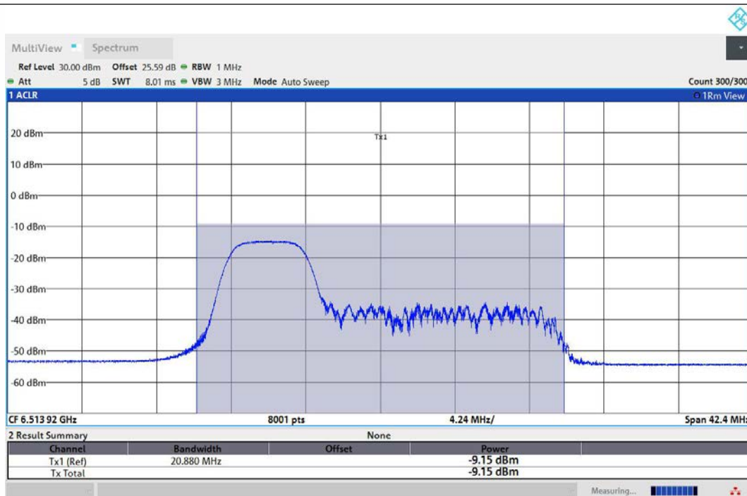
11AX20MIMO-Ant1-6515-52Tone-RU37-PASS
