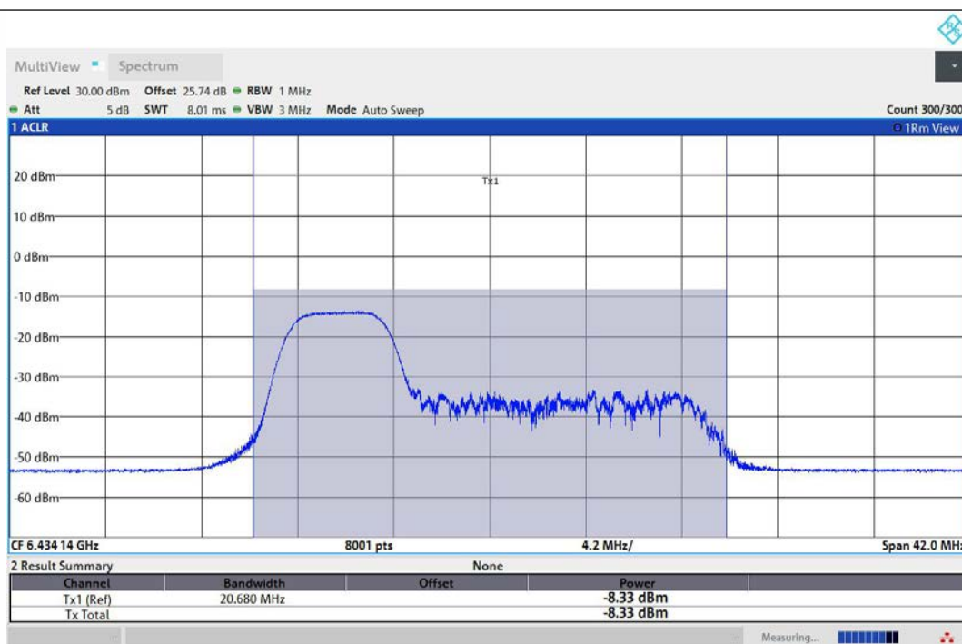
11AX20MIMO-Ant1-6435-52Tone-RU37-PASS
