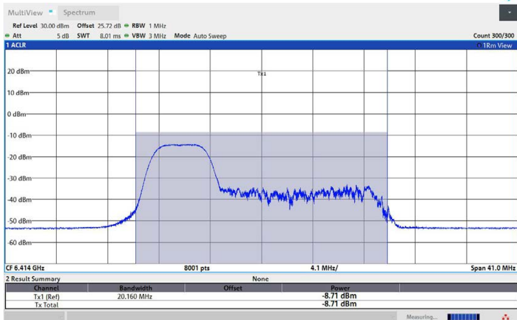
11AX20MIMO-Ant2-6415-52Tone-RU37-PASS
