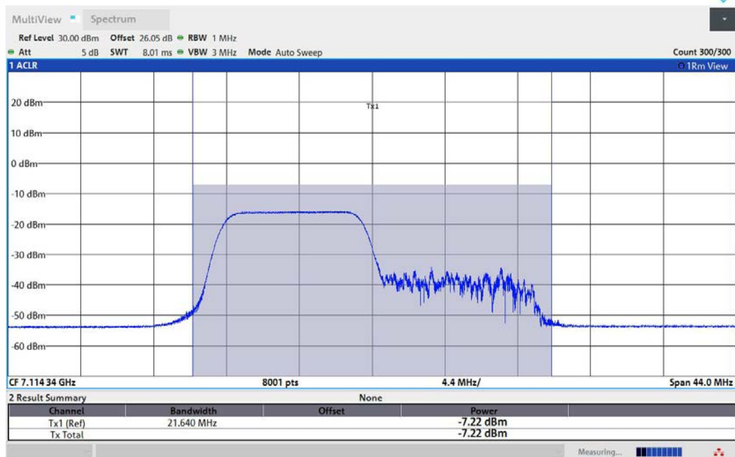
11AX20MIMO-Ant1-7115-106Tone-RU53-PASS
