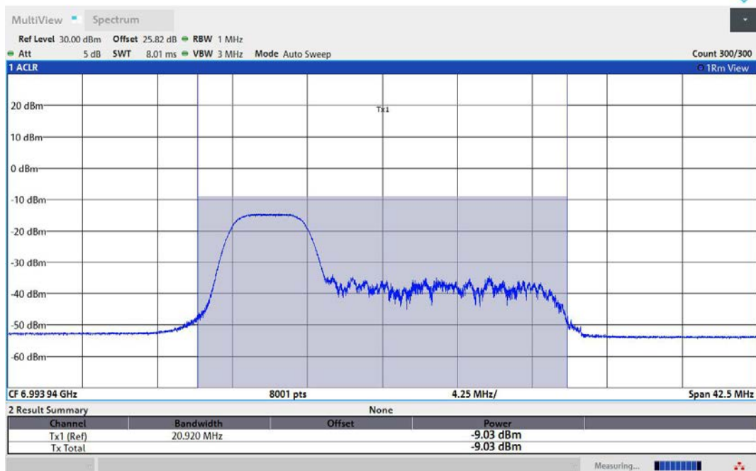
11AX20MIMO-Ant1-6995-52Tone-RU37-PASS
