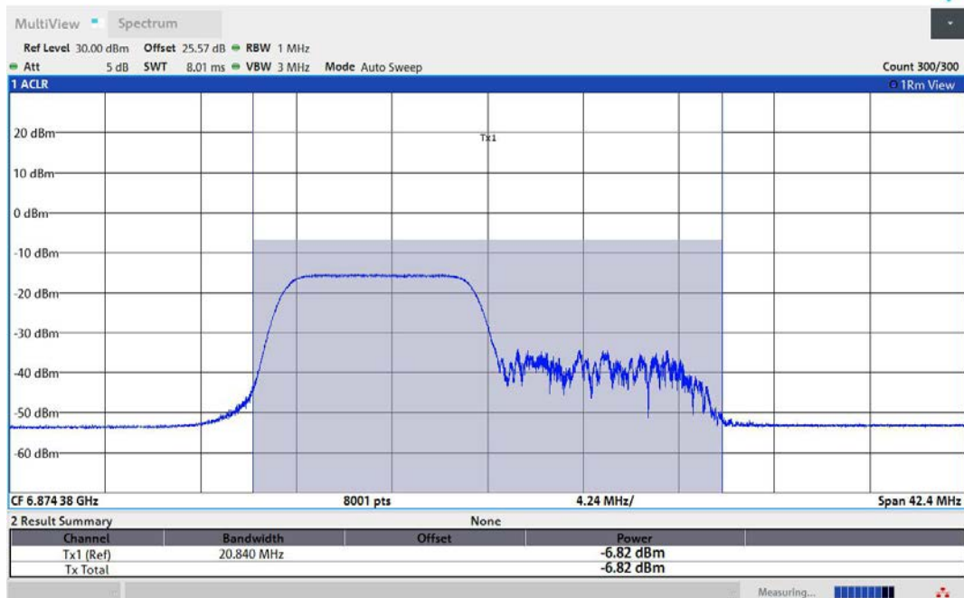
11AX20MIMO-Ant2-6875-106Tone-RU53-PASS
