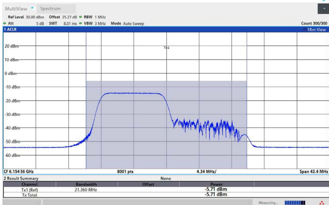
11AX40MIMO-Ant1-6165-106Tone-RU53-PASS
