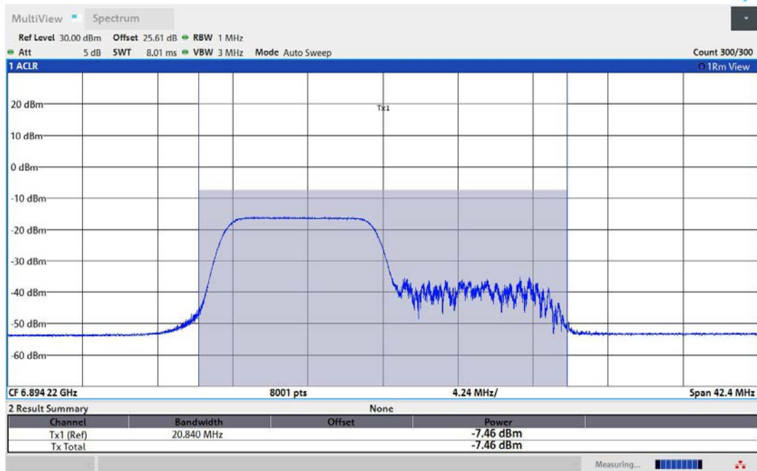
11AX20MIMO-Ant2-6895-106Tone-RU53-PASS
