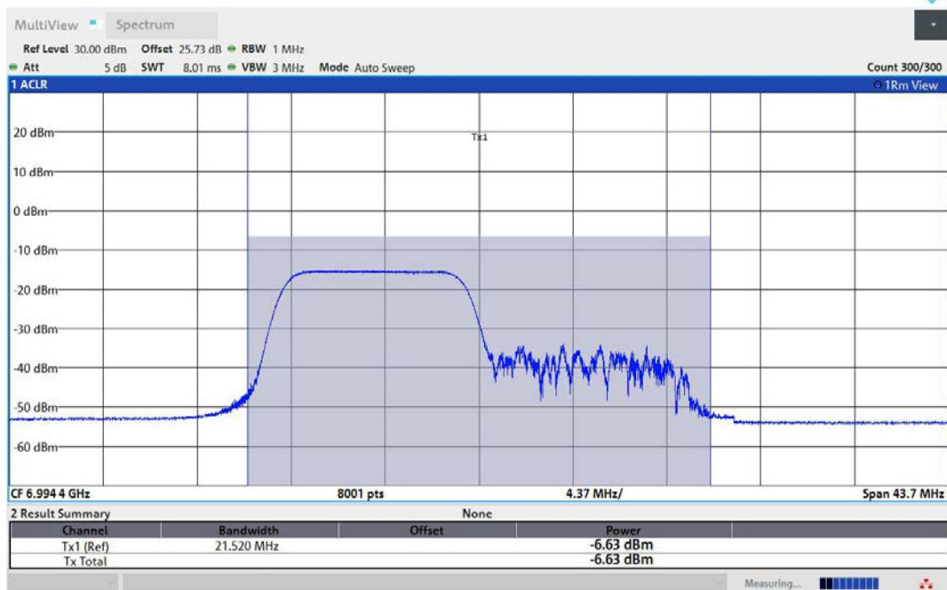
11AX20MIMO-Ant1-6995-106Tone-RU53-PASS
