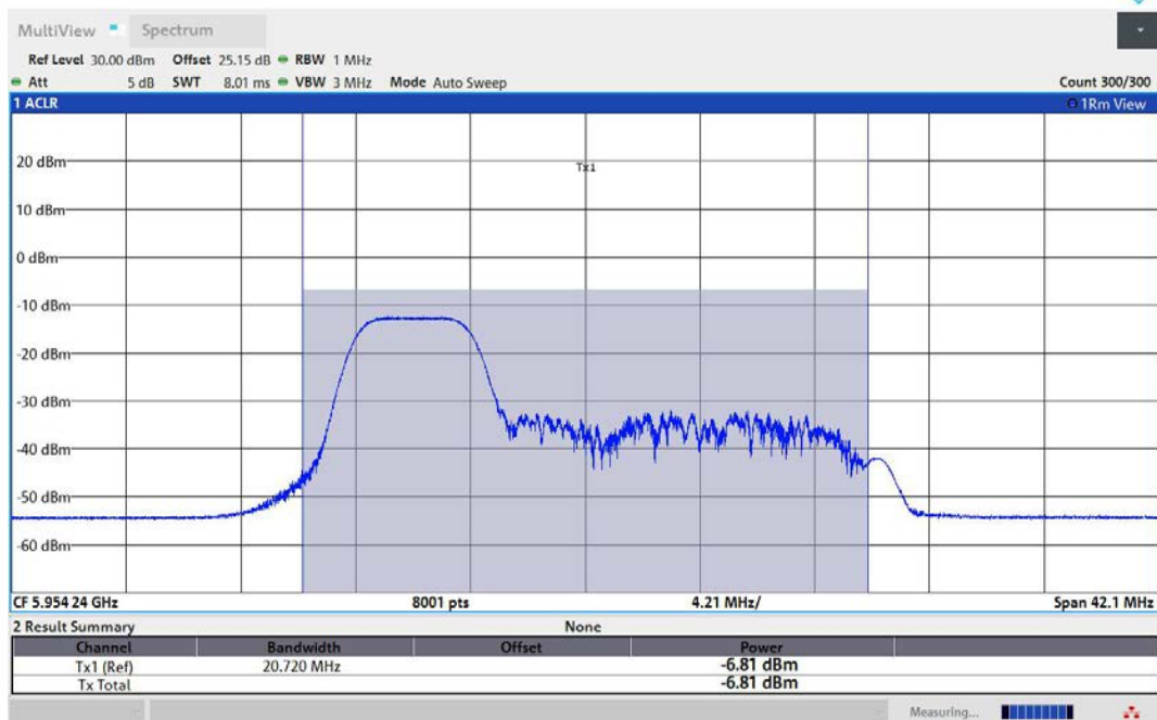
11AX40MIMO-Ant1-5965-52Tone-RU37-PASS
