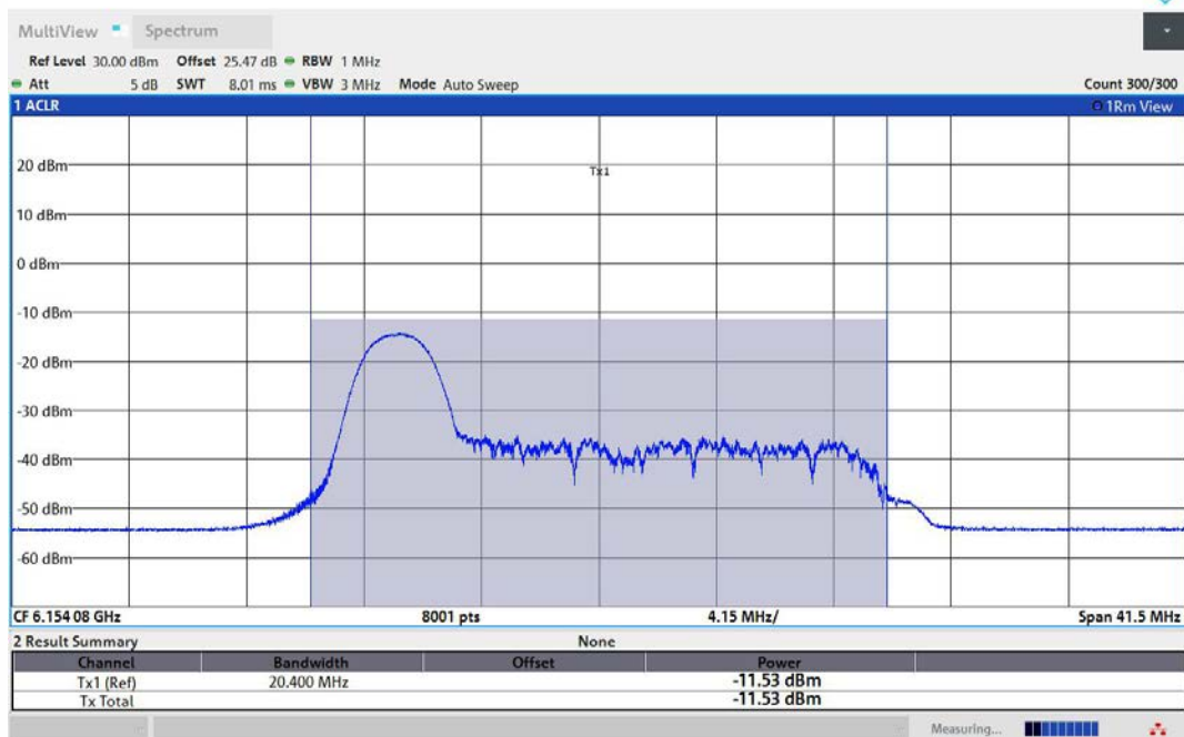
11AX40MIMO-Ant1-6165-26Tone-RU0-PASS
