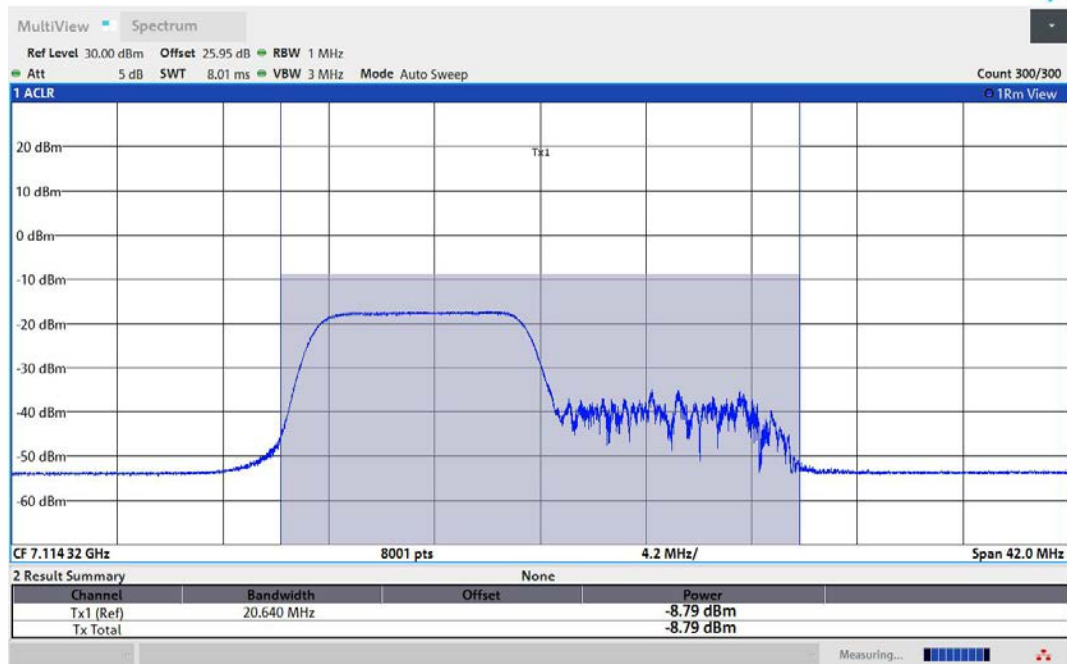
11AX20MIMO-Ant2-7115-106Tone-RU53-PASS
