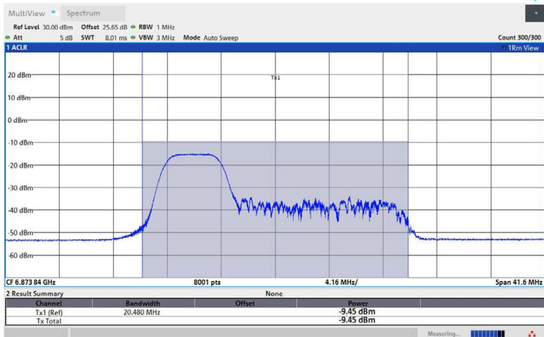
11AX20MIMO-Ant2-6875-52Tone-RU37-PASS
