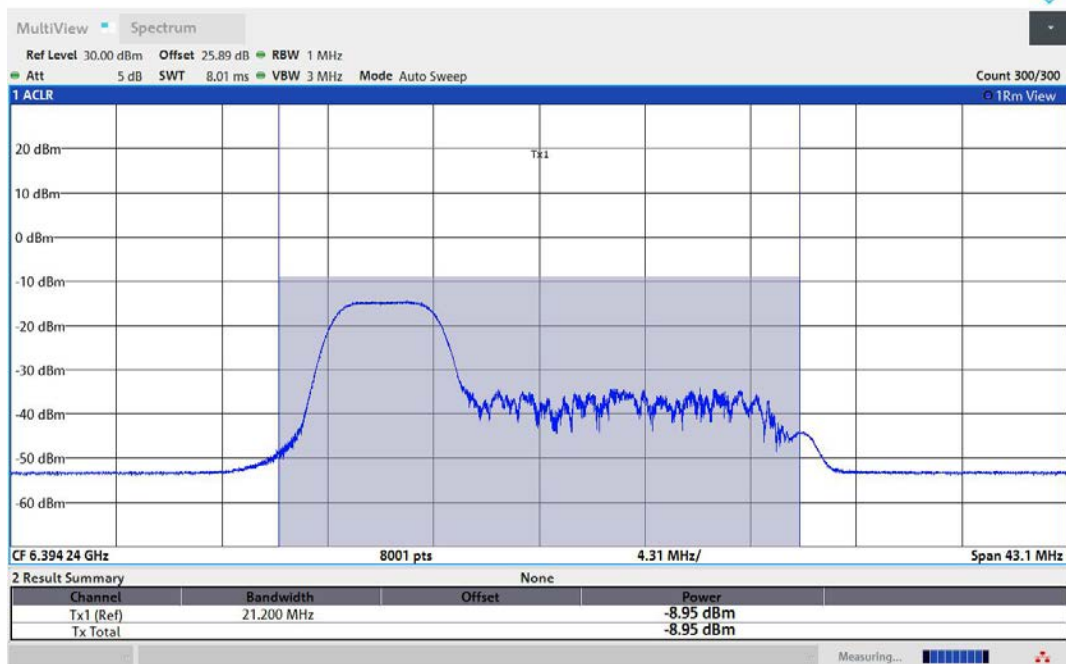
11AX40MIMO-Ant1-6405-52Tone-RU37-PASS
