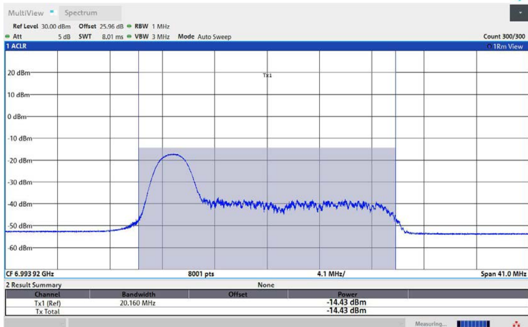
11AX20MIMO-Ant2-6995-26Tone-RU0-PASS
