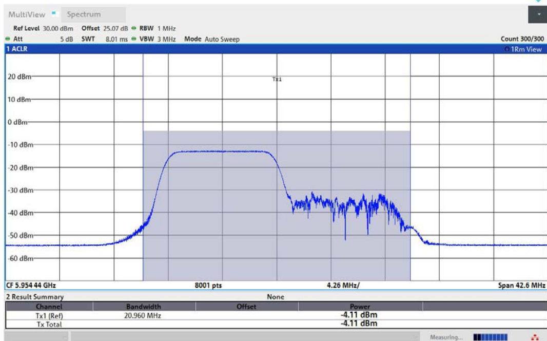
11AX40MIMO-Ant1-5965-106Tone-RU53-PASS
