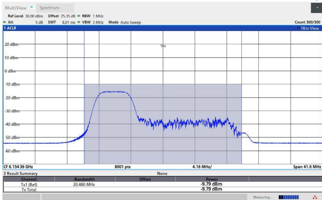
11AX40MIMO-Ant2-6165-52Tone-RU37-PASS
