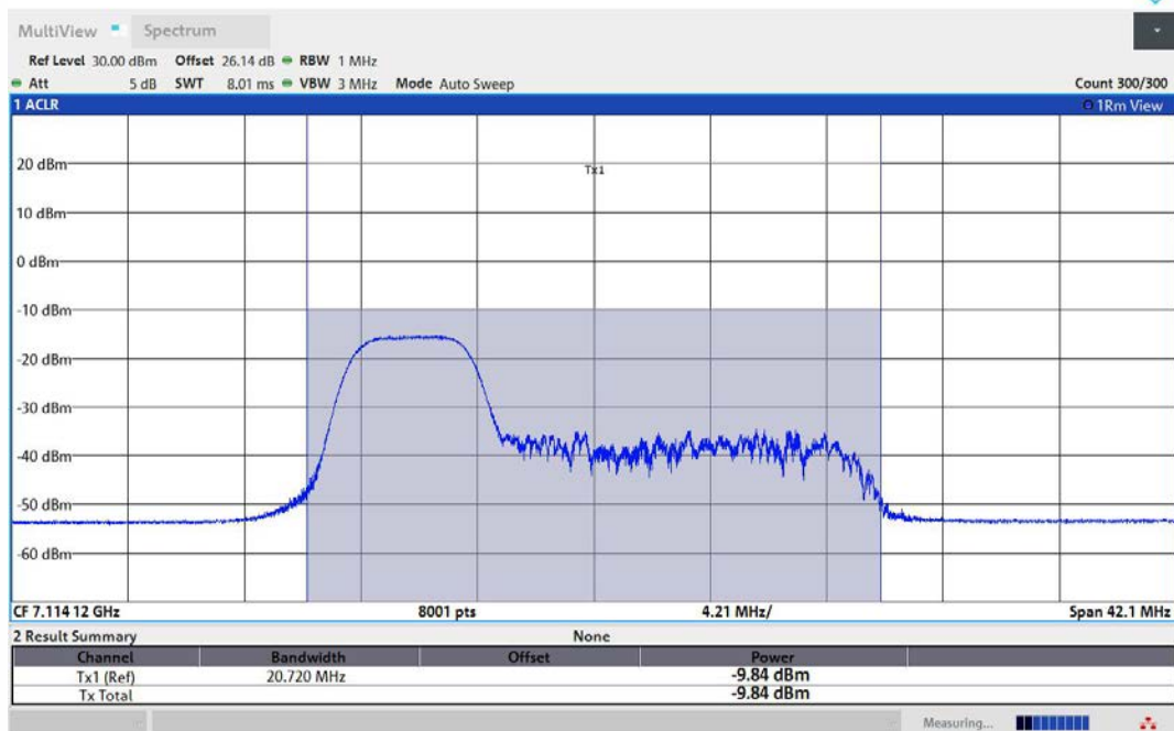
11AX20MIMO-Ant1-7115-52Tone-RU37-PASS
