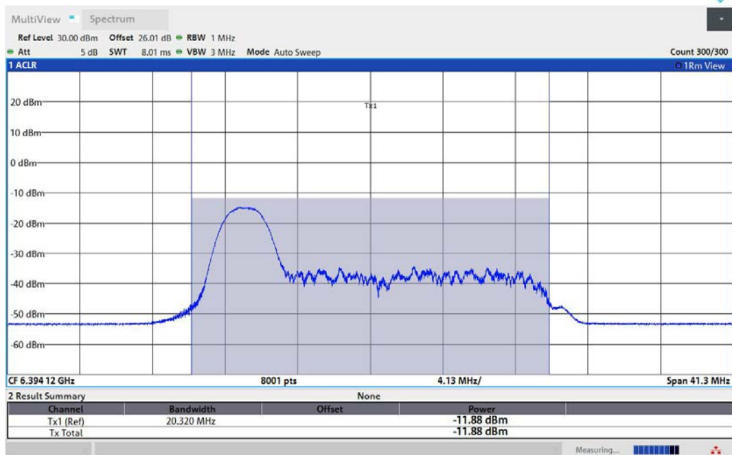
11AX40MIMO-Ant1-6405-26Tone-RU0-PASS
