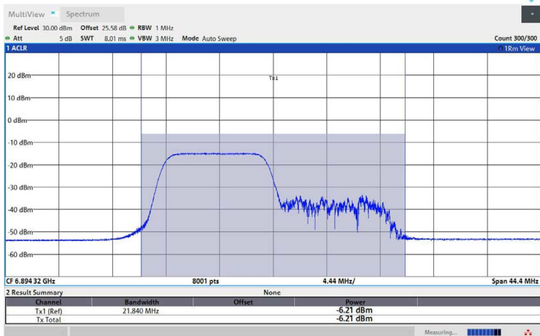
11AX20MIMO-Ant1-6895-106Tone-RU53-PASS
