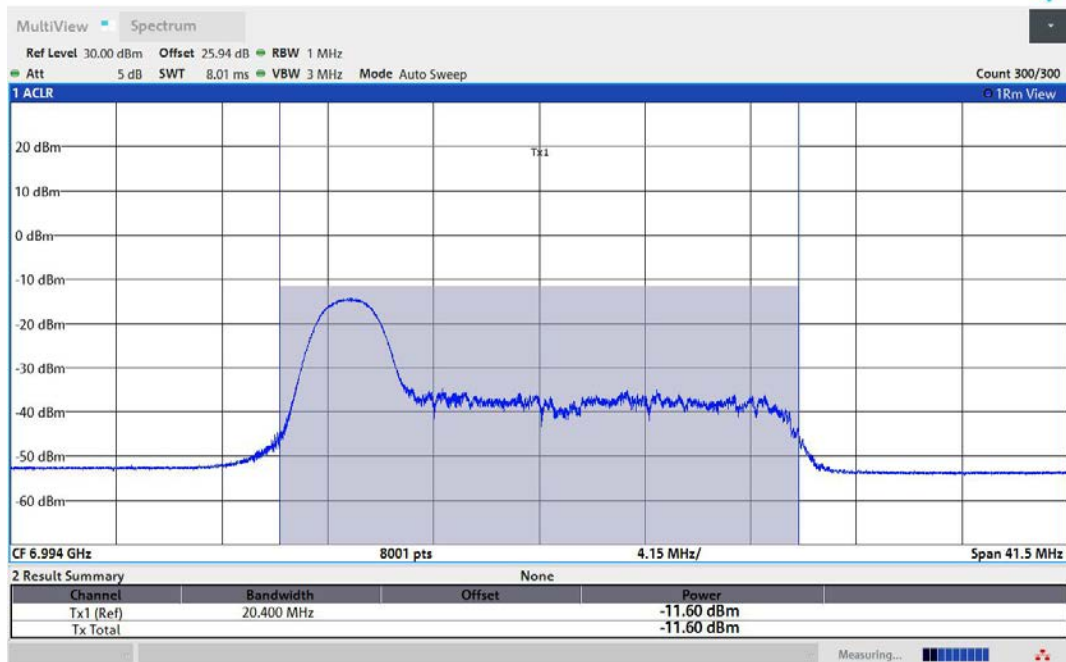
11AX20MIMO-Ant1-6995-26Tone-RU0-PASS
