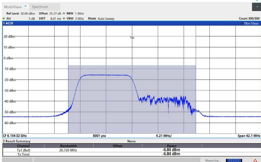
11AX40MIMO-Ant2-6165-106Tone-RU53-PASS
