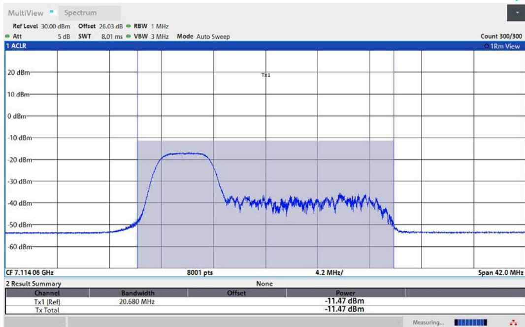
11AX20MIMO-Ant2-7115-52Tone-RU37-PASS
