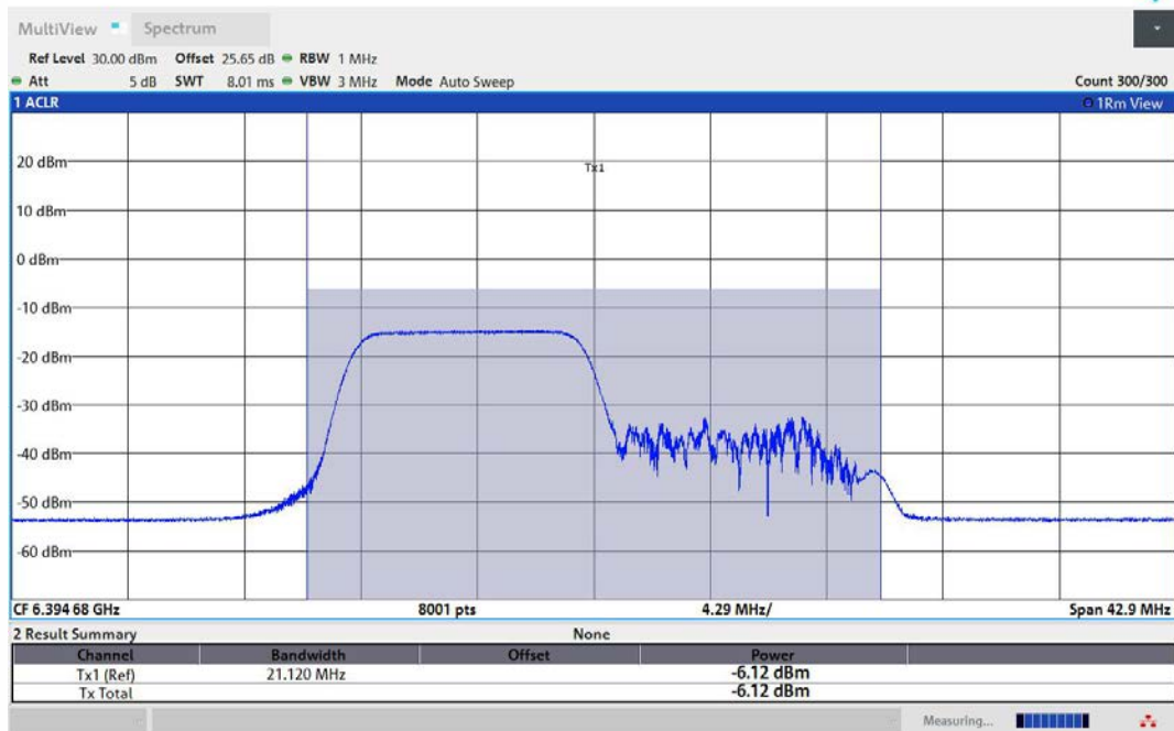
11AX40MIMO-Ant2-6405-106Tone-RU53-PASS
