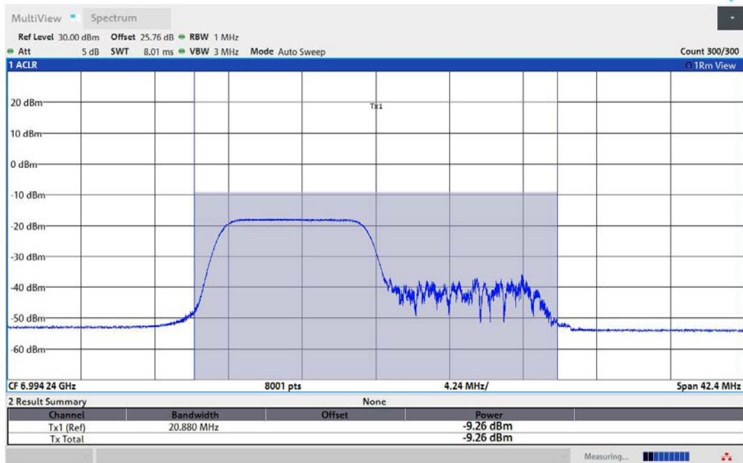
11AX20MIMO-Ant2-6995-106Tone-RU53-PASS
