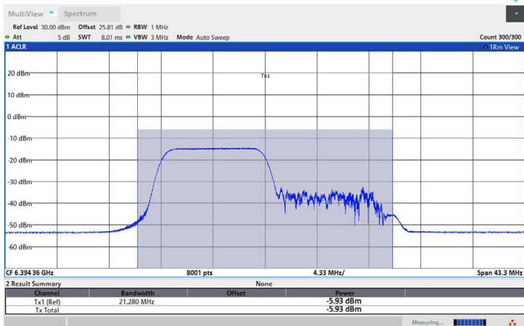
11AX40MIMO-Ant1-6405-106Tone-RU53-PASS
