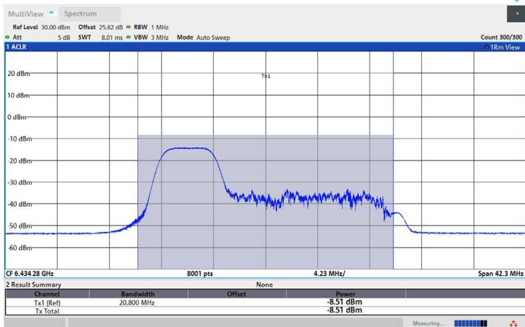
11AX40MIMO-Ant1-6445-52Tone-RU37-PASS
