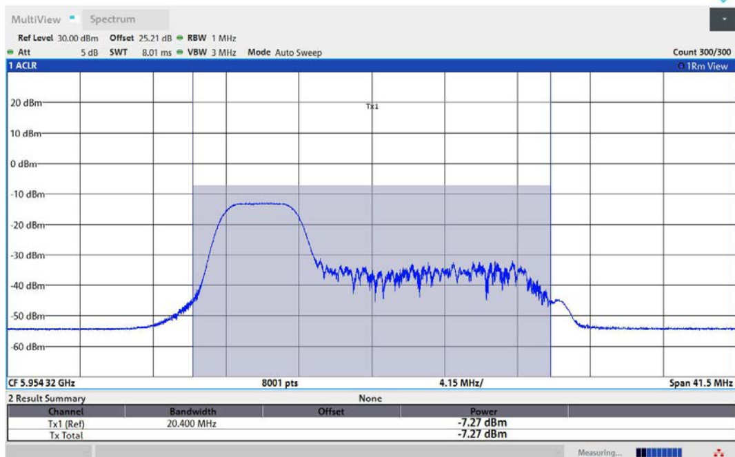
11AX40MIMO-Ant2-5965-52Tone-RU37-PASS
