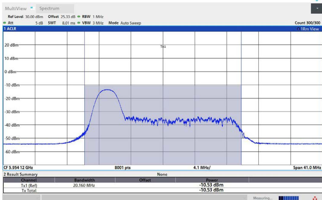
11AX40MIMO-Ant2-5965-26Tone-RU0-PASS
