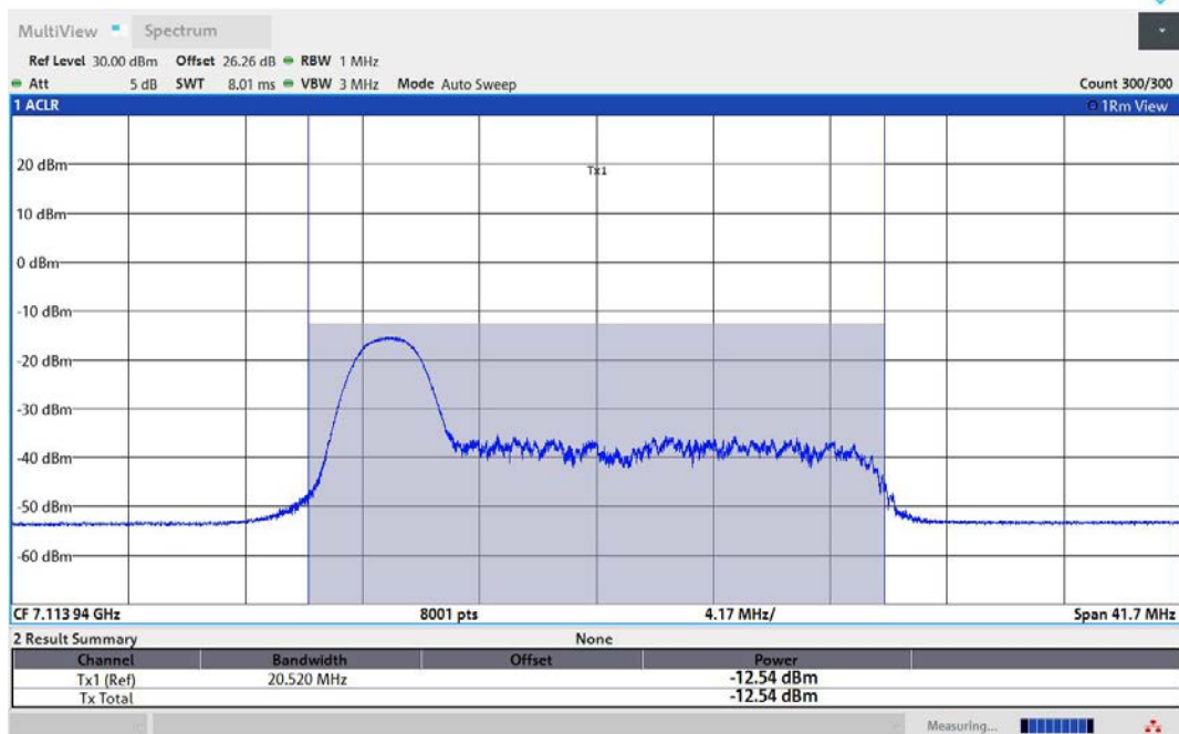
11AX20MIMO-Ant1-7115-26Tone-RU0-PASS
