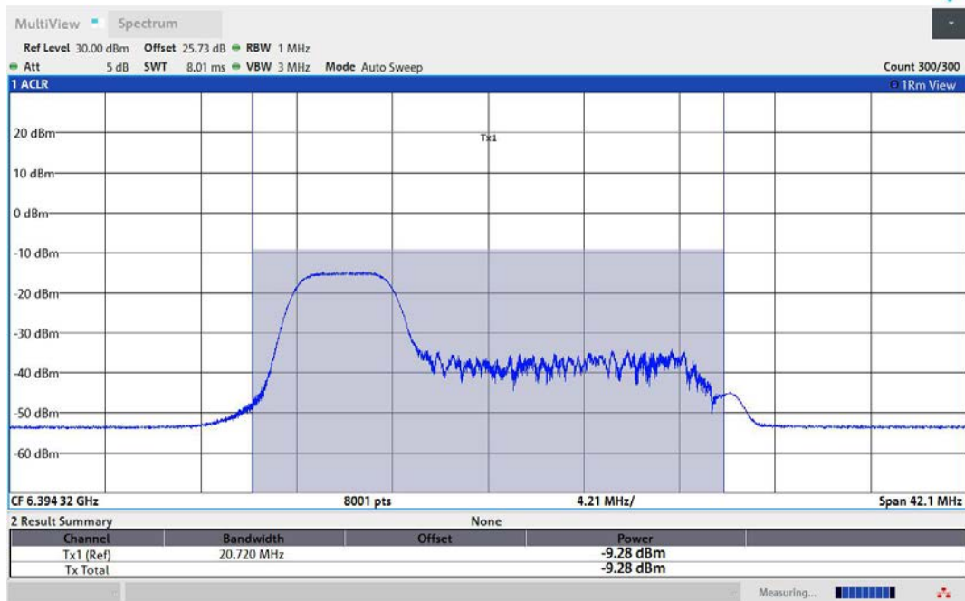
11AX40MIMO-Ant2-6405-52Tone-RU37-PASS
