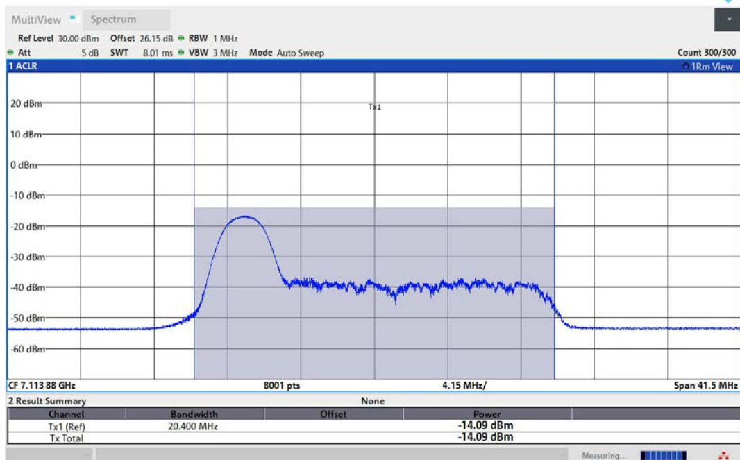
11AX20MIMO-Ant2-7115-26Tone-RU0-PASS
