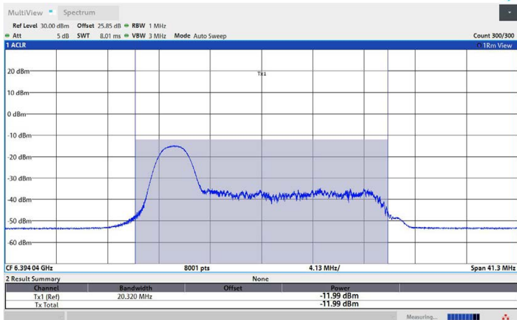
11AX40MIMO-Ant2-6405-26Tone-RU0-PASS
