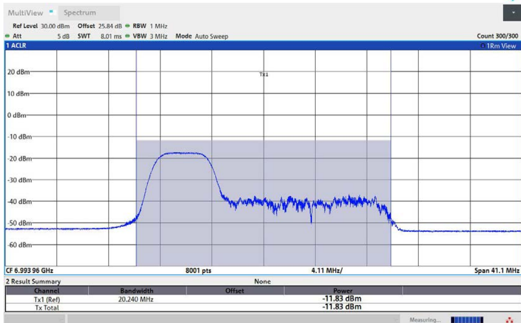
11AX20MIMO-Ant2-6995-52Tone-RU37-PASS
