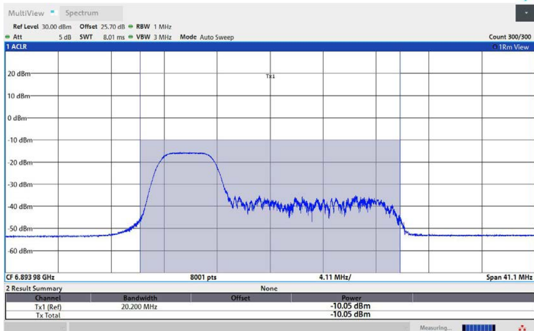
11AX20MIMO-Ant2-6895-52Tone-RU37-PASS
