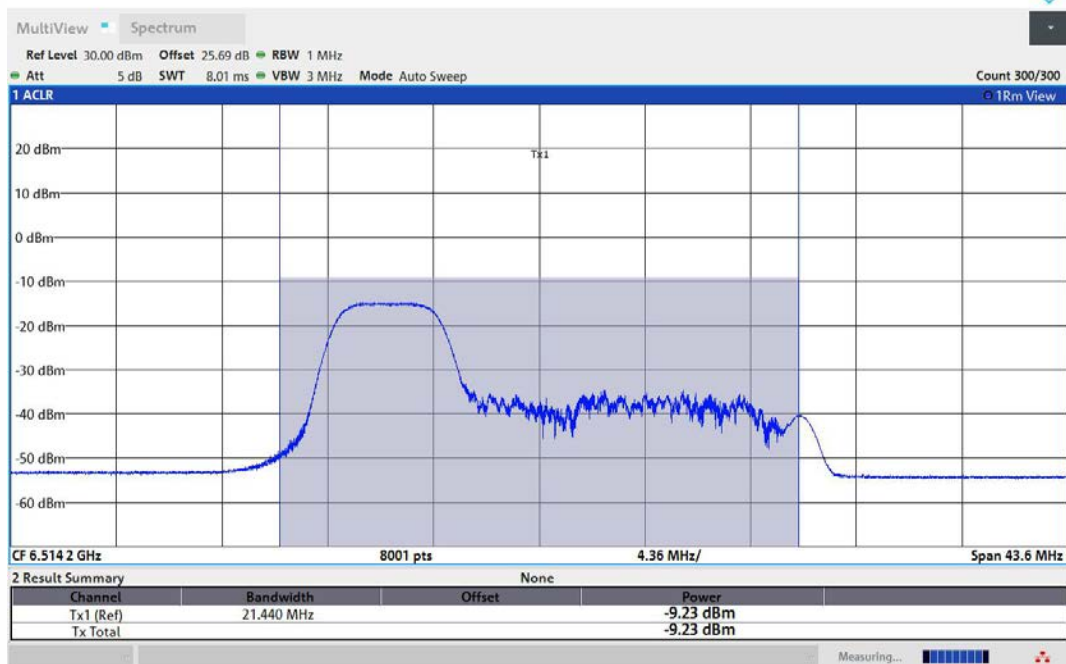
11AX40MIMO-Ant1-6525-52Tone-RU37-PASS
