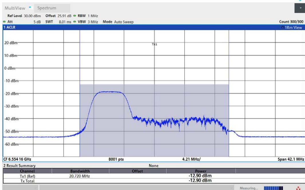
11AX40MIMO-Ant2-6565-52Tone-RU37-PASS
