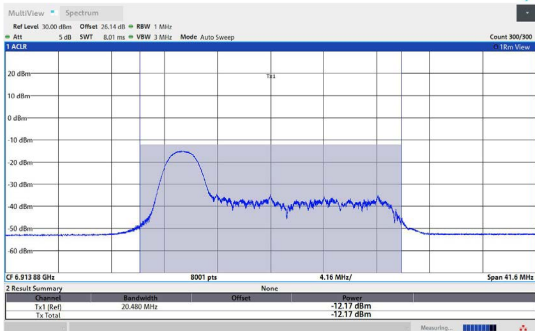
11AX40MIMO-Ant2-6925-26Tone-RU0-PASS
