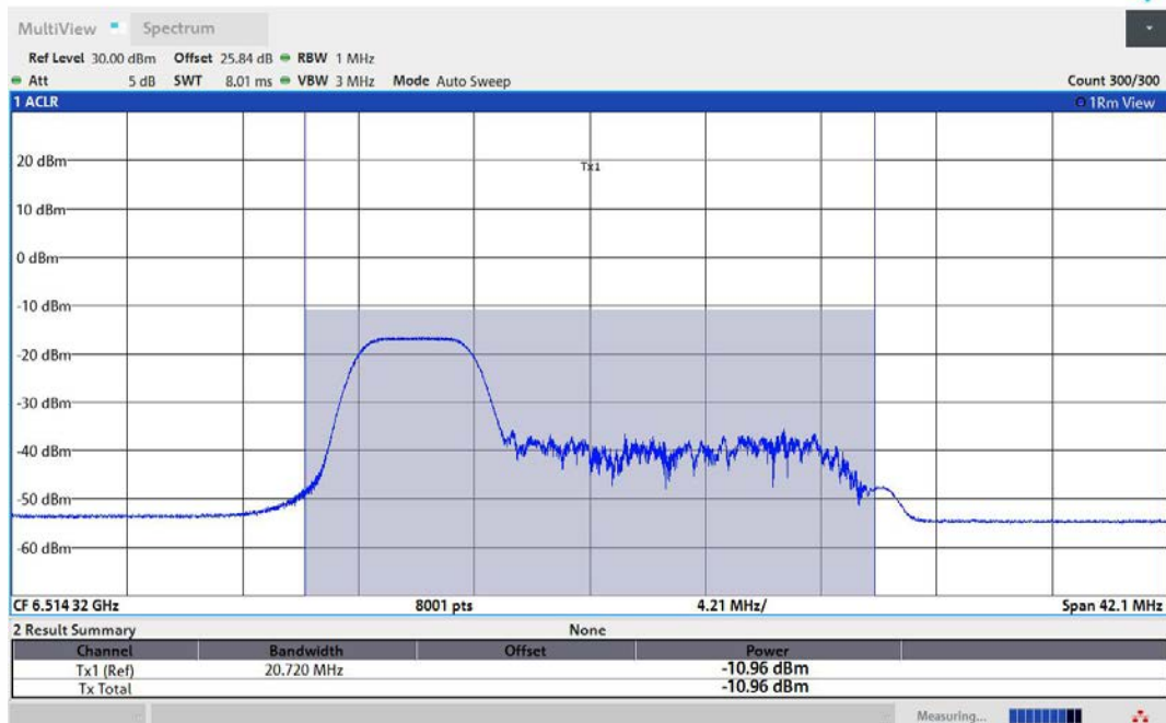
11AX40MIMO-Ant2-6525-52Tone-RU37-PASS
