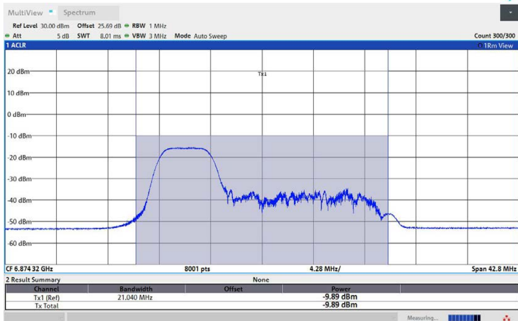
11AX40MIMO-Ant2-6885-52Tone-RU37-PASS
