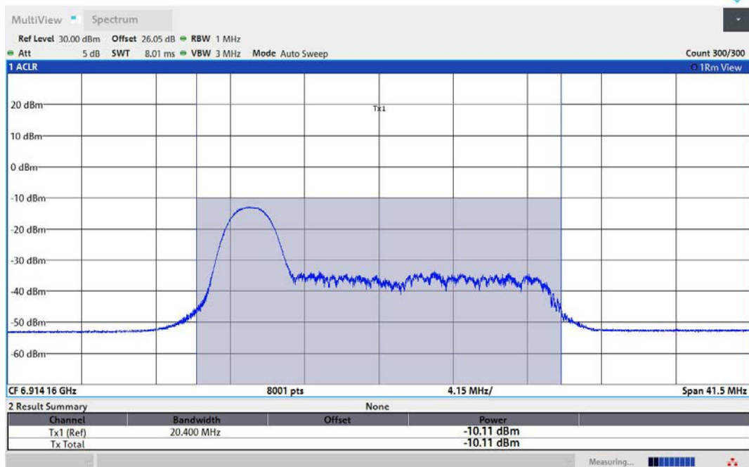
11AX40MIMO-Ant1-6925-26Tone-RU0-PASS
