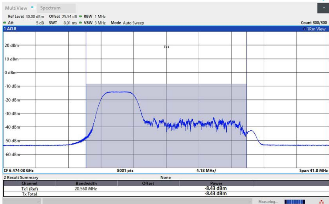
11AX40MIMO-Ant1-6485-52Tone-RU37-PASS
