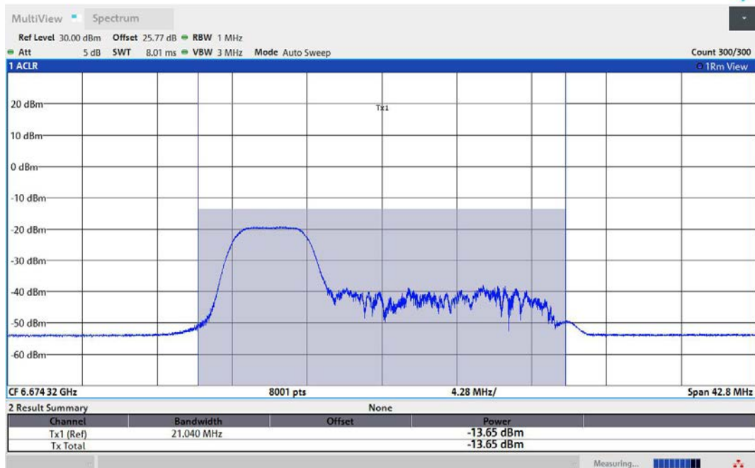
11AX40MIMO-Ant2-6685-52Tone-RU37-PASS
