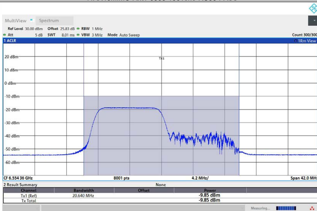
11AX40MIMO-Ant2-6565-106Tone-RU53-PASS
