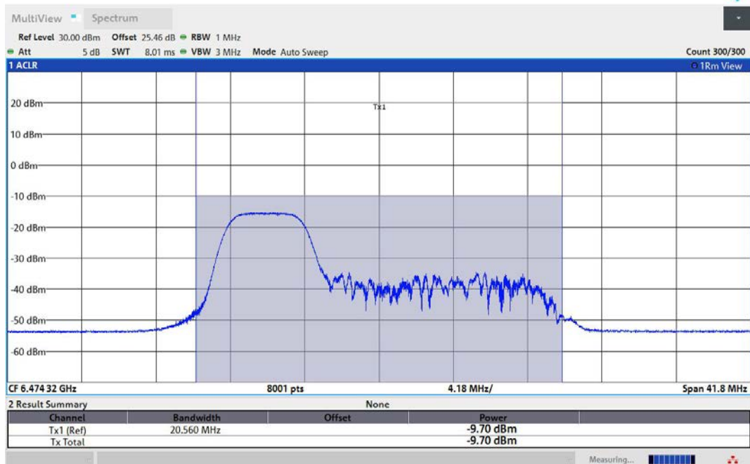
11AX40MIMO-Ant2-6485-52Tone-RU37-PASS
