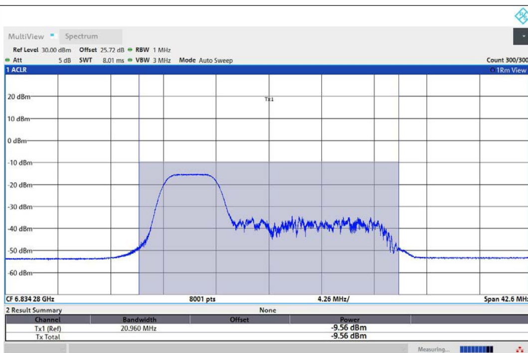
11AX40MIMO-Ant1-6845-52Tone-RU37-PASS
