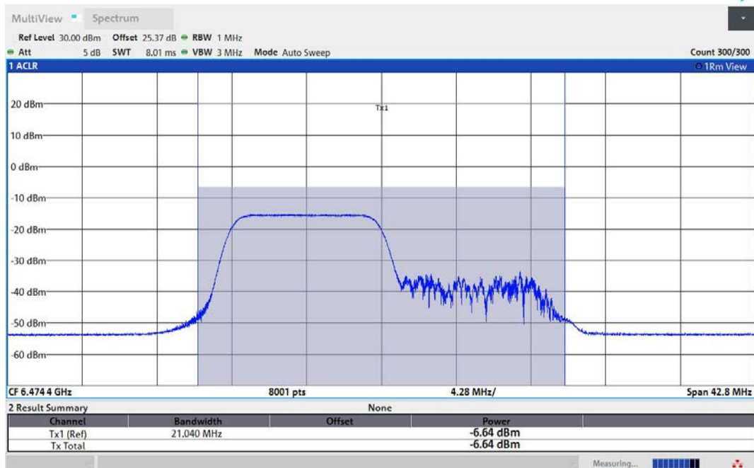
11AX40MIMO-Ant2-6485-106Tone-RU53-PASS
