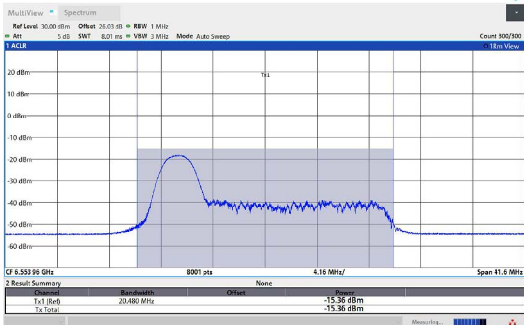
11AX40MIMO-Ant2-6565-26Tone-RU0-PASS
