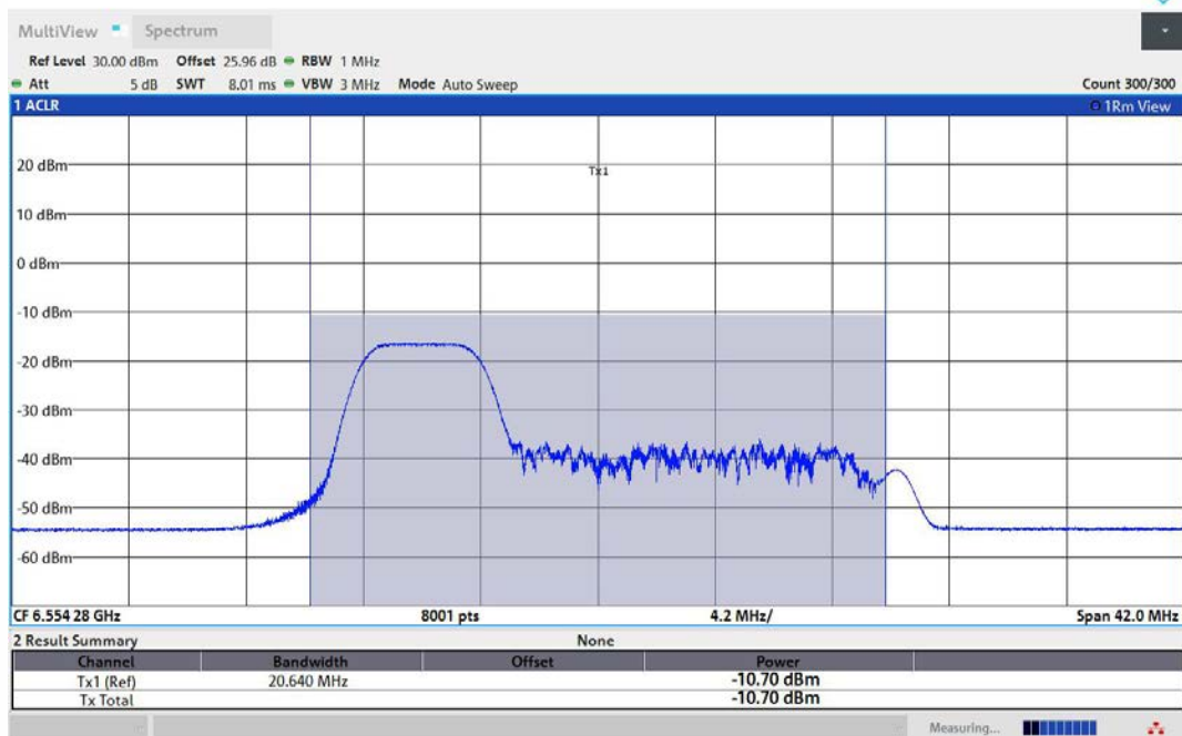
11AX40MIMO-Ant1-6565-52Tone-RU37-PASS
