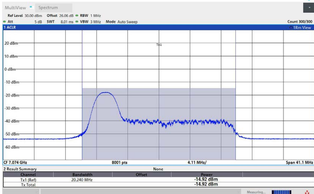
11AX40MIMO-Ant2-7085-26Tone-RU0-PASS
