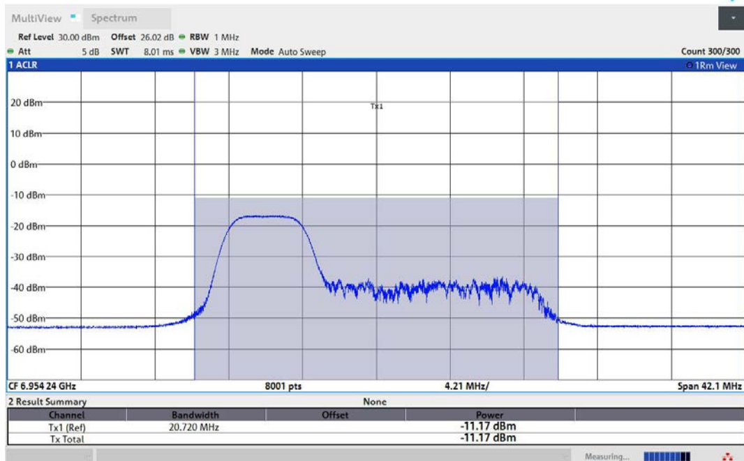
11AX40MIMO-Ant2-6965-52Tone-RU37-PASS
