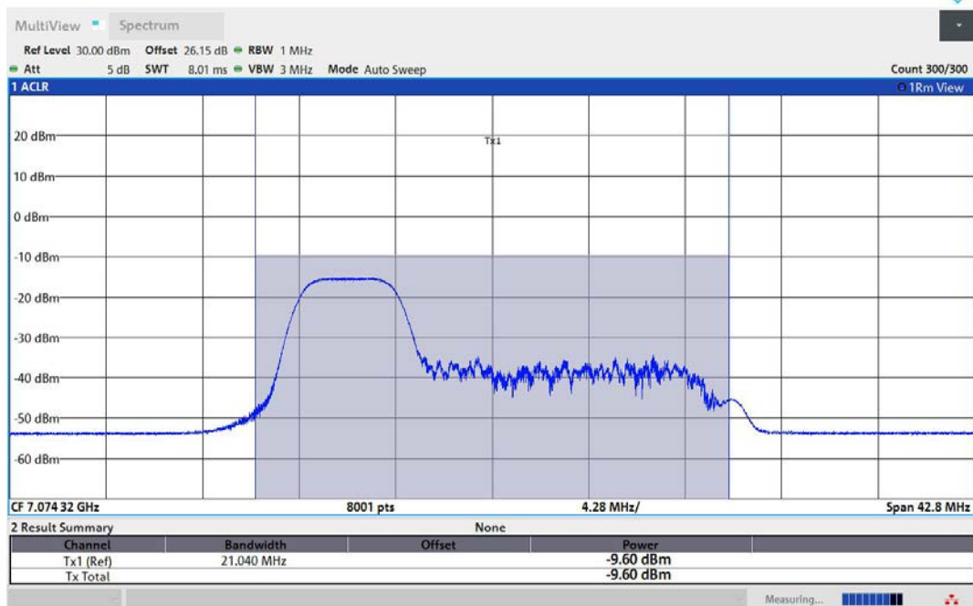
11AX40MIMO-Ant1-7085-52Tone-RU37-PASS
