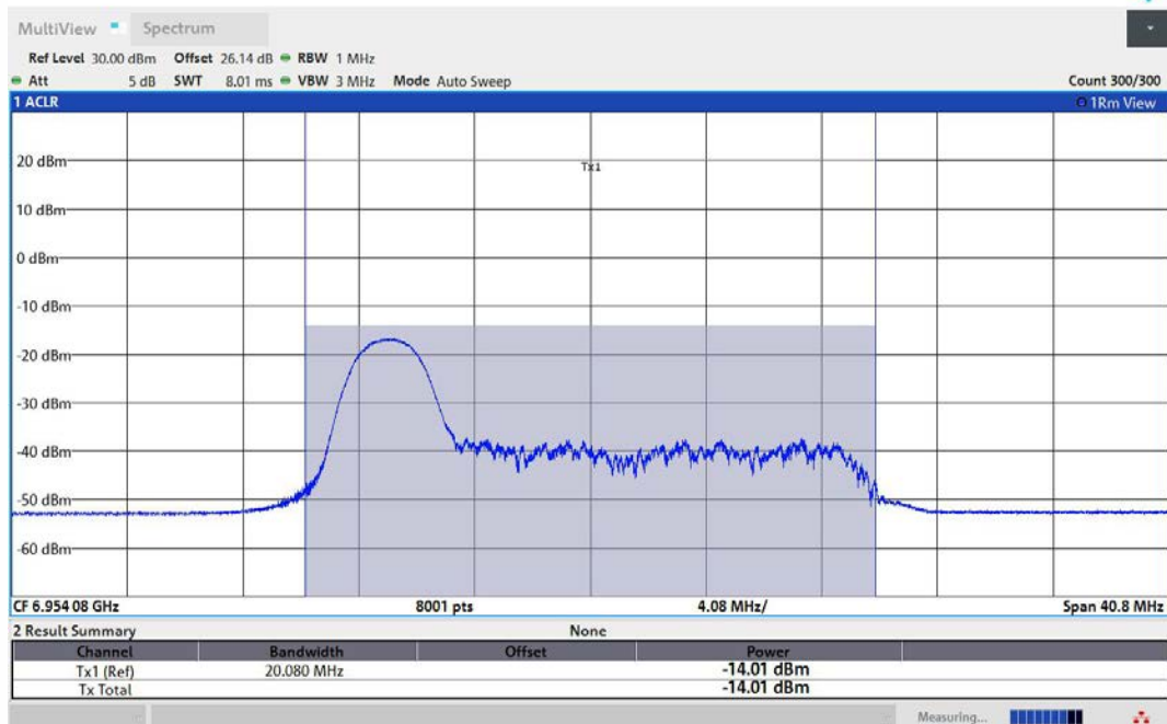
11AX40MIMO-Ant2-6965-26Tone-RU0-PASS
