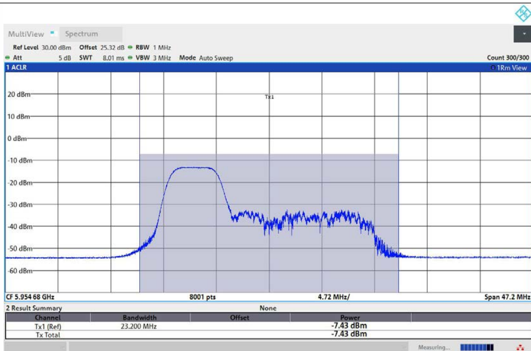
11AX80MIMO-Ant1-5985-52Tone-RU37-PASS
