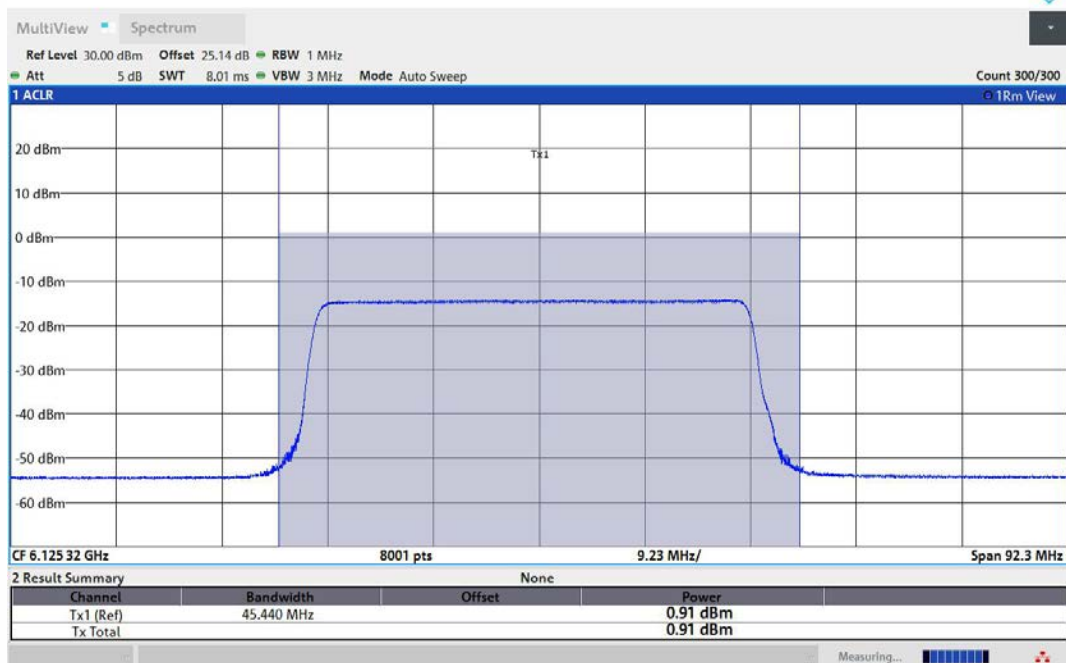
11AX80MIMO-Ant2-6145-484Tone-RU65-PASS
