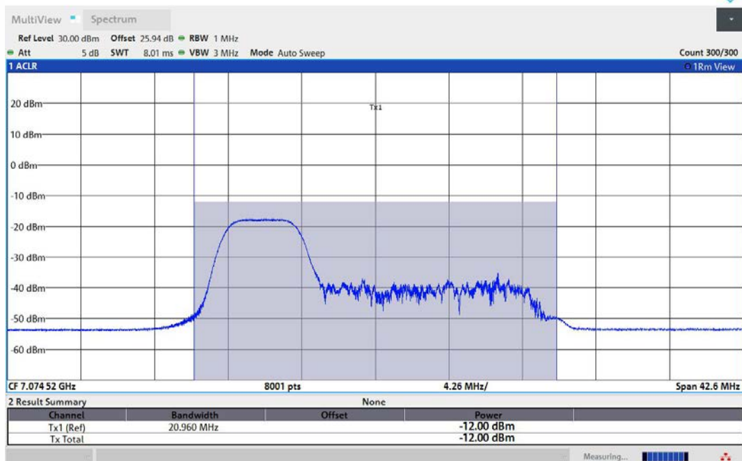
11AX40MIMO-Ant2-7085-52Tone-RU37-PASS
