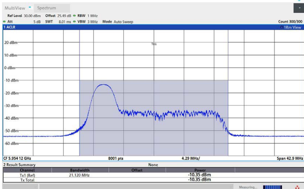
11AX80MIMO-Ant2-5985-26Tone-RU0-PASS
