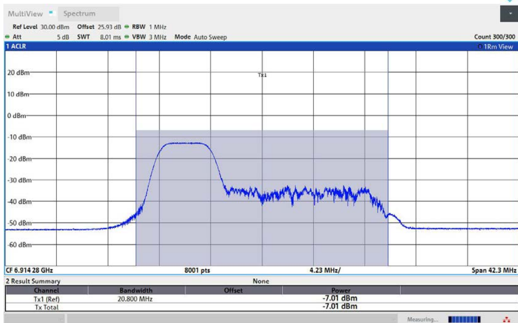
11AX40MIMO-Ant1-6925-52Tone-RU37-PASS
