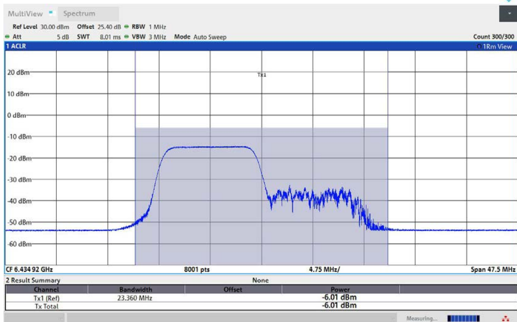
11AX80MIMO-Ant1-6465-106Tone-RU53-PASS
