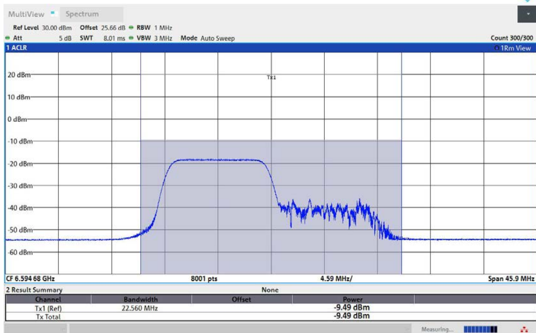
11AX80MIMO-Ant1-6625-106Tone-RU53-PASS
