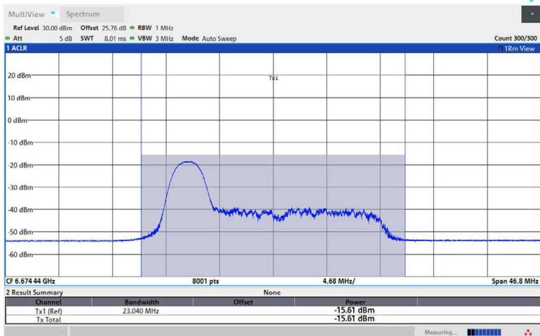
11AX80MIMO-Ant1-6705-26Tone-RU0-PASS
