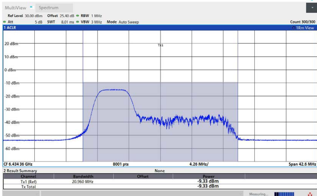
11AX80MIMO-Ant2-6465-52Tone-RU37-PASS
