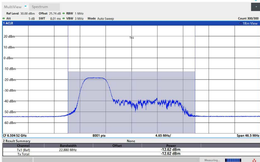
11AX80MIMO-Ant1-6625-52Tone-RU37-PASS
