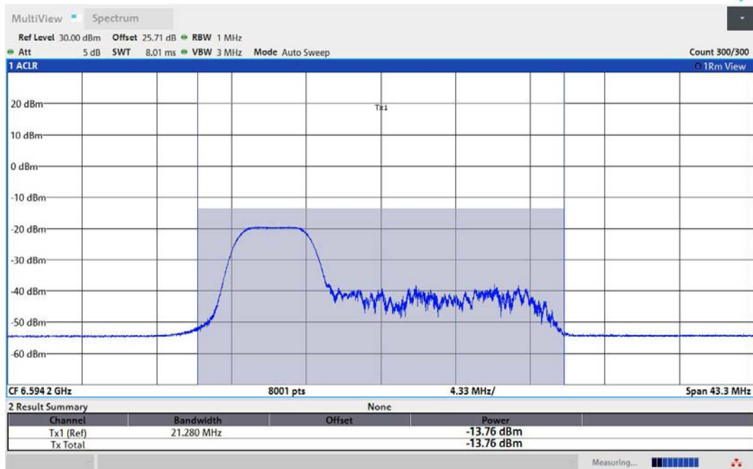
11AX80MIMO-Ant2-6625-52Tone-RU37-PASS
