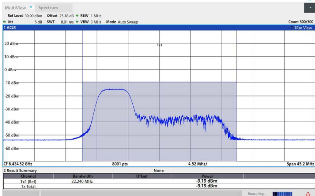
11AX80MIMO-Ant1-6465-52Tone-RU37-PASS
