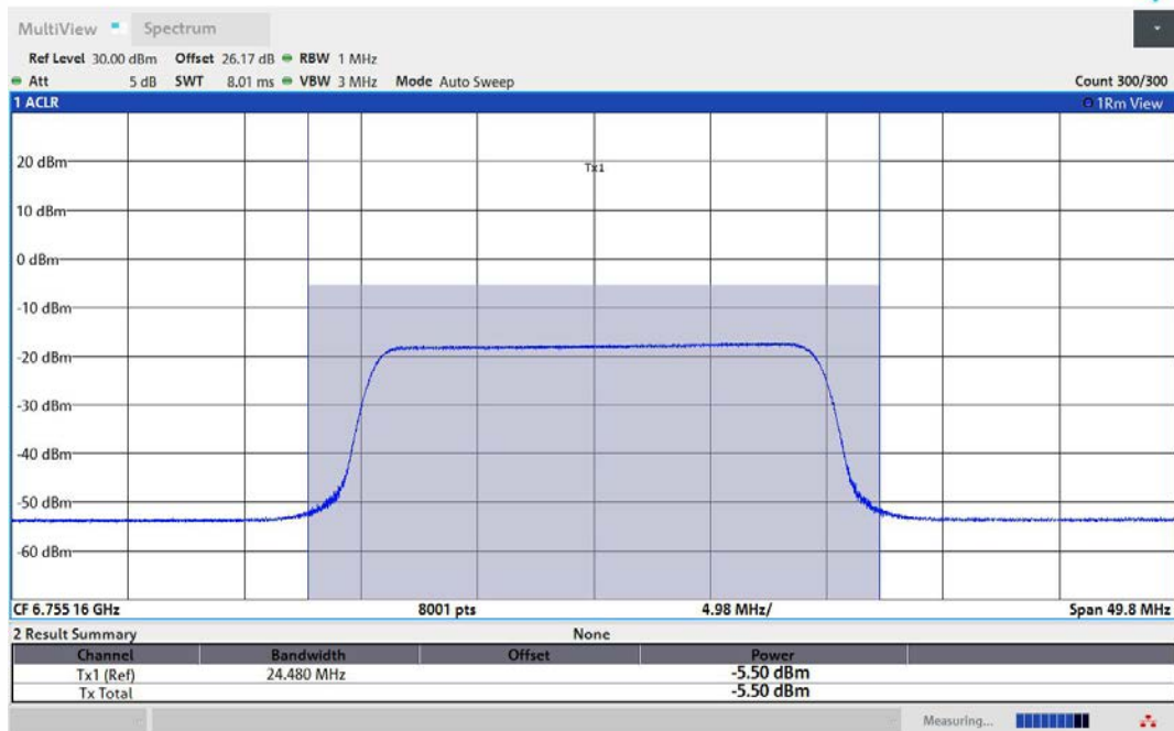
11AX80MIMO-Ant2-6785-242Tone-RU61-PASS
