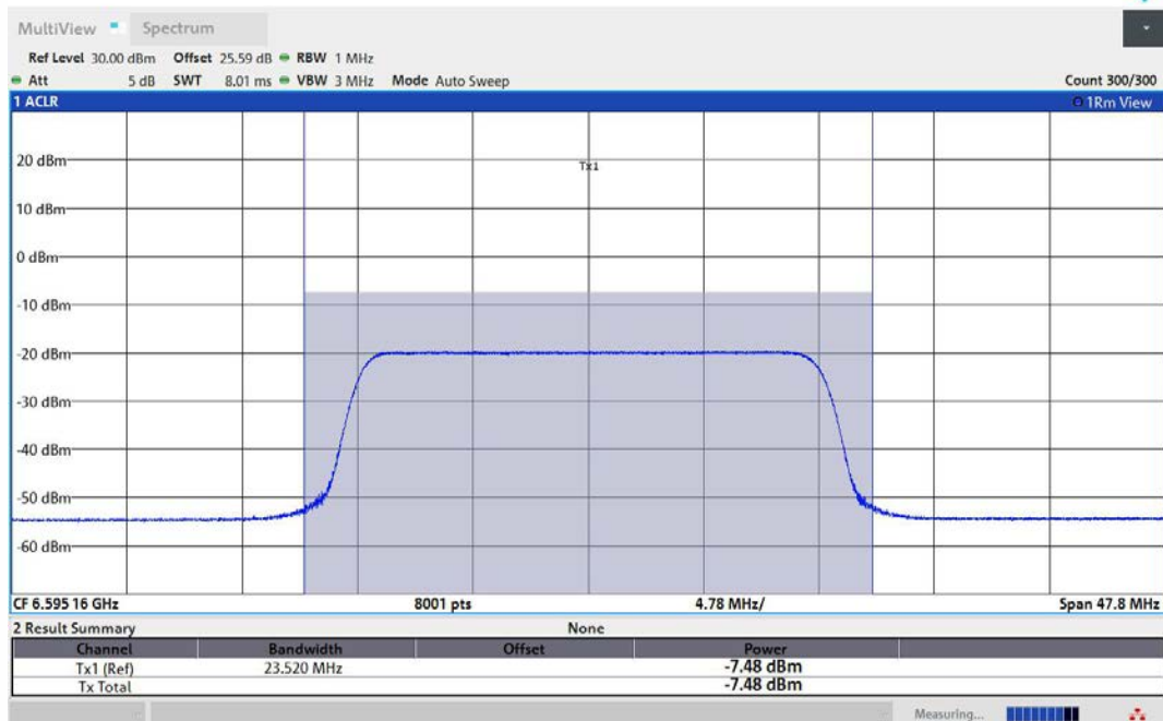
11AX80MIMO-Ant2-6625-242Tone-RU61-PASS
