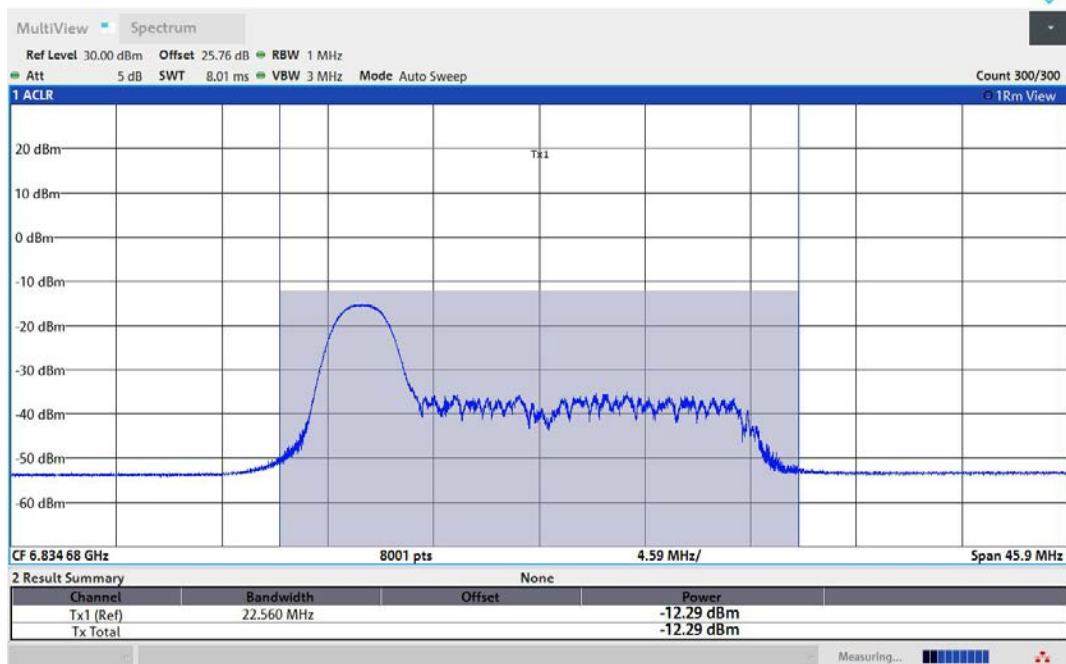
11AX80MIMO-Ant1-6865-26Tone-RU0-PASS
