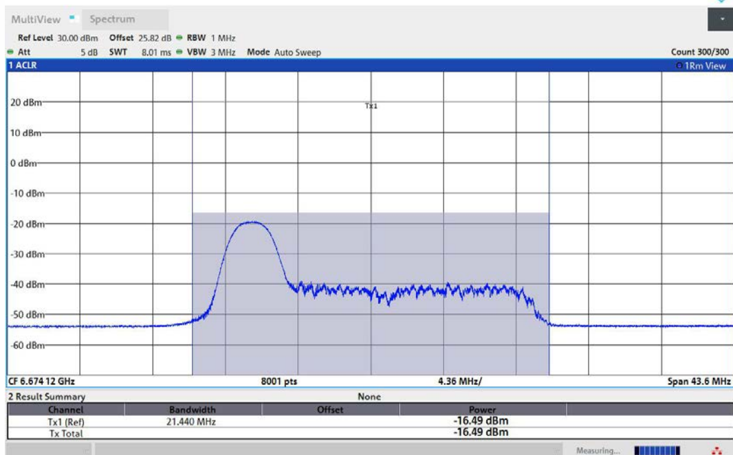
11AX80MIMO-Ant2-6705-26Tone-RU0-PASS
