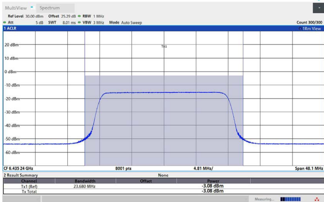
11AX80MIMO-Ant2-6465-242Tone-RU61-PASS
