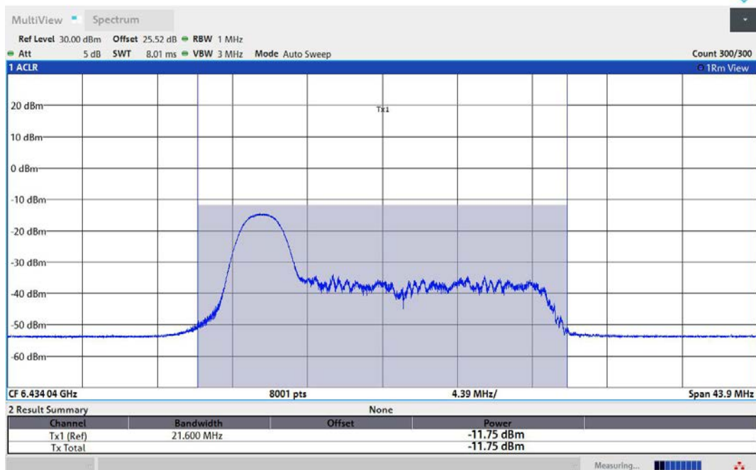
11AX80MIMO-Ant2-6465-26Tone-RU0-PASS
