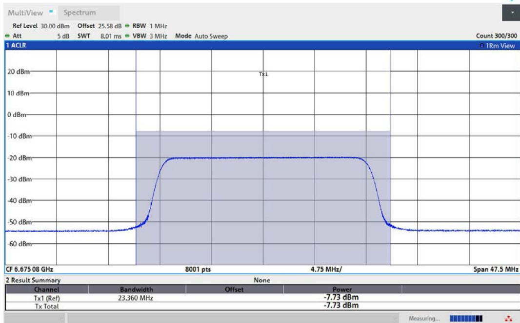
11AX80MIMO-Ant2-6705-242Tone-RU61-PASS
