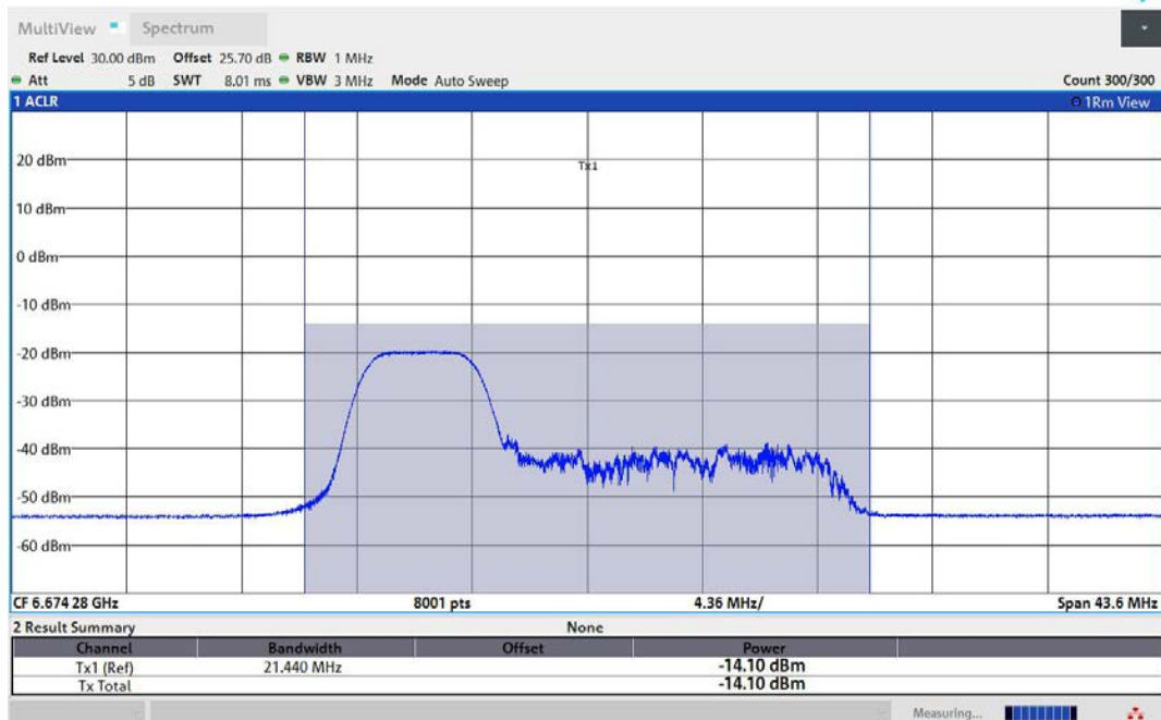
11AX80MIMO-Ant2-6705-52Tone-RU37-PASS
