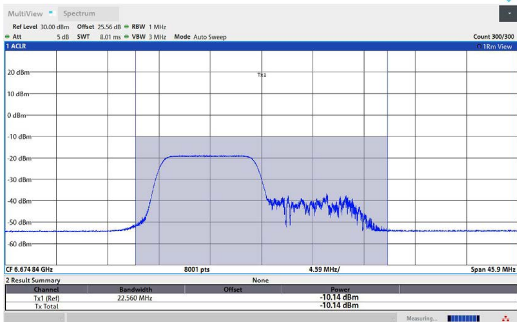
11AX80MIMO-Ant1-6705-106Tone-RU53-PASS
