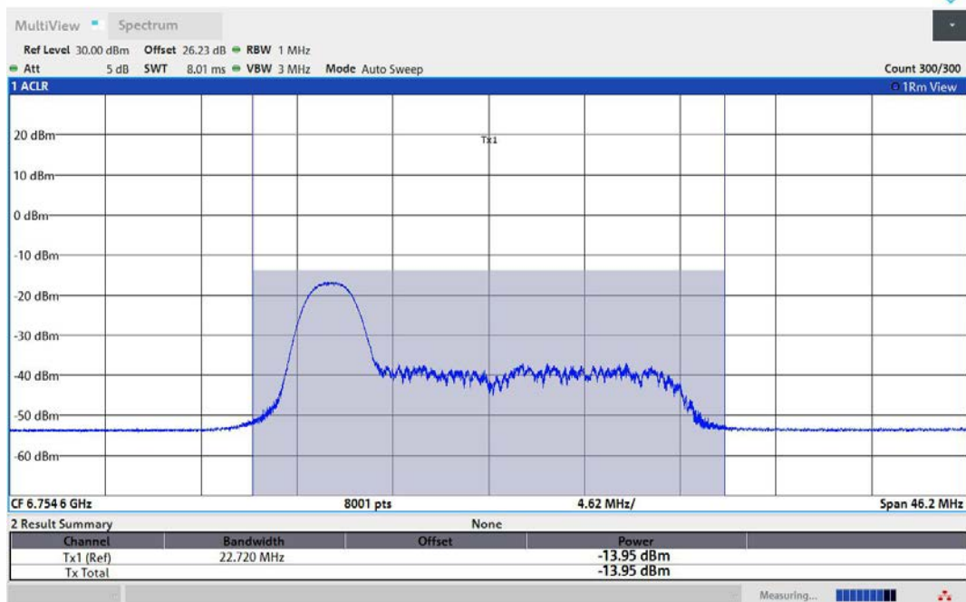
11AX80MIMO-Ant1-6785-26Tone-RU0-PASS
