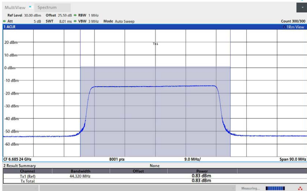
11AX80MIMO-Ant2-6705-484Tone-RU65-PASS
