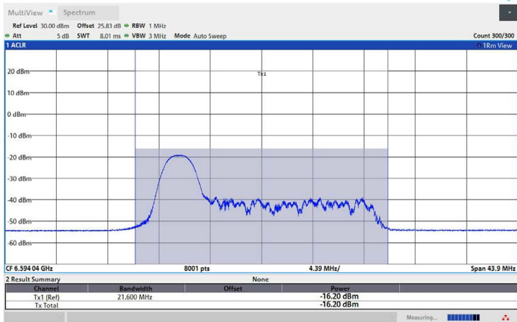
11AX80MIMO-Ant2-6625-26Tone-RU0-PASS
