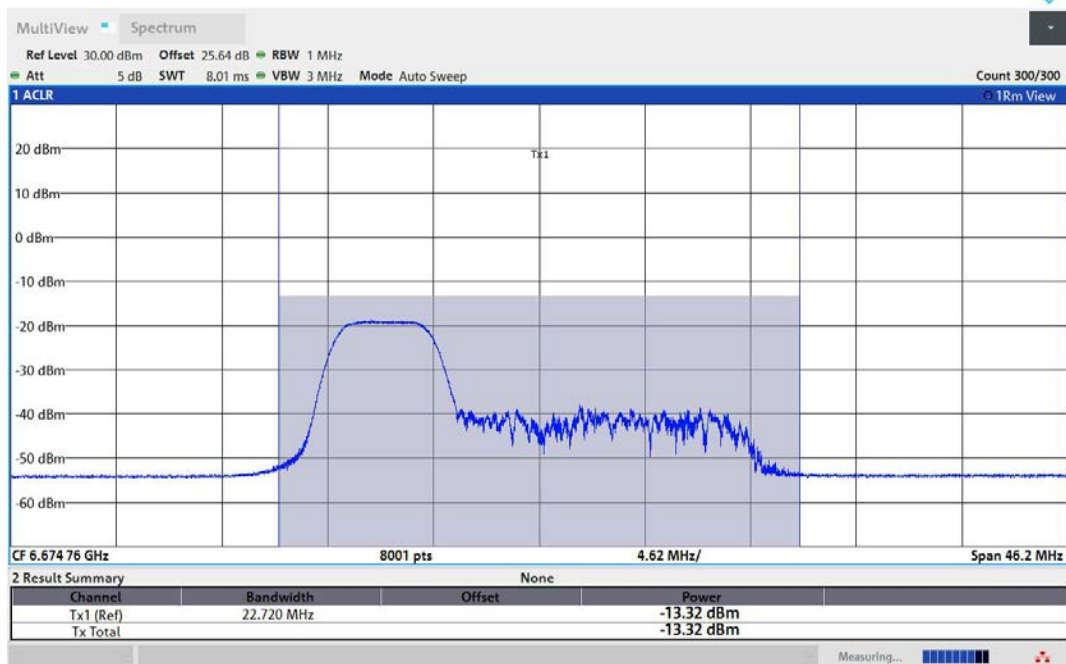
11AX80MIMO-Ant1-6705-52Tone-RU37-PASS
