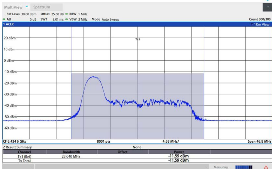
11AX80MIMO-Ant1-6465-26Tone-RU0-PASS
