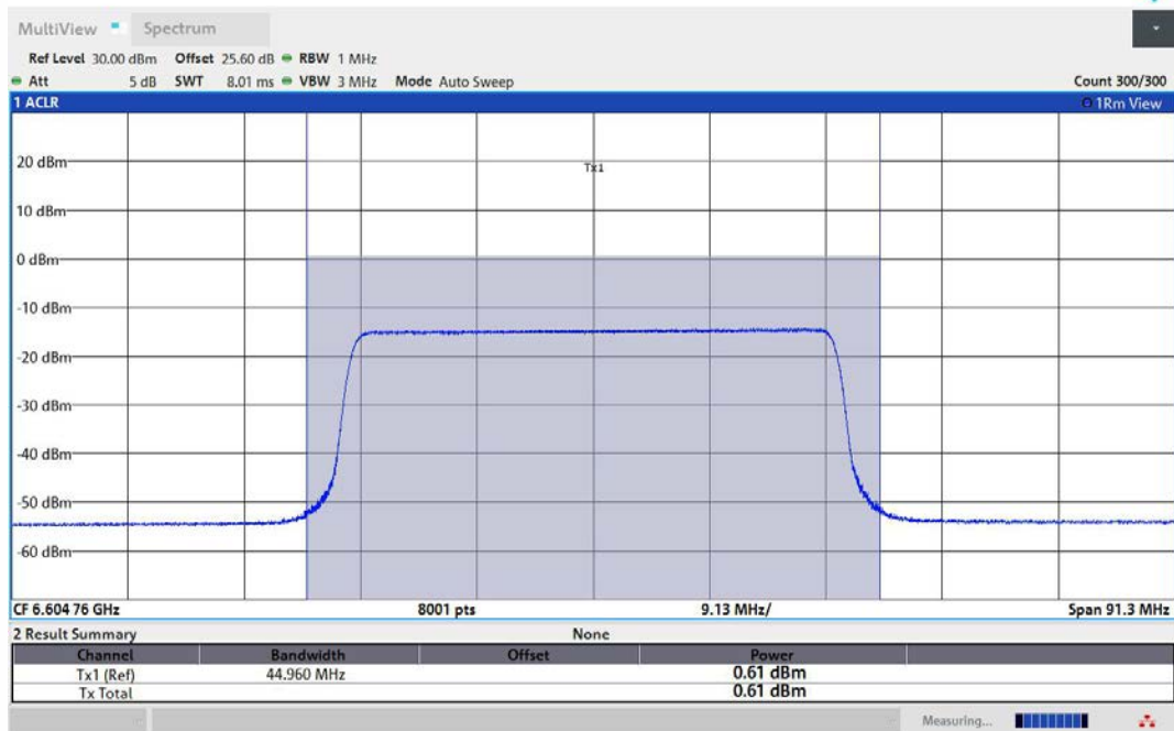
11AX80MIMO-Ant2-6625-484Tone-RU65-PASS
