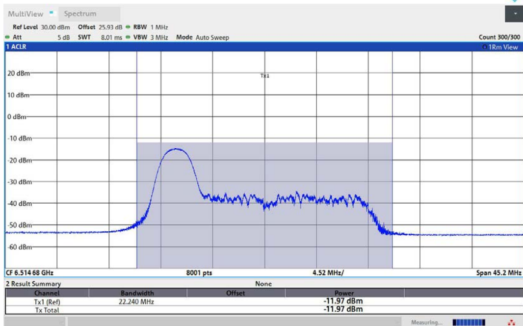
11AX80MIMO-Ant1-6545-26Tone-RU0-PASS
