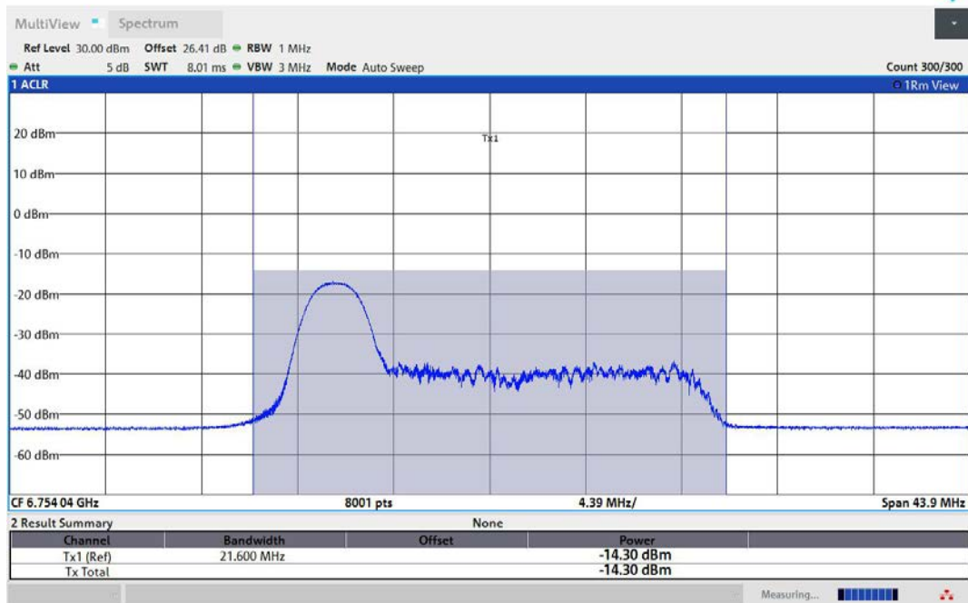
11AX80MIMO-Ant2-6785-26Tone-RU0-PASS
