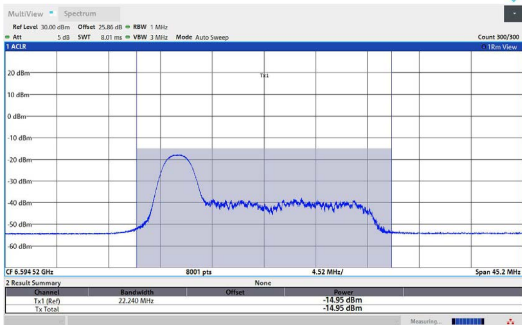
11AX80MIMO-Ant1-6625-26Tone-RU0-PASS
