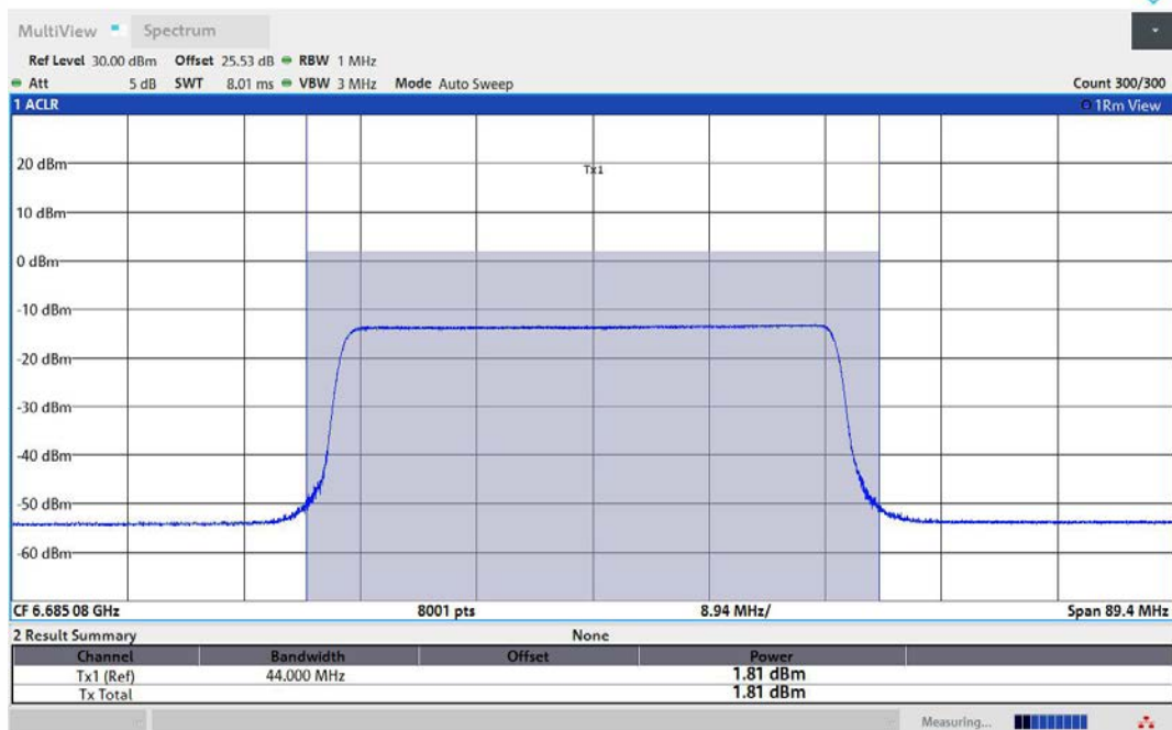
11AX80MIMO-Ant1-6705-484Tone-RU65-PASS
