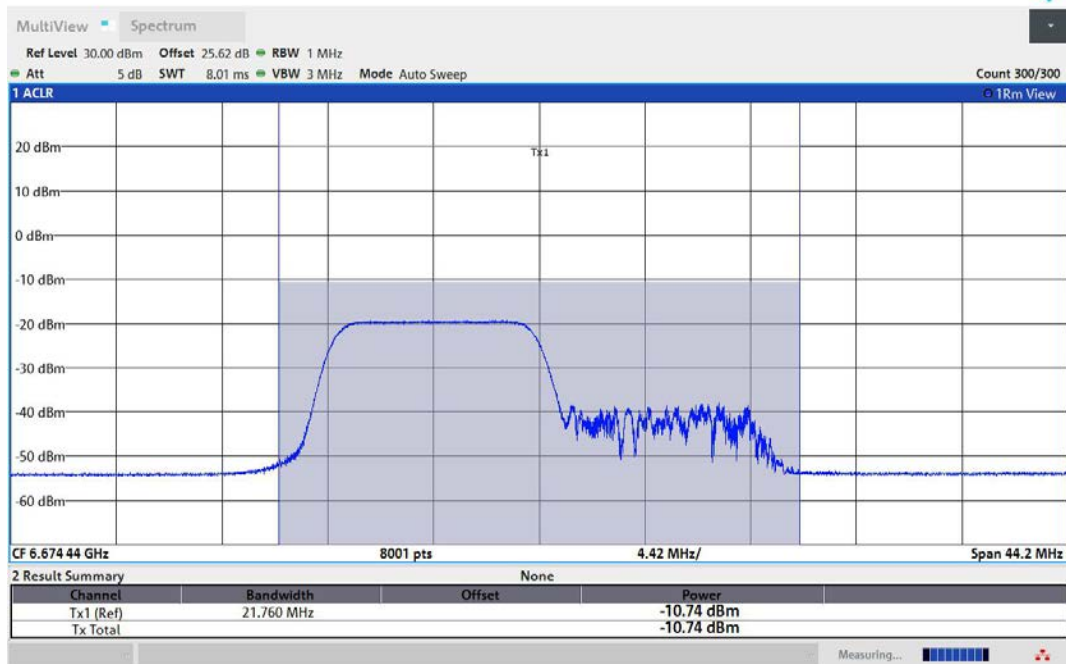
11AX80MIMO-Ant2-6705-106Tone-RU53-PASS
