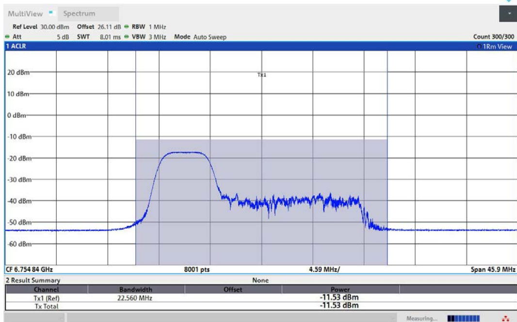
11AX80MIMO-Ant1-6785-52Tone-RU37-PASS
