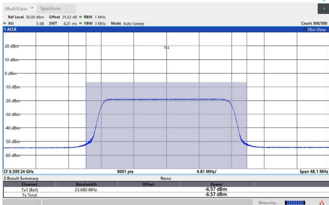
11AX80MIMO-Ant1-6625-242Tone-RU61-PASS
