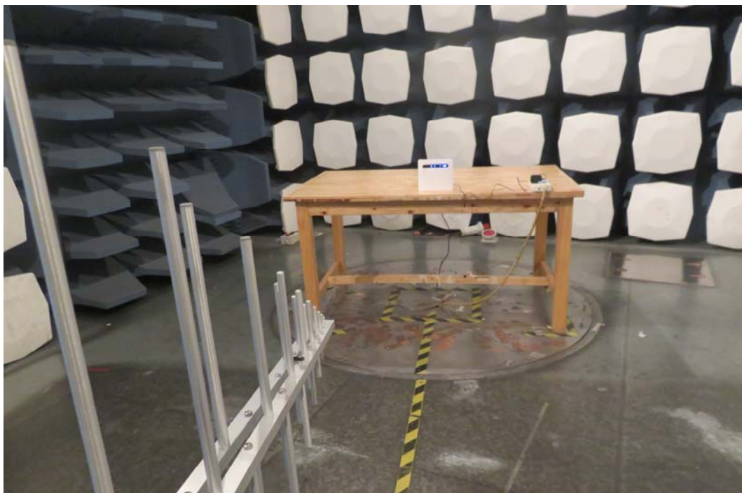
30M Hz-1GHz
