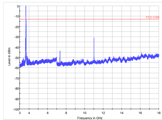
LTE Band 43 15MHz CH44340 3GHz~18GHz
