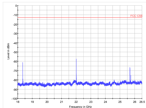
LTE Band 43 15MHz CH44340 18GHz~26.5GHz
