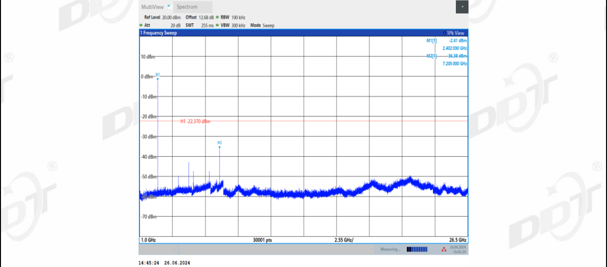
BLE_1M_Right side_2440_0~Reference
