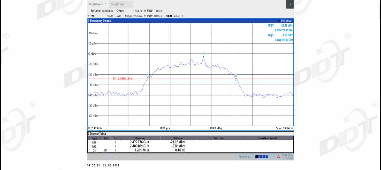
3DH5_Left side_2480
