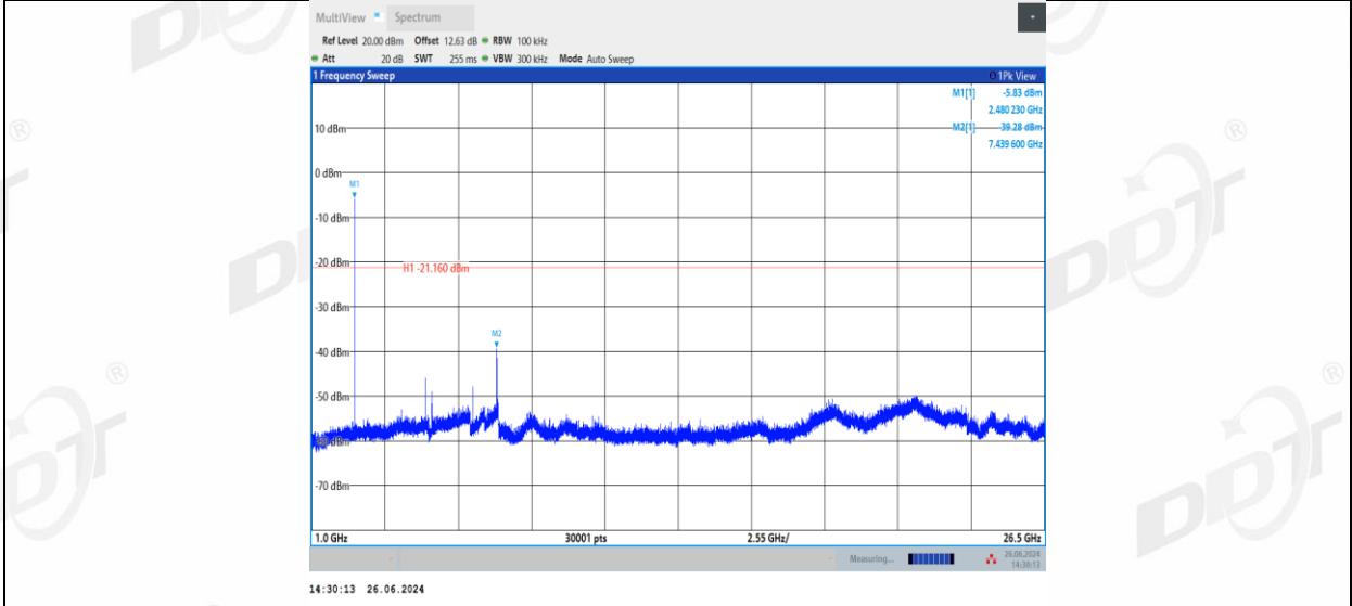
3DH5_Right side_2402_0~Reference
