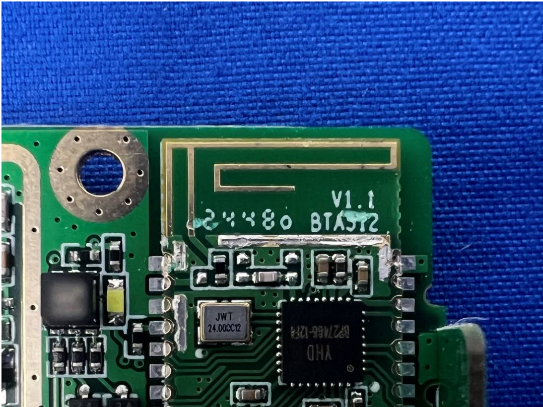
Bluetooth Antenna
