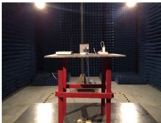
Above 1GHz
