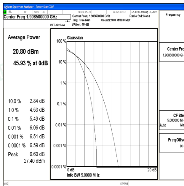
Band2-3MHz-16QAM-19185-15RB#0-PASS
