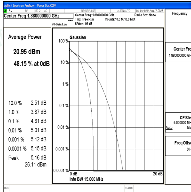
Band2-15MHz-QPSK-18900-1RB#0-PASS
