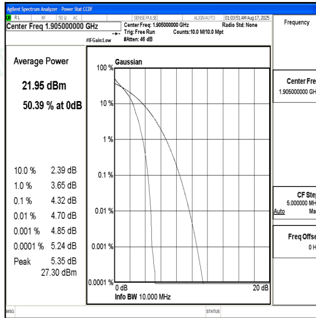
Band2-10MHz-QPSK-19150-1RB#0-PASS
