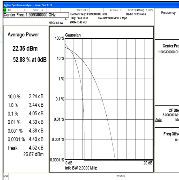
Band2-1.4MHz-QPSK-19193-1RB#0-PASS
