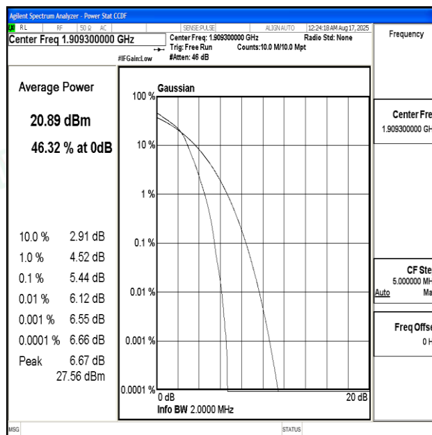
Band2-1.4MHz-16QAM-19193-6RB#0-PASS
