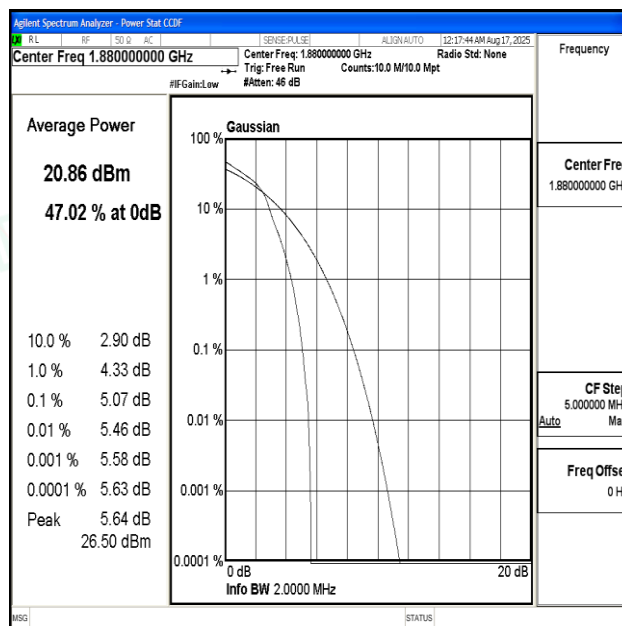
Band2-1.4MHz-16QAM-18900-1RB#0-PASS
