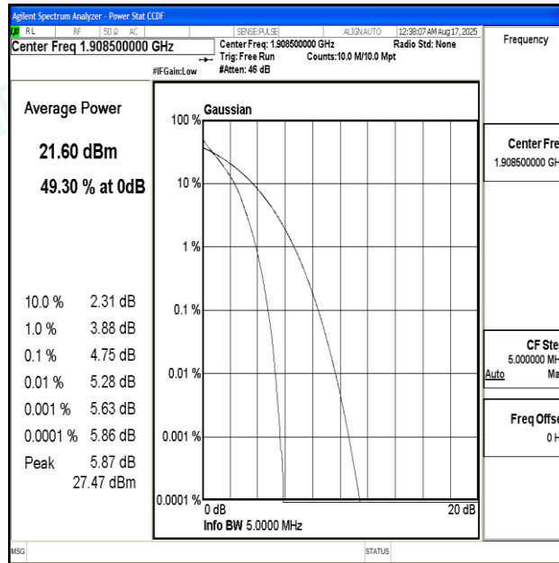
Band2-3MHz-QPSK-19185-15RB#0-PASS
