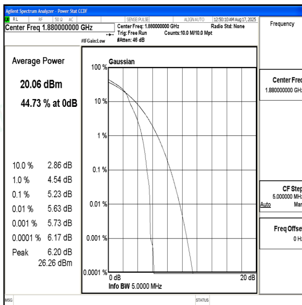
Band2-5MHz-16QAM-18900-1RB#0-PASS
