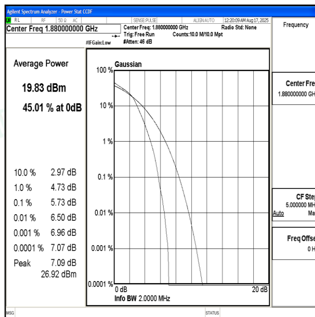
Band2-1.4MHz-16QAM-18900-6RB#0-PASS
