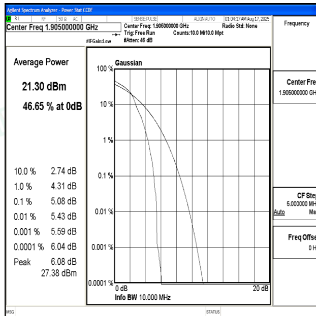
Band2-10MHz-16QAM-19150-1RB#0-PASS
