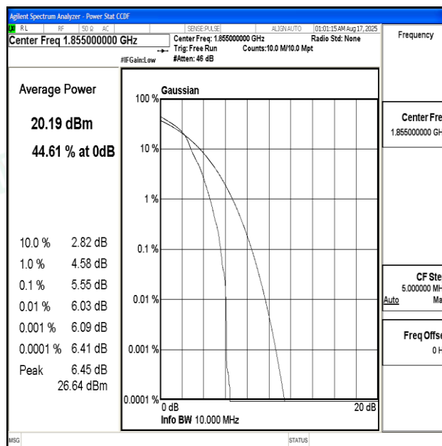
Band2-10MHz-16QAM-18650-1RB#0-PASS
