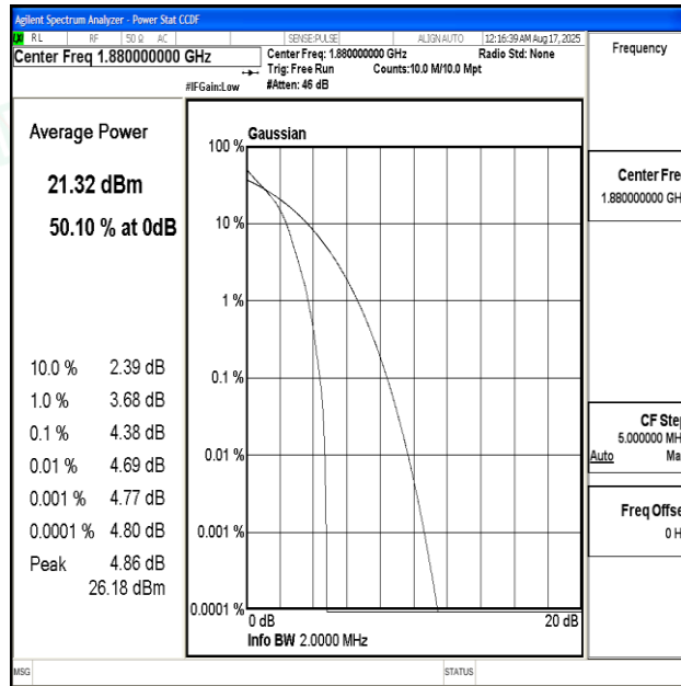
Band2-1.4MHz-QPSK-18900-1RB#0-PASS
