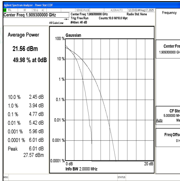
Band2-1.4MHz-QPSK-19193-6RB#0-PASS
