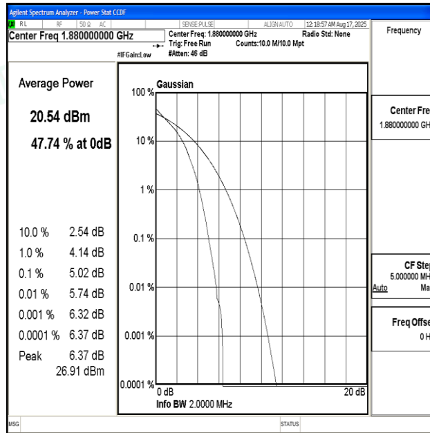
Band2-1.4MHz-QPSK-18900-6RB#0-PASS
