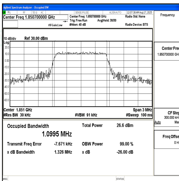
Band2-1.4MHz-16QAM-18607-6RB#0-PASS
