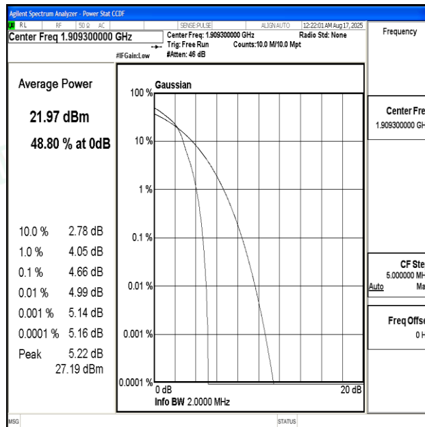
Band2-1.4MHz-16QAM-19193-1RB#0-PASS
