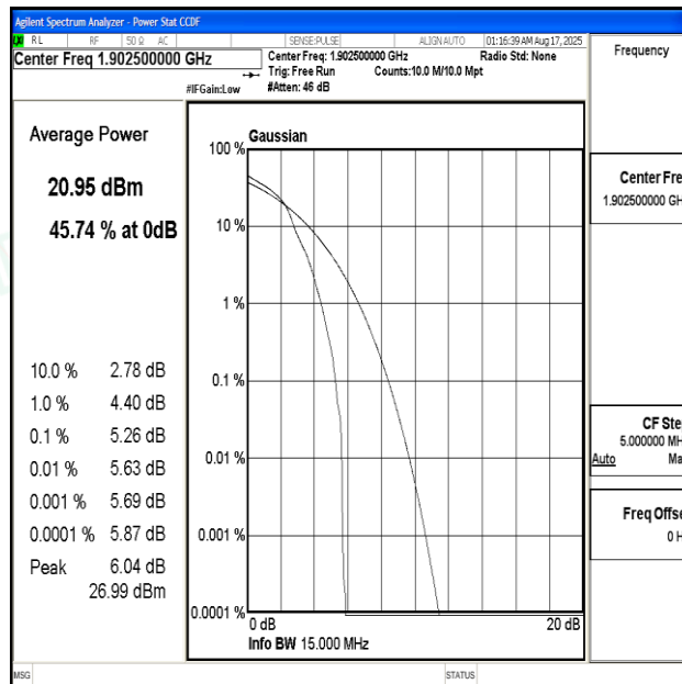
Band2-15MHz-16QAM-19125-1RB#0-PASS
