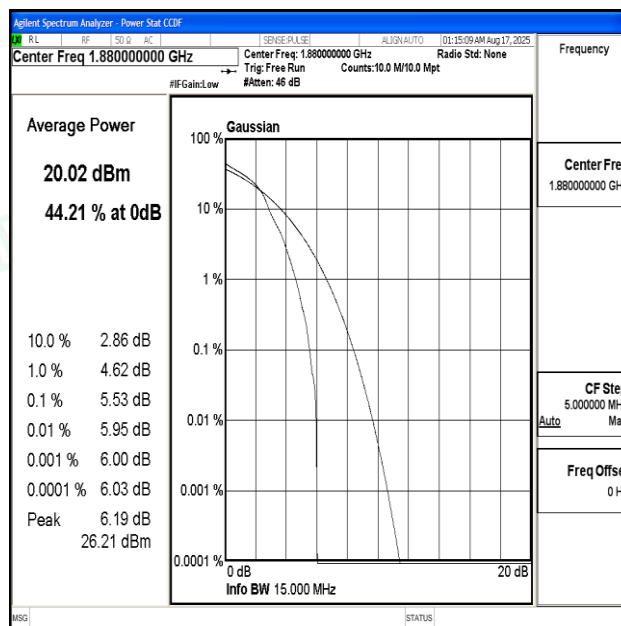
Band2-15MHz-16QAM-18900-1RB#0-PASS
