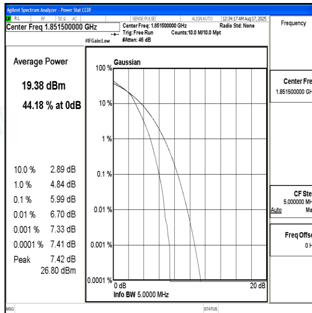
Band2-3MHz-16QAM-18615-15RB#0-PASS
