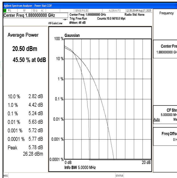
Band2-3MHz-16QAM-18900-1RB#0-PASS
