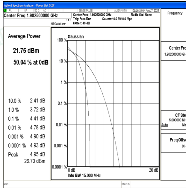
Band2-15MHz-QPSK-19125-1RB#0-PASS
