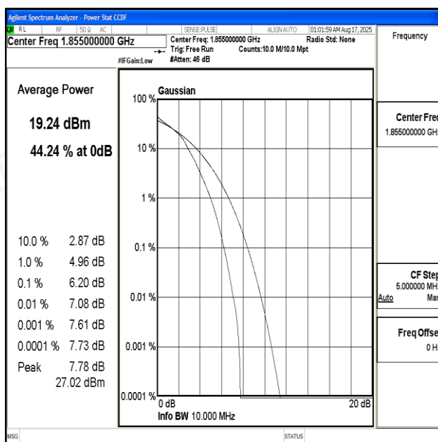
Band2-10MHz-16QAM-18650-50RB#0-PASS
