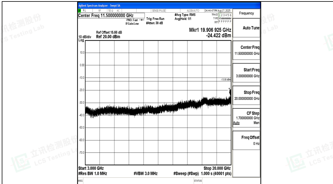
Band2_3MHz_QPSK_19185_1RB#0_3000~20000_3000~20000
