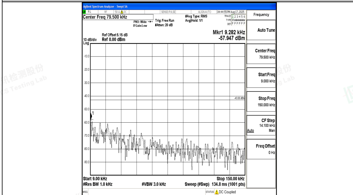
Band2_3MHz_16QAM_19185_1RB#0_0.009~0.15_0.009~0.15
