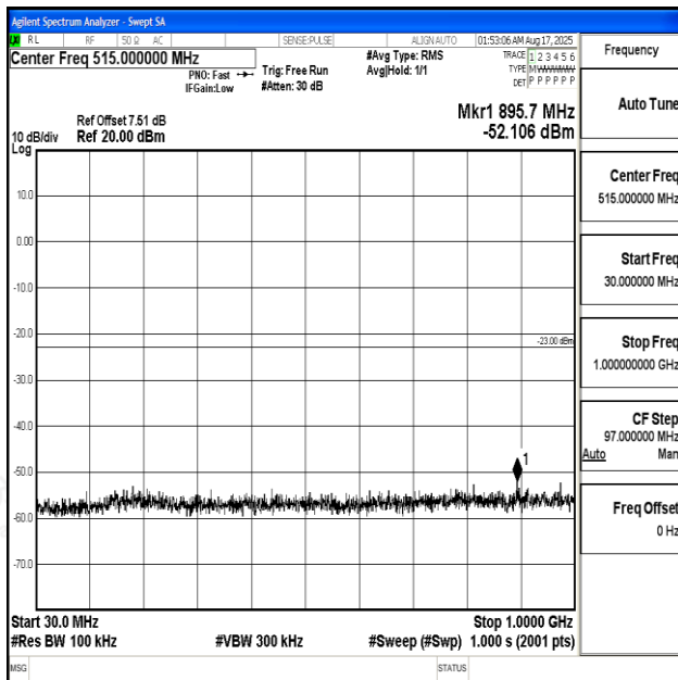
Band2_10MHz_QPSK_18650_1RB#0_30~1000_30~1000
