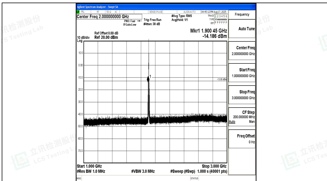
Band2_3MHz_16QAM_19185_1RB#0_1000~3000_1000~3000
