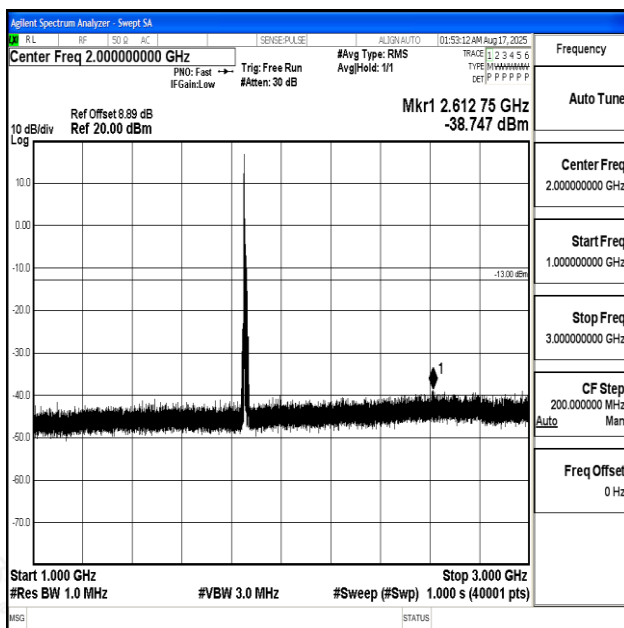
Band2_10MHz_QPSK_18650_1RB#0_1000~3000_1000~3000
