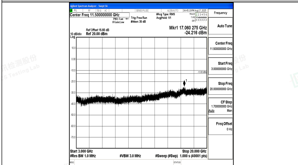
Band2_3MHz_16QAM_19185_1RB#0_3000~20000_3000~20000
