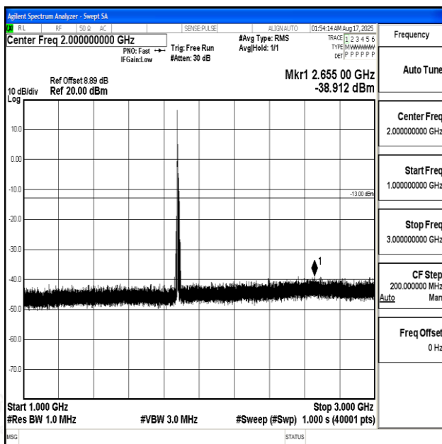
Band2_10MHz_QPSK_18900_1RB#0_1000~3000_1000~3000
