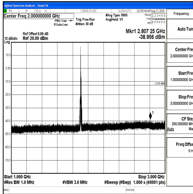
Band2_10MHz_16QAM_19150_1RB#0_1000~3000_1000~3000
