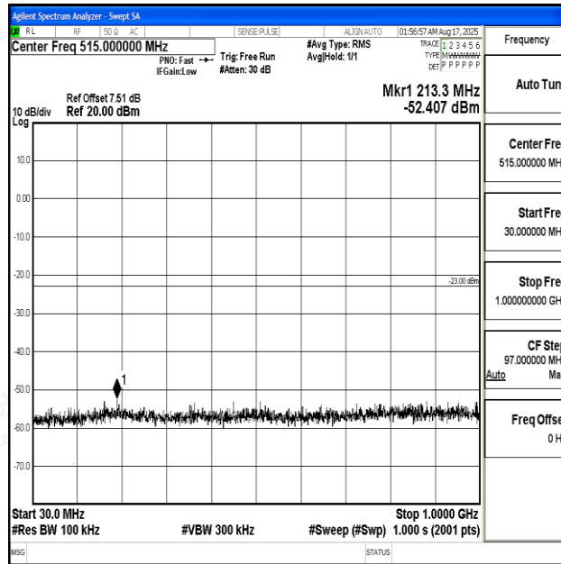
Band2_15MHz_QPSK_18675_1RB#0_30~1000_30~1000
