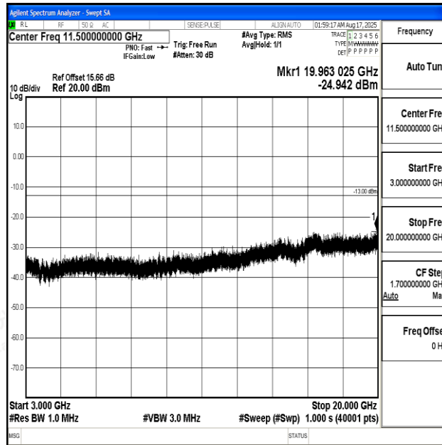
Band2_15MHz_QPSK_19125_1RB#0_3000~20000_3000~20000
