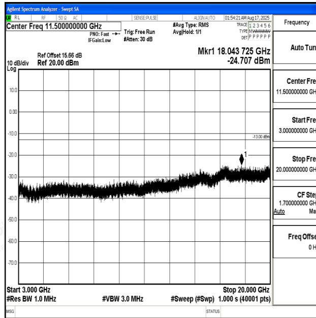
Band2_10MHz_QPSK_18900_1RB#0_3000~20000_3000~20000
