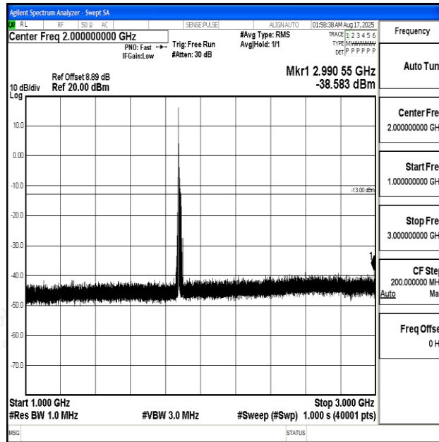
Band2_15MHz_16QAM_18900_1RB#0_1000~3000_1000~3000
