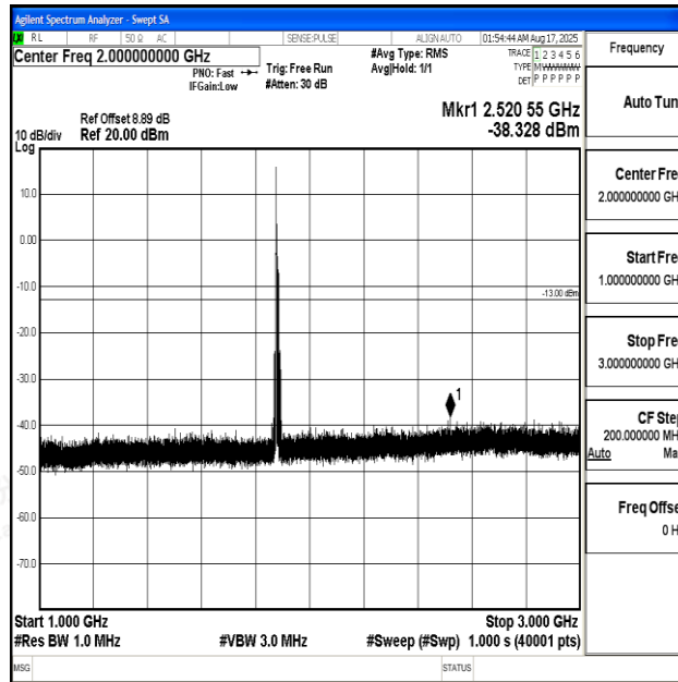
Band2_10MHz_16QAM_18900_1RB#0_1000~3000_1000~3000
