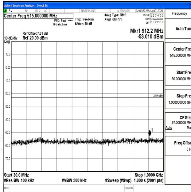
Band2_20MHz_QPSK_19100_1RB#0_30~1000_30~1000
