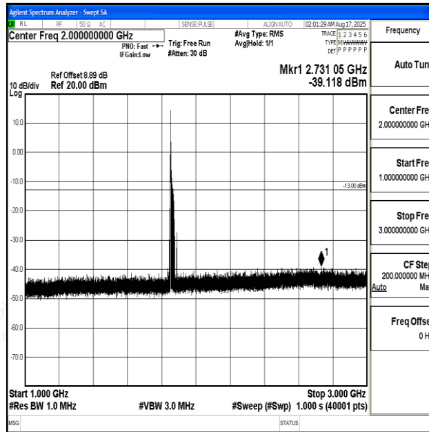
Band2_20MHz_16QAM_18700_1RB#0_1000~3000_1000~3000
