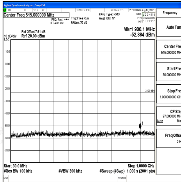
Band2_15MHz_QPSK_18900_1RB#0_30~1000_30~1000
