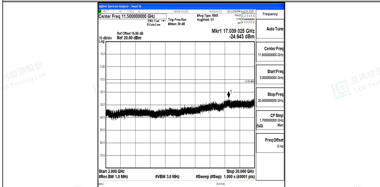
Band4_3MHz_QPSK_20385_1RB#0_3000~20000_3000~20000
