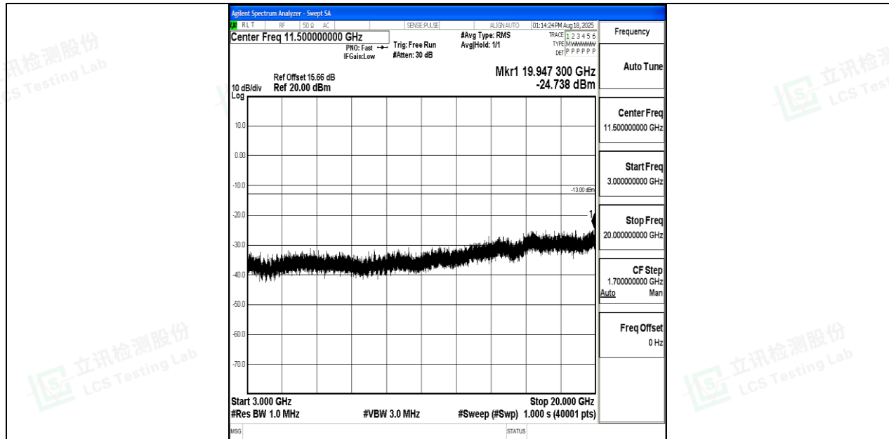
Band4_3MHz_16QAM_20385_1RB#0_3000~20000_3000~20000
