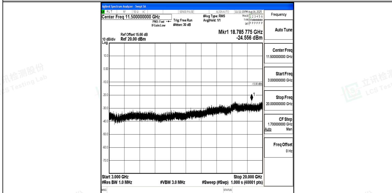
Band4_10MHz_QPSK_20350_1RB#0_3000~20000_3000~20000
