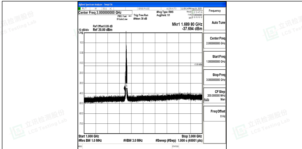
Band4_10MHz_QPSK_20000_1RB#0_1000~3000_1000~3000
