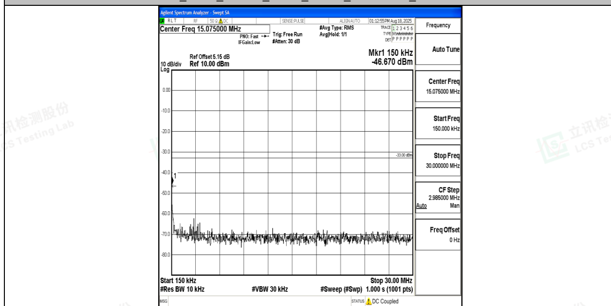
Band4_3MHz_16QAM_20175_1RB#0_0.15~30_0.15~30
