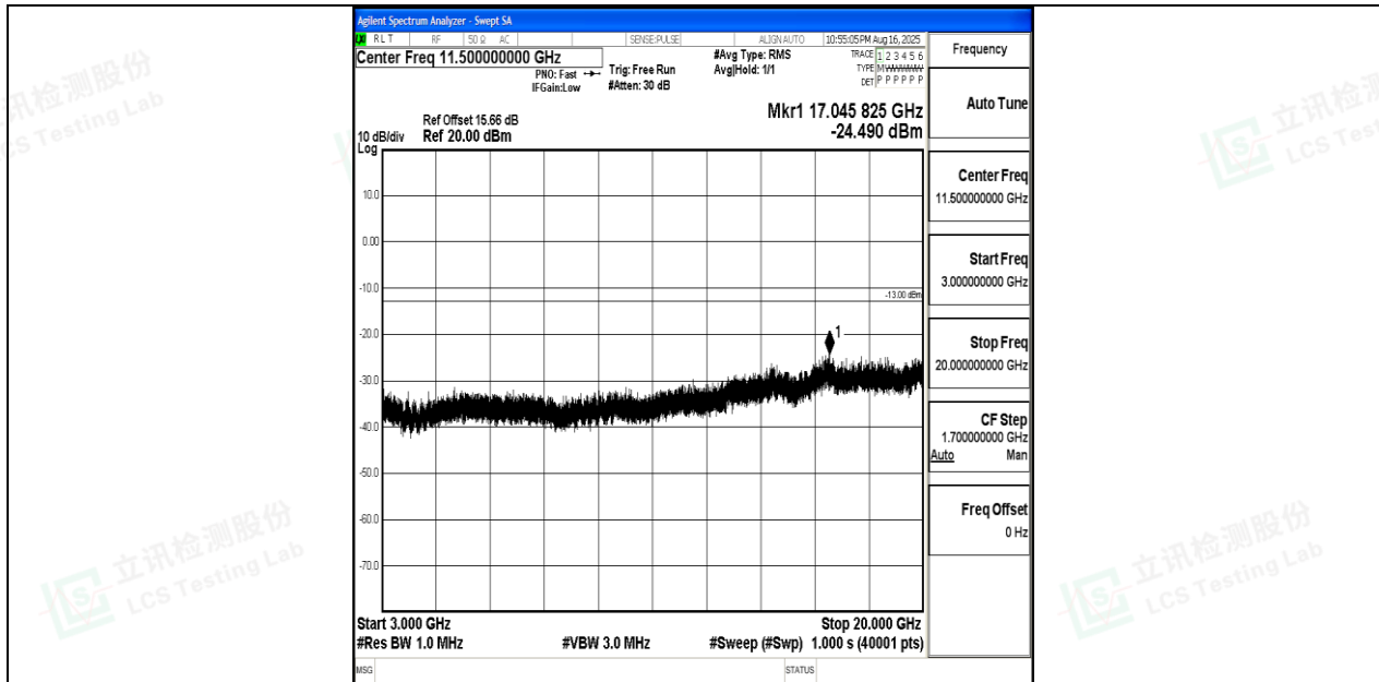
Band4_5MHz_16QAM_20375_1RB#0_3000~20000_3000~20000
