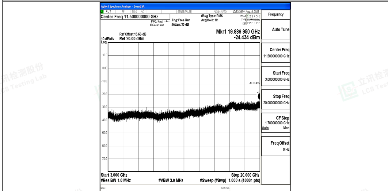
Band4_5MHz_QPSK_20175_1RB#0_3000~20000_3000~20000
