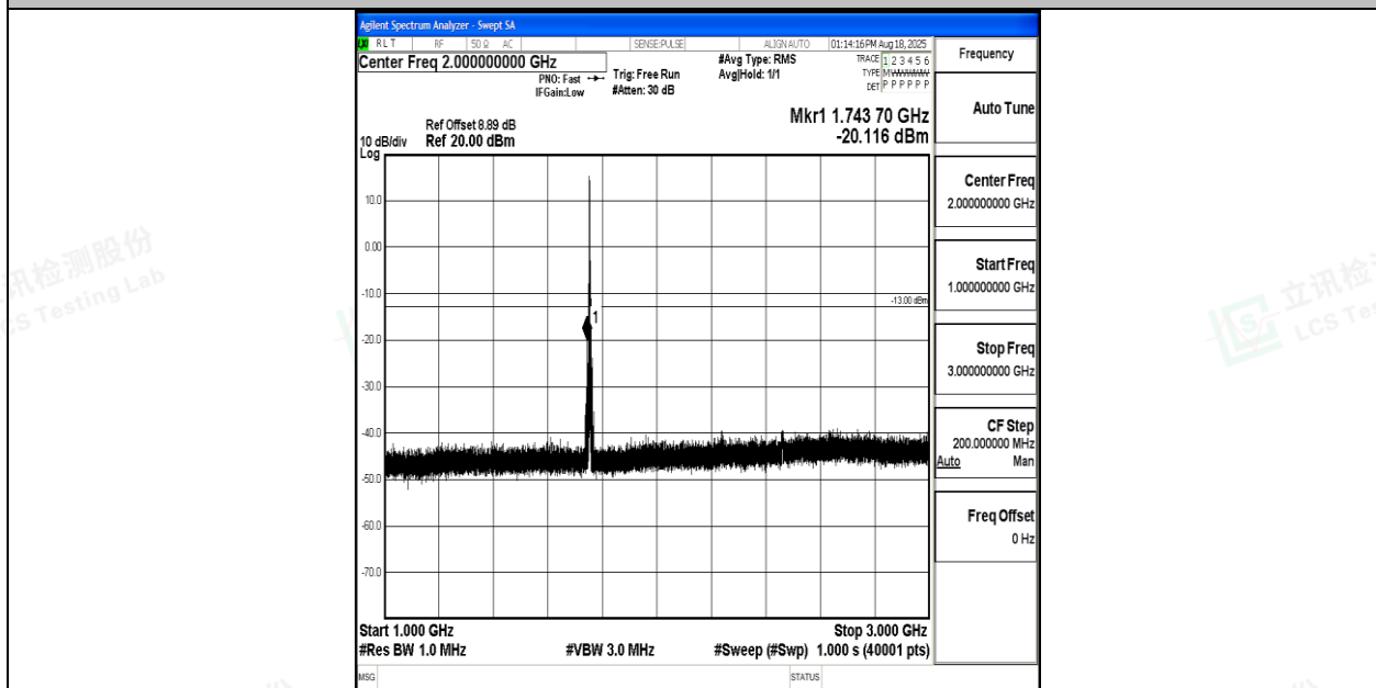
Band4_3MHz_16QAM_20385_1RB#0_1000~3000_1000~3000
