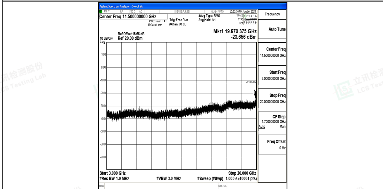
Band4_5MHz_QPSK_19975_1RB#0_3000~20000_3000~20000
