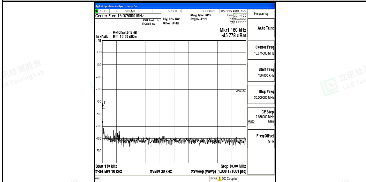
Band4_5MHz_QPSK_19975_1RB#0_0.15~30_0.15~30
