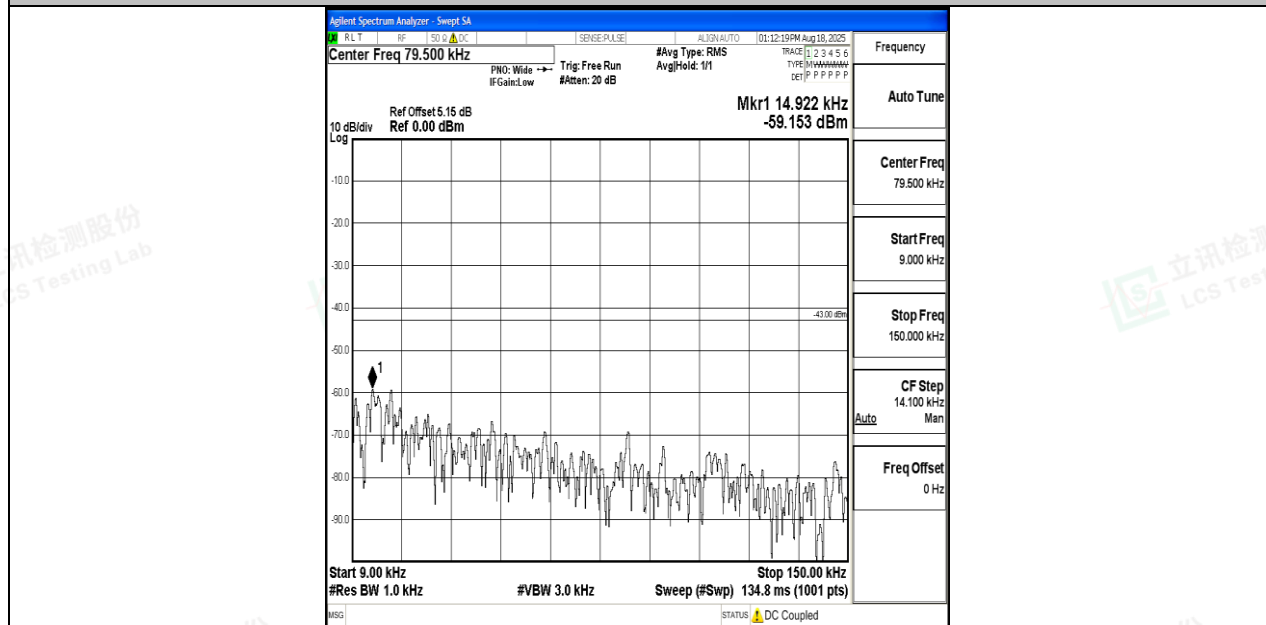
Band4_3MHz_QPSK_20175_1RB#0_0.009~0.15_0.009~0.15
