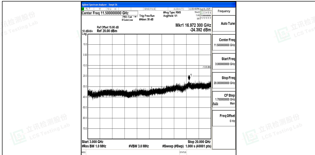
Band4_10MHz_16QAM_20000_1RB#0_3000~20000_3000~20000
