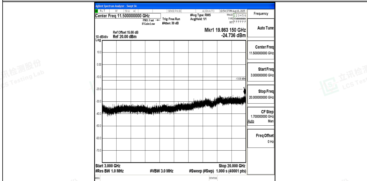
Band4_5MHz_QPSK_20375_1RB#0_3000~20000_3000~20000
