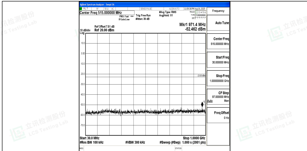
Band4_10MHz_16QAM_20000_1RB#0_30~1000_30~1000
