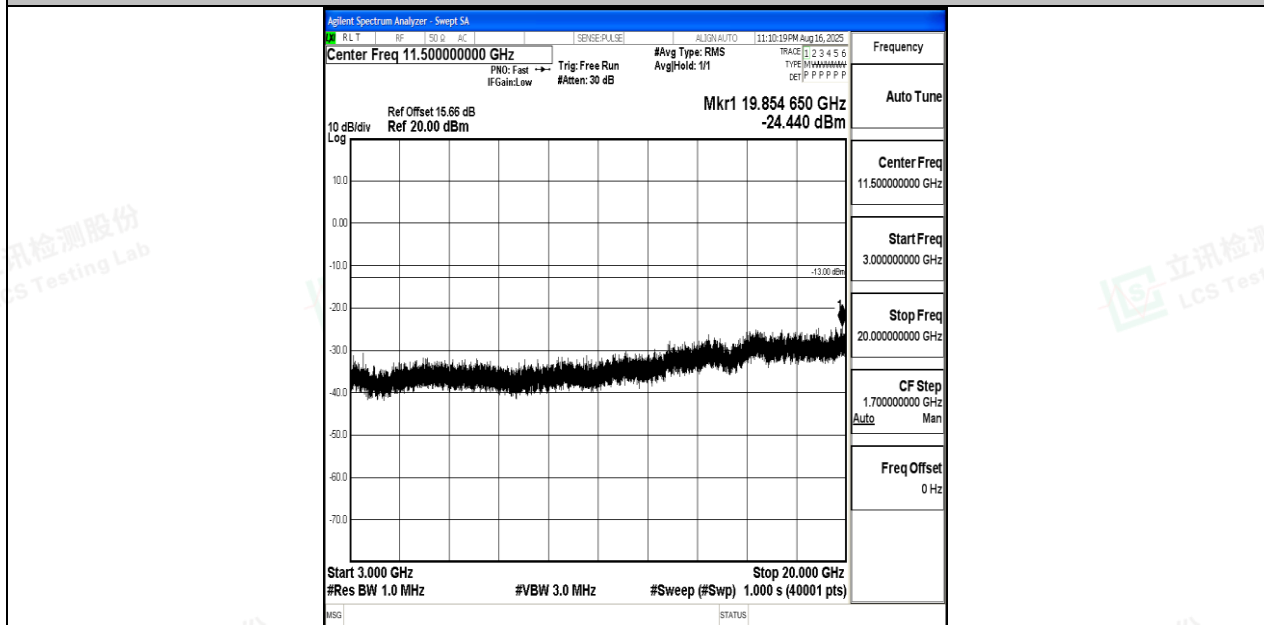
Band4_10MHz_QPSK_20175_1RB#0_3000~20000_3000~20000
