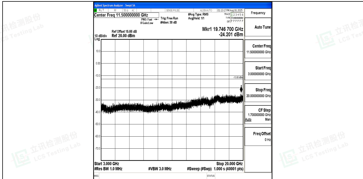
Band4_3MHz_16QAM_20175_1RB#0_3000~20000_3000~20000
