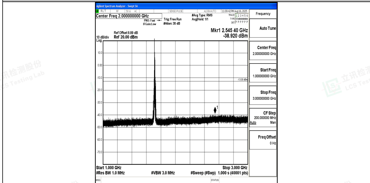
Band4_10MHz_16QAM_20000_1RB#0_1000~3000_1000~3000
