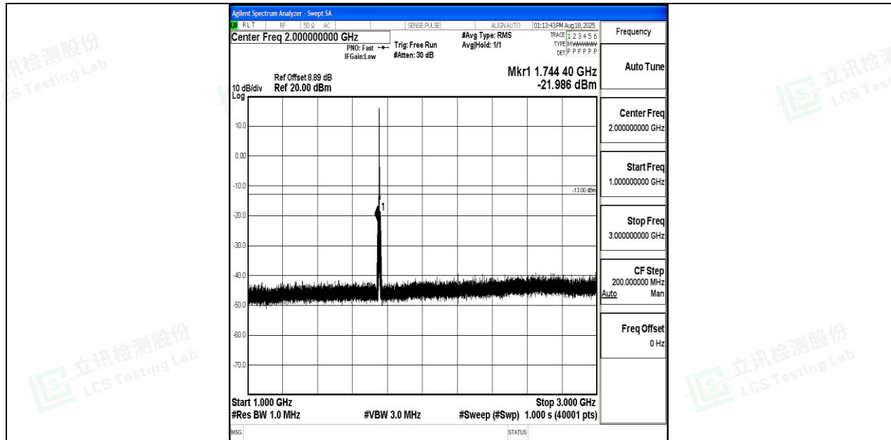
Band4_3MHz_QPSK_20385_1RB#0_1000~3000_1000~3000
