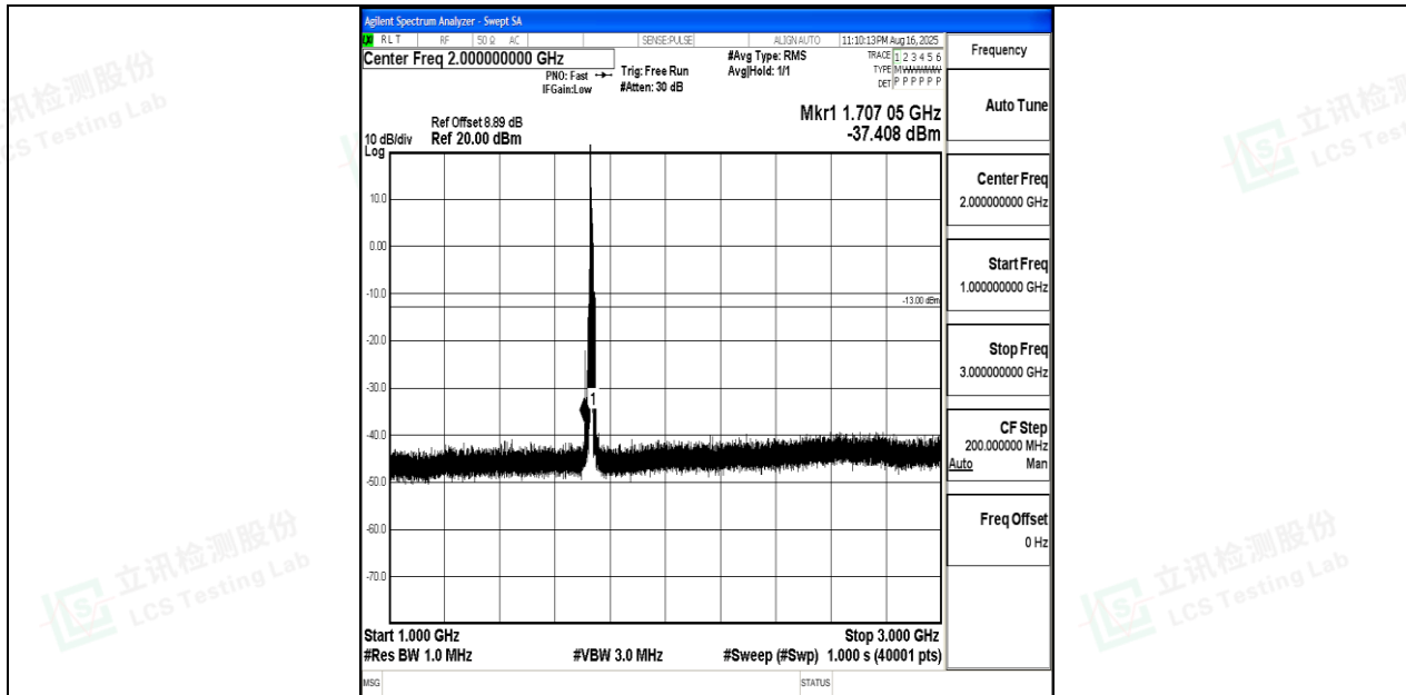
Band4_10MHz_QPSK_20175_1RB#0_1000~3000_1000~3000
