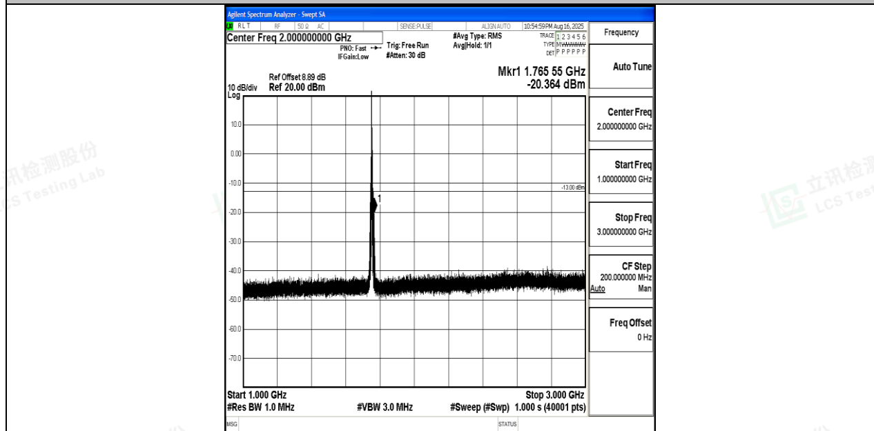
Band4_5MHz_16QAM_20375_1RB#0_1000~3000_1000~3000
