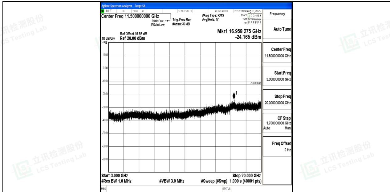
Band4_3MHz_16QAM_19965_1RB#0_3000~20000_3000~20000
