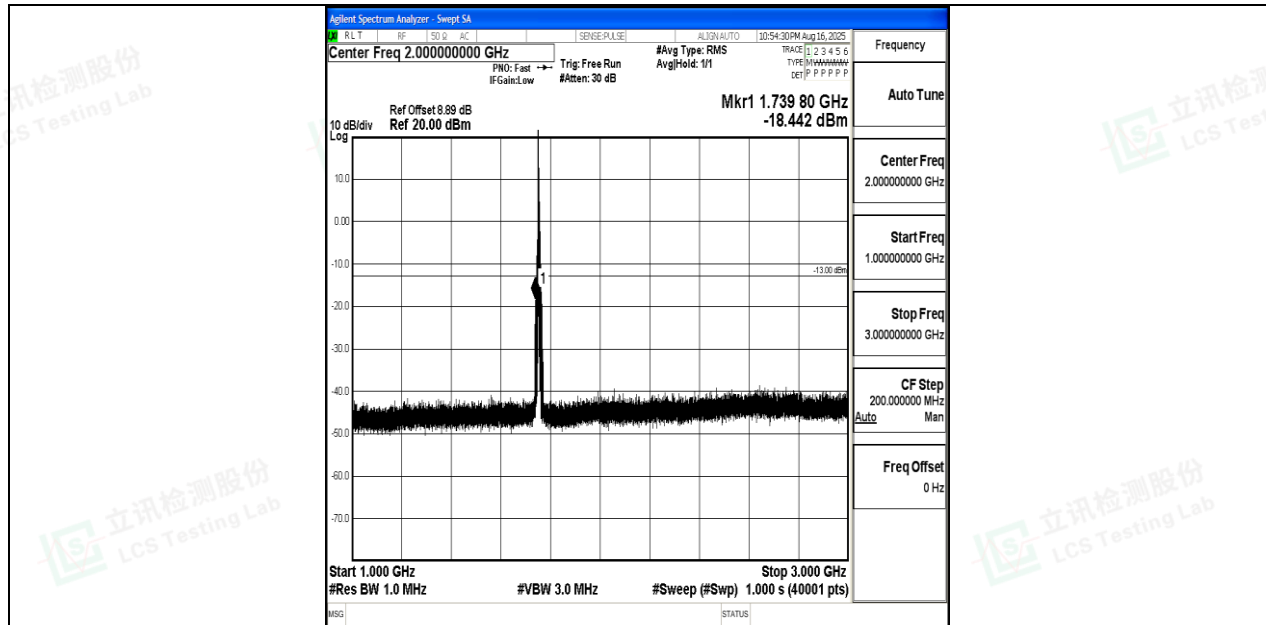
Band4_5MHz_QPSK_20375_1RB#0_1000~3000_1000~3000
