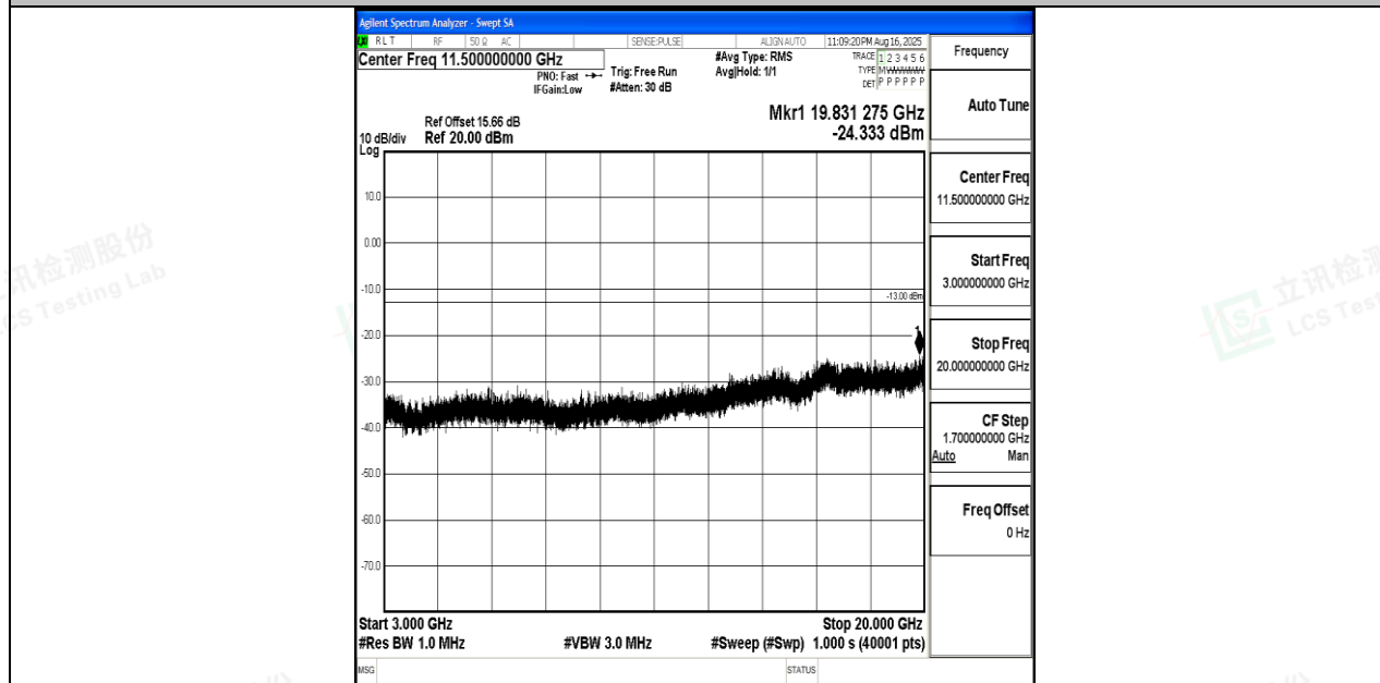
Band4_10MHz_QPSK_20000_1RB#0_3000~20000_3000~20000
