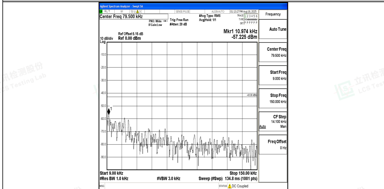
Band4_3MHz_QPSK_20385_1RB#0_0.009~0.15_0.009~0.15
