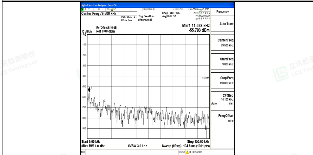
Band4_10MHz_QPSK_20175_1RB#0_0.009~0.15_0.009~0.15
