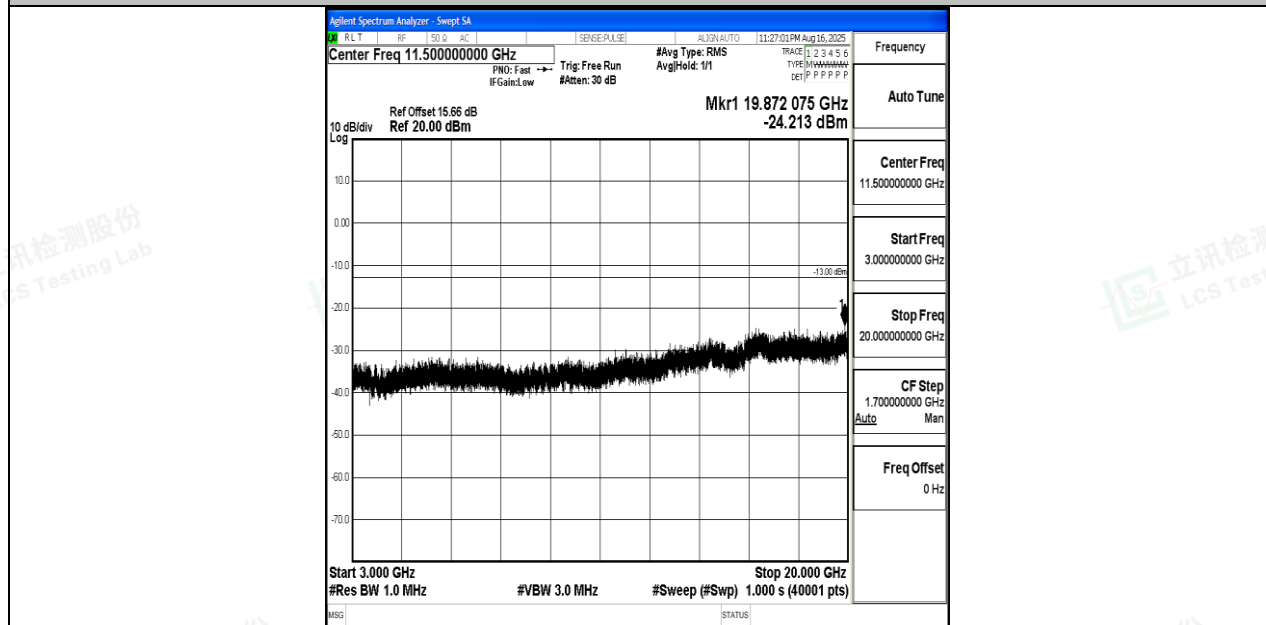
Band4_15MHz_QPSK_20325_1RB#0_3000~20000_3000~20000
