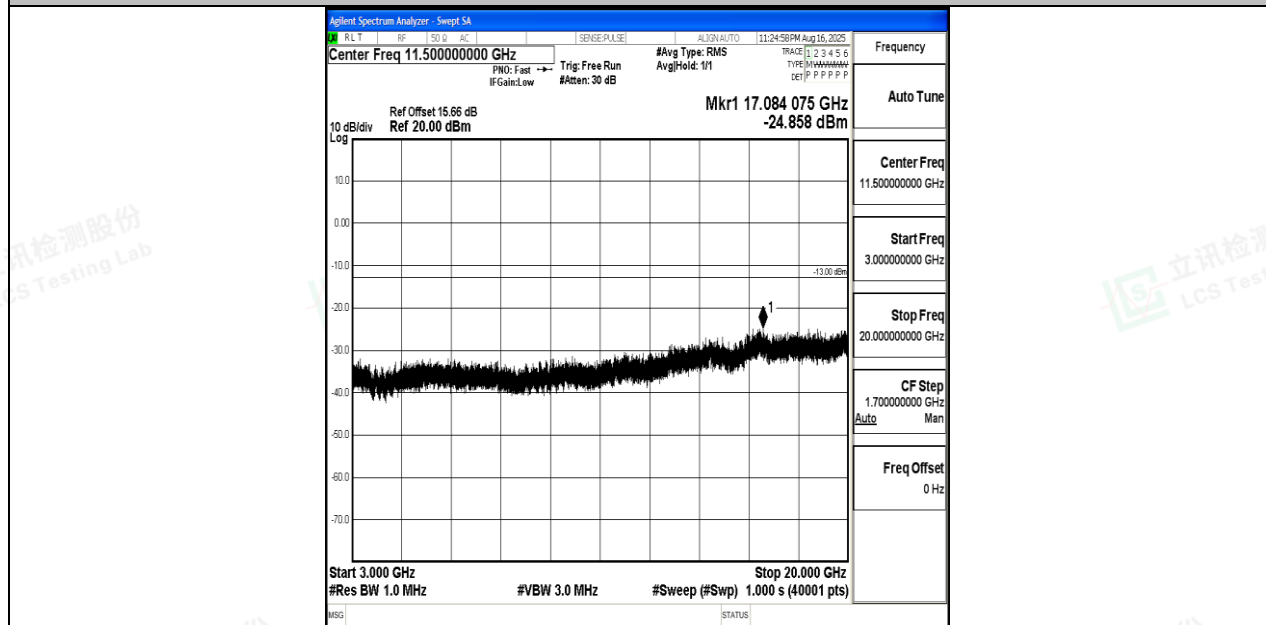
Band4_15MHz_QPSK_20025_1RB#0_3000~20000_3000~20000
