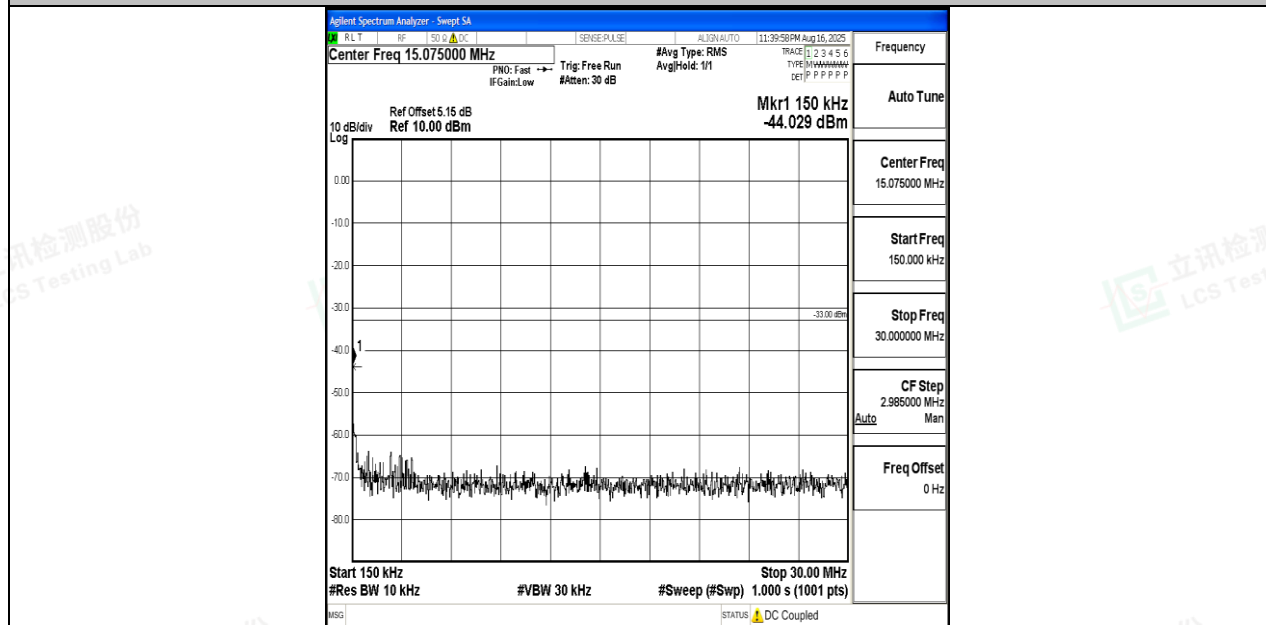
Band4_20MHz_16QAM_20050_1RB#0_0.15~30_0.15~30
