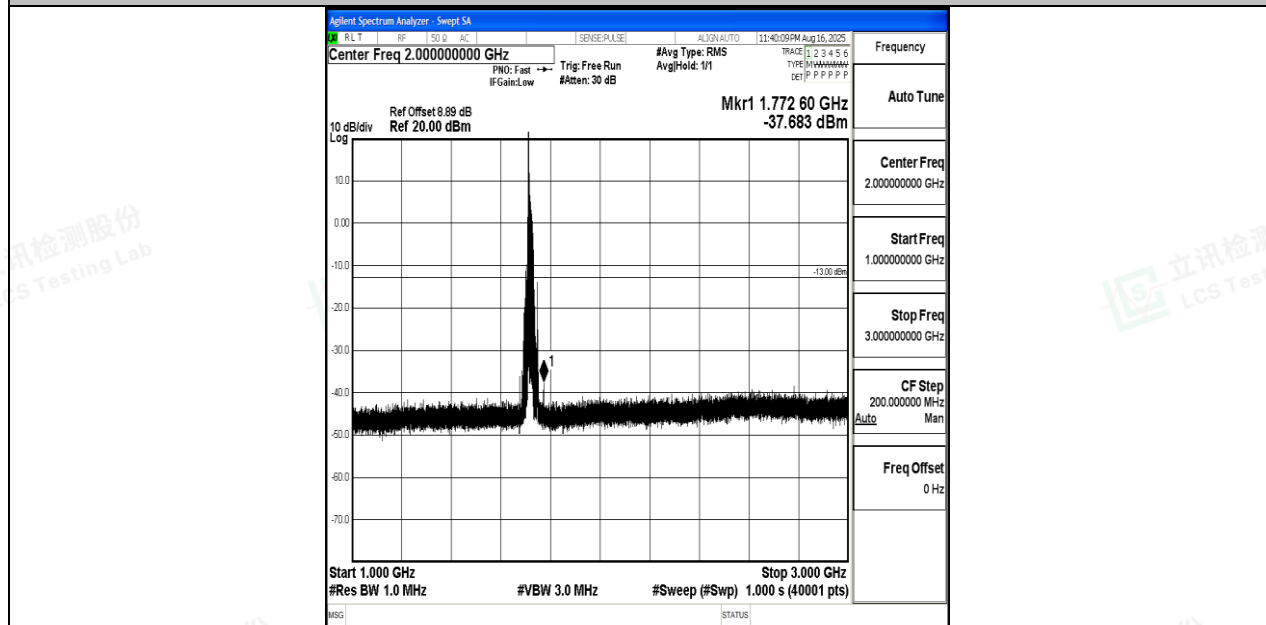
Band4_20MHz_16QAM_20050_1RB#0_1000~3000_1000~3000
