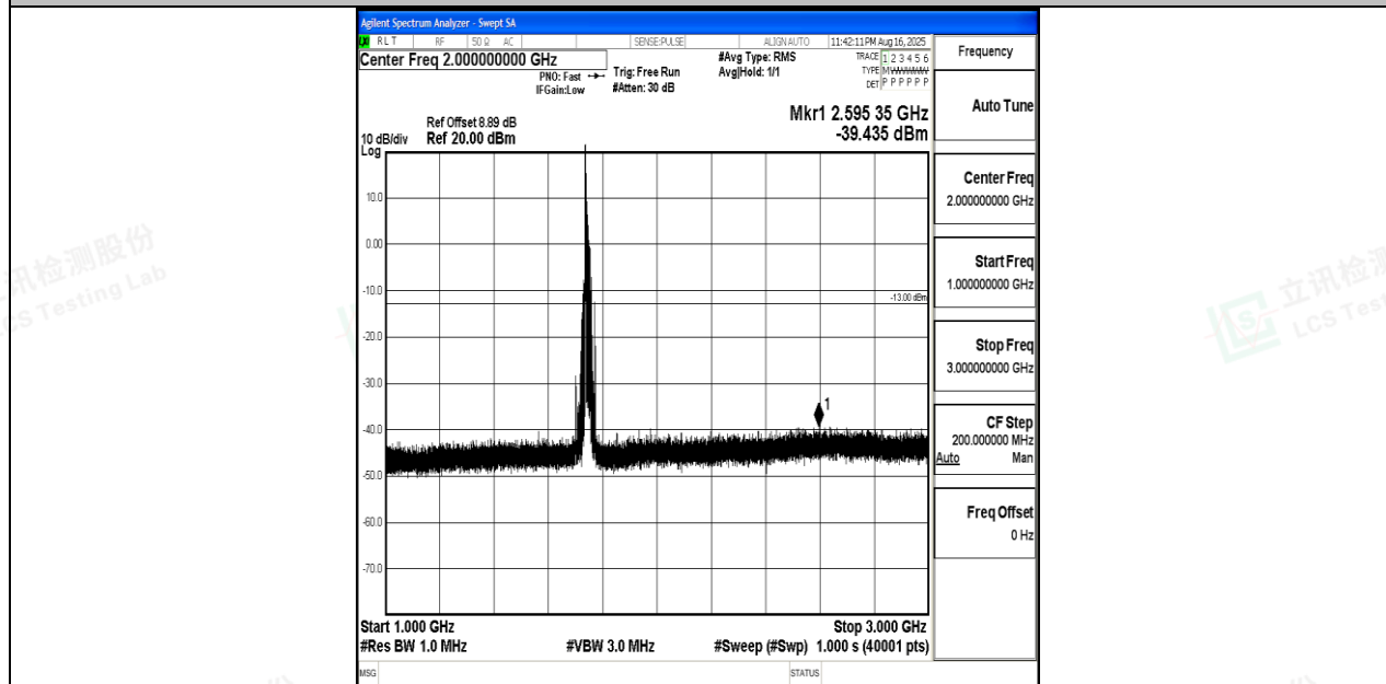
Band4_20MHz_16QAM_20300_1RB#0_1000~3000_1000~3000
