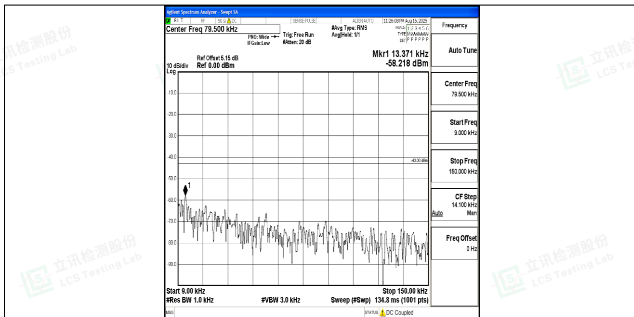
Band4 15MHz 16QAM 20175 1RB#0 0.009~0.15 0.009~0.15
