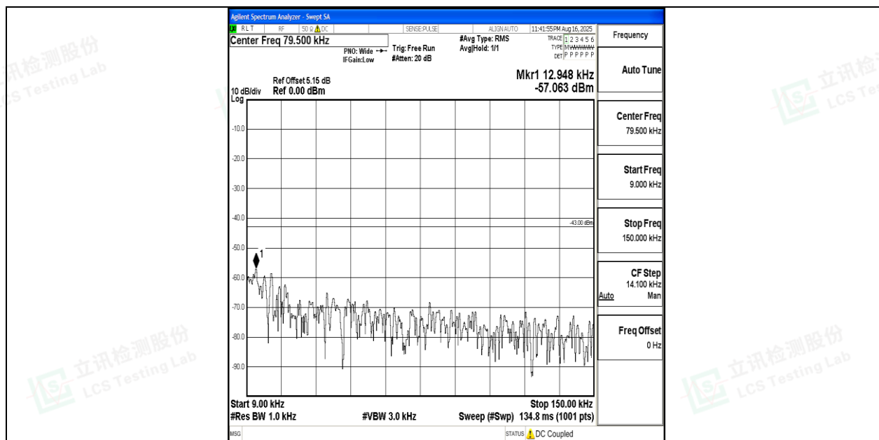
Band4_20MHz_16QAM_20300_1RB#0_0.009~0.15_0.009~0.15
