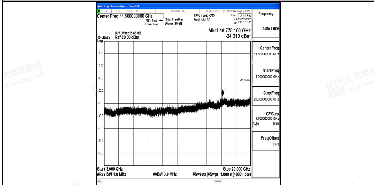
Band4_15MHz_QPSK_20175_1RB#0_3000~20000_3000~20000
