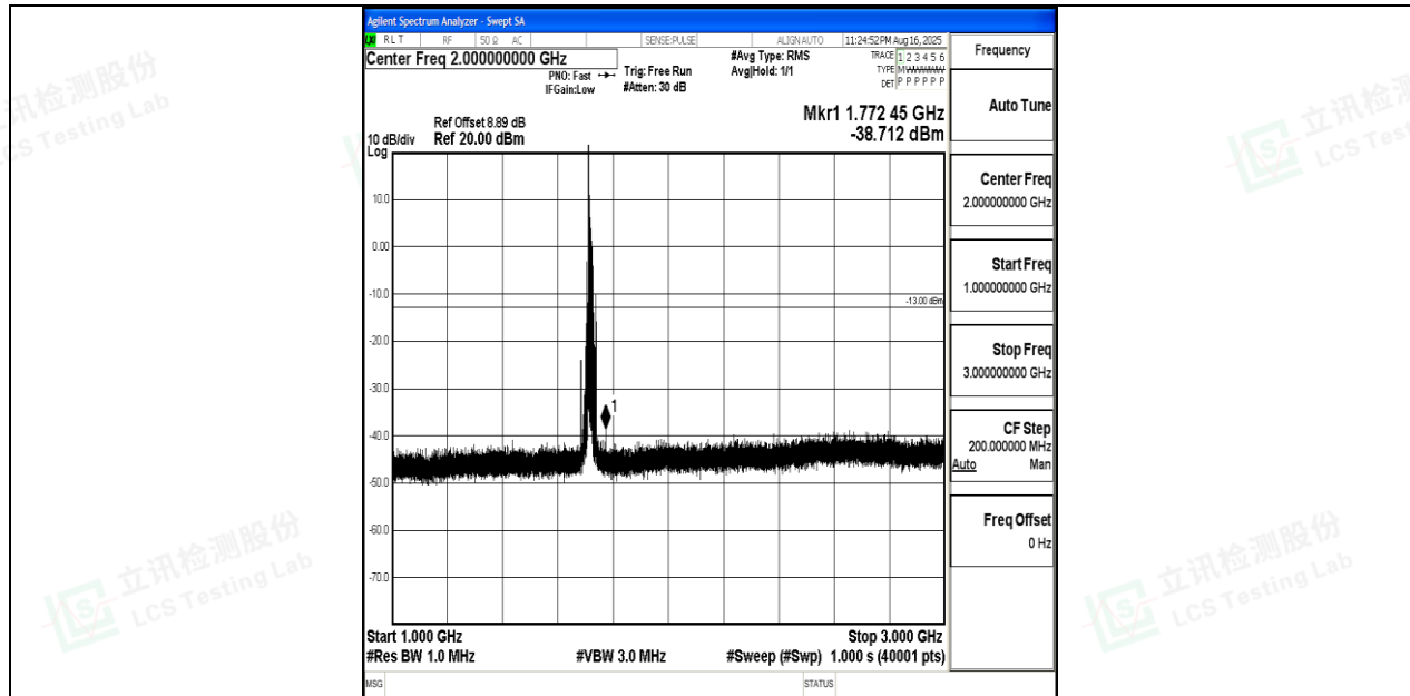
Band4_15MHz_QPSK_20025_1RB#0_1000~3000_1000~3000
