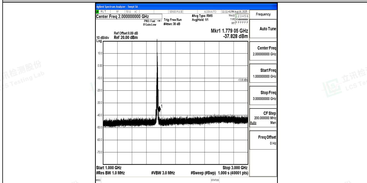
Band4_10MHz_16QAM_20350_1RB#0_1000~3000_1000~3000
