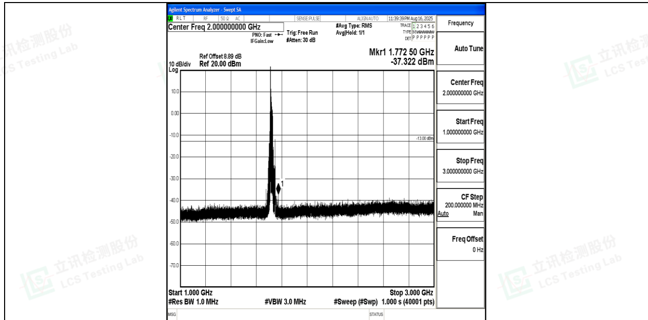
Band4_20MHz_QPSK_20050_1RB#0_1000~3000_1000~3000
