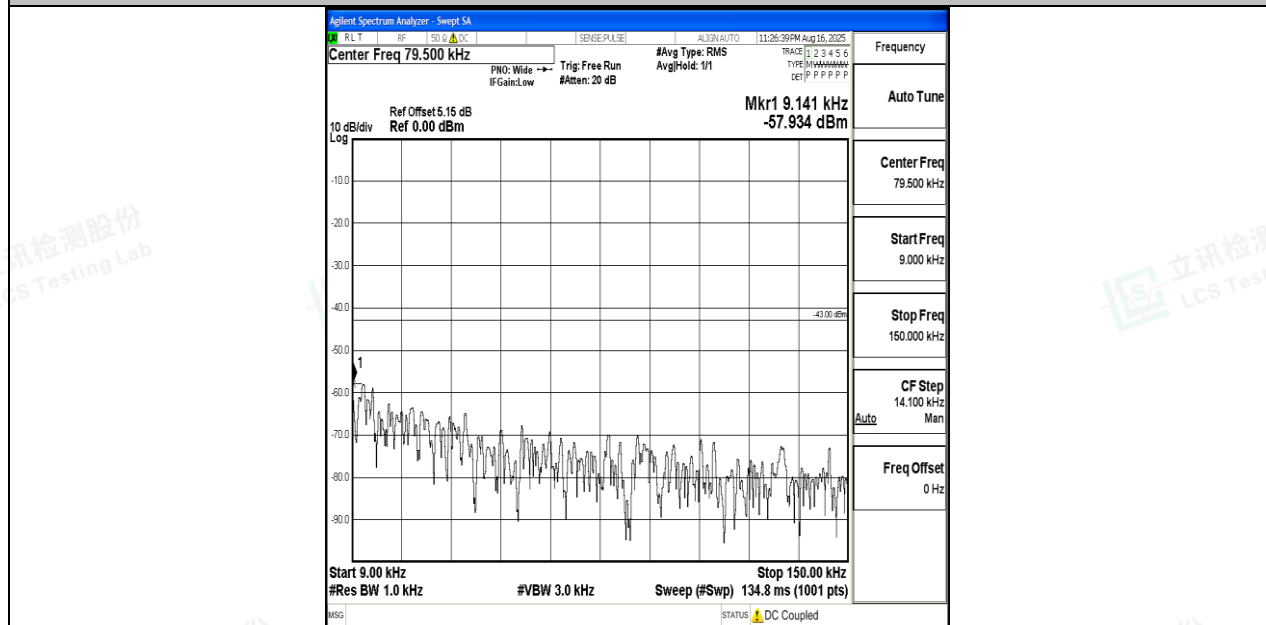
Band4_15MHz_QPSK_20325_1RB#0_0.009~0.15_0.009~0.15
