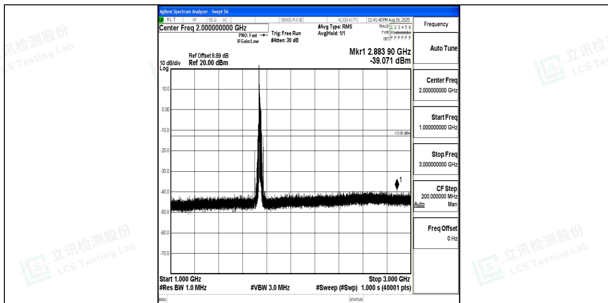
Band4_20MHz_QPSK_20300_1RB#0_1000~3000_1000~3000
