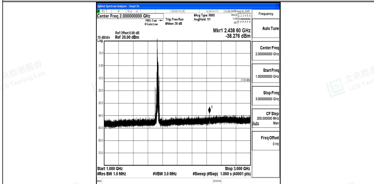
Band4_15MHz_16QAM_20175_1RB#0_1000~3000_1000~3000
