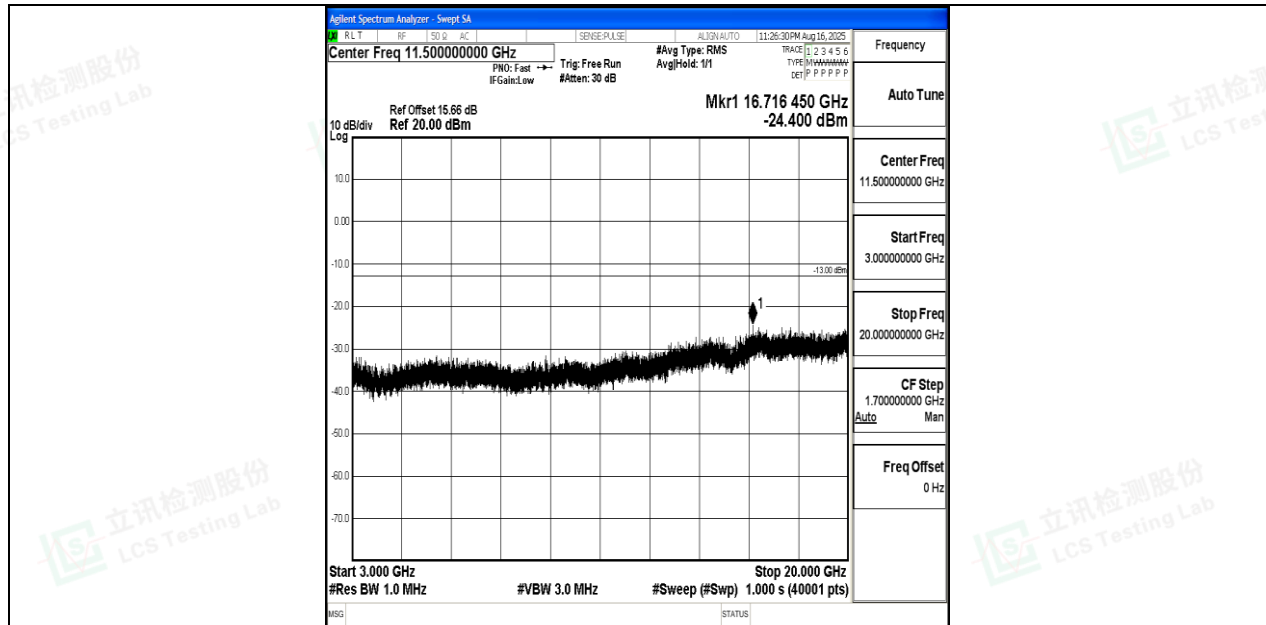
Band4_15MHz_16QAM_20175_1RB#0_3000~20000_3000~20000
