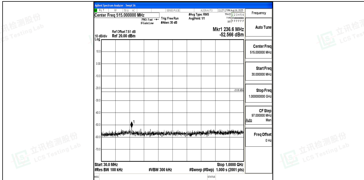
Band4_15MHz_16QAM_20325_1RB#0_30~1000_30~1000
