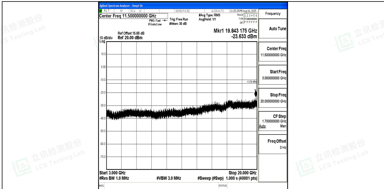
Band4_15MHz_16QAM_20025_1RB#0_3000~20000_3000~20000
