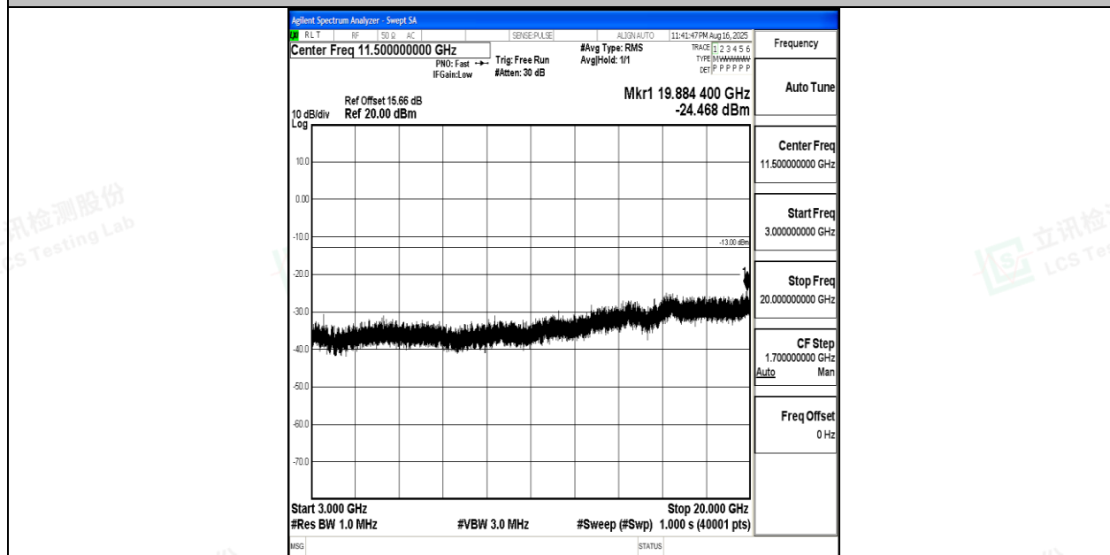
Band4_20MHz_QPSK_20300_1RB#0_3000~20000_3000~20000
