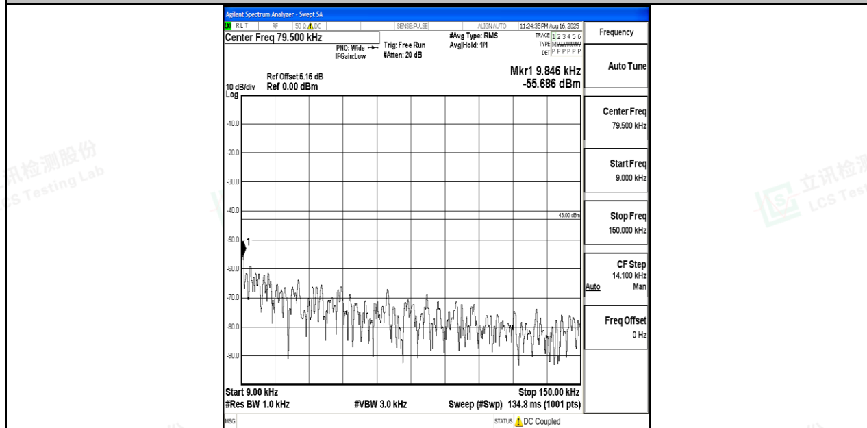
Band4_15MHz_QPSK_20025_1RB#0_0.009~0.15_0.009~0.15
