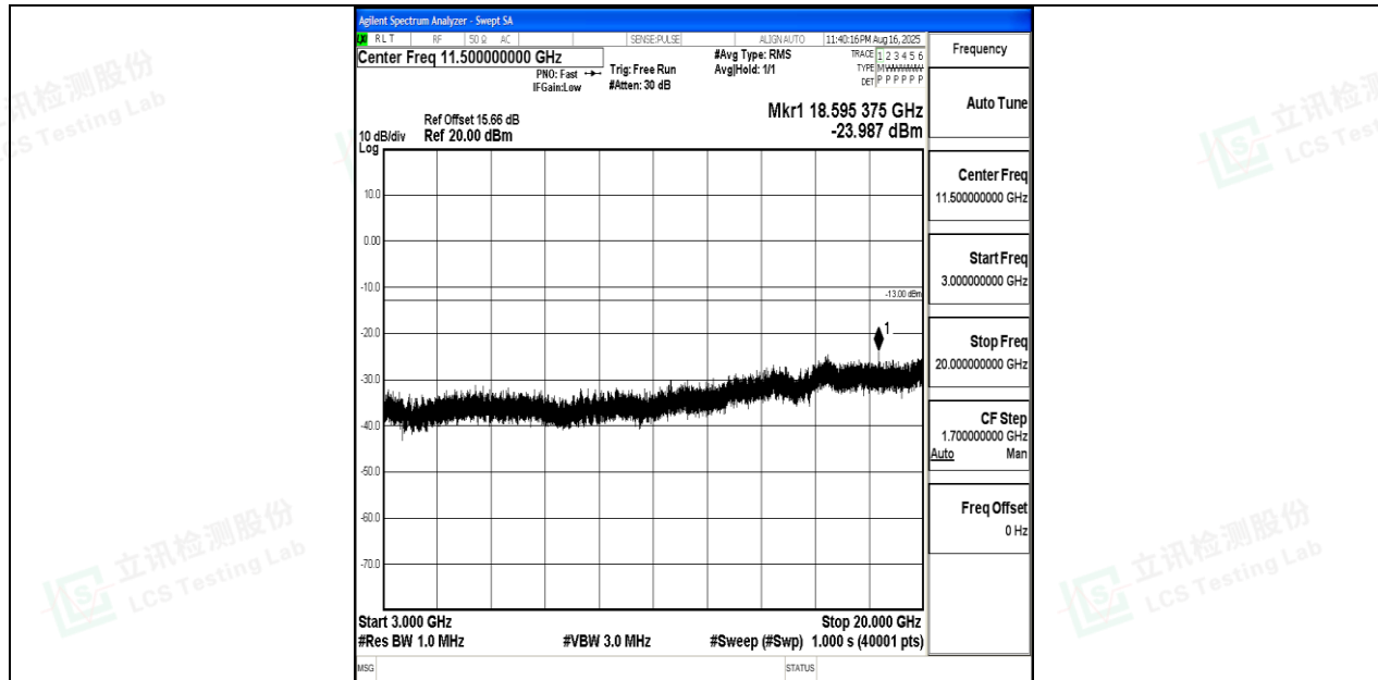
Band4_20MHz_16QAM_20050_1RB#0_3000~20000_3000~20000
