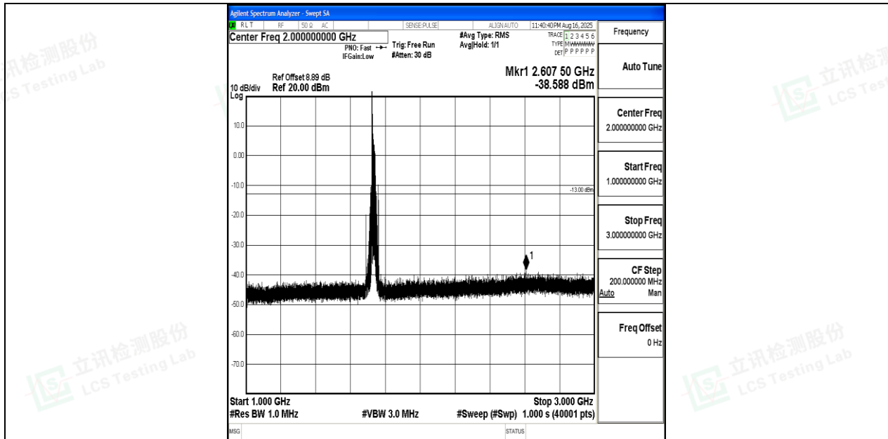
Band4_20MHz_QPSK_20175_1RB#0_1000~3000_1000~3000
