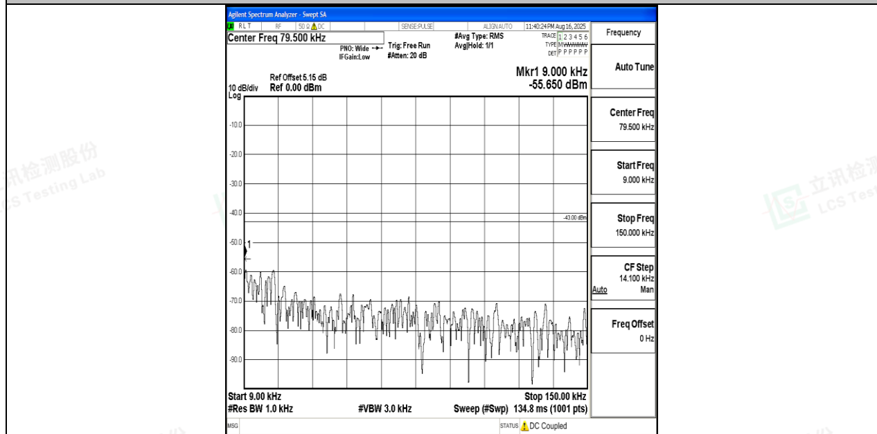
Band4_20MHz_QPSK_20175_1RB#0_0.009~0.15_0.009~0.15
