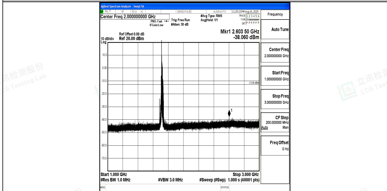
Band4_15MHz_16QAM_20025_1RB#0_1000~3000_1000~3000
