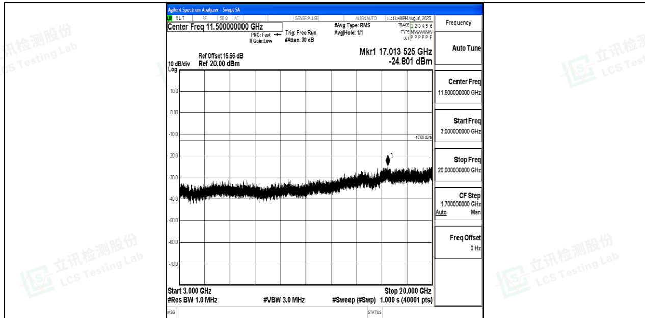
Band4_10MHz_16QAM_20350_1RB#0_3000~20000_3000~20000
