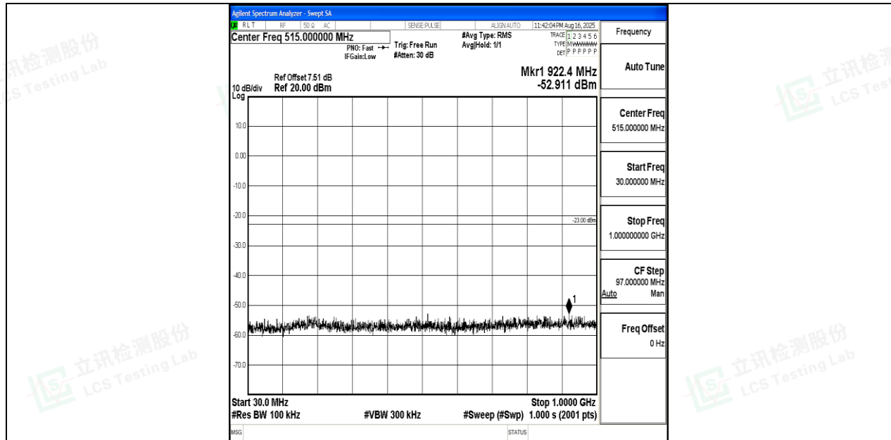
Band4_20MHz_16QAM_20300_1RB#0_30~1000_30~1000
