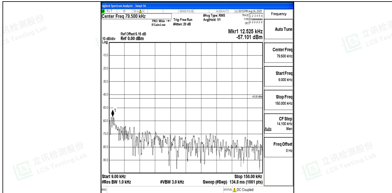
Band4_20MHz_16QAM_20050_1RB#0_0.009~0.15_0.009~0.15
