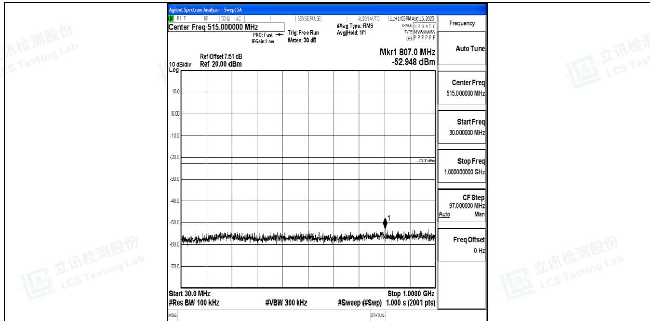
Band4_20MHz_16QAM_20175_1RB#0_30~1000_30~1000
