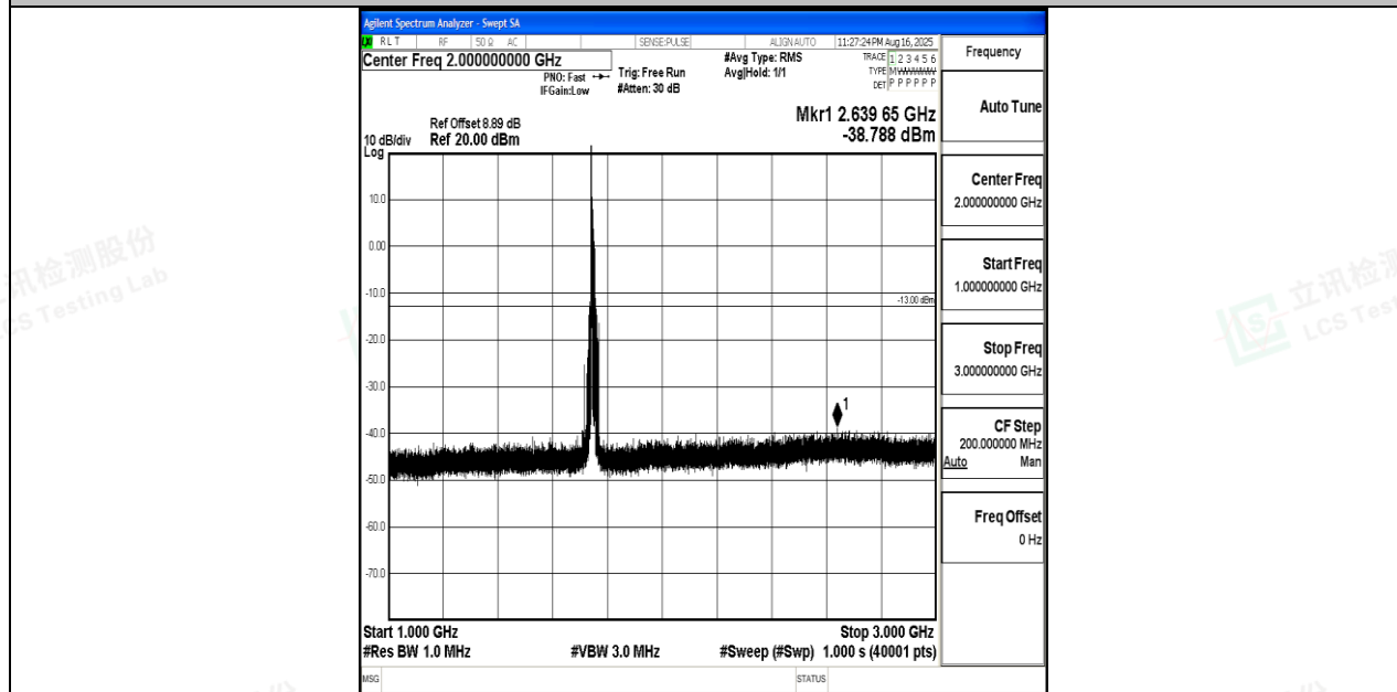
Band4_15MHz_16QAM_20325_1RB#0_1000~3000_1000~3000
