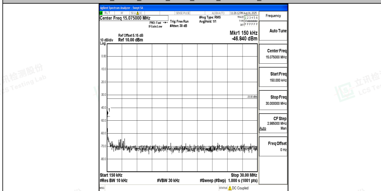
Band4_15MHz_16QAM_20175_1RB#0_0.15~30_0.15~30
