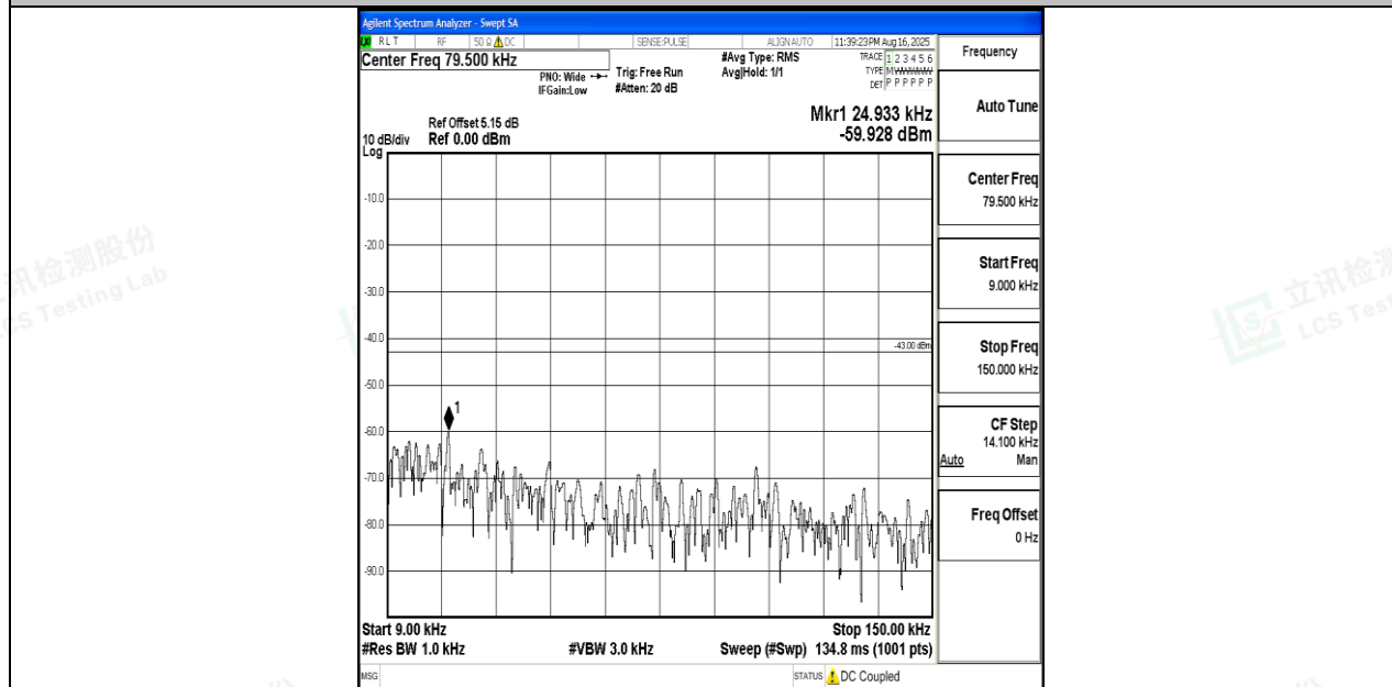
Band4_20MHz_QPSK_20050_1RB#0_0.009~0.15_0.009~0.15
