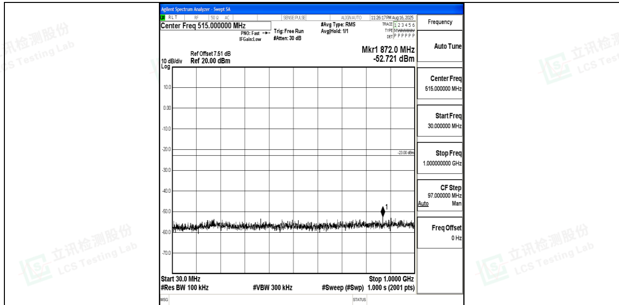
Band4_15MHz_16QAM_20175_1RB#0_30~1000_30~1000
