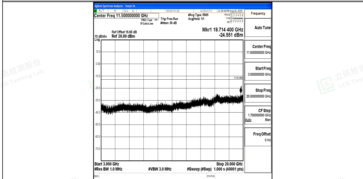
Band4_20MHz_QPSK_20050_1RB#0_3000~20000_3000~20000
