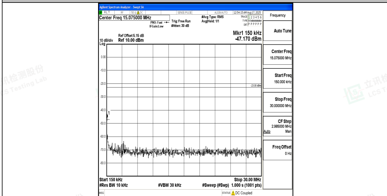
Band5_10MHz_QPSK_20450_1RB#0_0.15~30_0.15~30
