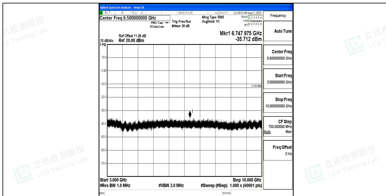
Band5_5MHz_QPSK_20625_1RB#0_3000~10000_3000~10000
