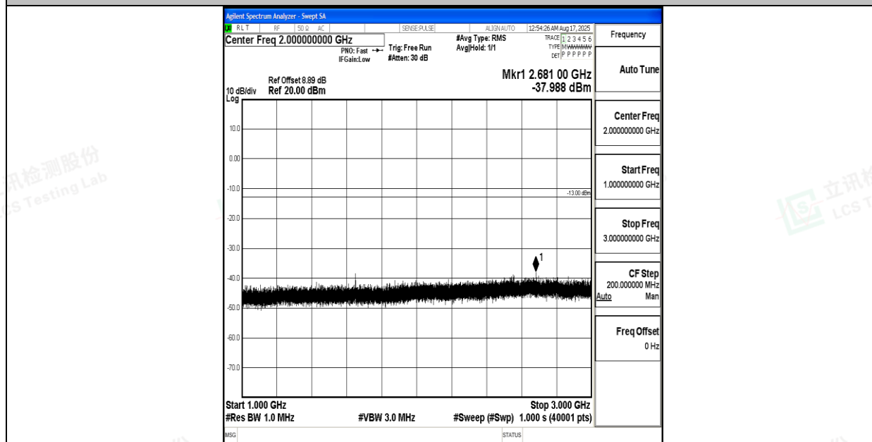
Band5_10MHz_QPSK_20450_1RB#0_1000~3000_1000~3000
