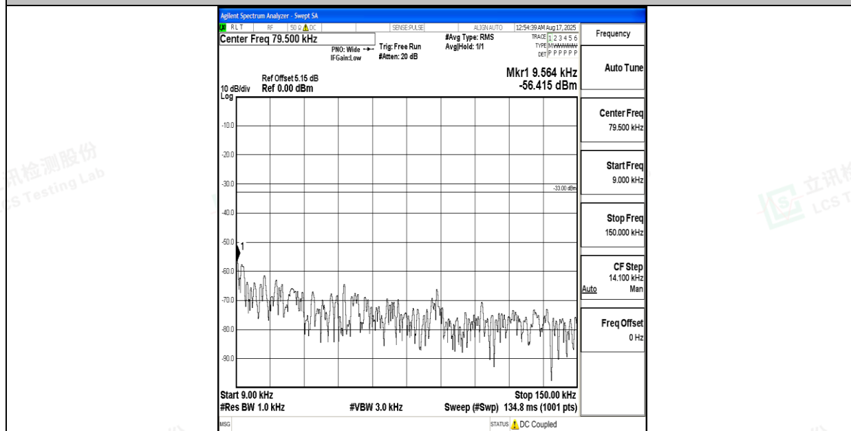
Band5_10MHz_16QAM_20450_1RB#0_0.009~0.15_0.009~0.15
