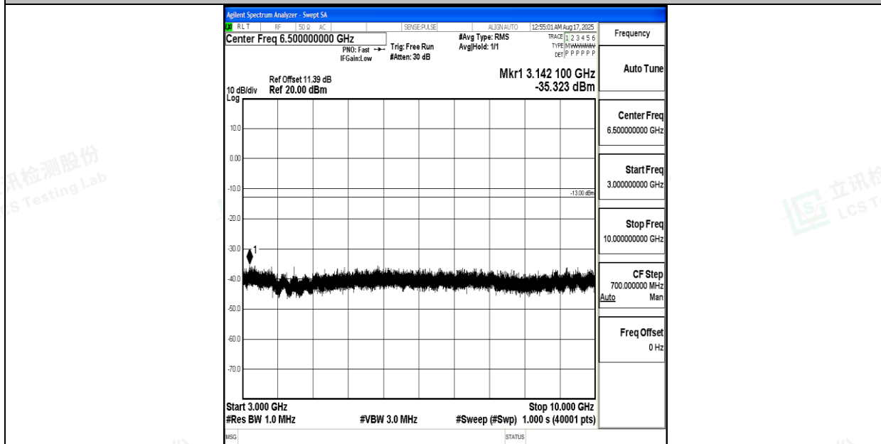
Band5_10MHz_16QAM_20450_1RB#0_3000~10000_3000~10000
