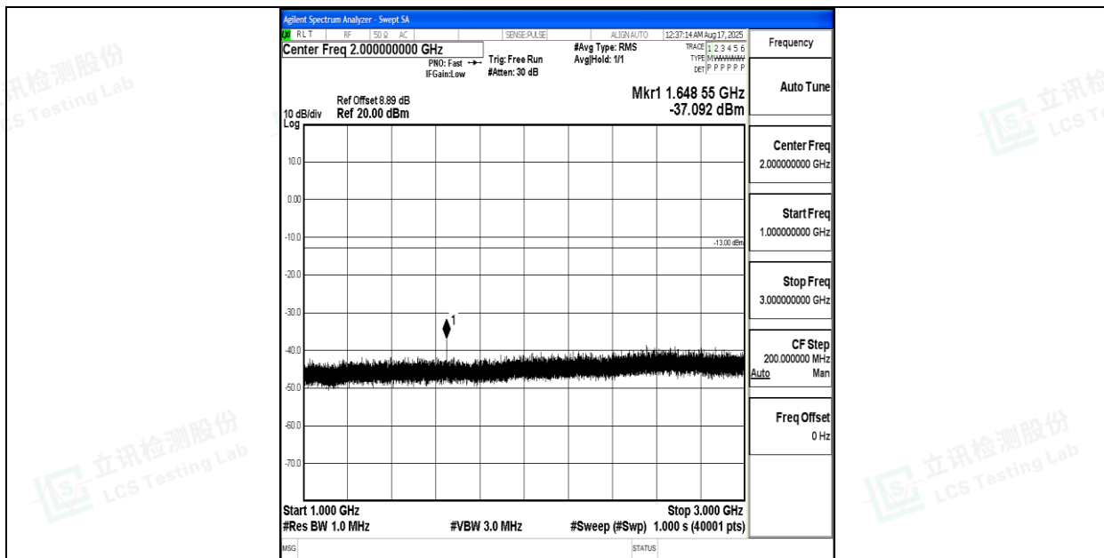
Band5_5MHz_16QAM_20425_1RB#0_1000~3000_1000~3000
