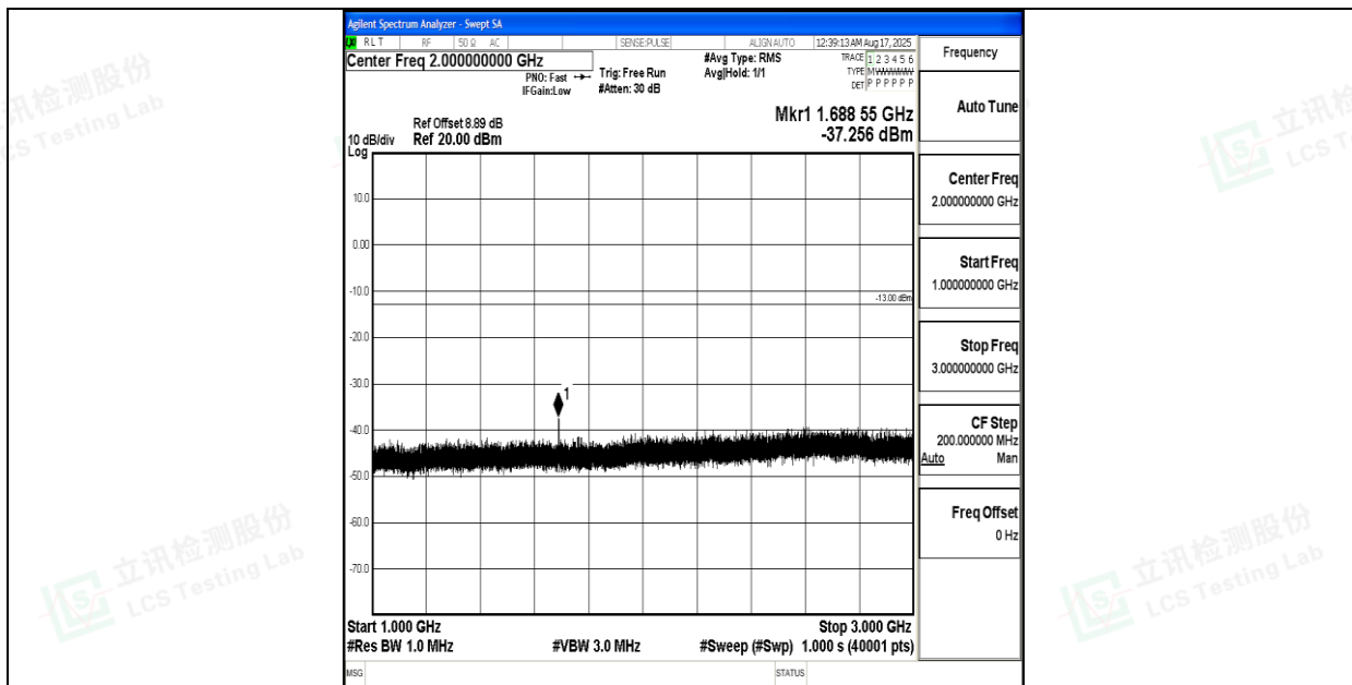
Band5_5MHz_16QAM_20625_1RB#0_1000~3000_1000~3000
