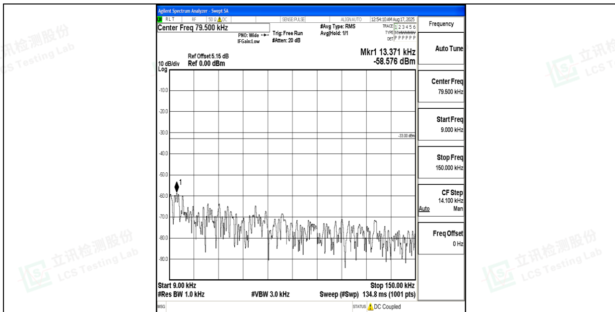
Band5_10MHz_QPSK_20450_1RB#0_0.009~0.15_0.009~0.15
