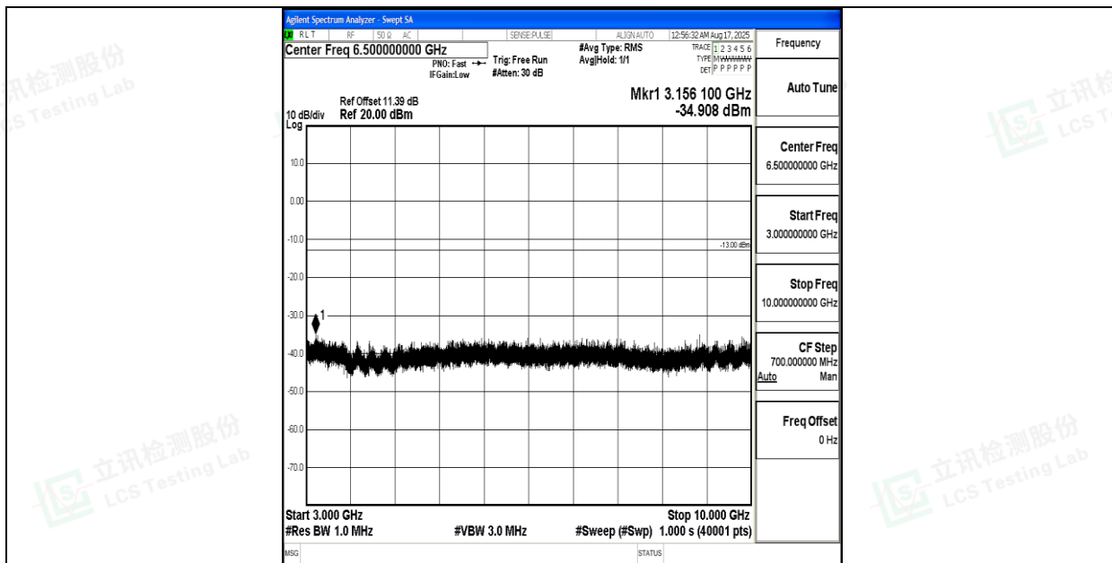
Band5_10MHz_QPSK_20600_1RB#0_3000~10000_3000~10000
