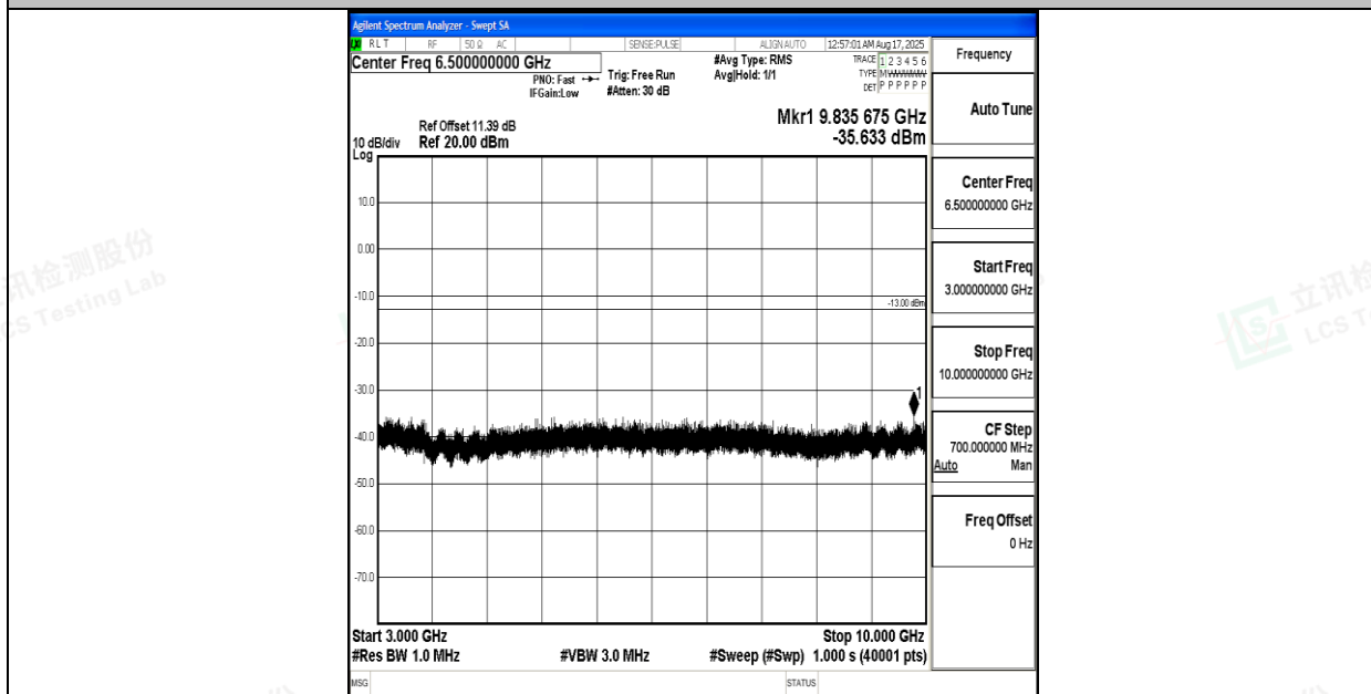
Band5_10MHz_16QAM_20600_1RB#0_3000~10000_3000~10000
