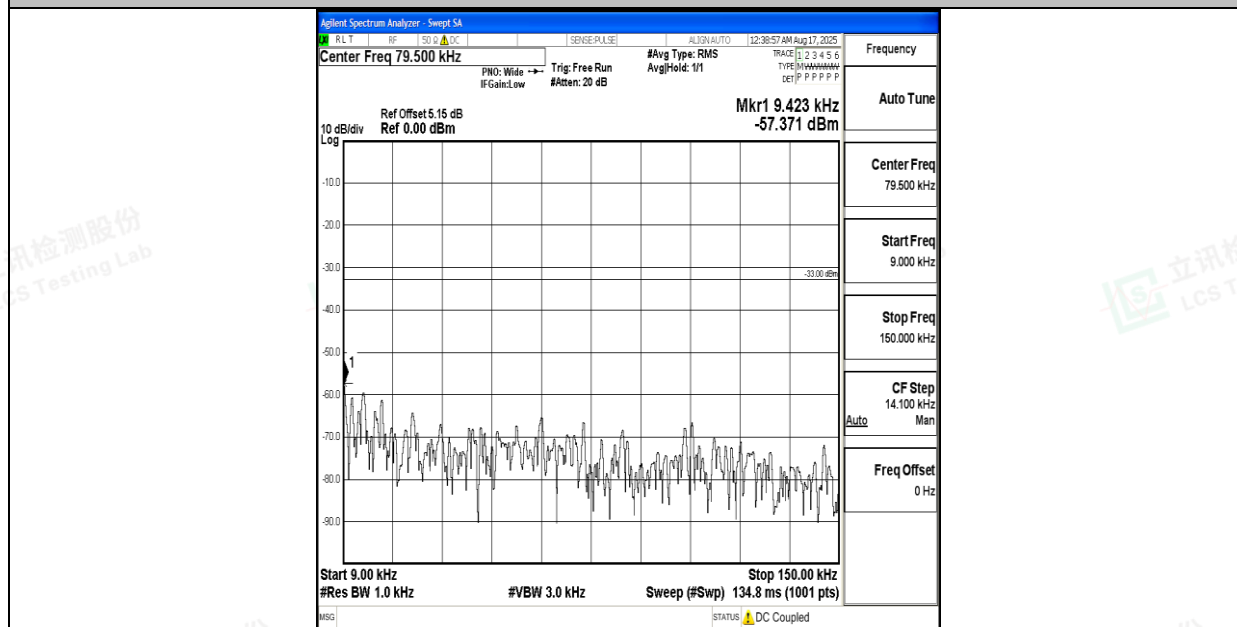
Band5_5MHz_16QAM_20625_1RB#0_0.009~0.15_0.009~0.15
