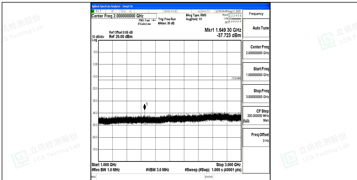
Band5_10MHz_16QAM_20450_1RB#0_1000~3000_1000~3000
