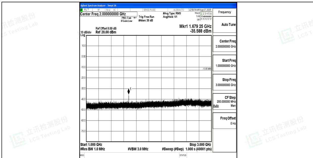
Band5_10MHz_16QAM_20600_1RB#0_1000~3000_1000~3000
