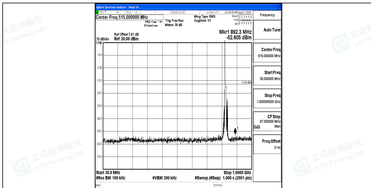
Band5_10MHz_QPSK_20450_1RB#0_30~1000_30~1000
