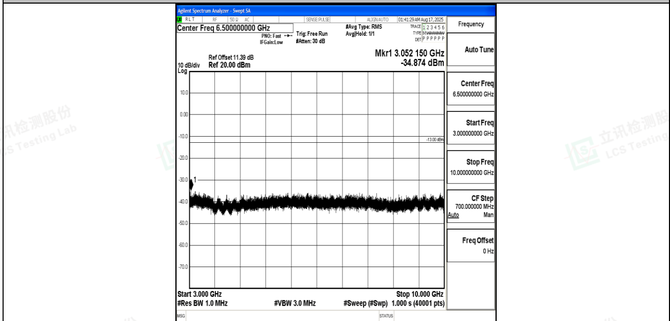
Band12_3MHz_16QAM_23165_1RB#0_3000~10000_3000~10000
