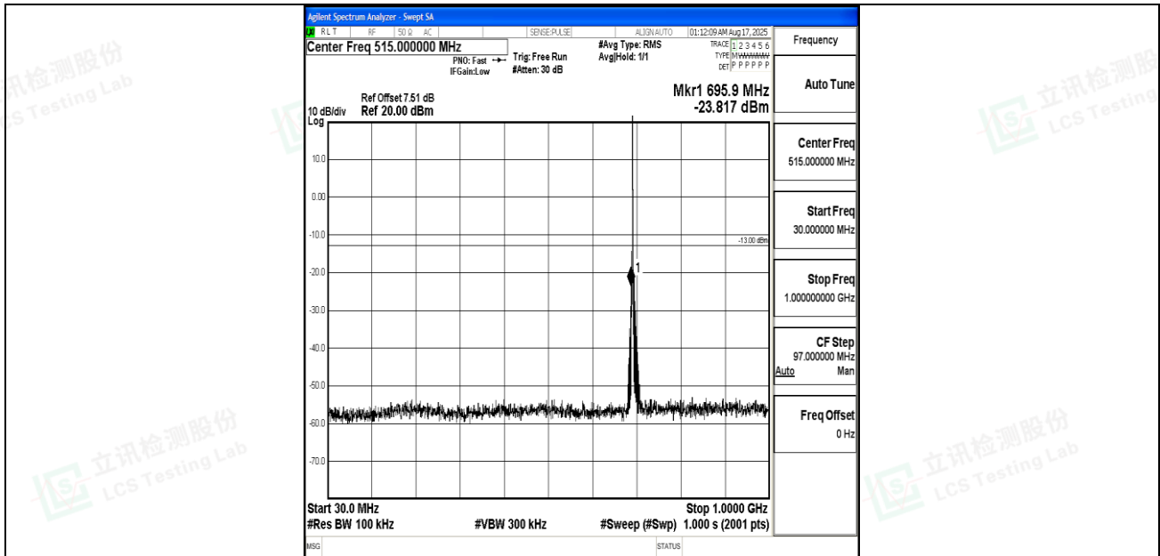
Band12_1.4MHz_QPSK_23017_1RB#0_30~1000_30~1000
