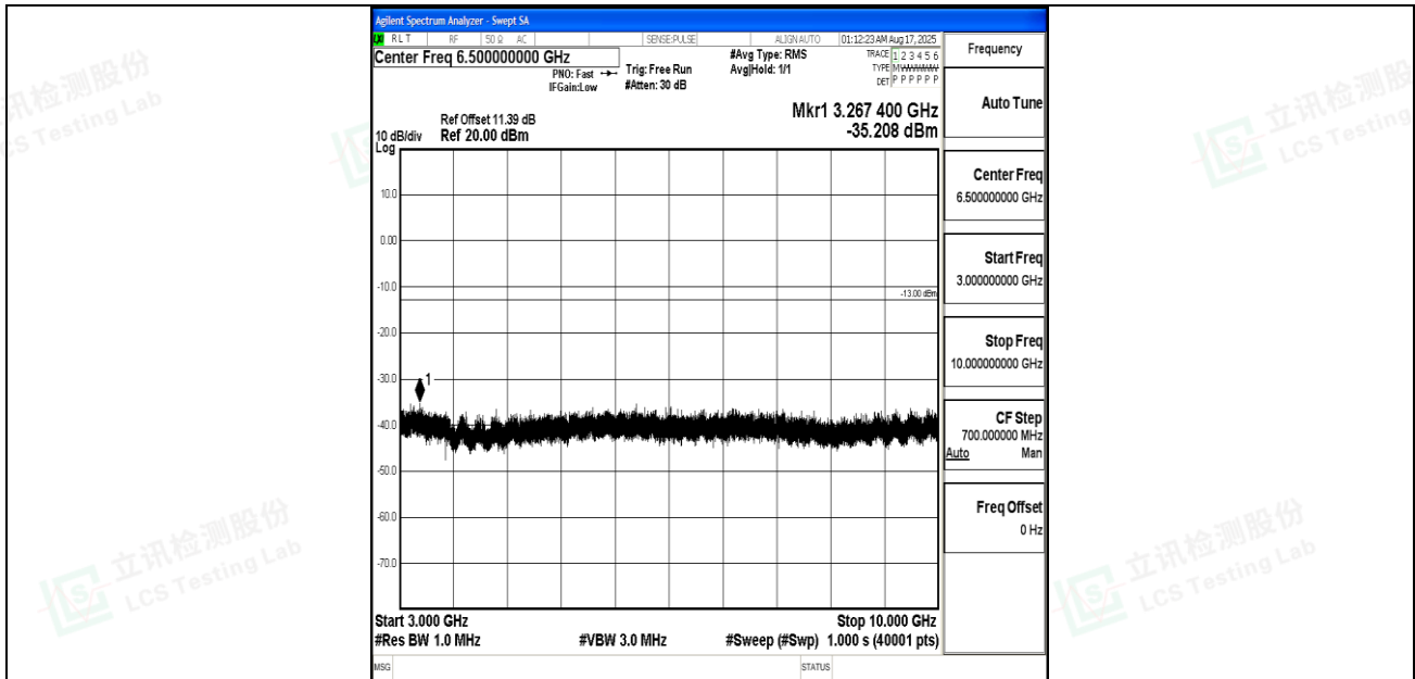
Band12_1.4MHz_QPSK_23017_1RB#0_3000~10000_3000~10000
