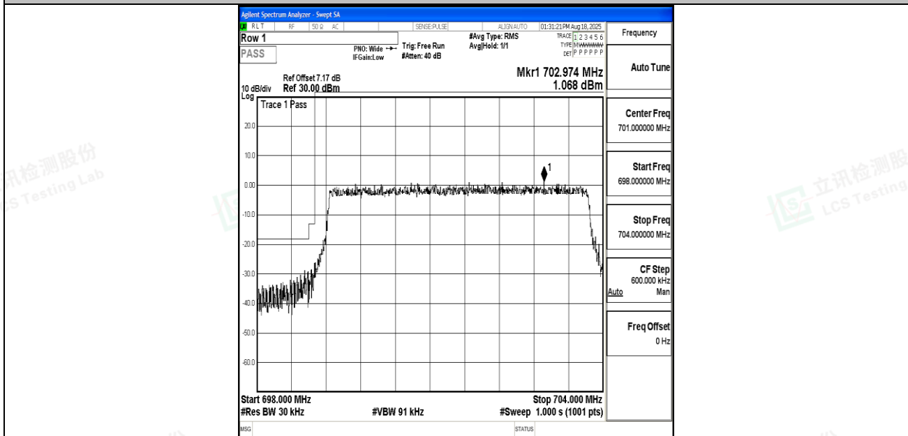
Band12_5MHz_16QAM_23035_25RB#0
