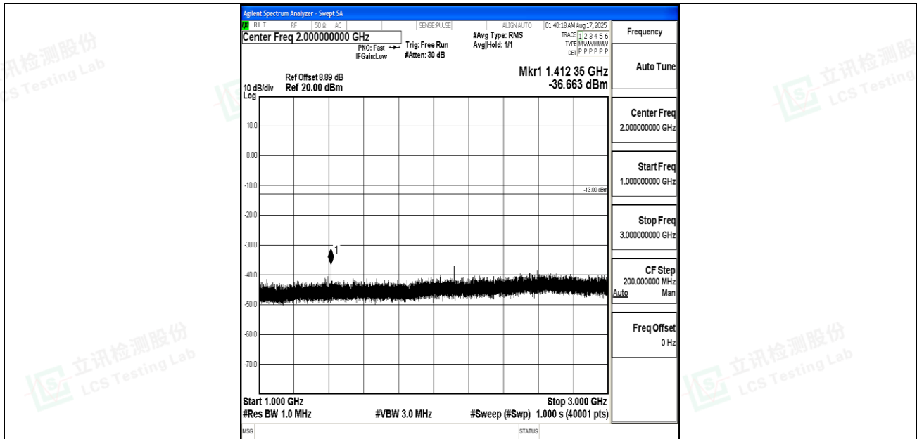
Band12_3MHz_16QAM_23095_1RB#0_1000~3000_1000~3000
