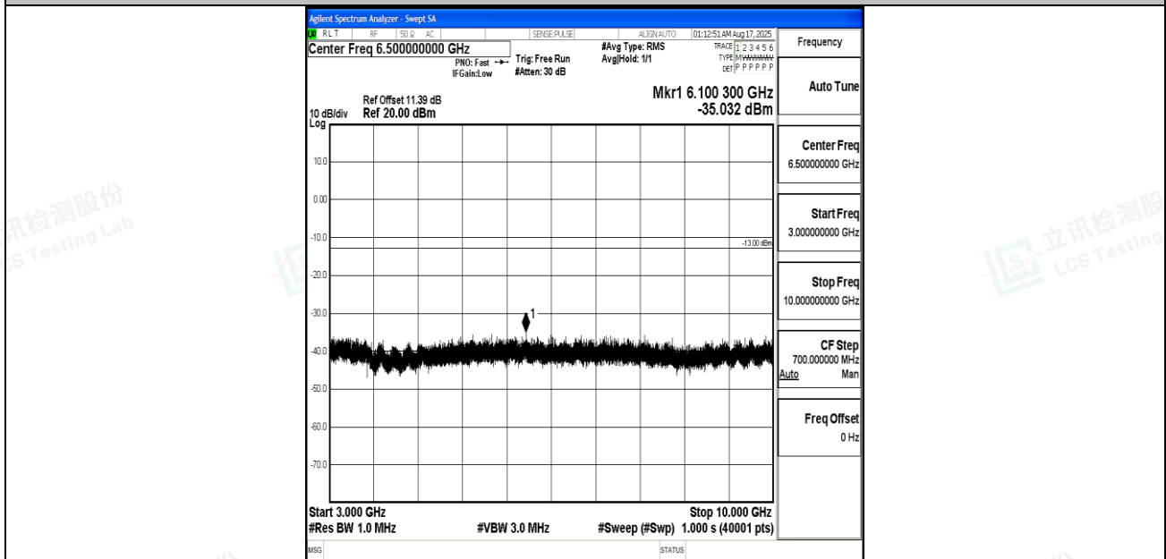
Band12_1.4MHz_16QAM_23017_1RB#0_3000~10000_3000~10000
