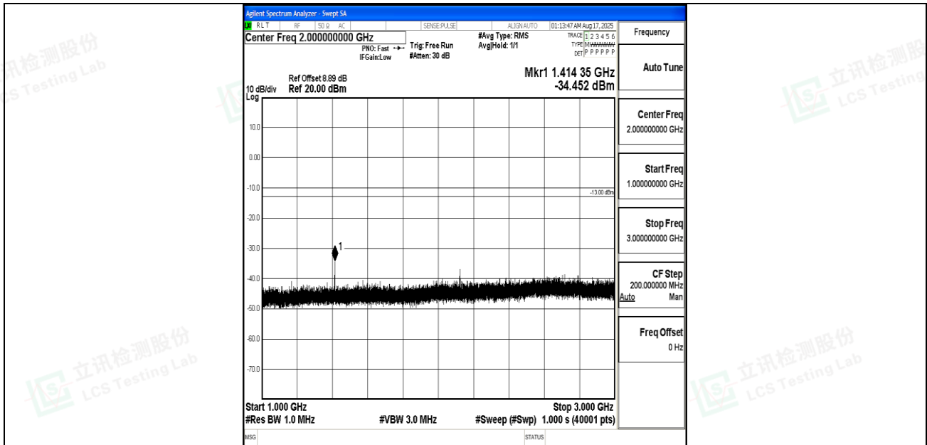
Band12_1.4MHz_16QAM_23095_1RB#0_1000~3000_1000~3000
