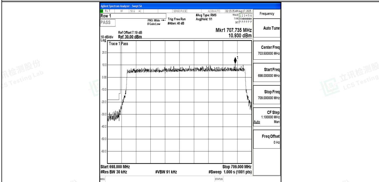
Band12_10MHz_16QAM_23060_50RB#0
