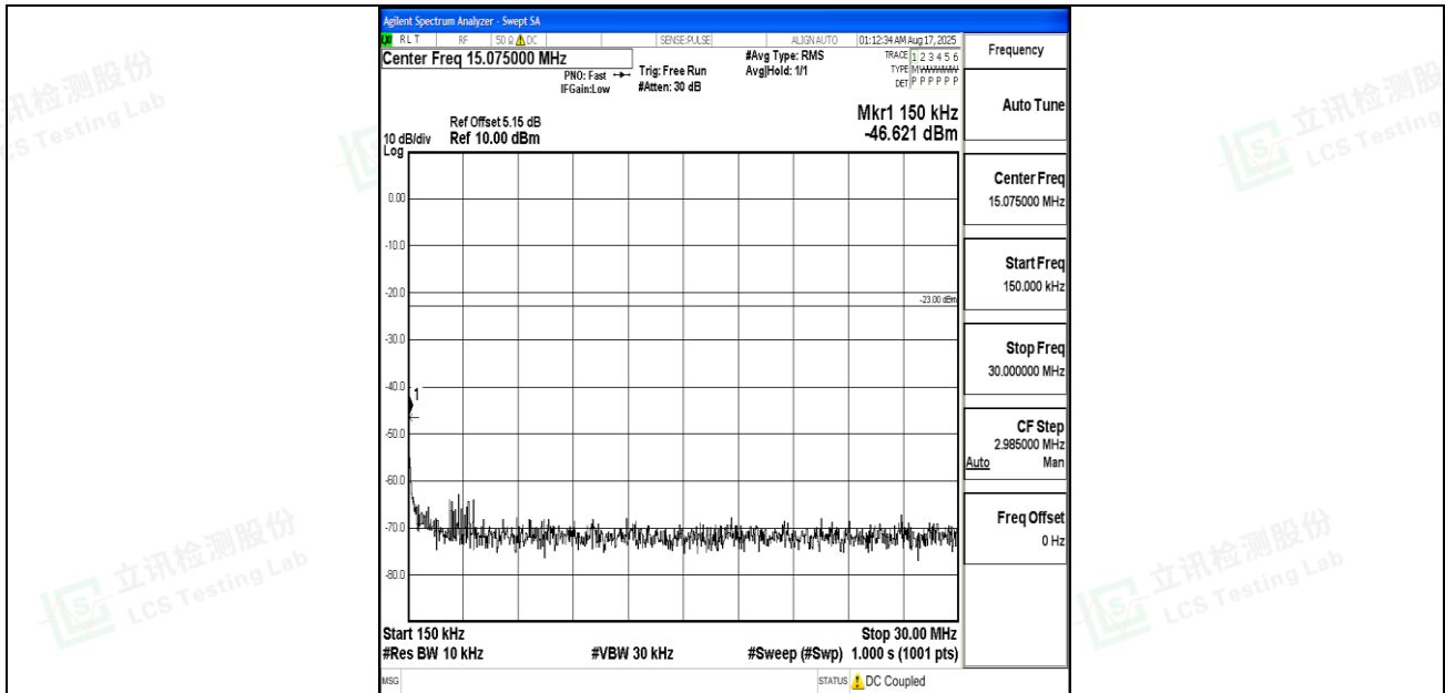
Band12_1.4MHz_16QAM_23017_1RB#0_0.15~30_0.15~30
