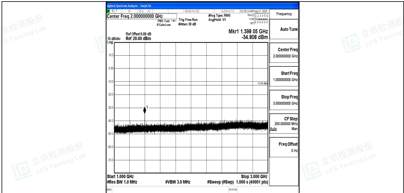
Band12_3MHz_16QAM_23025_1RB#0_1000~3000_1000~3000
