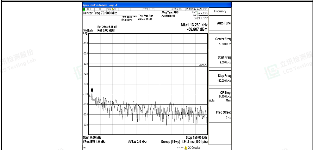
Band12_3MHz_16QAM_23095_1RB#0_0.009~0.15_0.009~0.15
