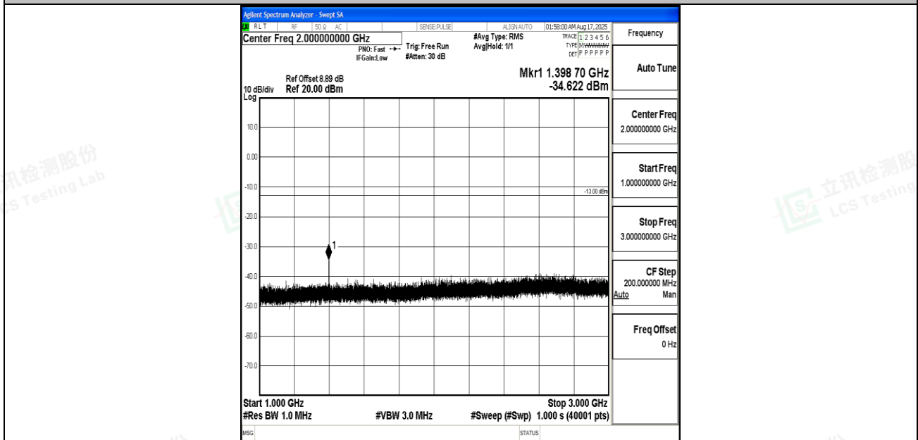
Band12_5MHz_QPSK_23035_1RB#0_1000~3000_1000~3000
