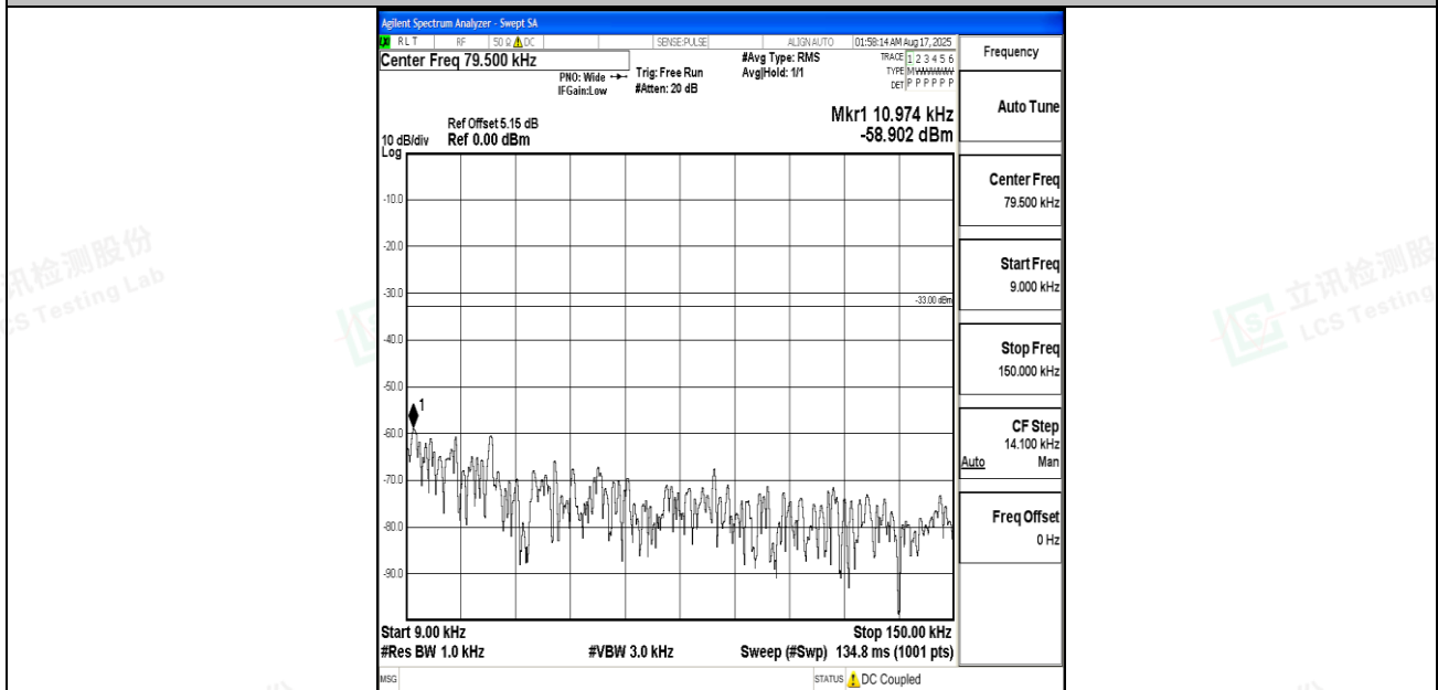
Band12_5MHz_16QAM_23035_1RB#0_0.009~0.15_0.009~0.15
