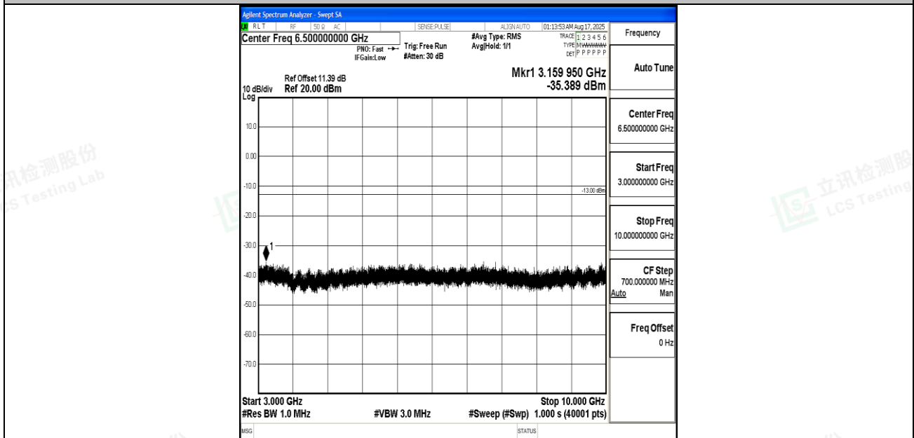
Band12_1.4MHz_16QAM_23095_1RB#0_3000~10000_3000~10000
