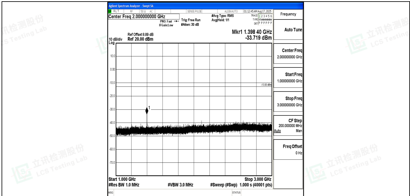
Band12_1.4MHz_16QAM_23017_1RB#0_1000~3000_1000~3000
