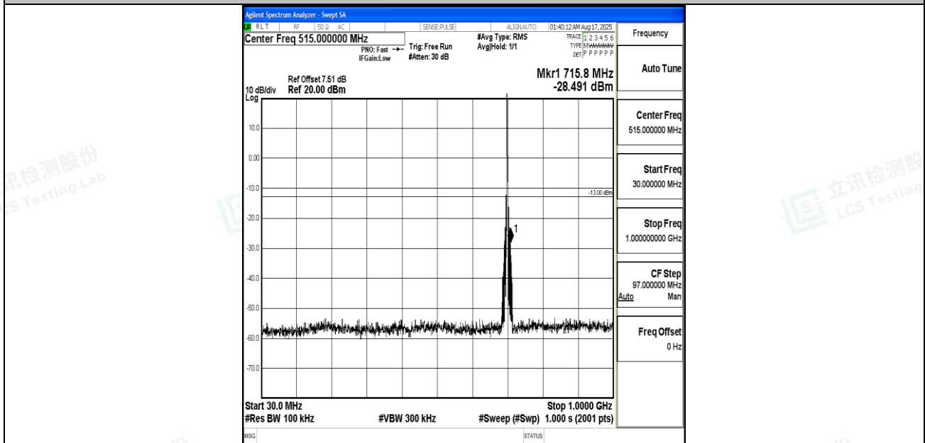
Band12_3MHz_16QAM_23095_1RB#0_30~1000_30~1000
