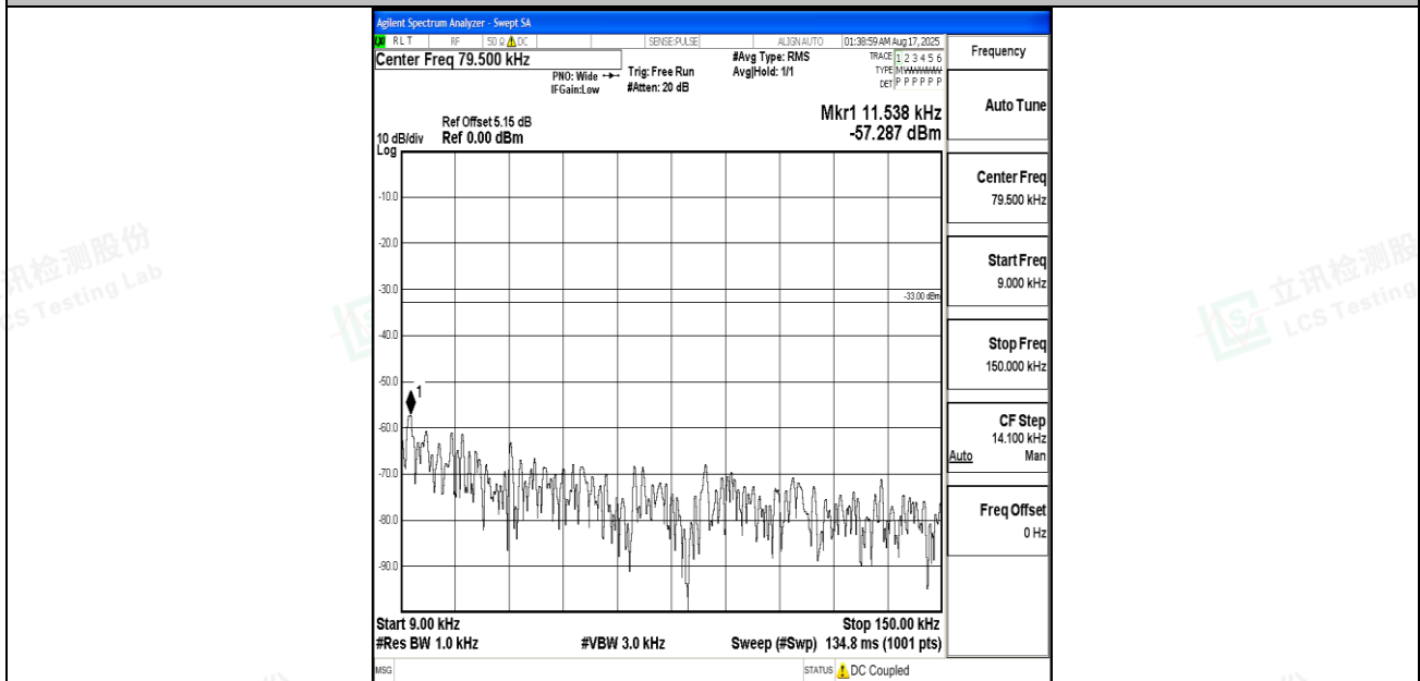
Band12_3MHz_16QAM_23025_1RB#0_0.009~0.15_0.009~0.15
