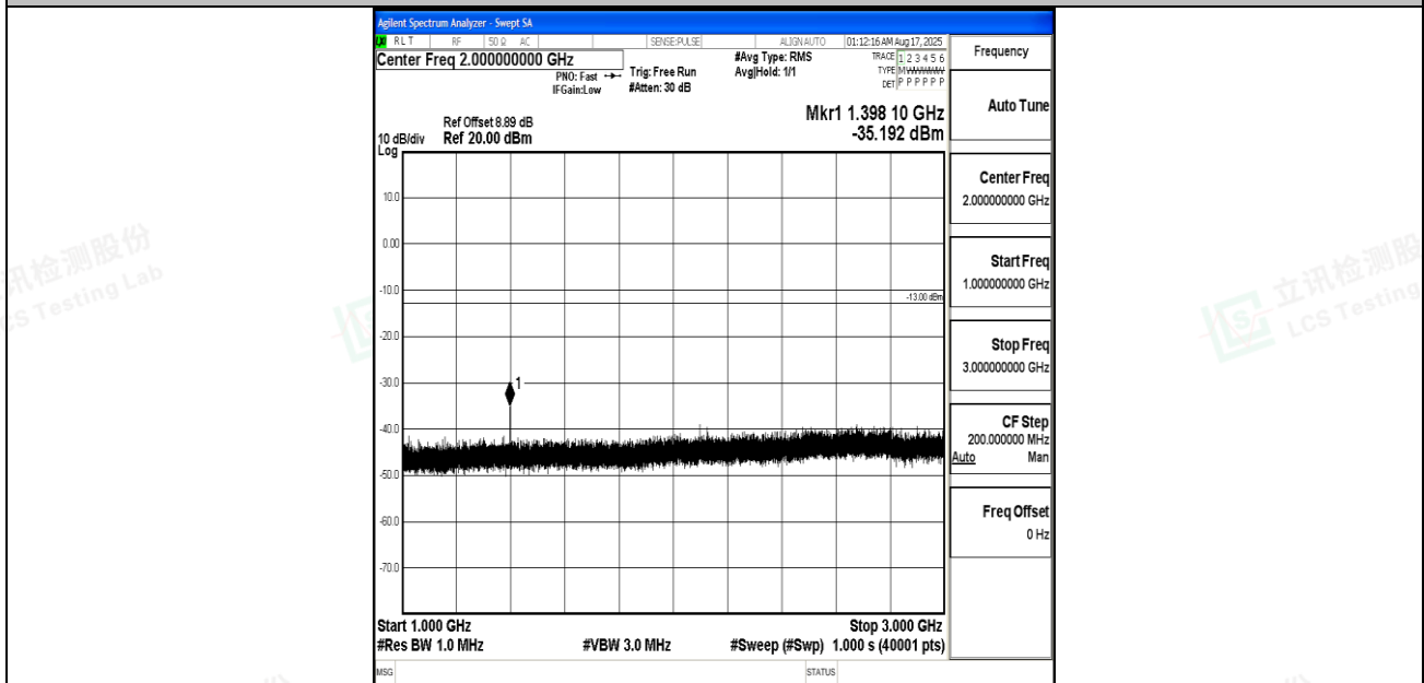
Band12_1.4MHz_QPSK_23017_1RB#0_1000~3000_1000~3000
