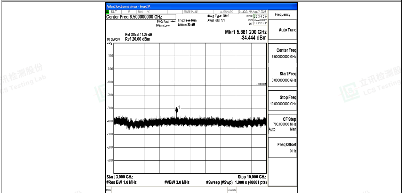
Band12_3MHz_16QAM_23025_1RB#0_3000~10000_3000~10000
