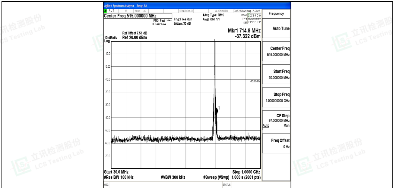
Band12_5MHz_QPSK_23035_1RB#0_30~1000_30~1000
