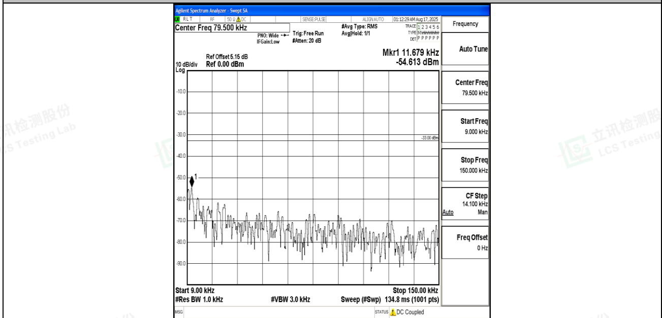
Band12_1.4MHz_16QAM_23017_1RB#0_0.009~0.15_0.009~0.15
