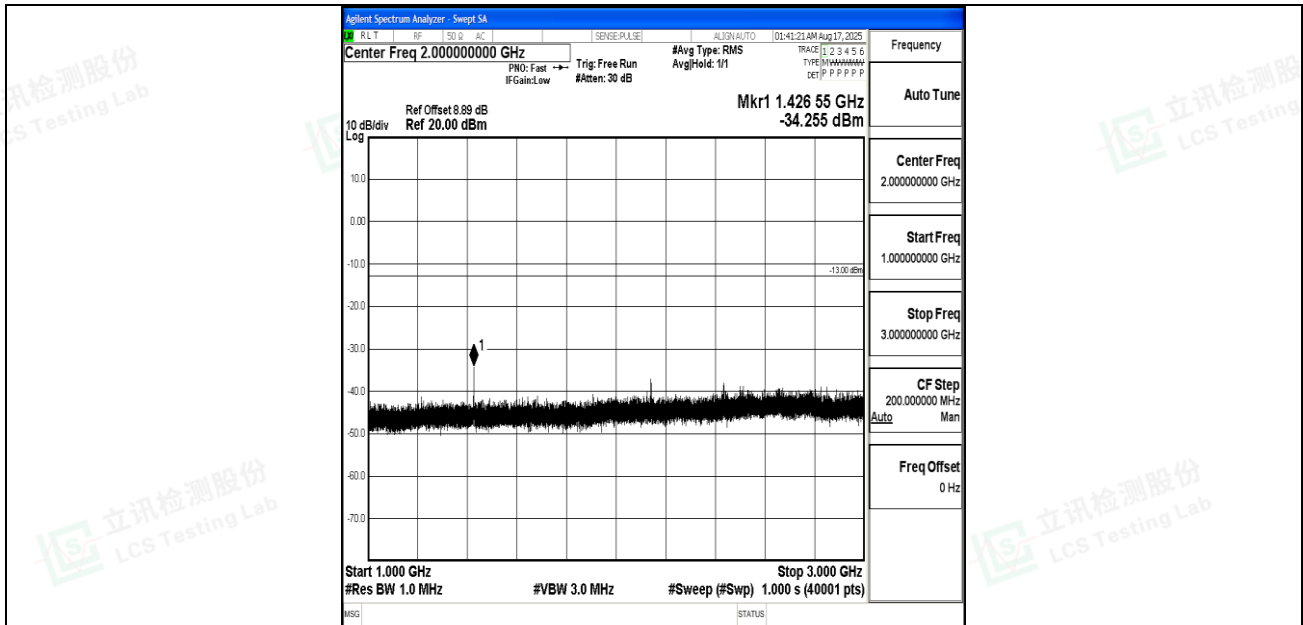
Band12_3MHz_16QAM_23165_1RB#0_1000~3000_1000~3000
