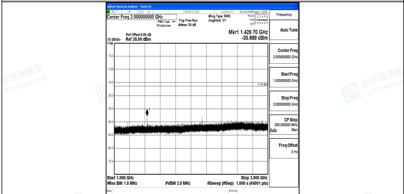
Band12_1.4MHz_QPSK_23173_1RB#0_1000~3000_1000~3000
