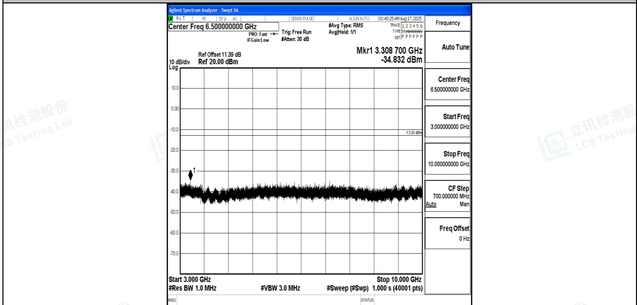
Band12_3MHz_16QAM_23095_1RB#0_3000~10000_3000~10000
