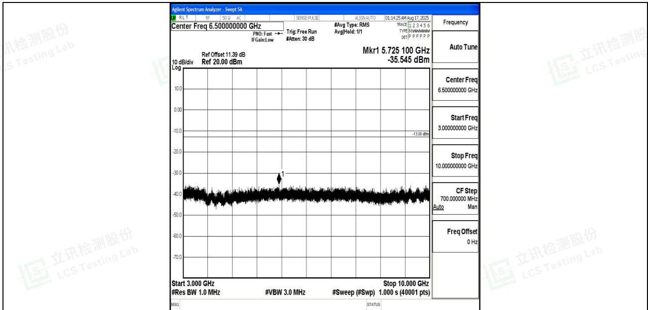
Band12_1.4MHz_QPSK_23173_1RB#0_3000~10000_3000~10000
