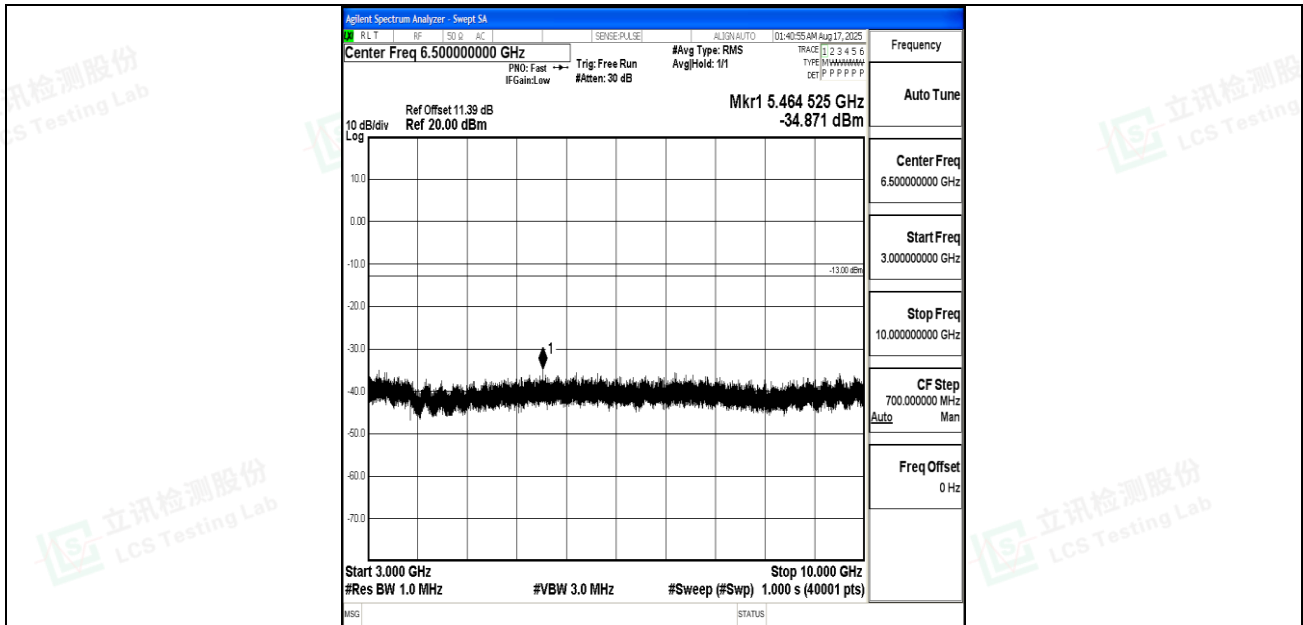
Band12_3MHz_QPSK_23165_1RB#0_3000~10000_3000~10000
