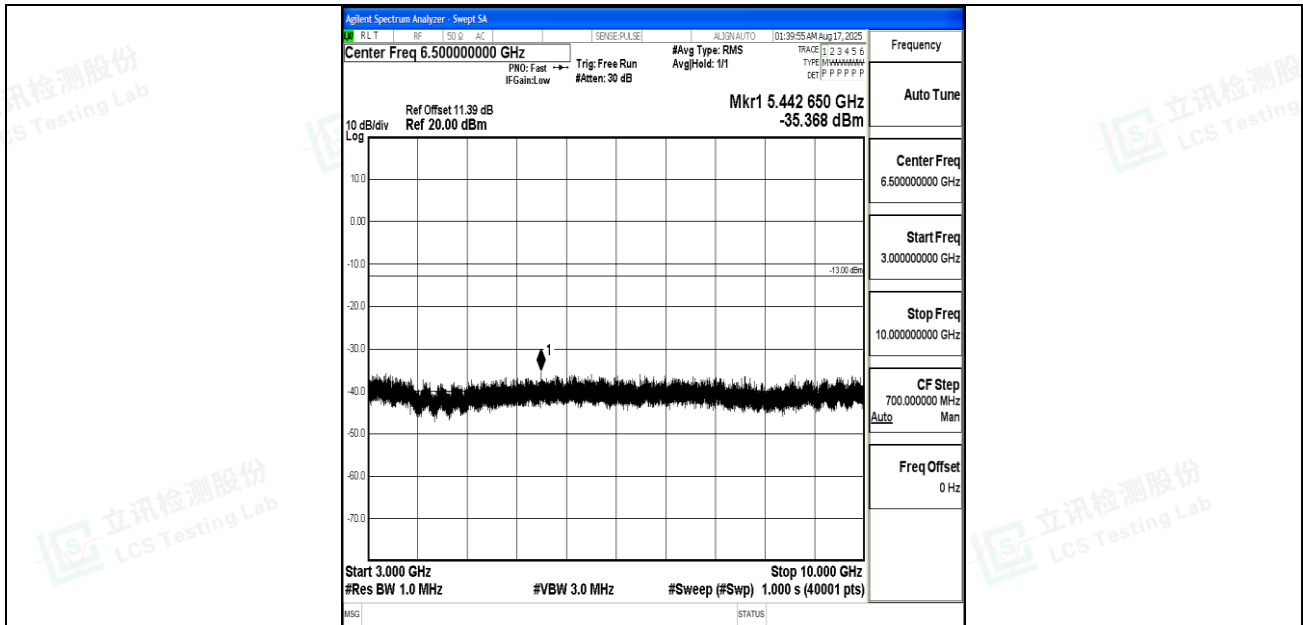
Band12_3MHz_QPSK_23095_1RB#0_3000~10000_3000~10000
