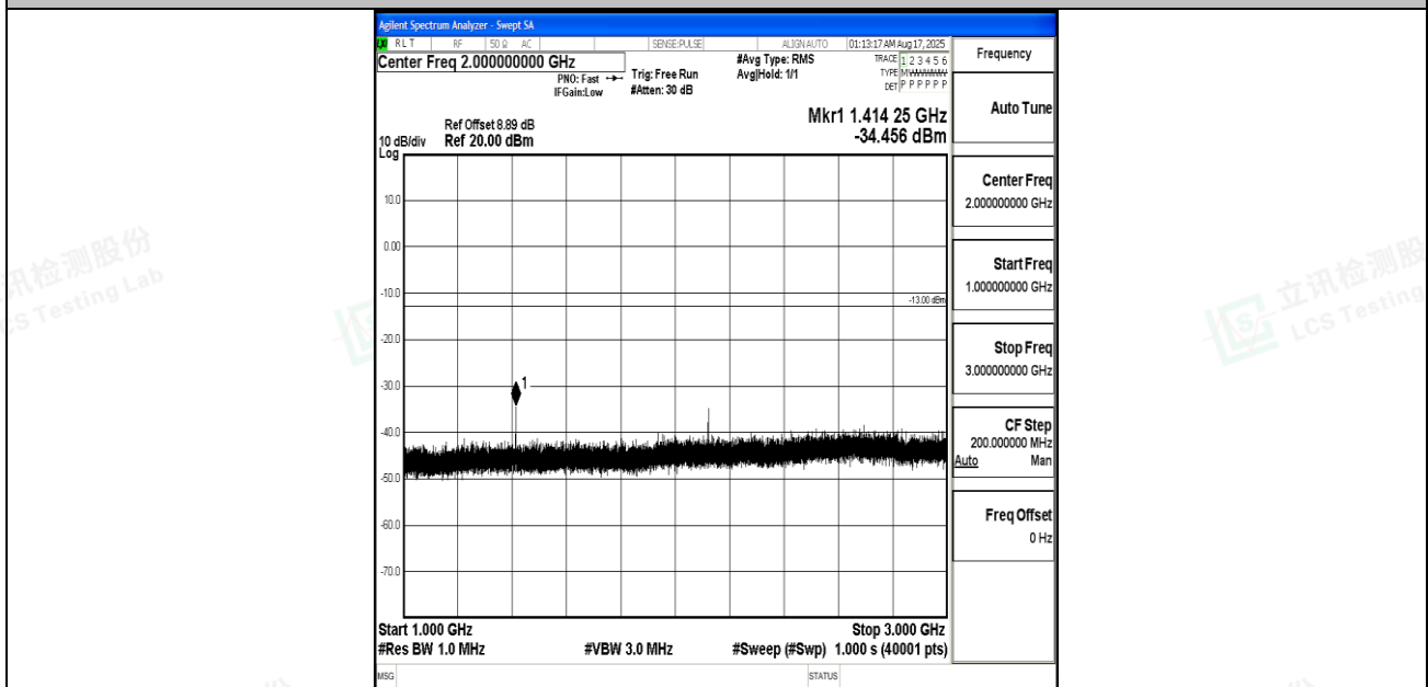
Band12_1.4MHz_QPSK_23095_1RB#0_1000~3000_1000~3000
