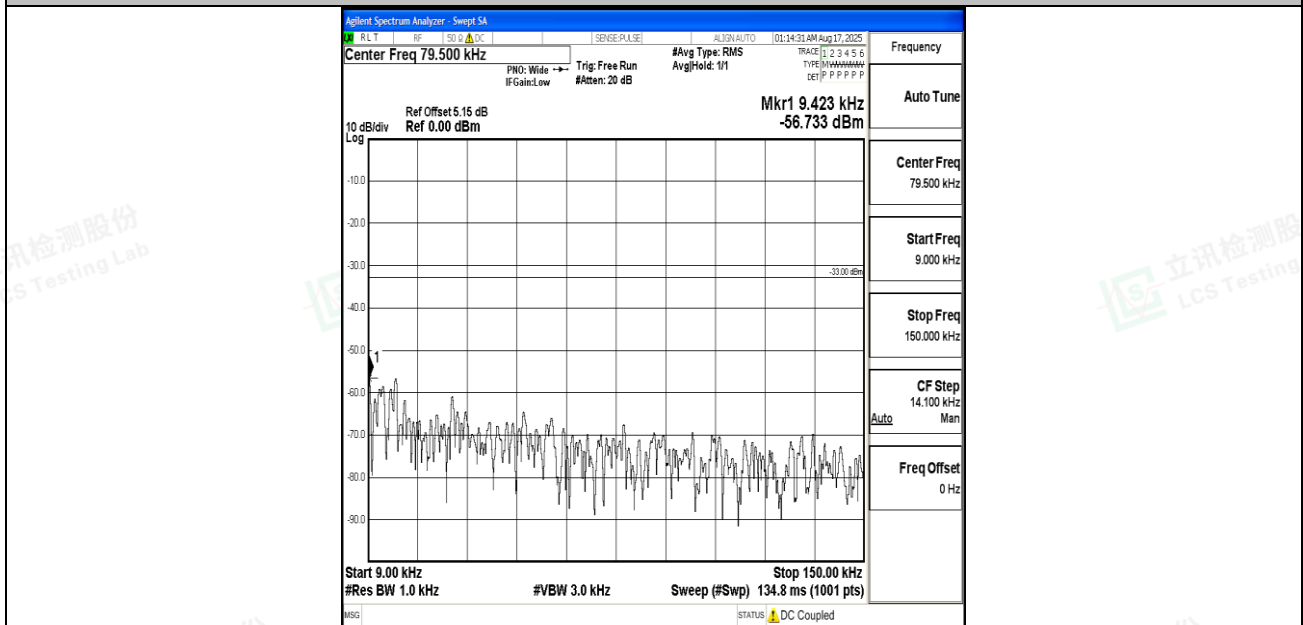
Band12_1.4MHz_16QAM_23173_1RB#0_0.009~0.15_0.009~0.15
