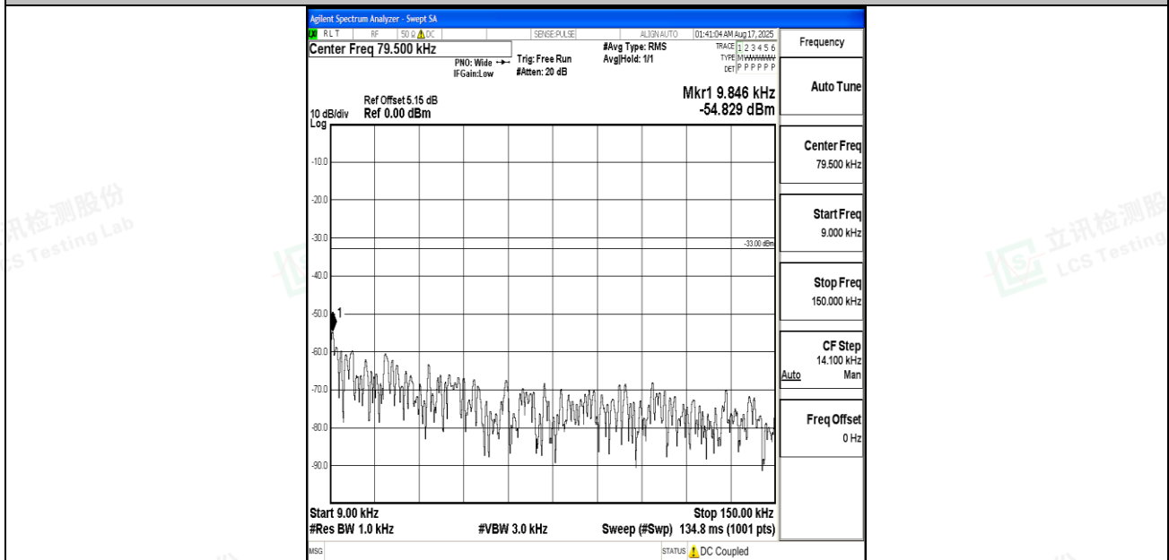
Band12_3MHz_16QAM_23165_1RB#0_0.009~0.15_0.009~0.15
