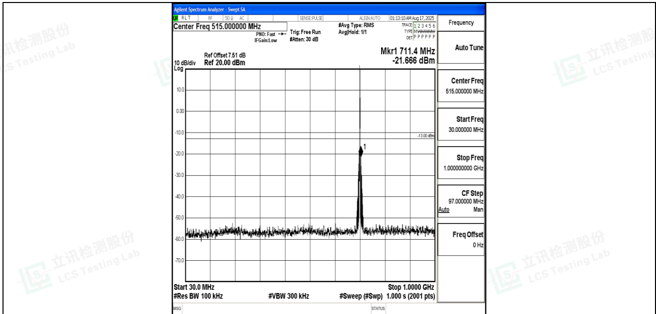
Band12_1.4MHz_QPSK_23095_1RB#0_30~1000_30~1000
