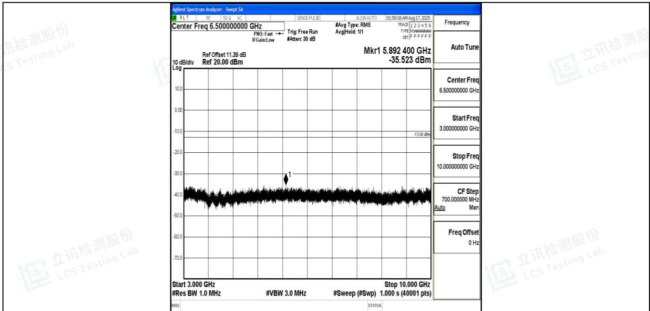
Band12_5MHz_QPSK_23035_1RB#0_3000~10000_3000~10000
