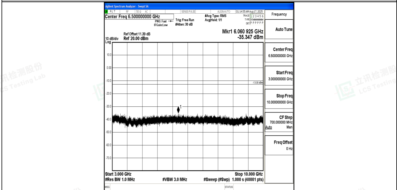
Band12_1.4MHz_16QAM_23173_1RB#0_3000~10000_3000~10000
