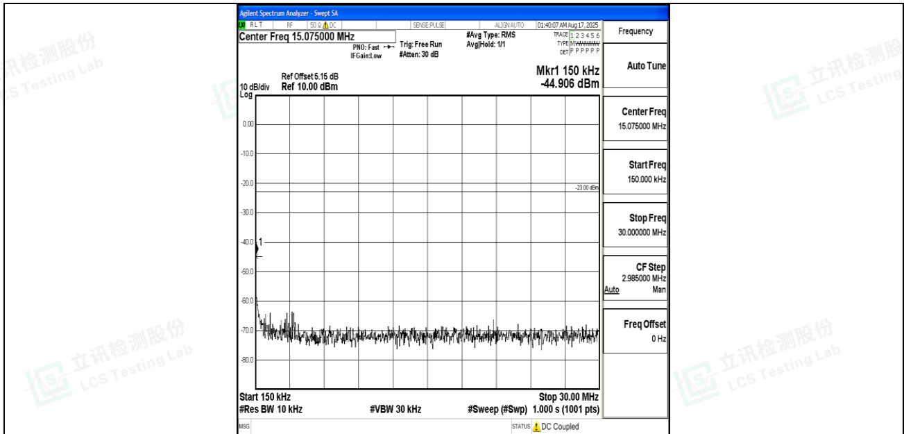
Band12_3MHz_16QAM_23095_1RB#0_0.15~30_0.15~30
