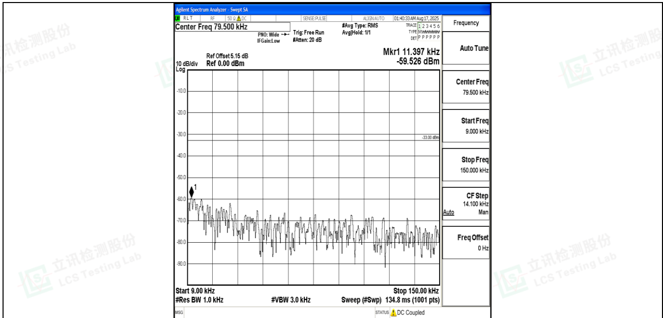
Band12_3MHz_QPSK_23165_1RB#0_0.009~0.15_0.009~0.15
