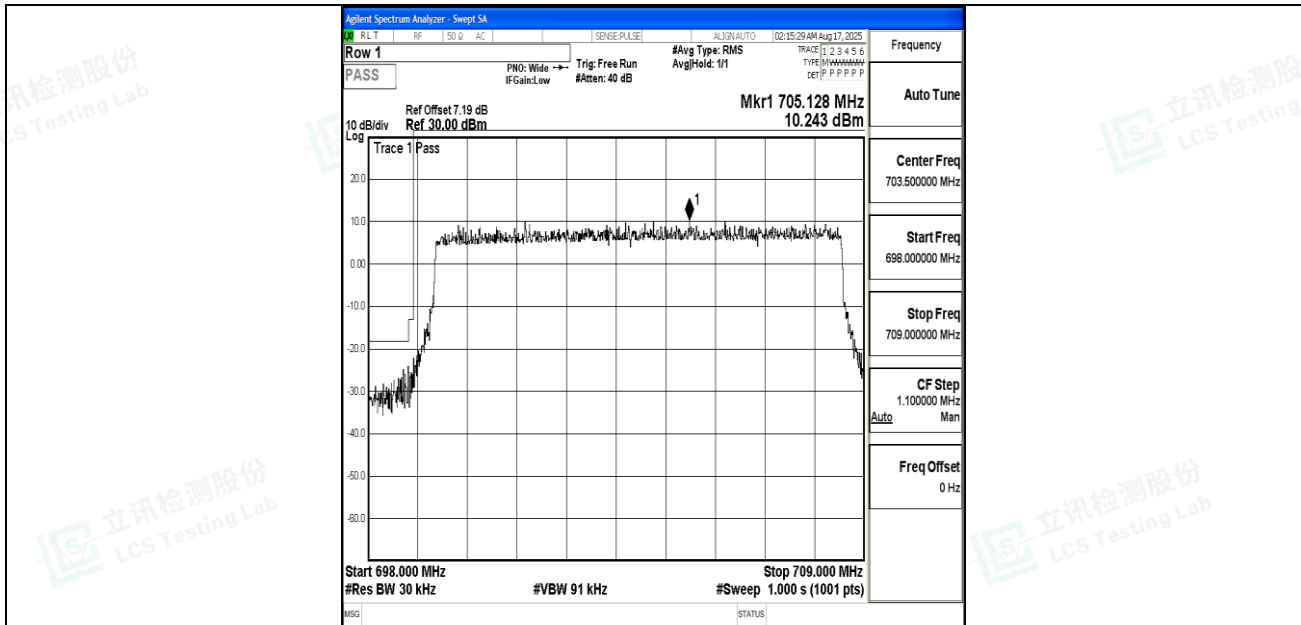
Band12_10MHz_QPSK_23060_50RB#0
