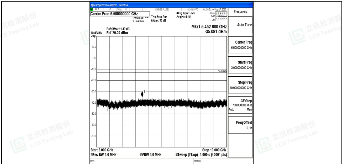
Band12_3MHz_QPSK_23025_1RB#0_3000~10000_3000~10000
