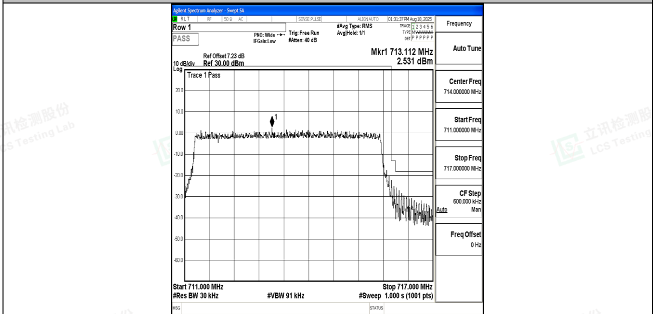
Band12_5MHz_16QAM_23155_25RB#0
